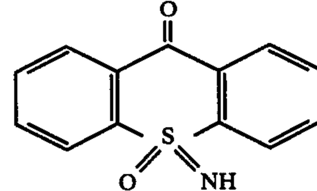
Phenoxathiine-S-oximide:
