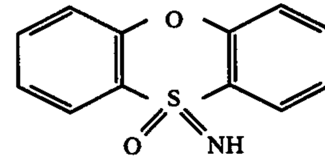
Thianthrene-S-oximide:
