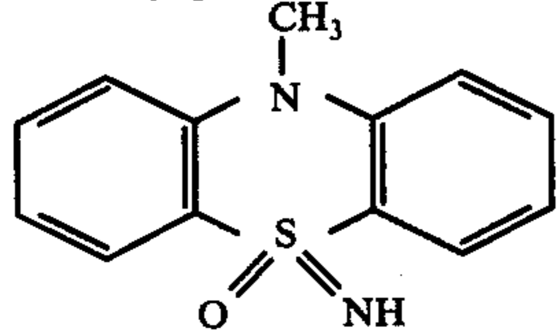
10-acetyl-phenothiazine-S-oximide:
