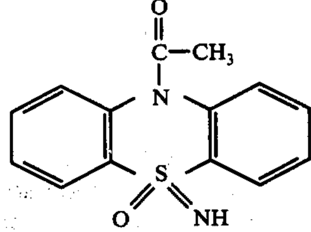
Phenothiazine-S-oximide:
