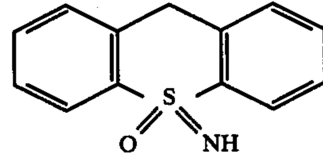
Thioxanthone-S-oximide:
