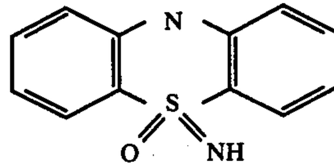
Dibenzothiophene-S-oximide:
