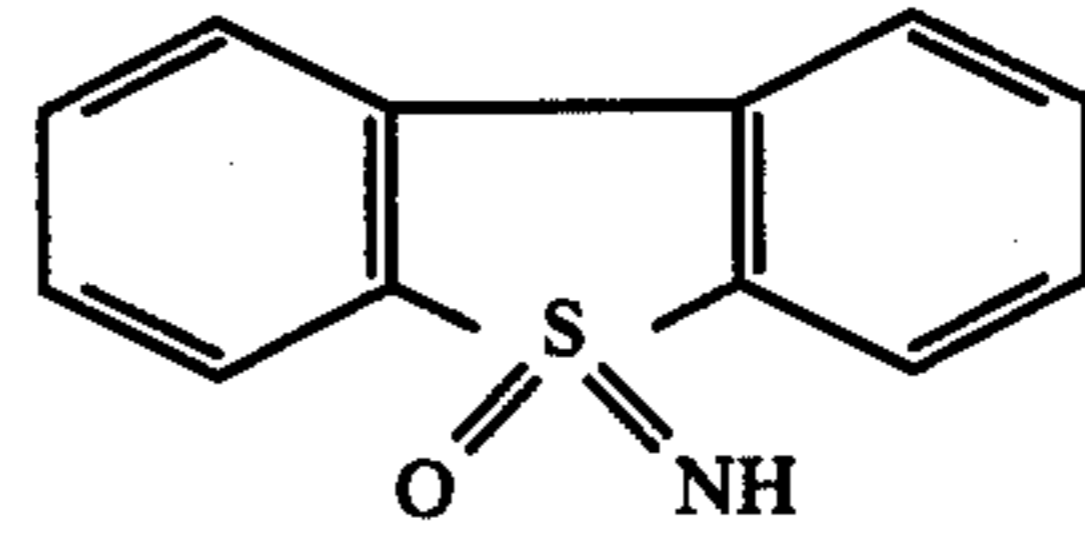
Thioxanthene-S-oximide:
