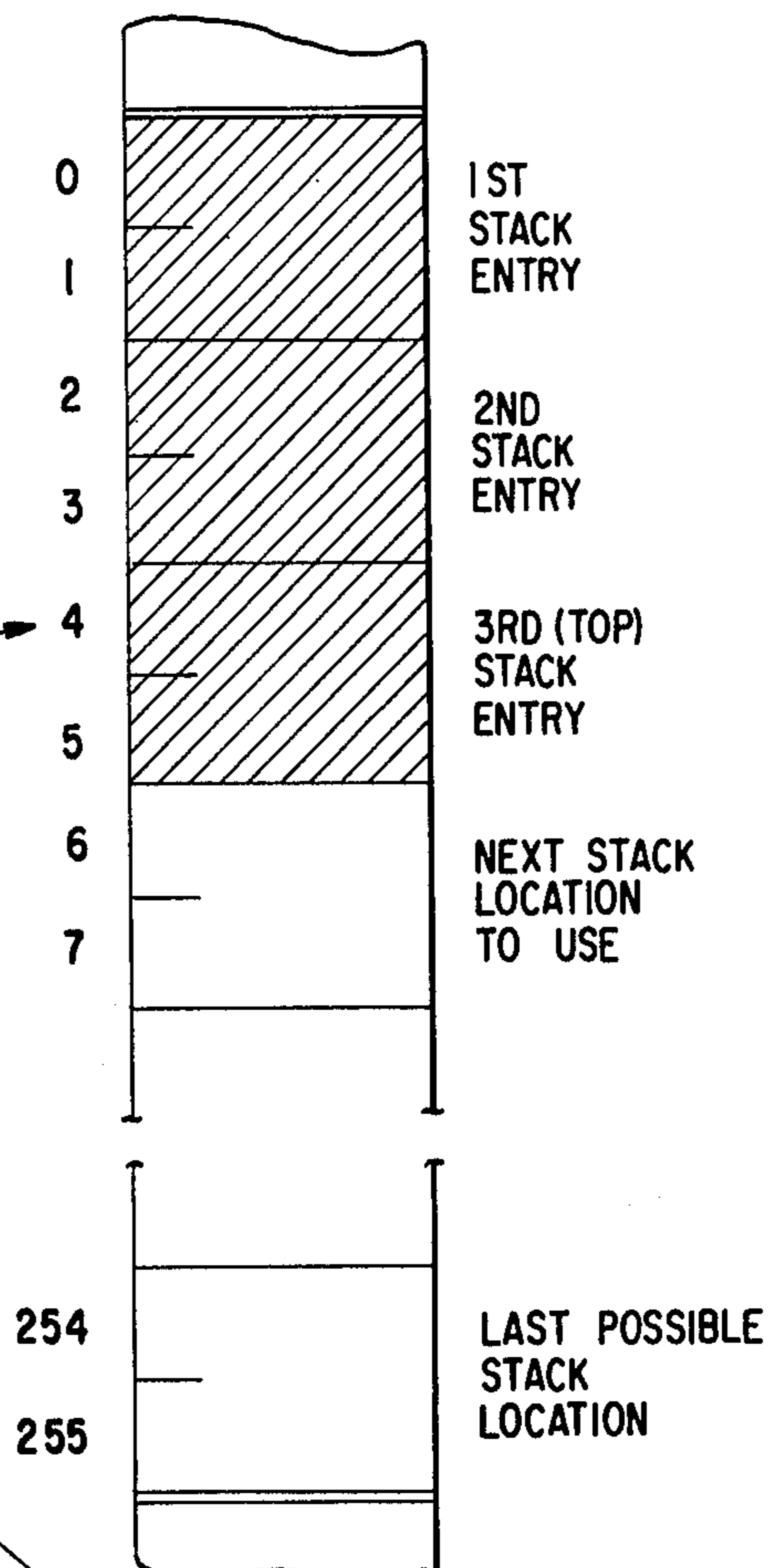
ONE MEMORY PAGE (256 8-BIT BYTES)
