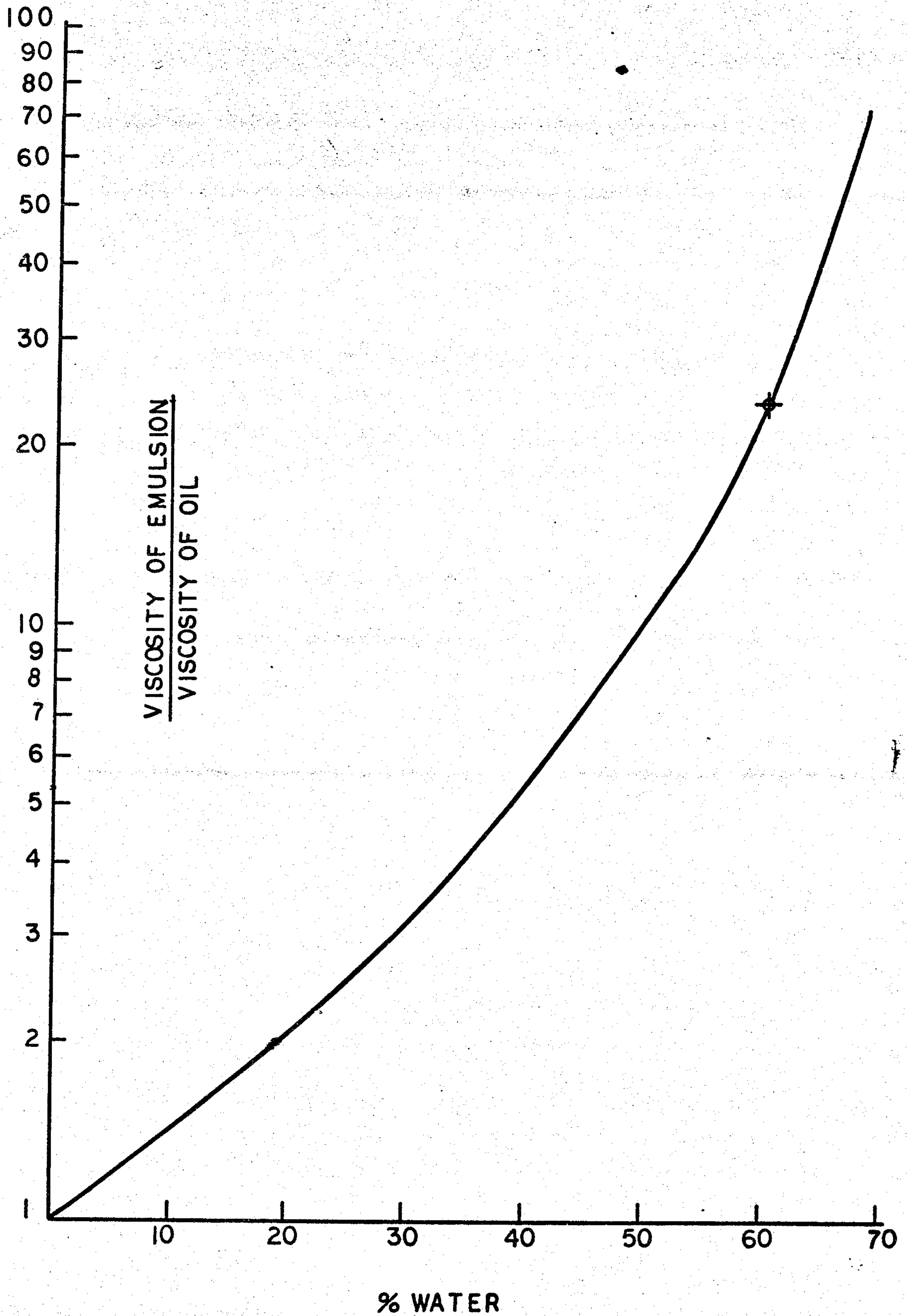
fig. 1 (PRIOR ART)
