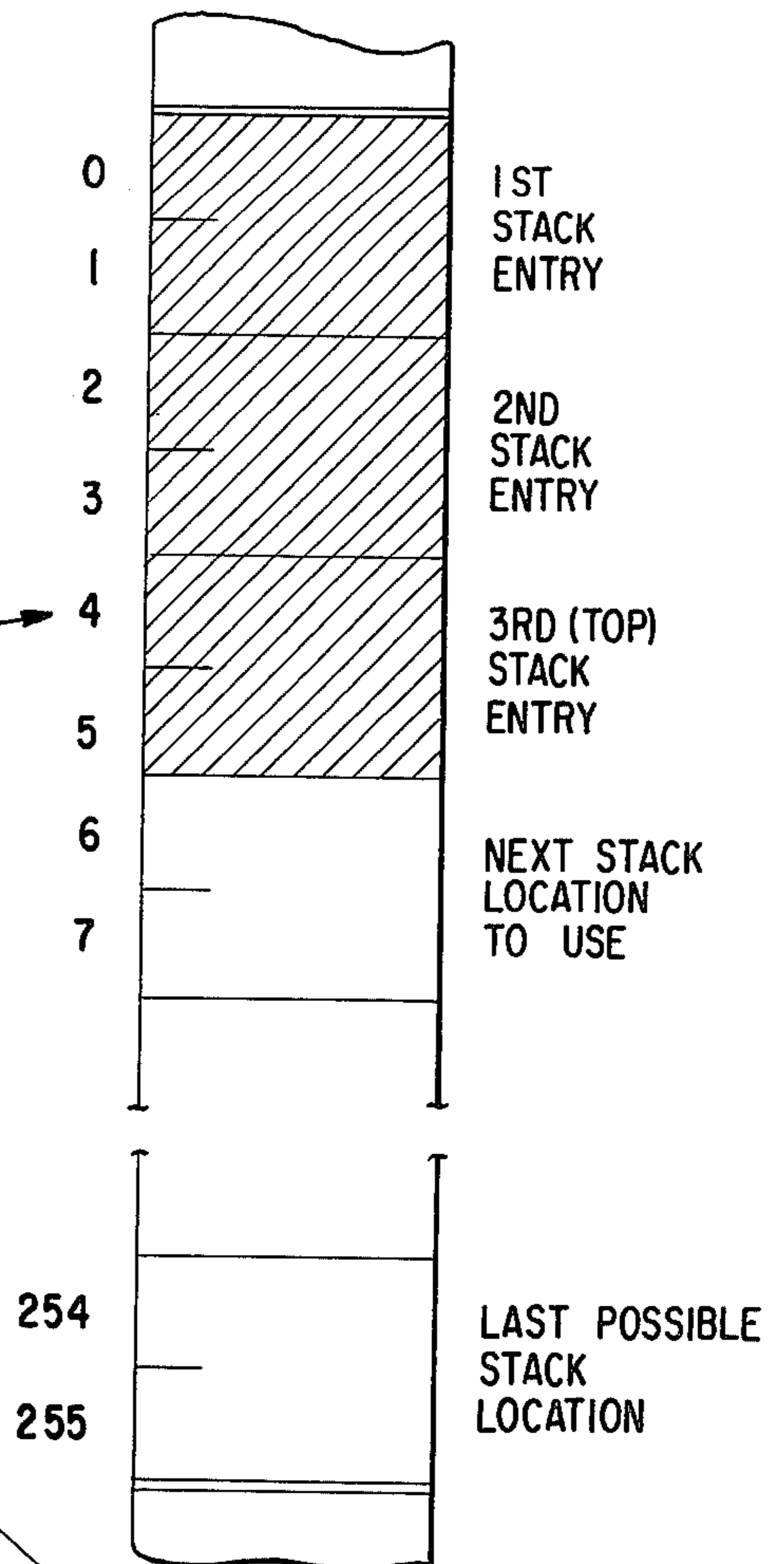
ONE MEMORY PAGE (256 8-BIT BYTES)
