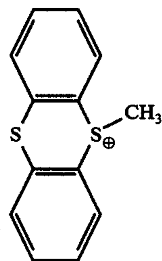
(5-methylthianthrenium hexafluorophosphate)
