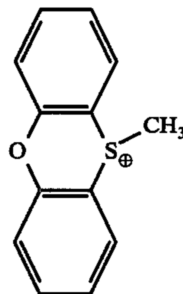
(10-methylphenoxythiinium hexafluorophosphate)
