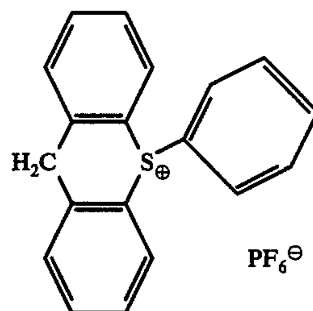
(10-phenylthioxanthenium hexafluorophosphate)
