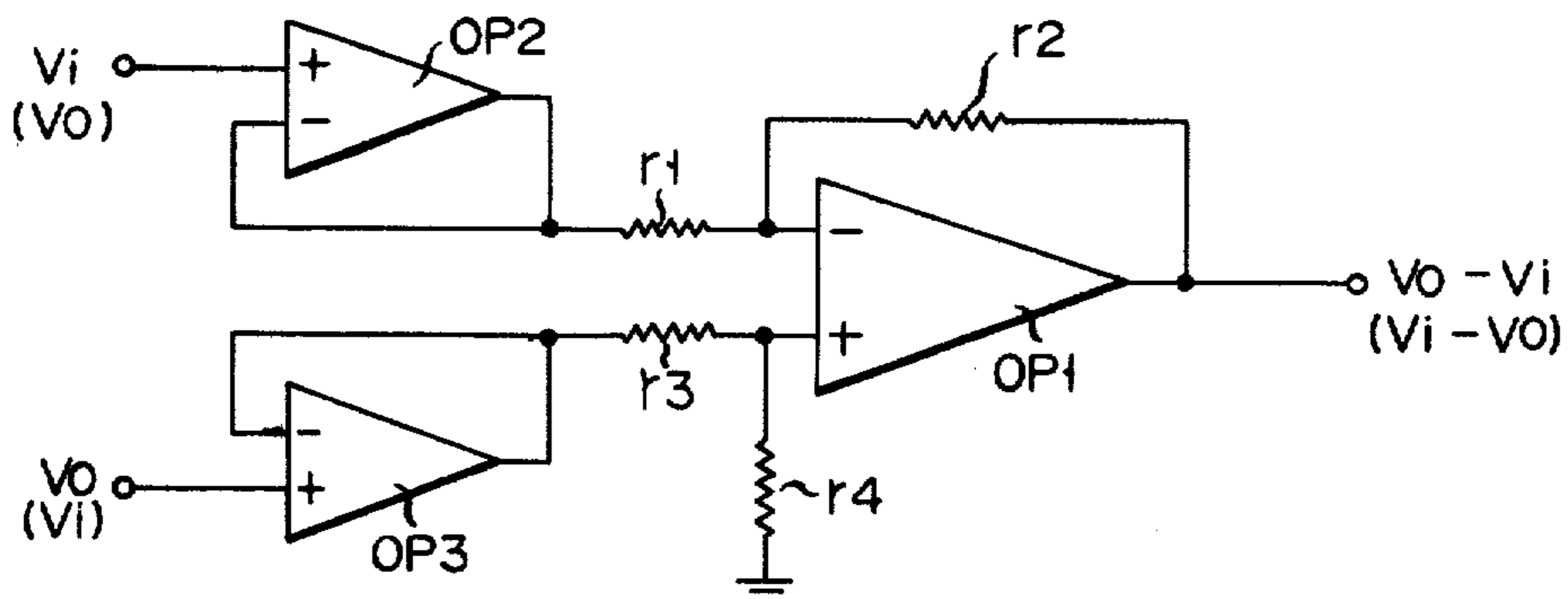
SUBTRACTOR 54 (55)
