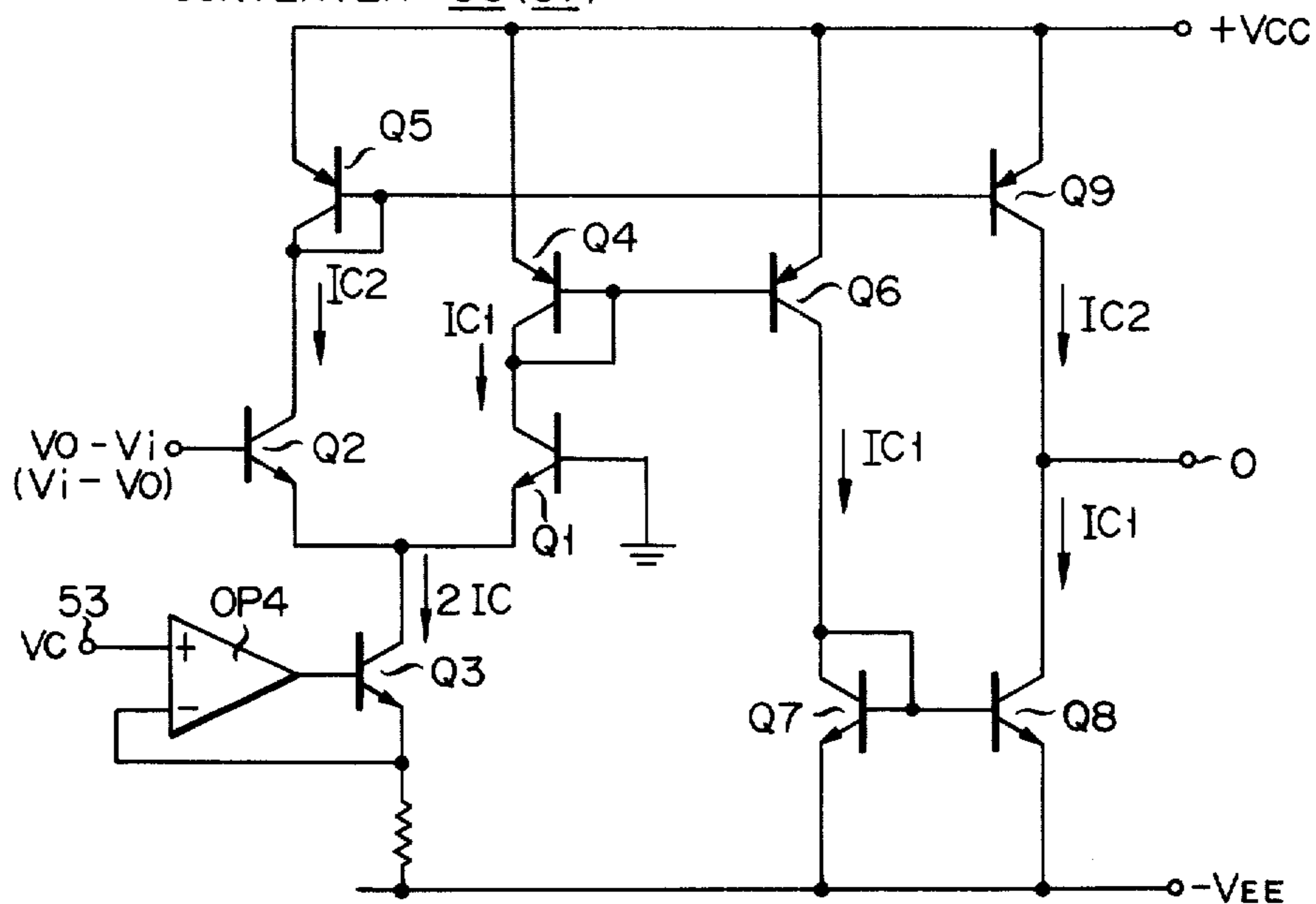
VOLTAGE-CONTROLLED CONDUCTANCE-VARIABLE VOLTAGE-TO-CURRENT CONVERTER 56 ( 57 )
