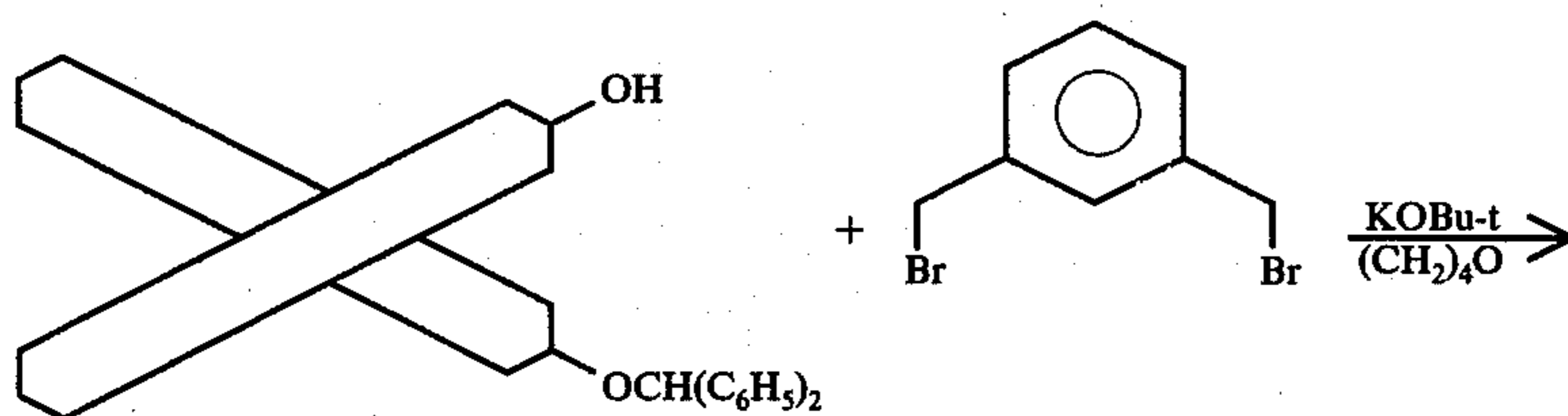
(S)-20
