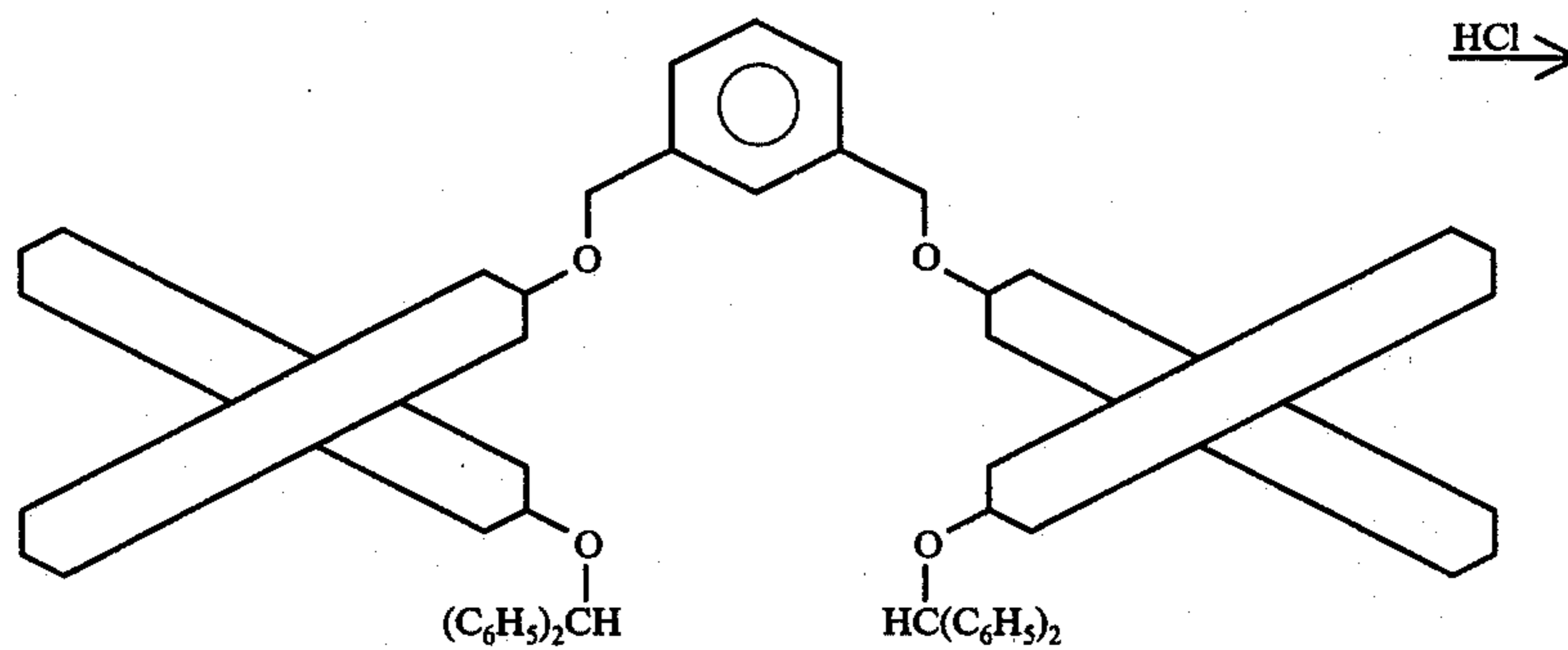
(SS)-109
