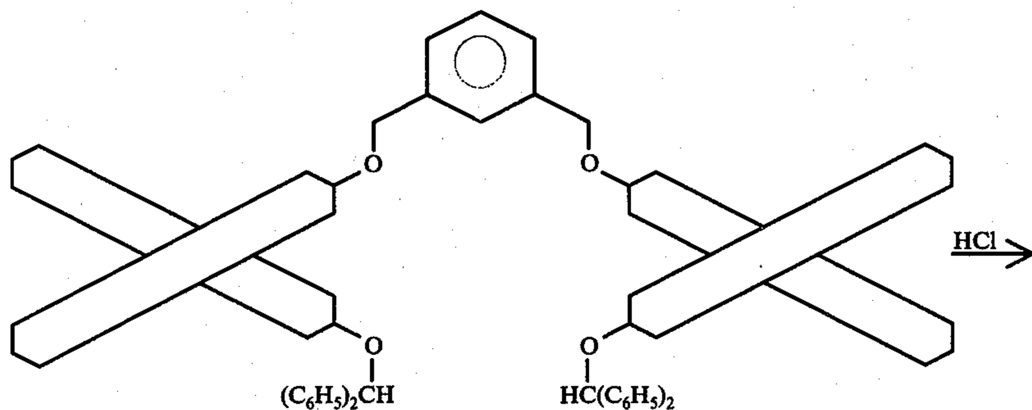
(SS)-109
