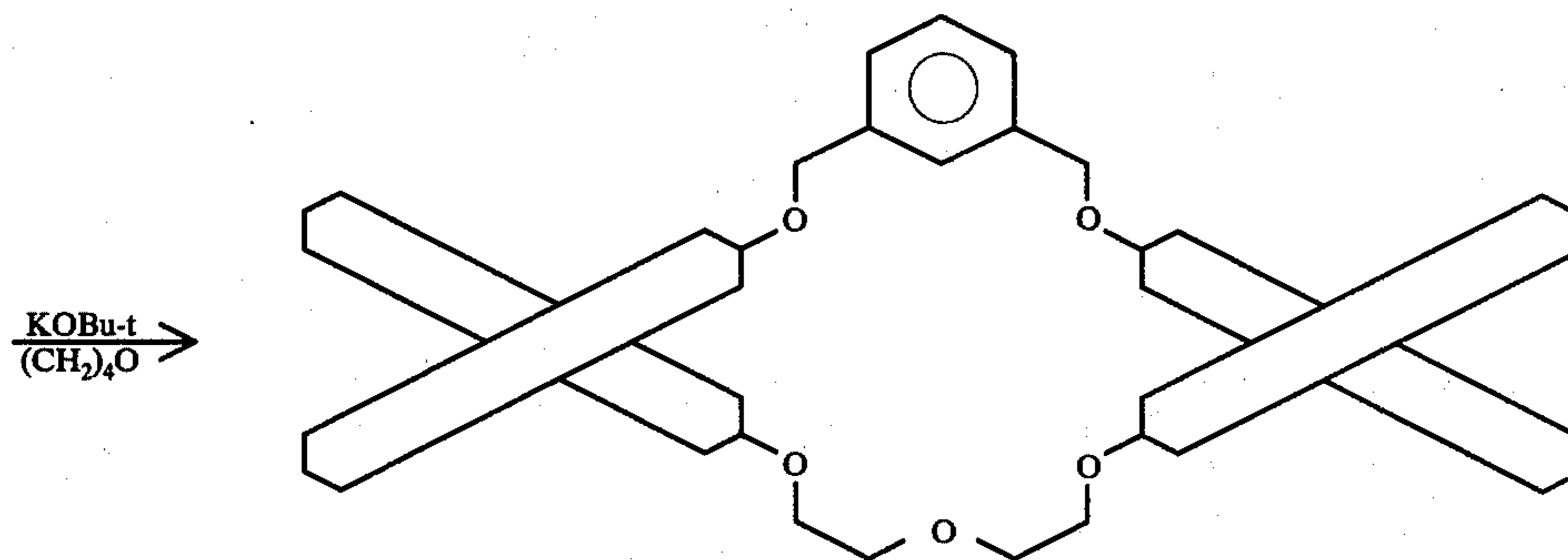
(SS)-108
