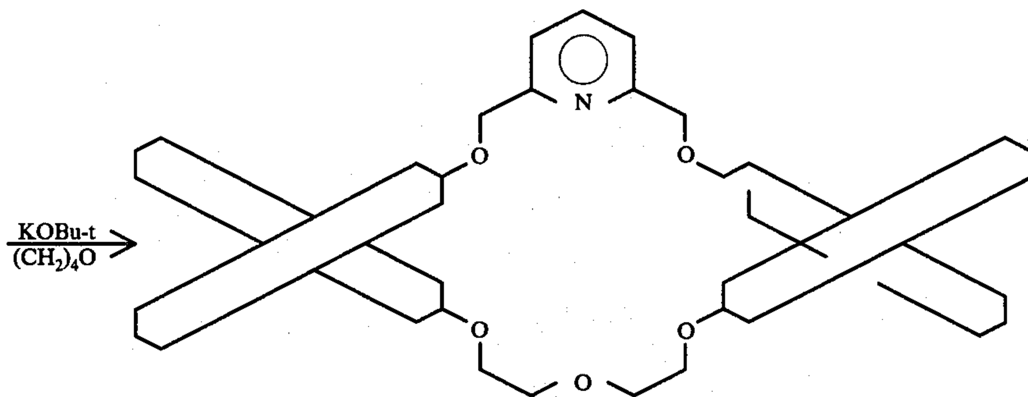
(SS)-22
