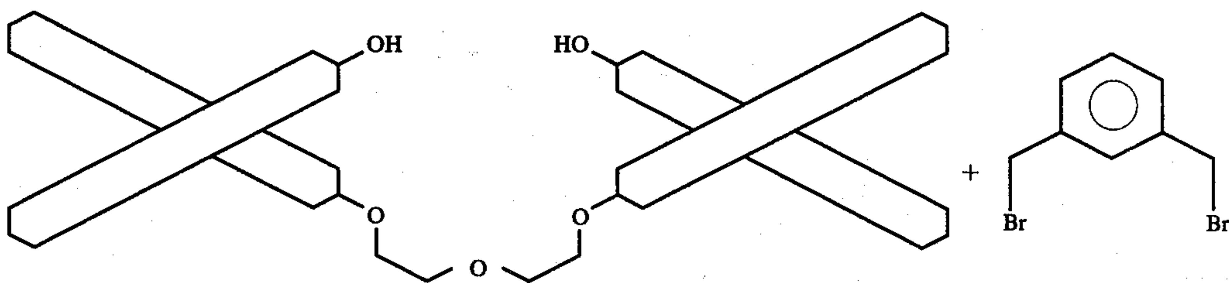
(SS)-22
