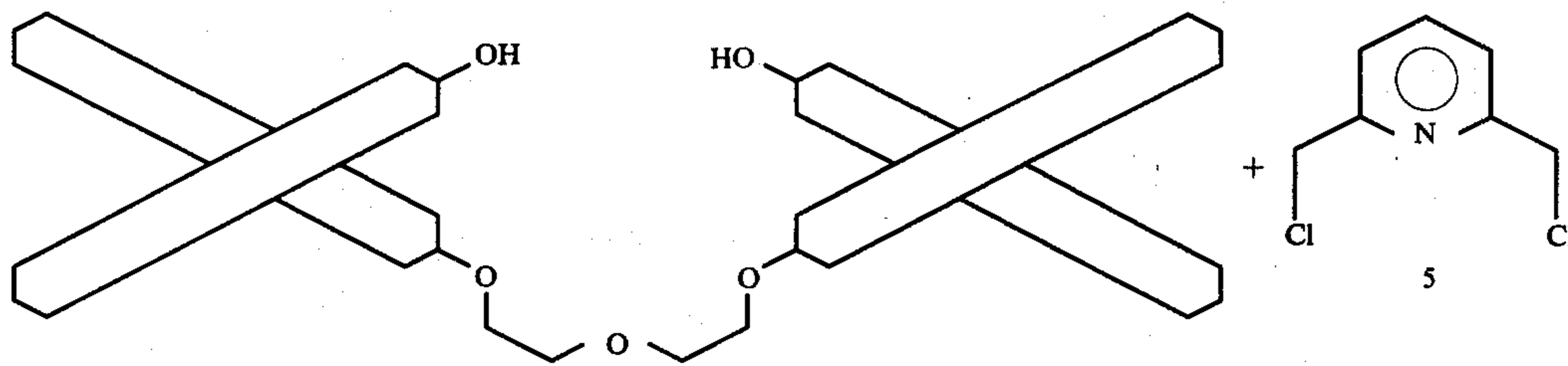
(SS)-22
