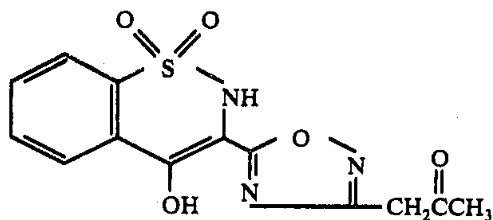
1-[[5-(4-Hydroxy-2H-1,2-benzothiazin-3-yl)-1,2,4-oxadiazol-3-yl]methyl]ethanone S,S-dioxide
