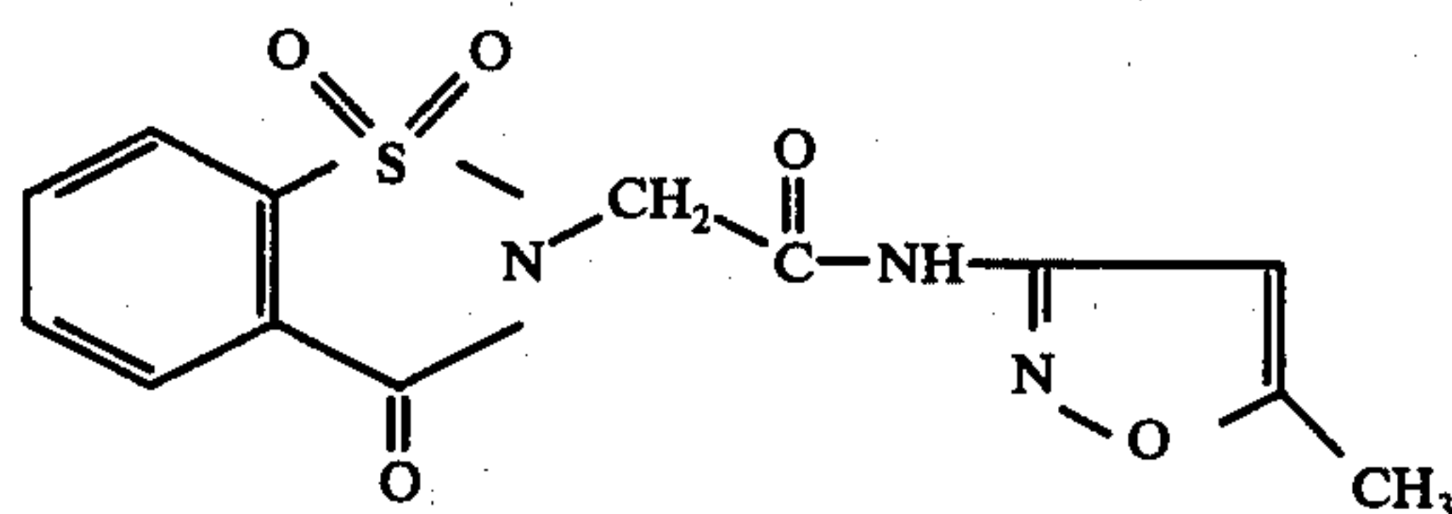
2,3-Dihydro-N-(5-methyl-3-isoxazolyl)-3-oxo-1,2-benzisothiazole-2-acetamide 1,1-dioxide
