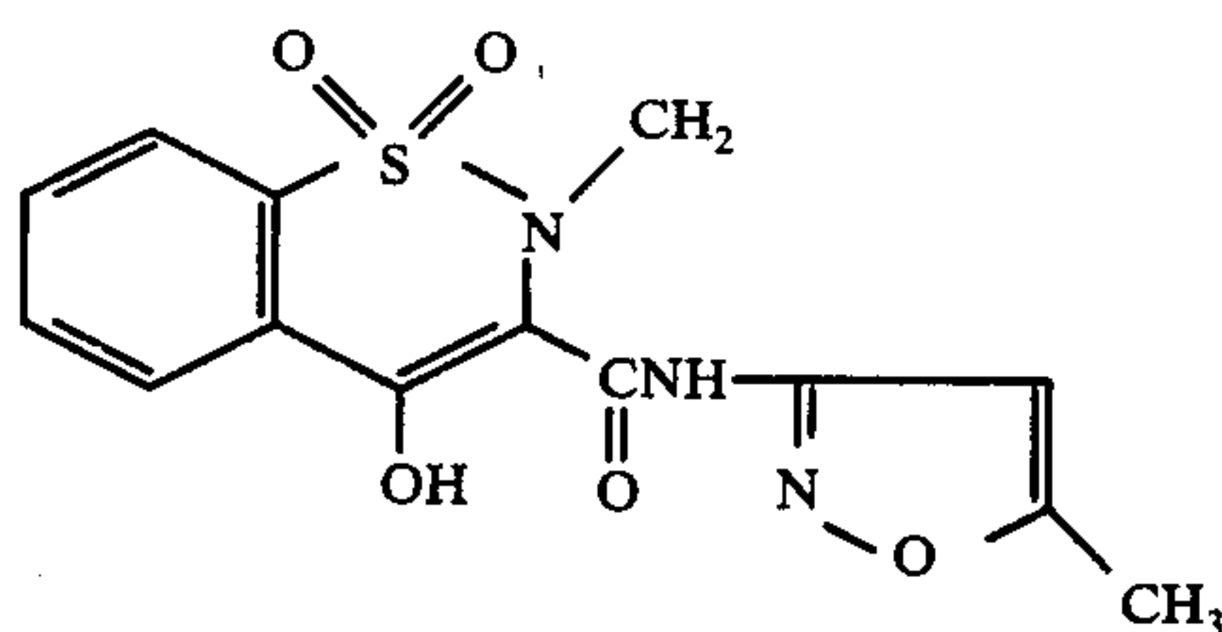
4-hydroxy-3-(5-methyl-3-isoxazolyl)-carbamoyl)-2-methyl-2H-1,2-benzothiazine 1,1-dioxide
