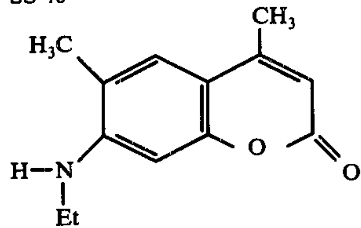
4,6-dimethyl-7-ethylaminocoumarin
