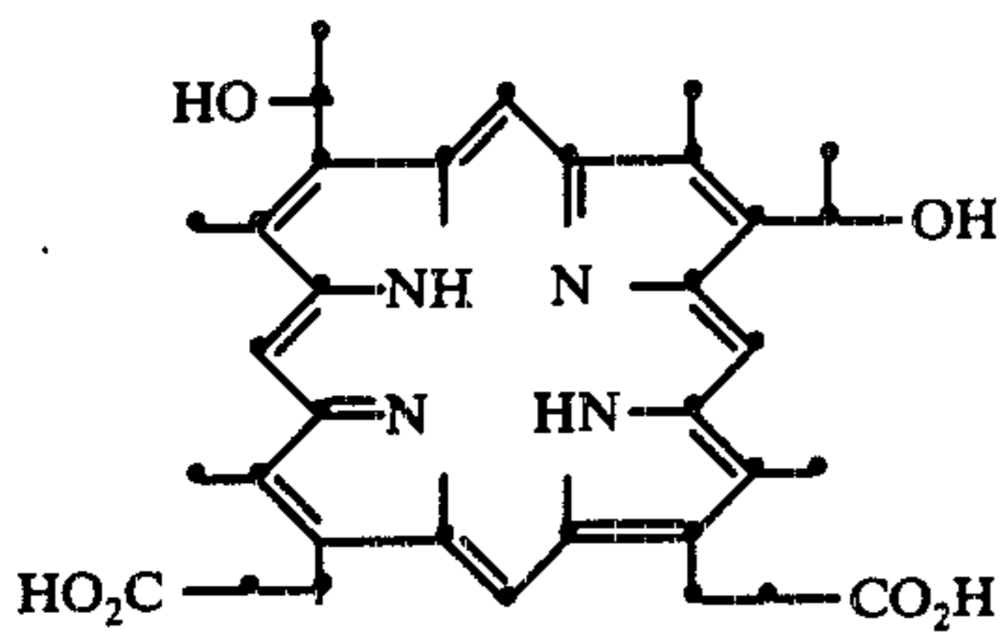
hematoporphyrin SS-38 NaO
