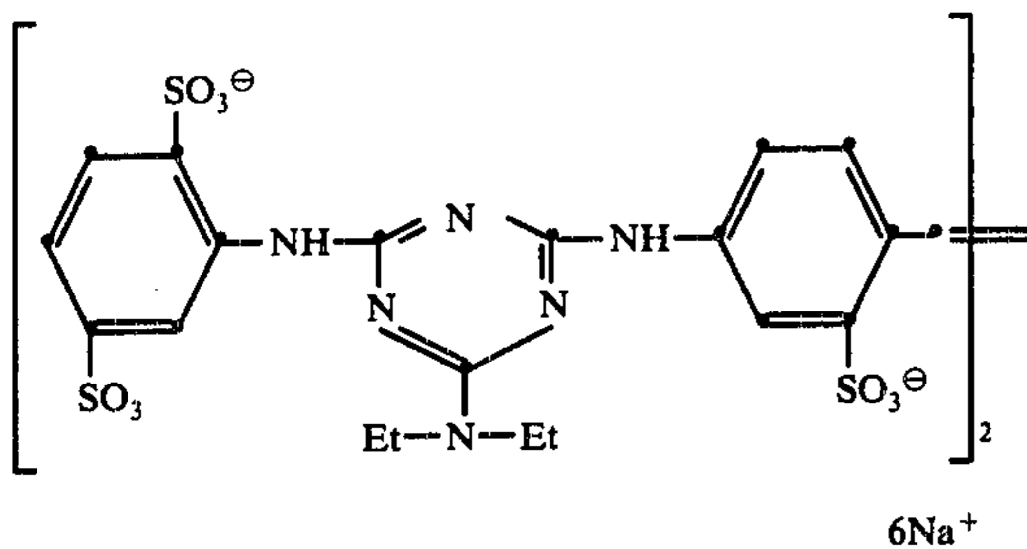
N,N'-di [4-diethylamino-6-(2,5-disulfoanilino)]- 2-s-triazinylamino-2,2'-stilbene disulfonic acid, hexasodium salt SS-37
