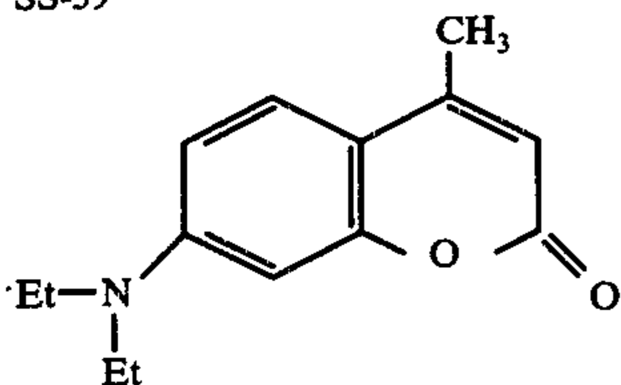
4-methyl-7-diethylaminocoumarin SS-40
