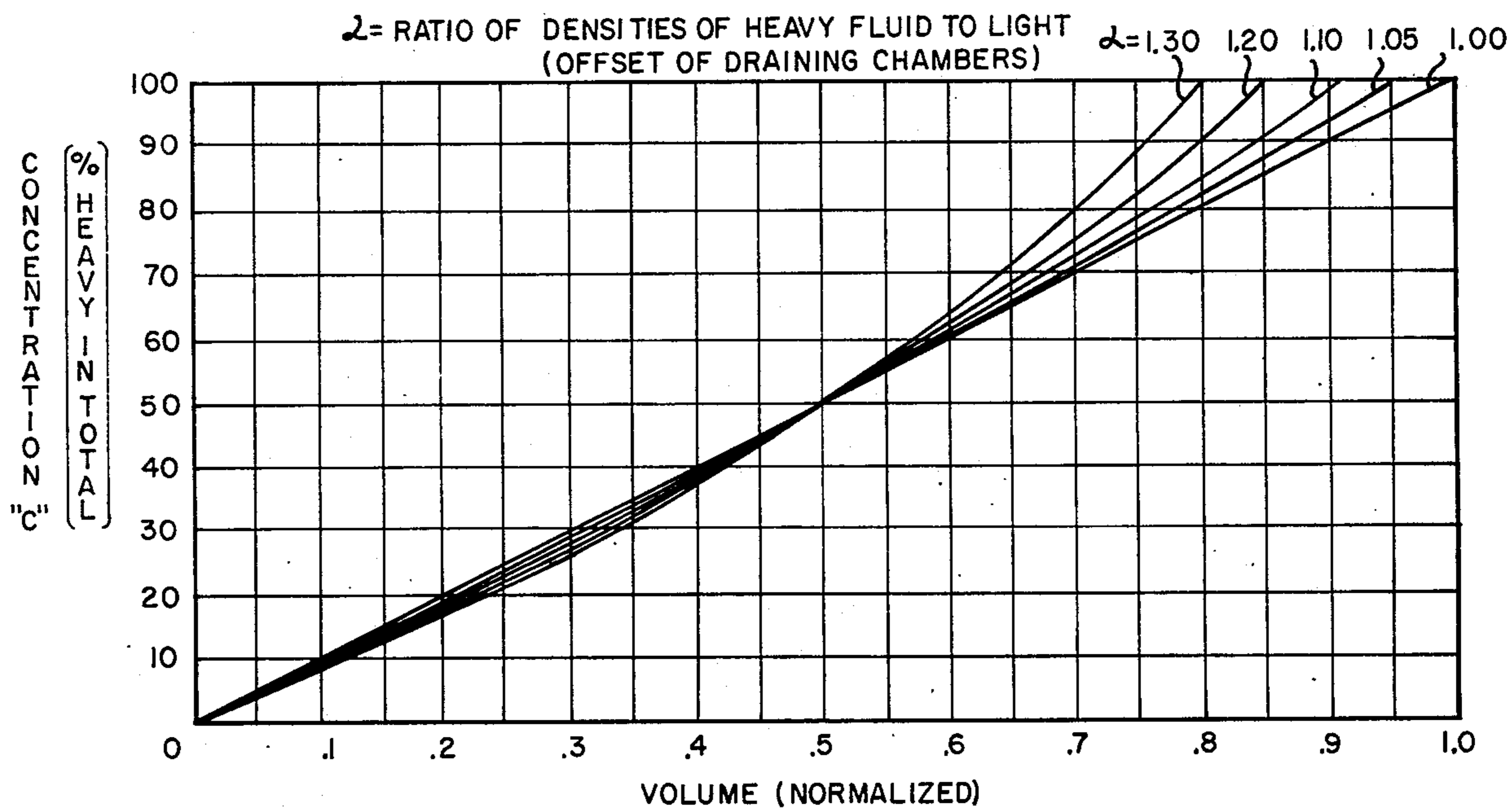
NORMALIZED GRADIENT CURVES FOR HYDROSTATIC GRADIENT GENERATORS
