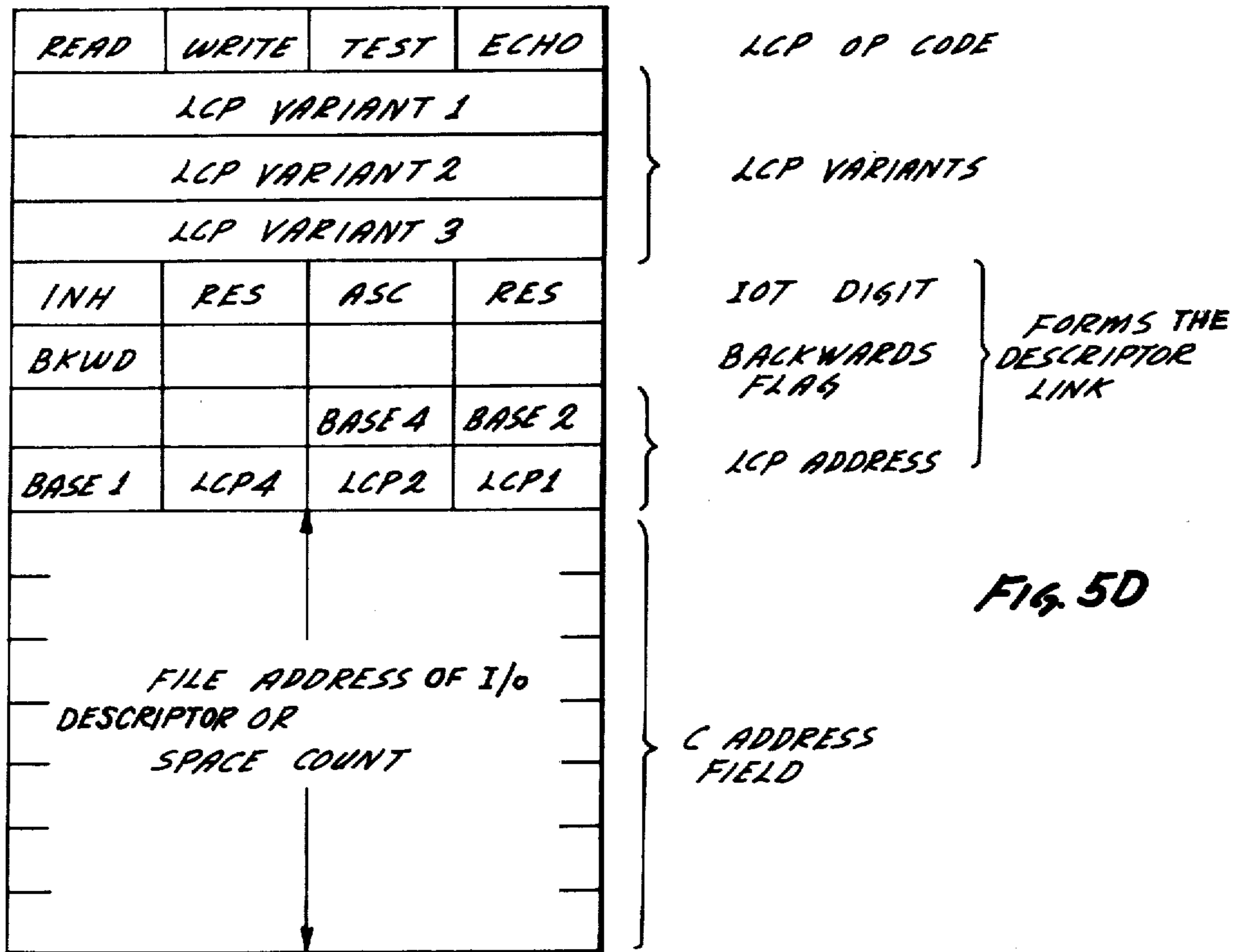
IOT DESCRIPTOR REGISTER INFORMATION
