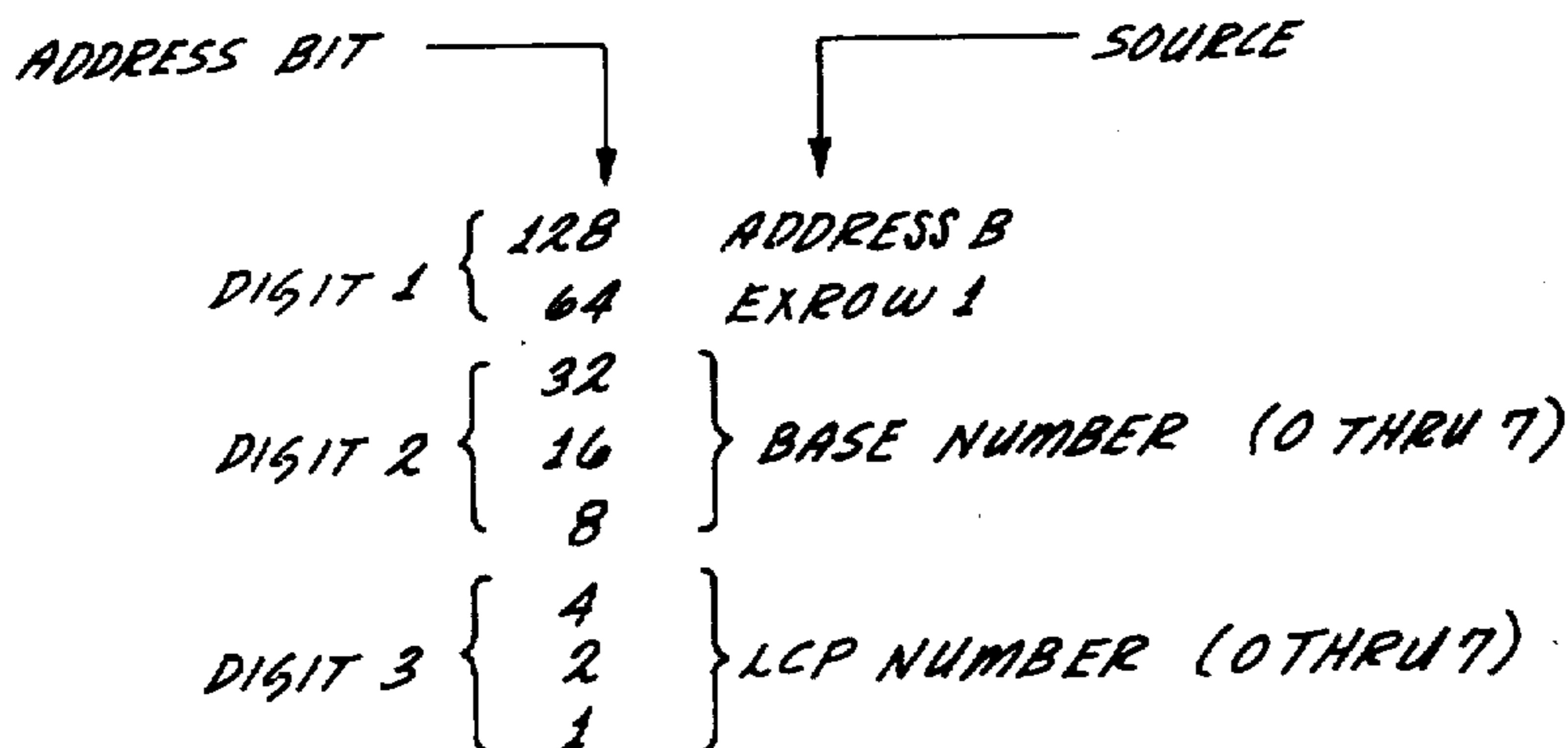
FIG. 5F IOT SCRATCHPAD MEMORY IOP A
