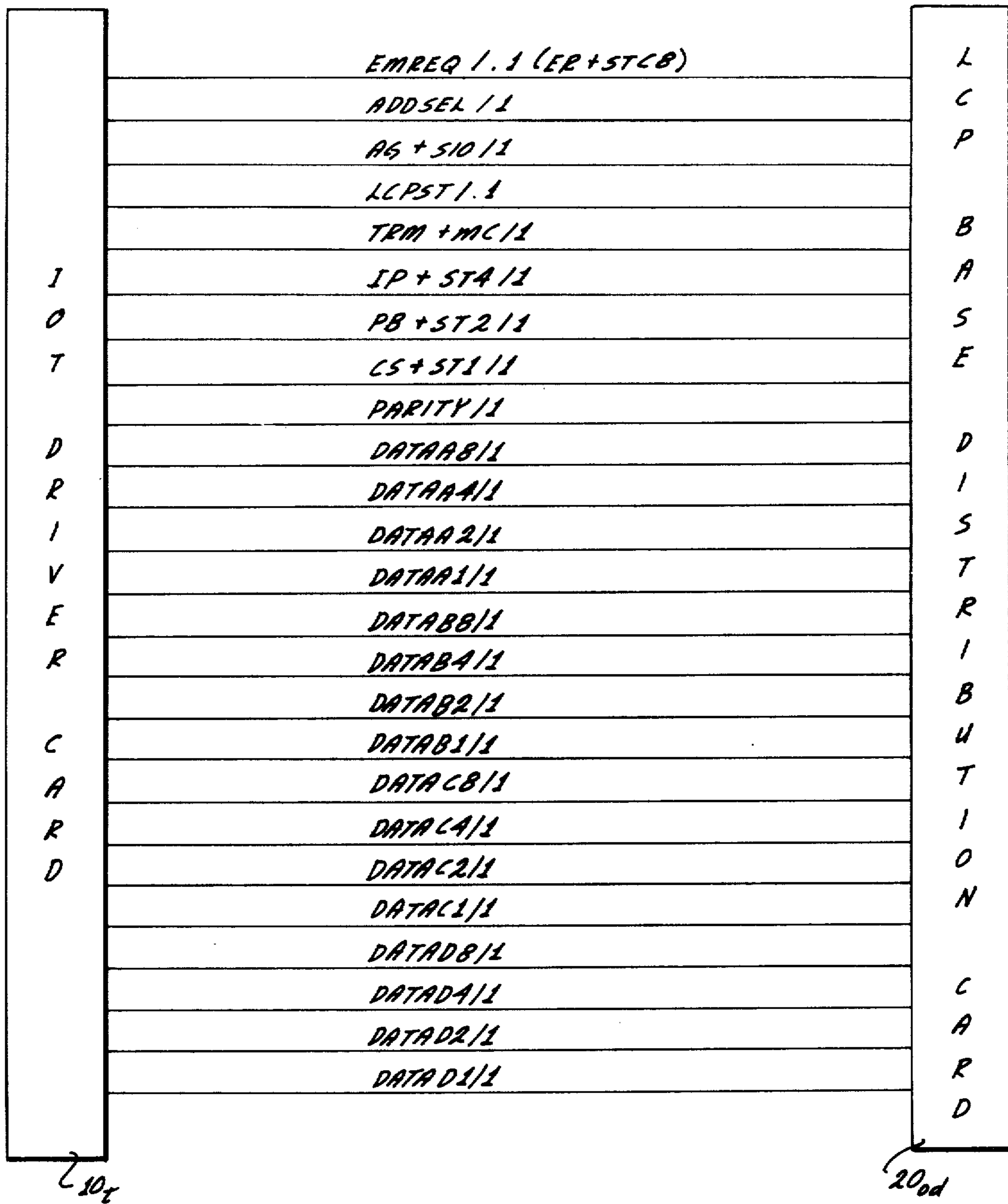
MESSAGE LEVEL INTERFACE
