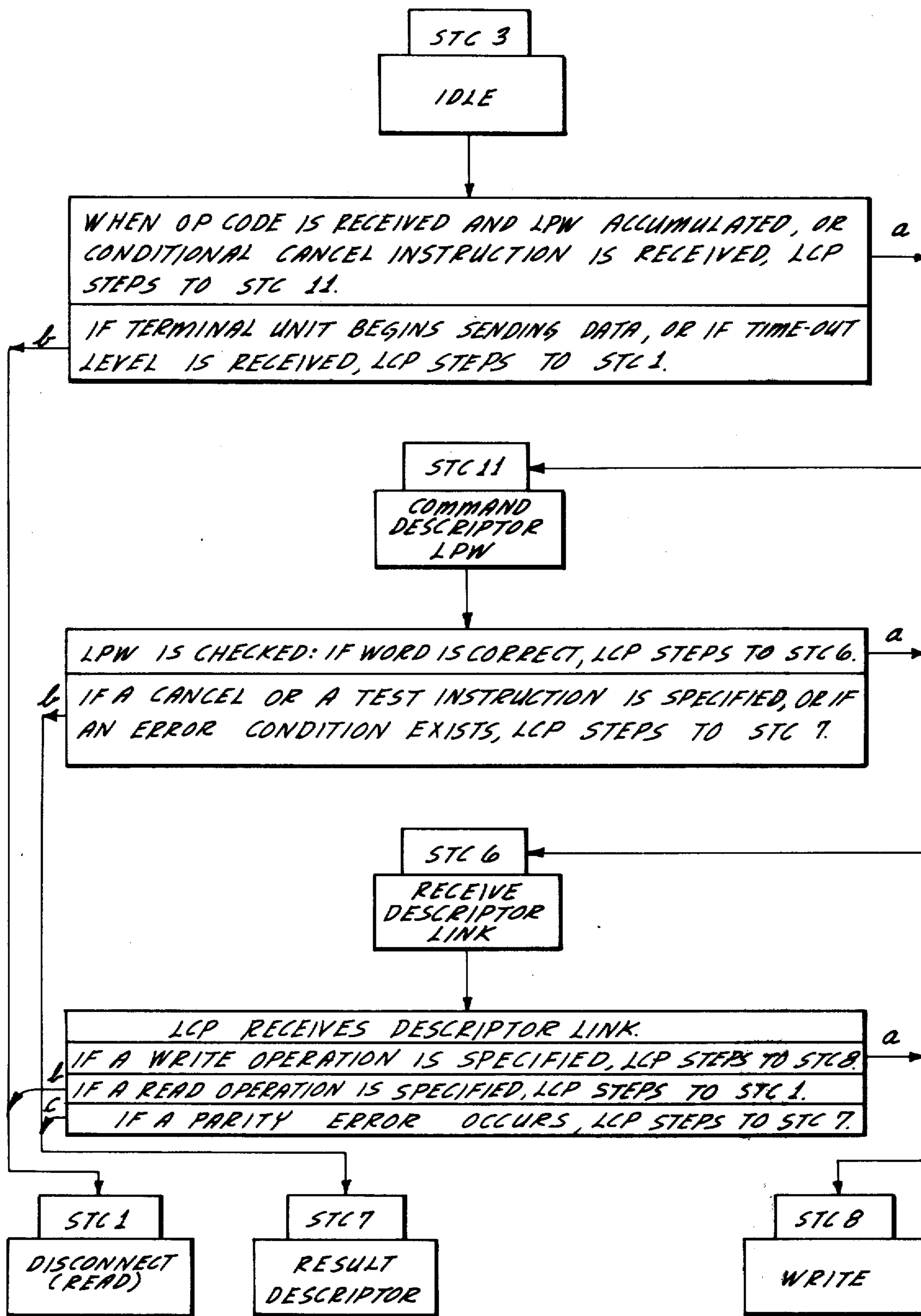
FIG. 7A SIMPLIFIED RECEIPT-OF-INSTRUCTIONS FLOW
