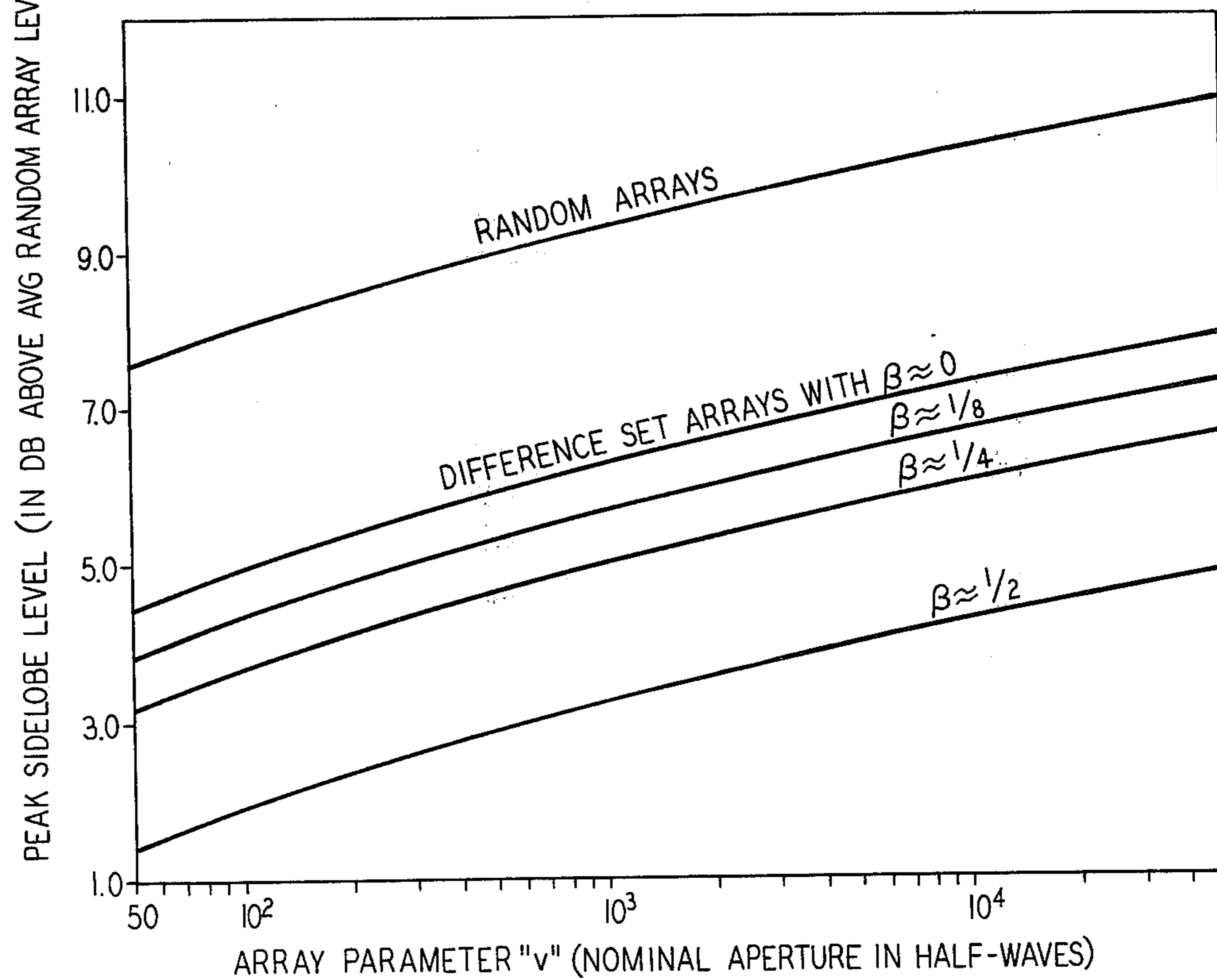
PEAK SIDELobe LEVEL VS ARRAY PARAMETER "v" FOR RANDOM ARRAYS AND DIFFERENCE SET ARRAYS
