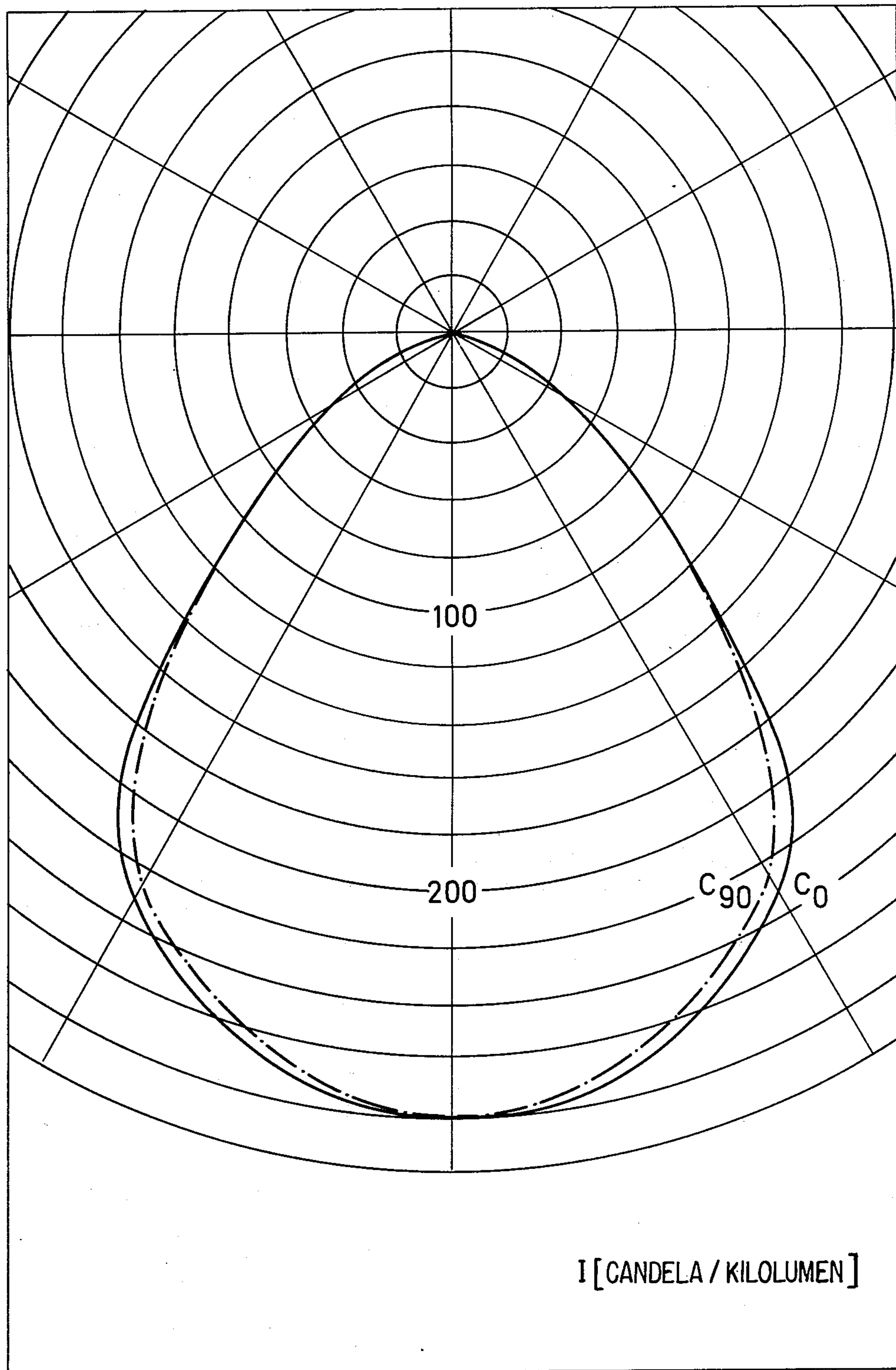
FIG. 1 (PRIOR ART)
