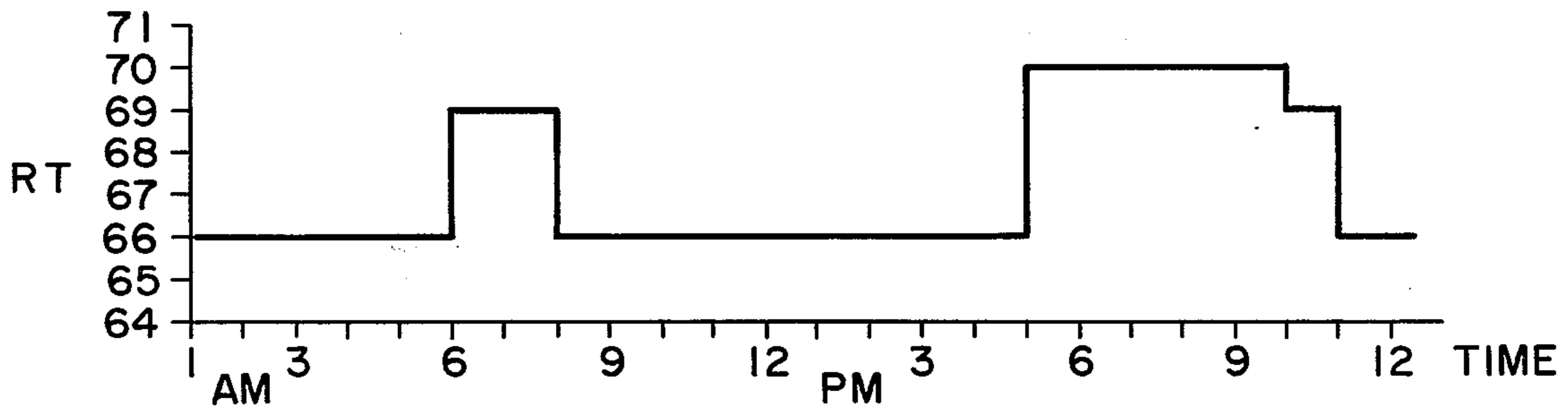
FIGURE 2C HEATING (OCCUPANTS NOT HOME DURING DAY)
