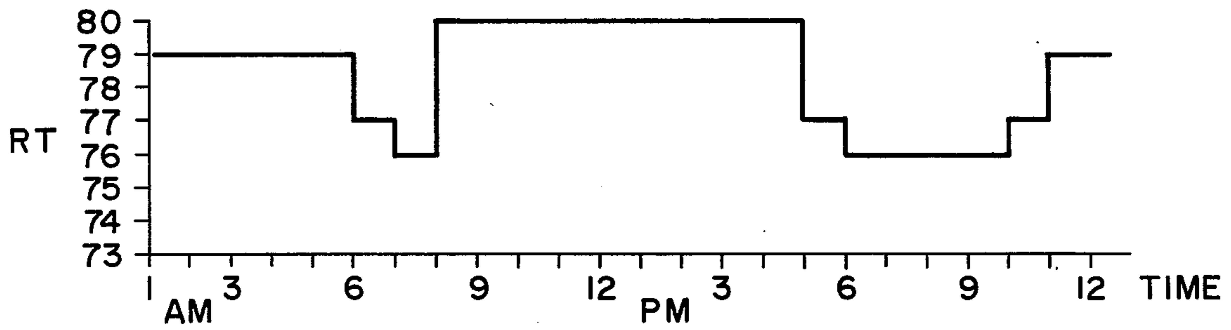
FIGURE 2A COOLING (OCCUPANTS NOT HOME DURING DAY)
