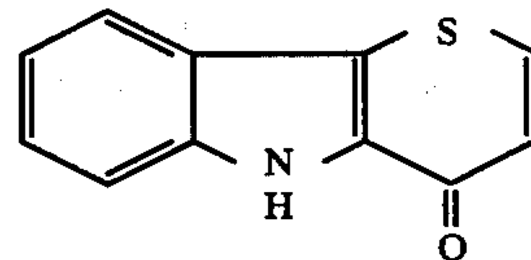
Thiopyrano[3,2-b]indol-4(5H)-one
