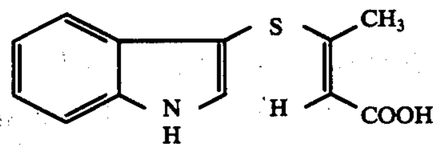
3-(Indol-3-ylthio)crotonic acid
