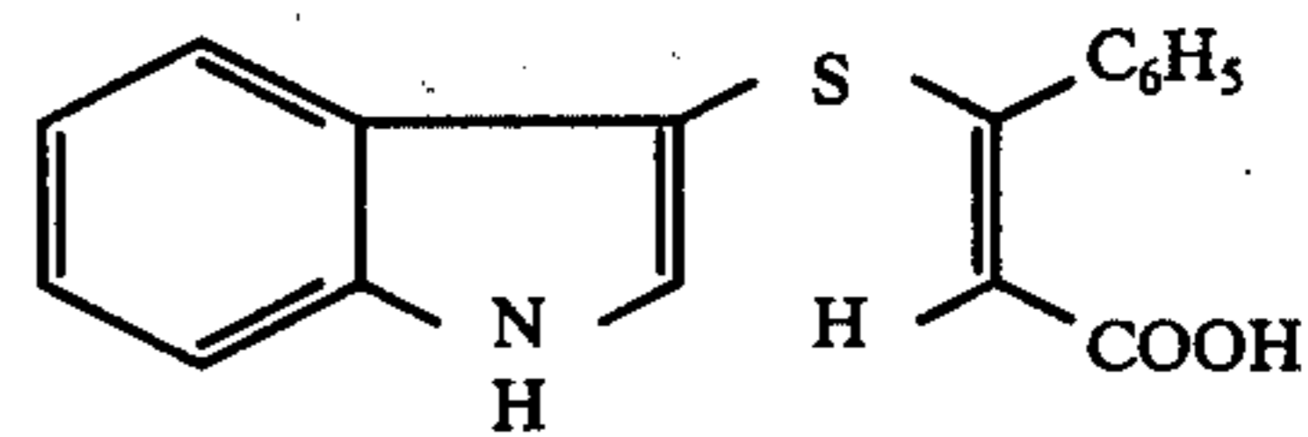
3-(Indol-3-ylthio)cinnamic acid
