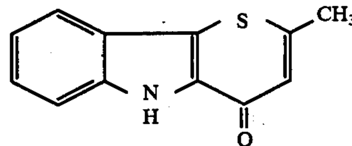
2-Methylthiopyrano[3,2-b]indol-4(5H)-one
