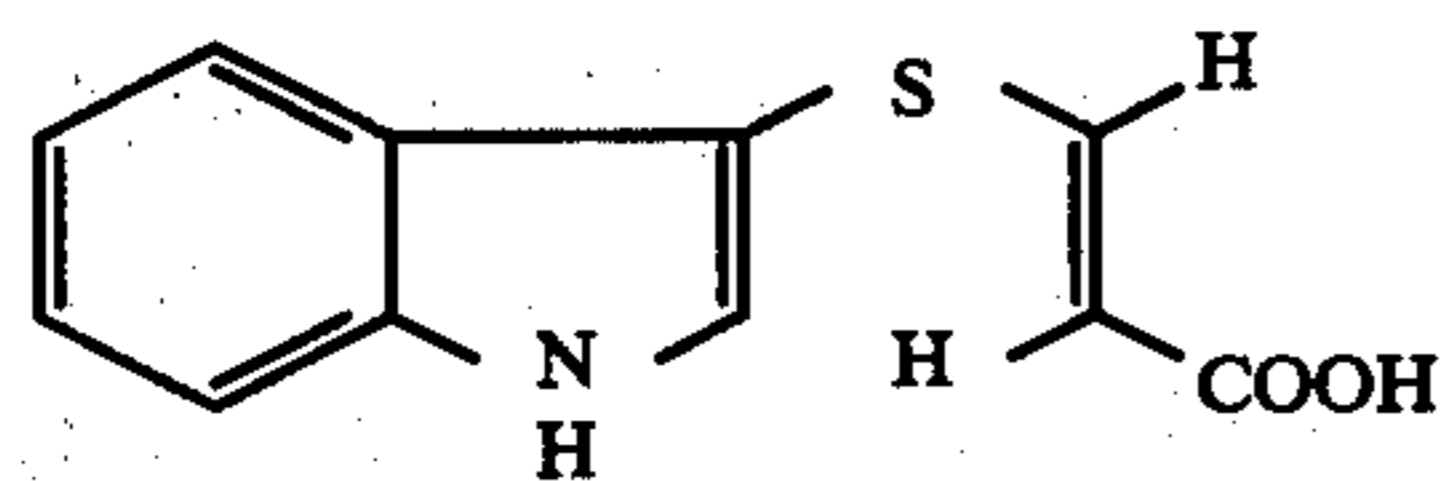
3-(Indol-3-ylthio)acrylic acid
