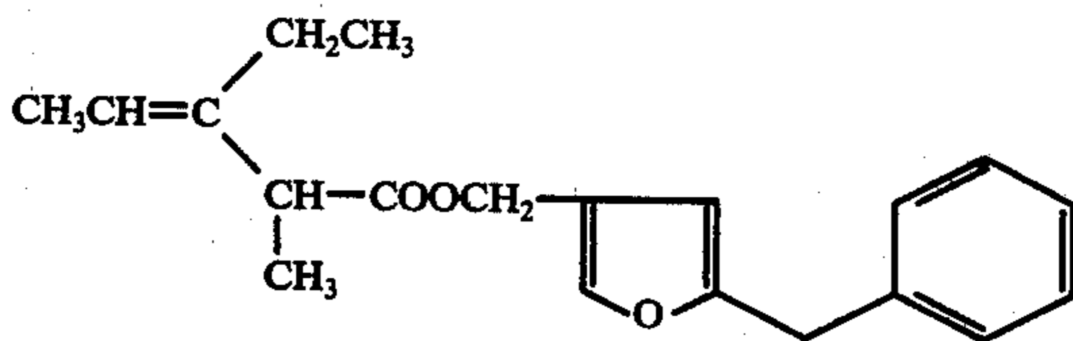
5'-Benzyl-3'-furylmethyl-2-methyl-3-ethyl-3-(cis,trans)-pentenoate n_D^{25} 1.5693
