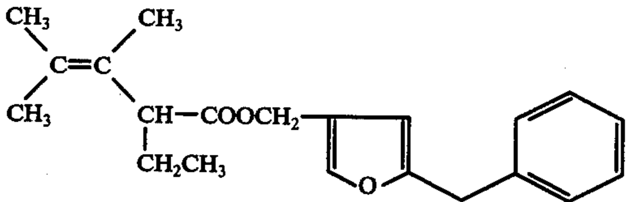
5'-Benzyl-3'-furylmethyl-2-ethyl-3,4-dimethyl-3-pentenoate n_D^{25} 1.5417
