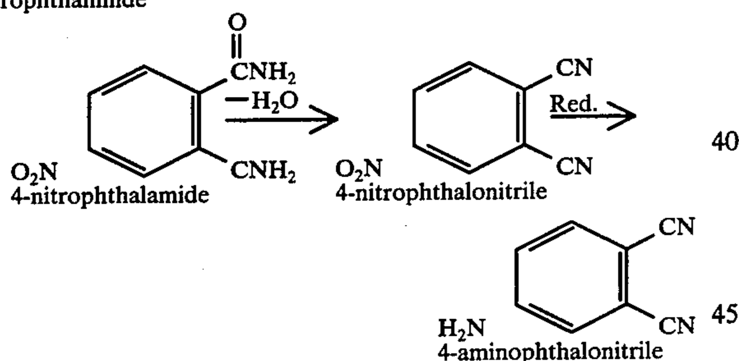
4-nitrophthalamide
