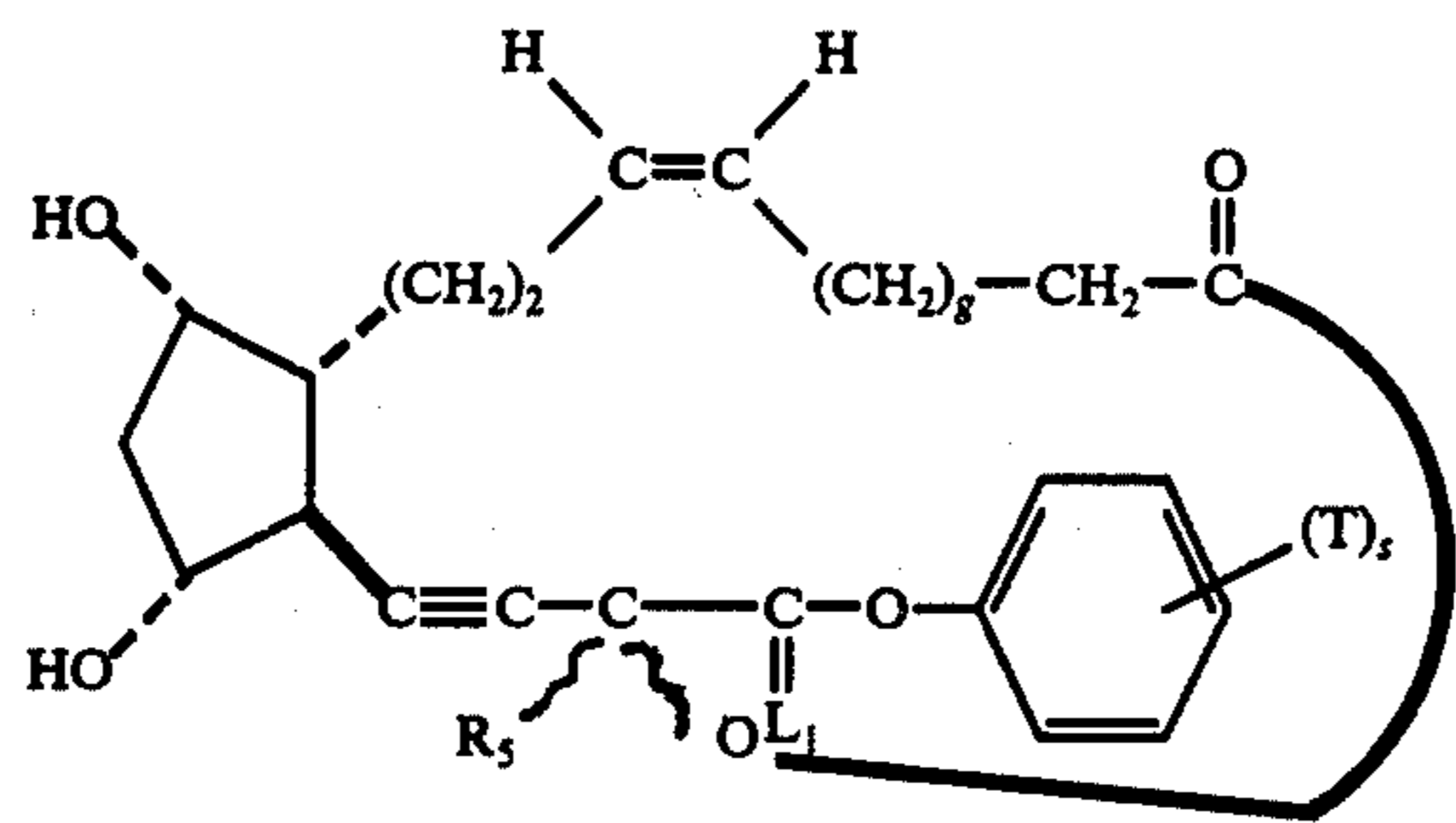
13,14-didehydro-cis-4,5-didehydro-PGF 1α -type, 1,15-lactones
