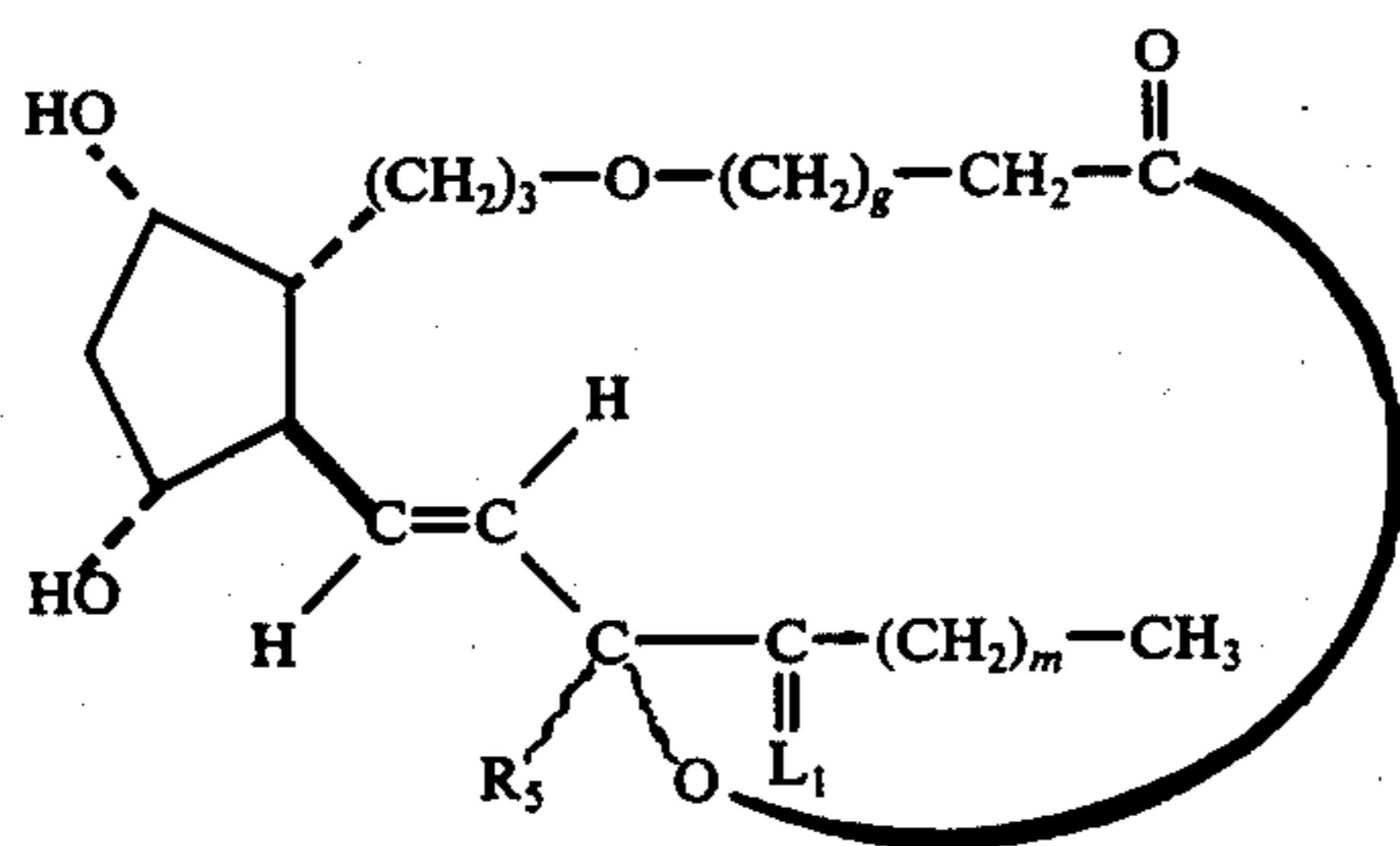
4-oxa-PGF 1α -type, 1,15-lactones
