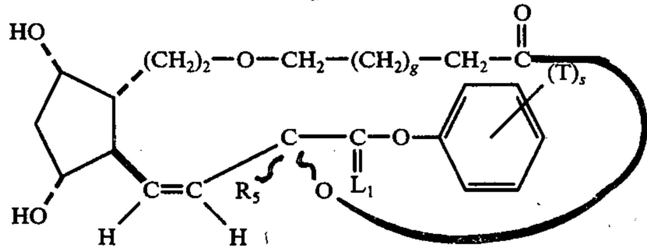
5-oxa-cis-13-PGF 1 \alpha -type, 1,15-lactones
