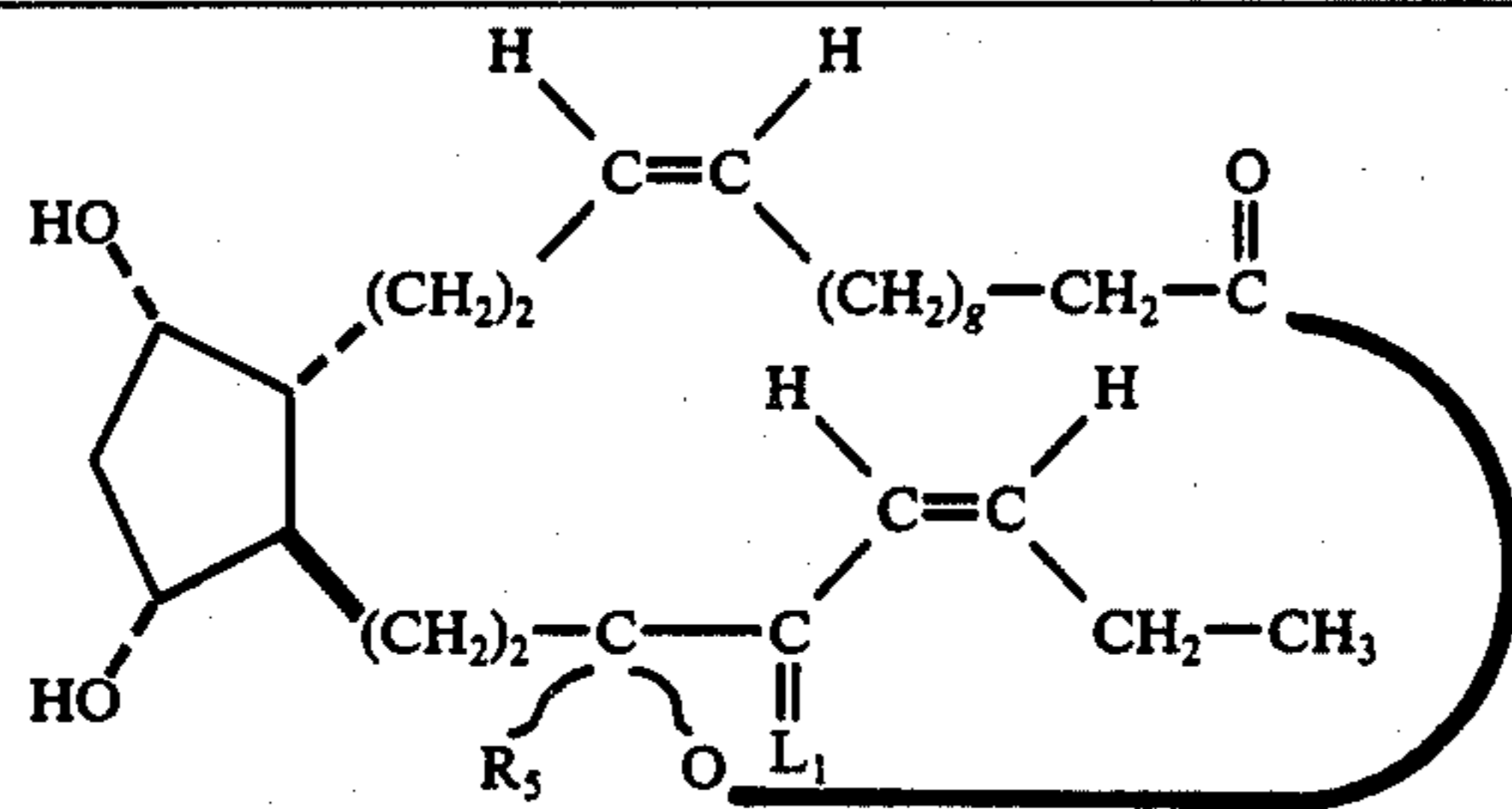
cis,cis-4,5,17,18-tetrahydro-13,14-dihydro-PGF 1α -type, 1,15-lactones
