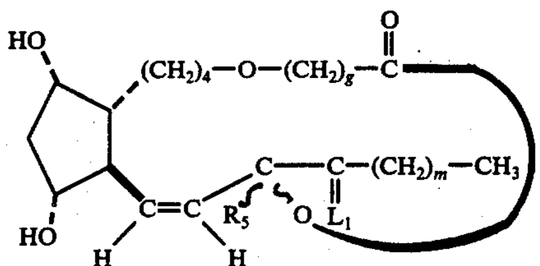
3-oxa-cis-13-PGF 1α -type, 1,15-lactones
