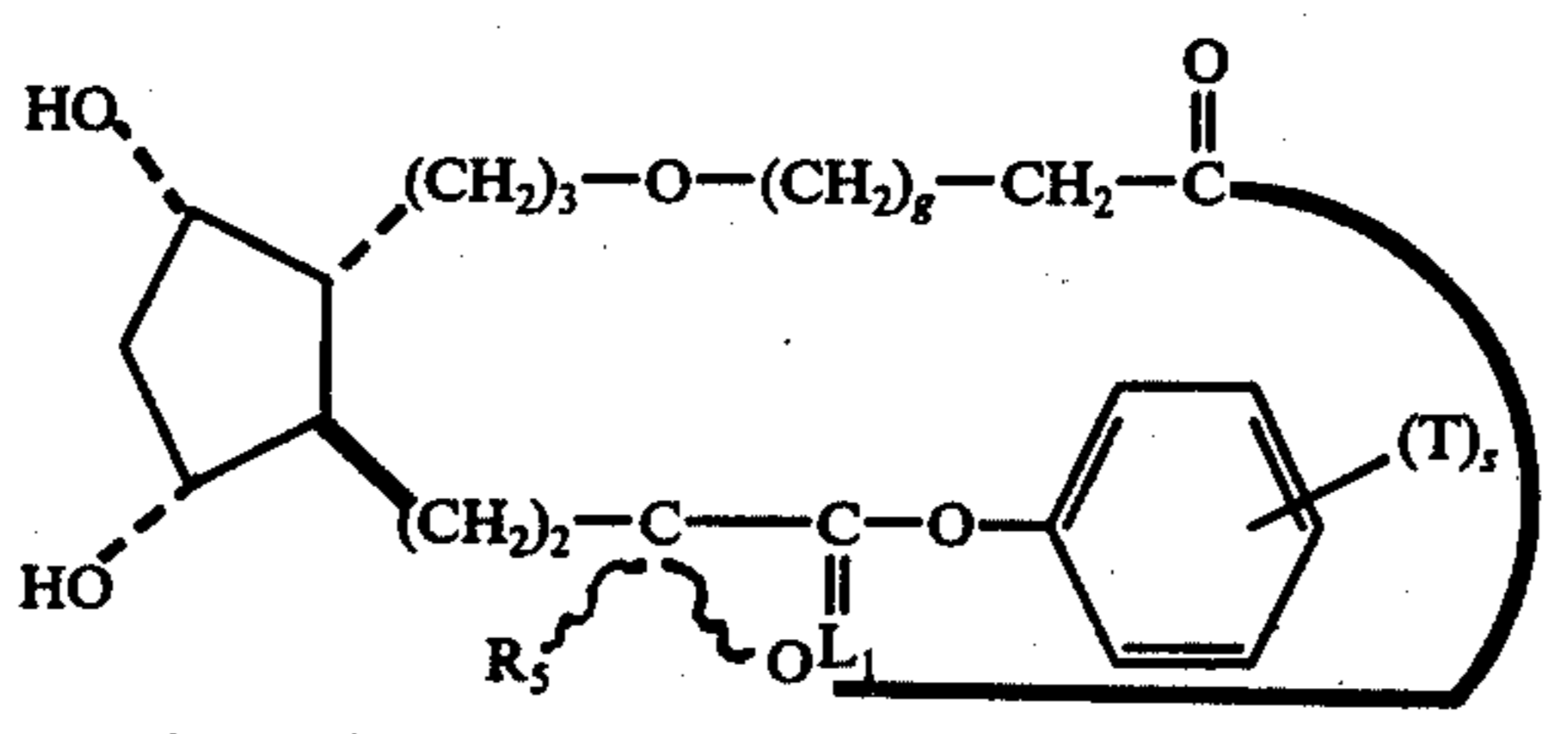
4-oxa-13,14-dihydro-PGF 1α -type, 1,15-lactones
