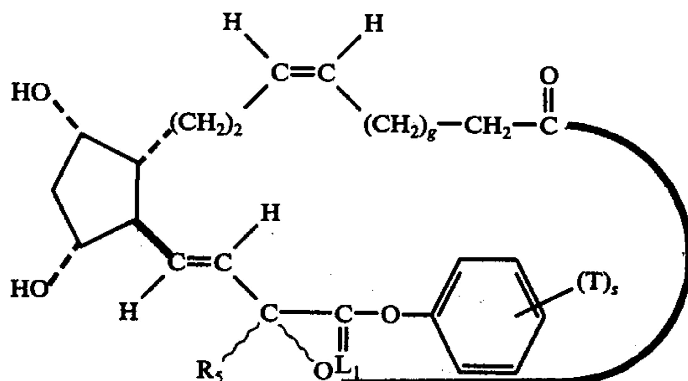
cis-4,5-didehydro-PGF 1α -type, 1,15-lactones
