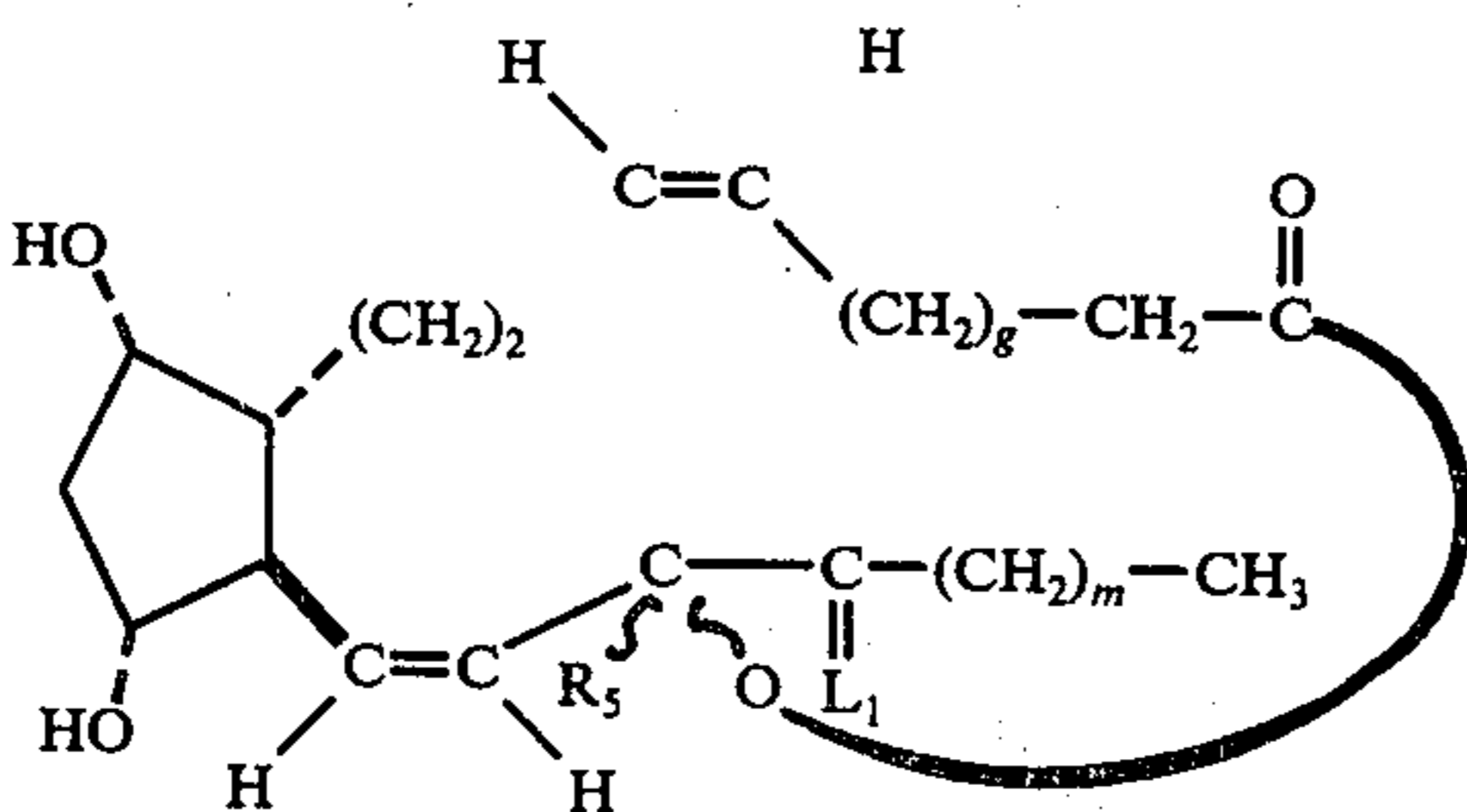
cis-13-PGF 1α -type, 1,15-lactones
