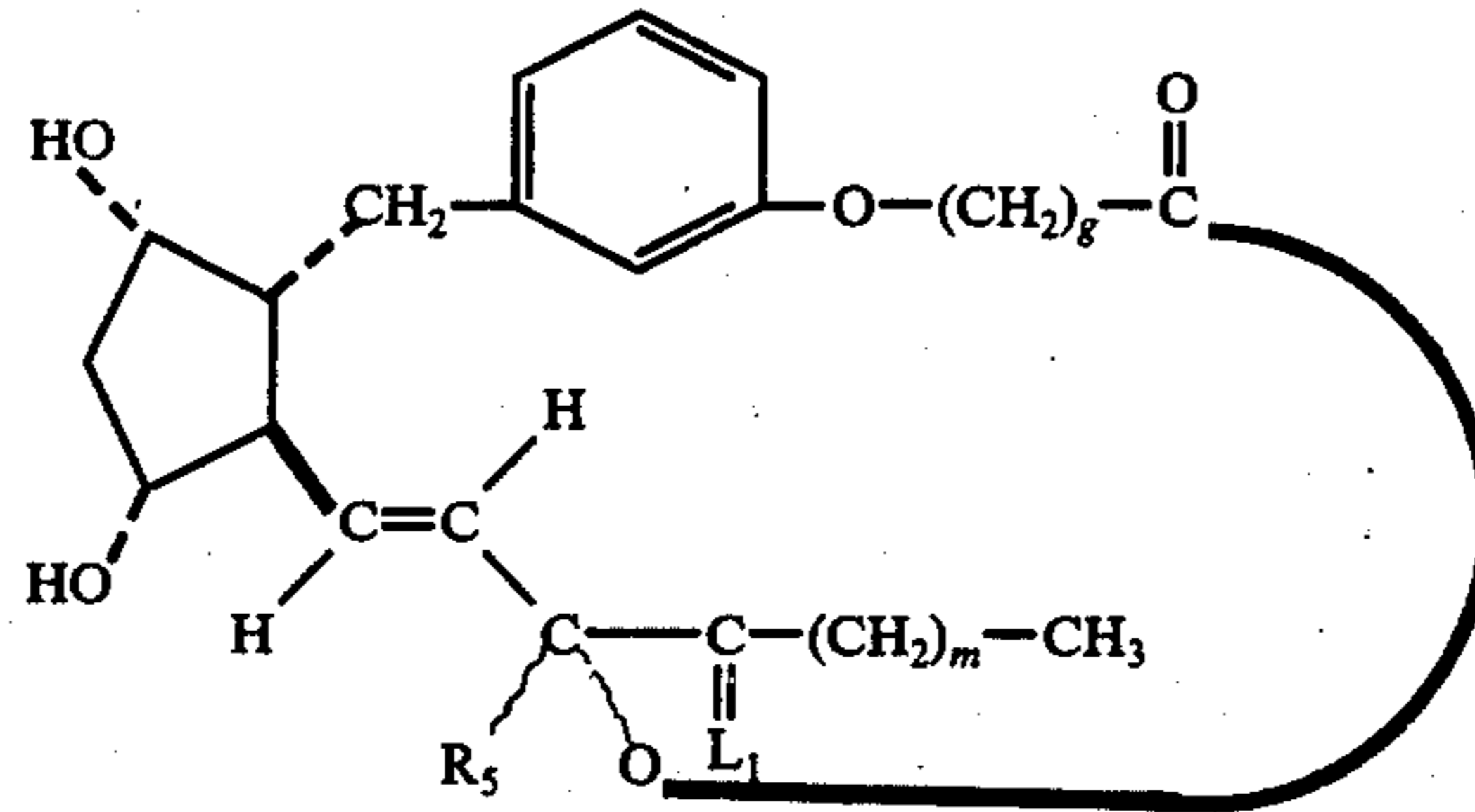
3,7-inter-m-phenylene-3-oxa-4,5,6-trinor-PGF 1α -type, 1,15-lactones
