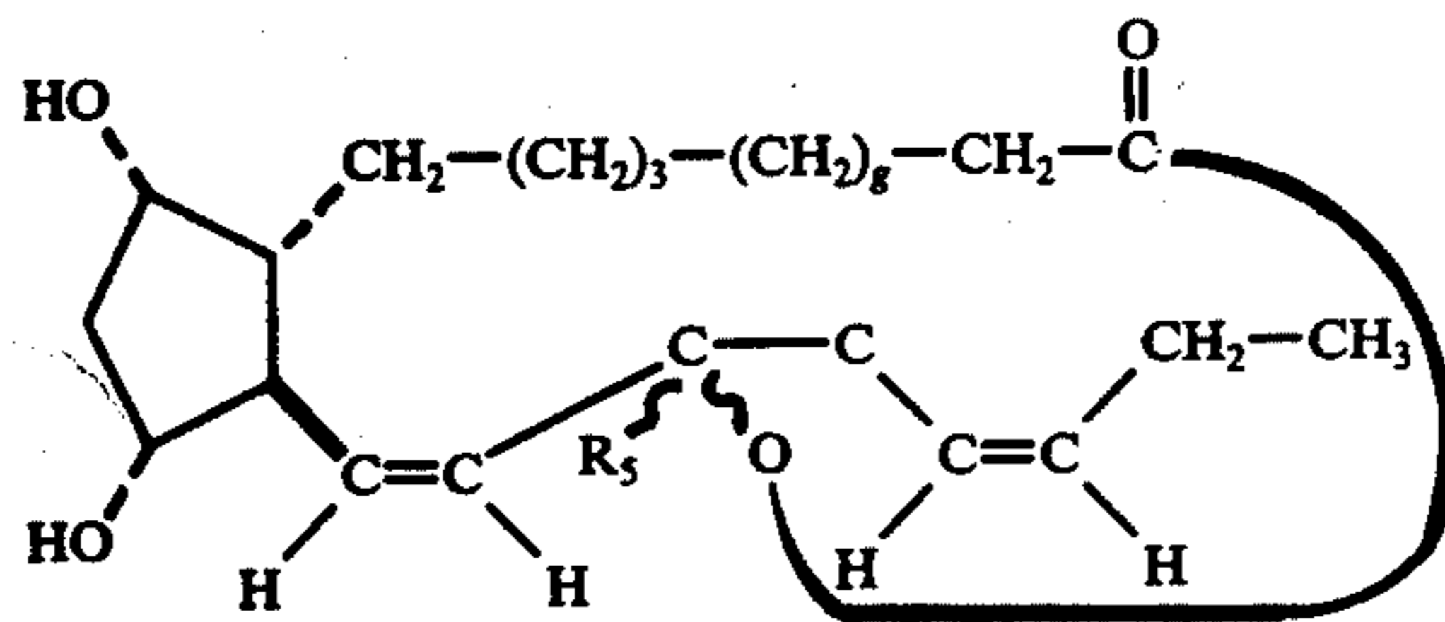
cis-13-5,6-dihydro-PGF 3 \alpha -type, 1,15-lactones
