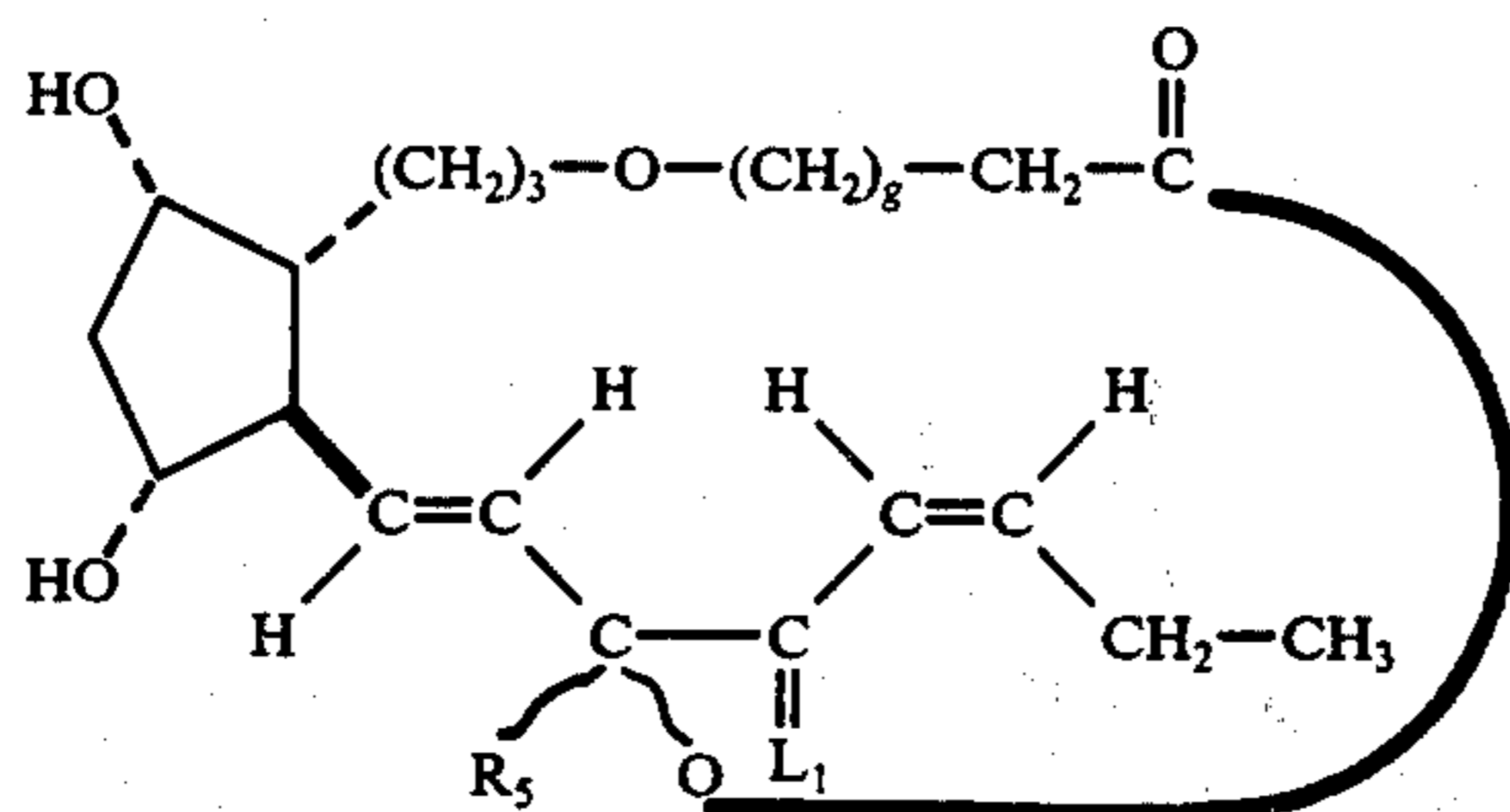
4-oxa-cis-17,18-didehydro-PGF 1α -type, 1,15- lactones
