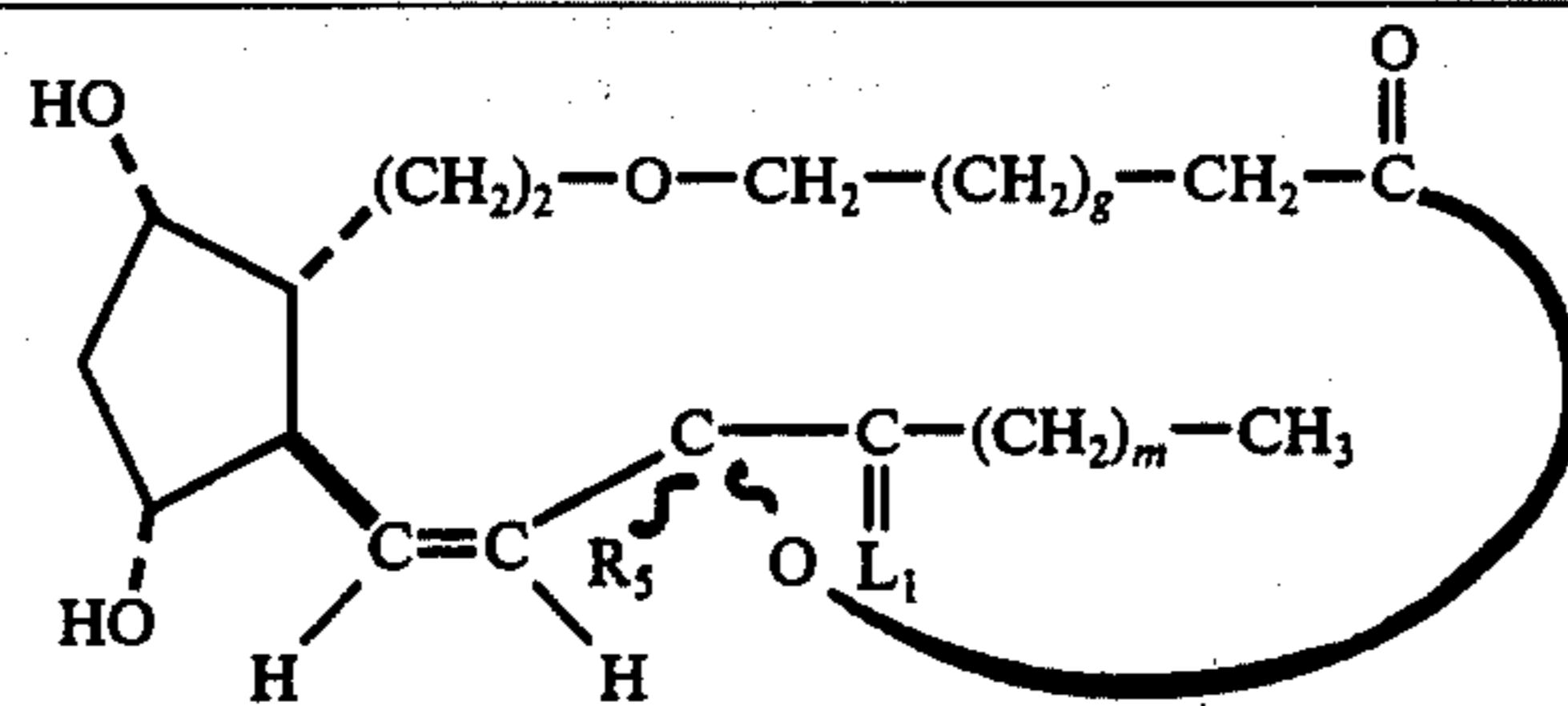
5-oxa-cis-13-PGF 1α -type, 1,15-lactones
