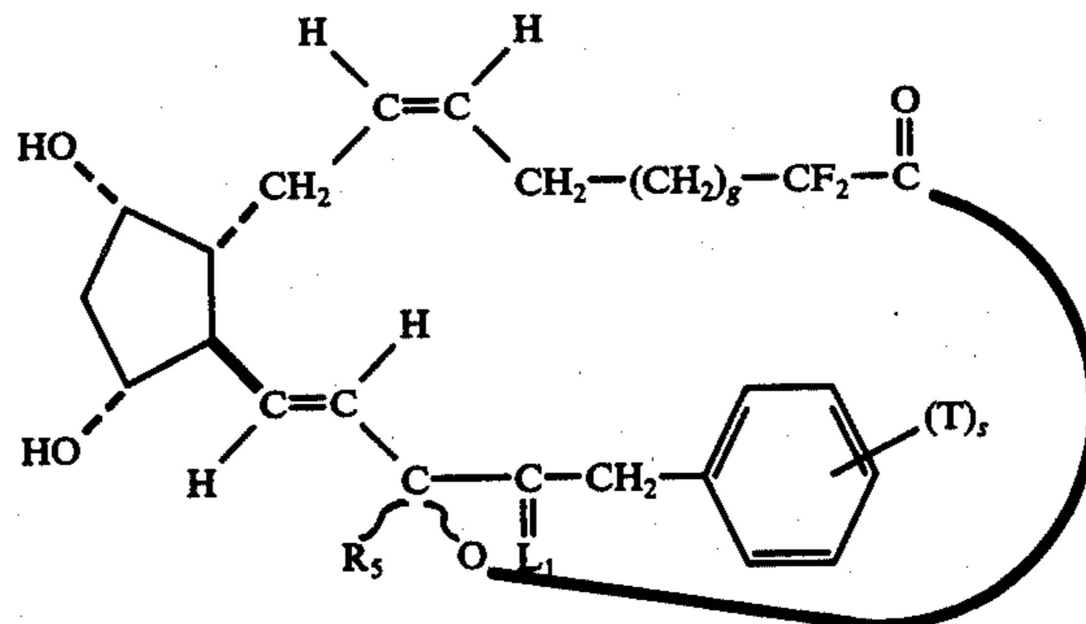
18,19,20-trinor-2,2-difluoro-PGF 2α -type, 1,15-lactones
