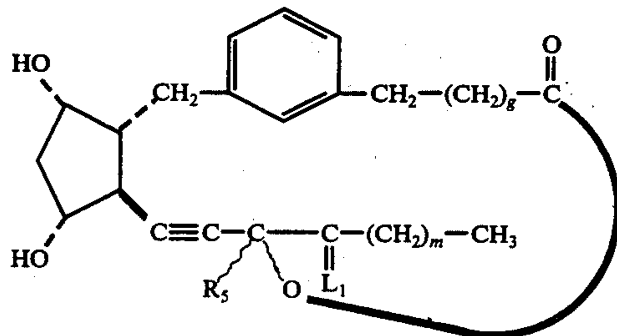
13,14-didehydro-3,7-inter-m-phenylene-4,5,6-trinor-PGF 1α -type, 1,15-lactones
