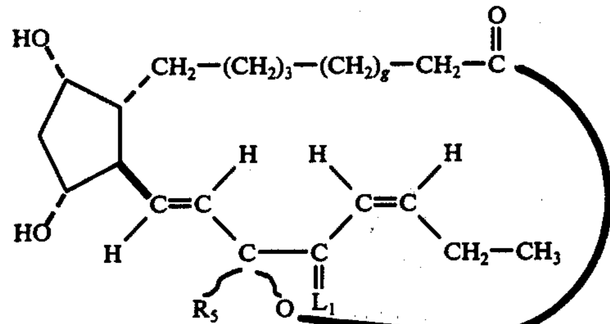
5,6-dihydro-PGF 3 \alpha -type, 1,15-lactones
