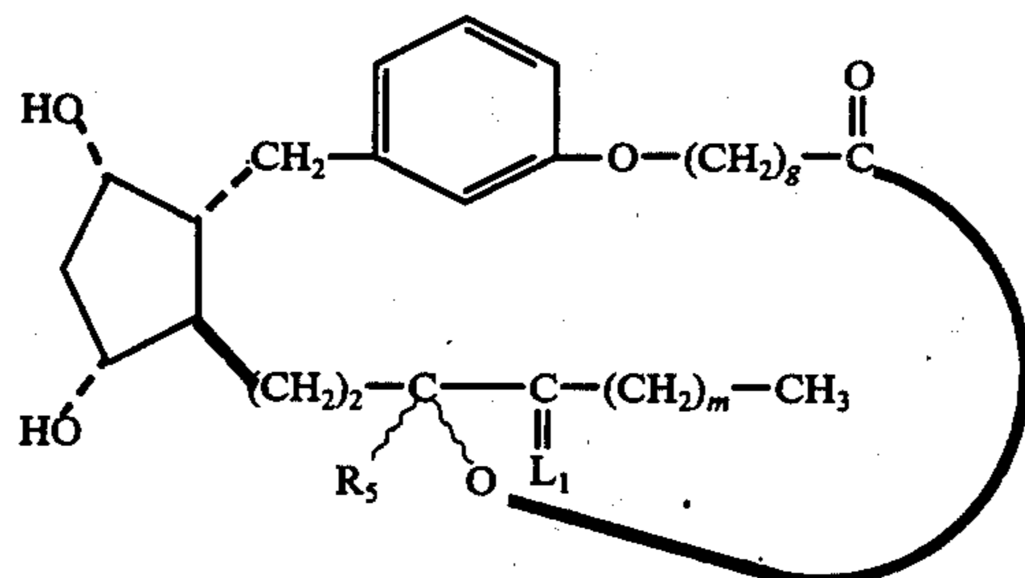
3,7-inter-m-phenylene-3-oxa-4,5,6-trinor-13,14-dihydro-PGF 1α -type, 1,15-lactones
