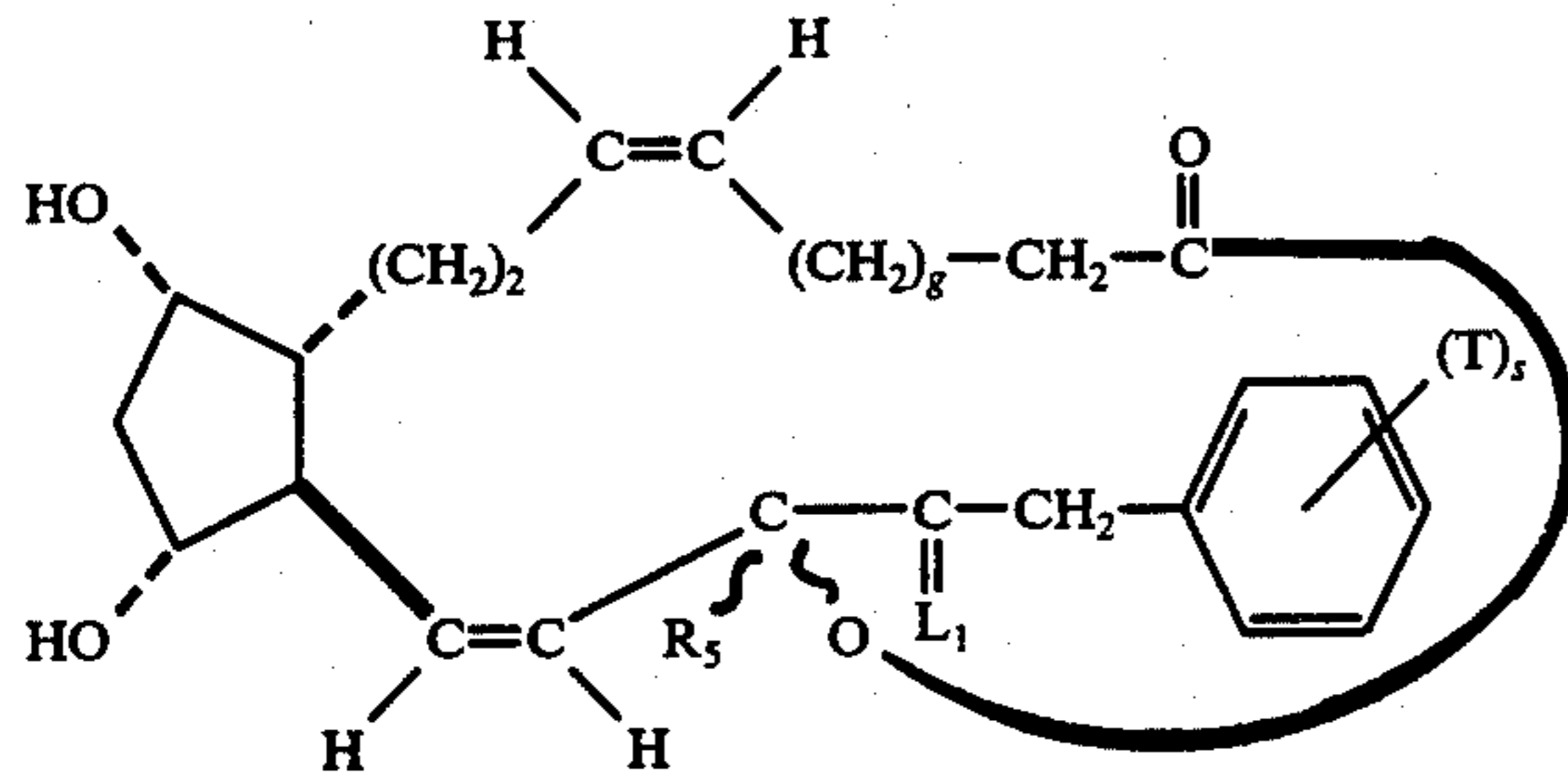
18,19,20-trinor-2,2-difluoro-cis-13-PGF 1α - type, 1,15-lactones
