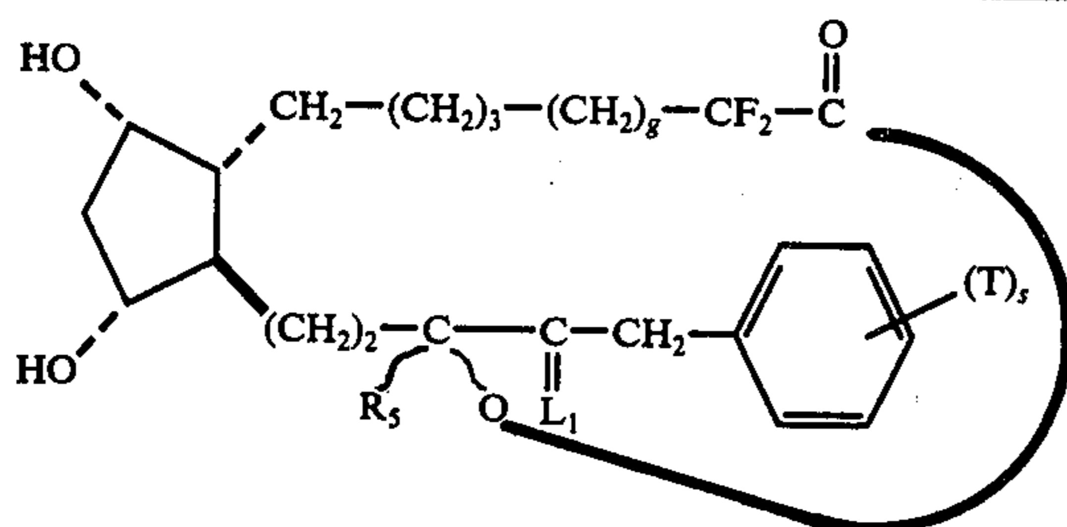
18,19,20-trinor-2,2-difluoro-13,14-dihydro- PGF 1α -type, 1,15-lactones
