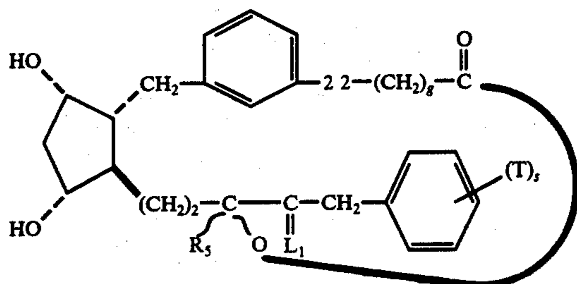
3,7-inter-m-phenylene-4,5,6,18,19,20-hexanor-13,14-dihydro-PGF 1α -type, 1,15-lactones
