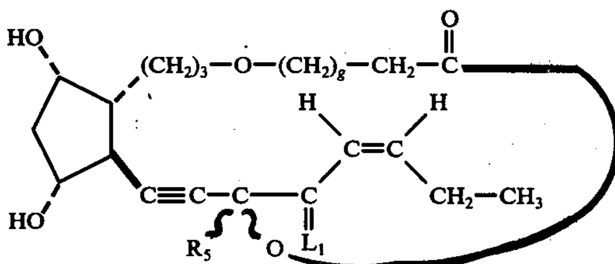
13,14-didehydro-4-oxa-cis-17,18-didehydro- PGF 1α -type, 1,15-lactones
