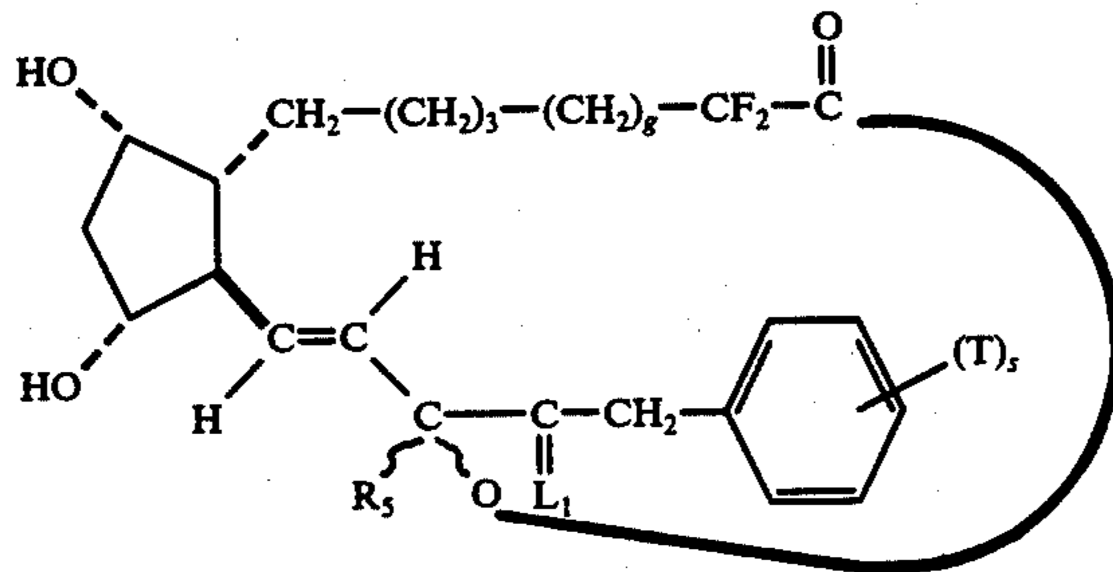
18,19,20-trinor-2,2-difluoro-PGF 1α -type, 1,15-lactones
