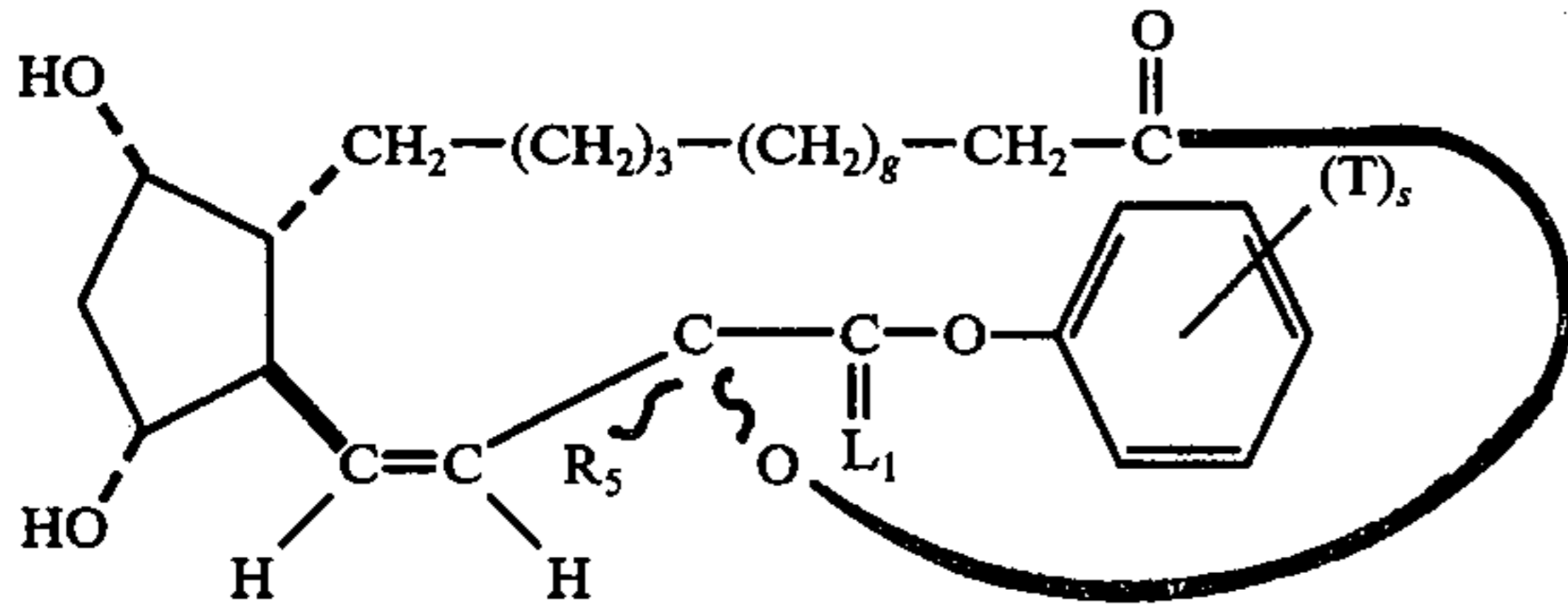
cis-13-PGF 1 \alpha -type, 1,15-lactones
