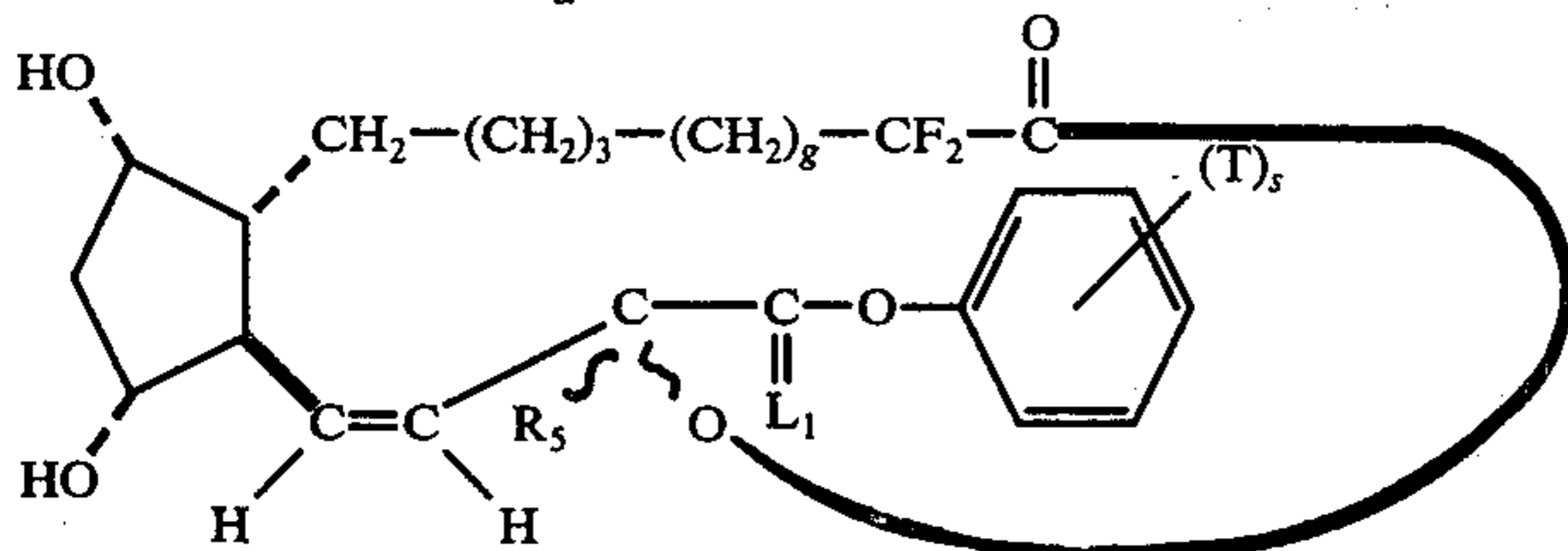
2,2-difluoro-cis-13-PGF 1 \alpha -type, 1,15-lactones
