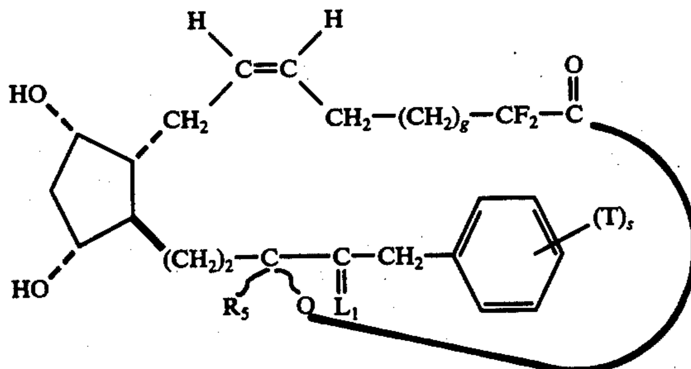
18,19,20-trinor-2,2-difluoro-13,14-dihydro- PGF 2α -type, 1,15-lactones
