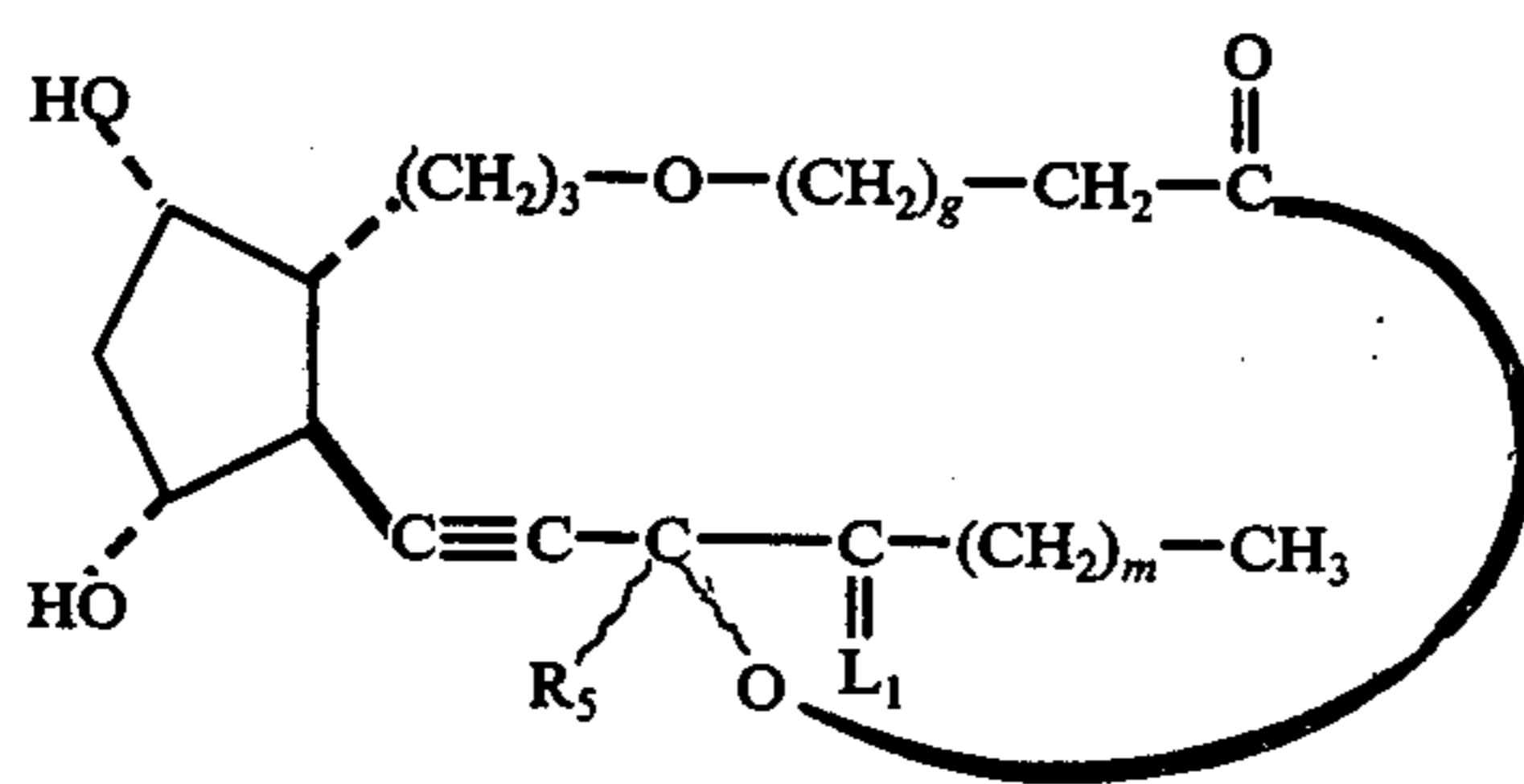
13,14-didehydro-4-oxa-PGF 1α -type, 1,15-lactones
