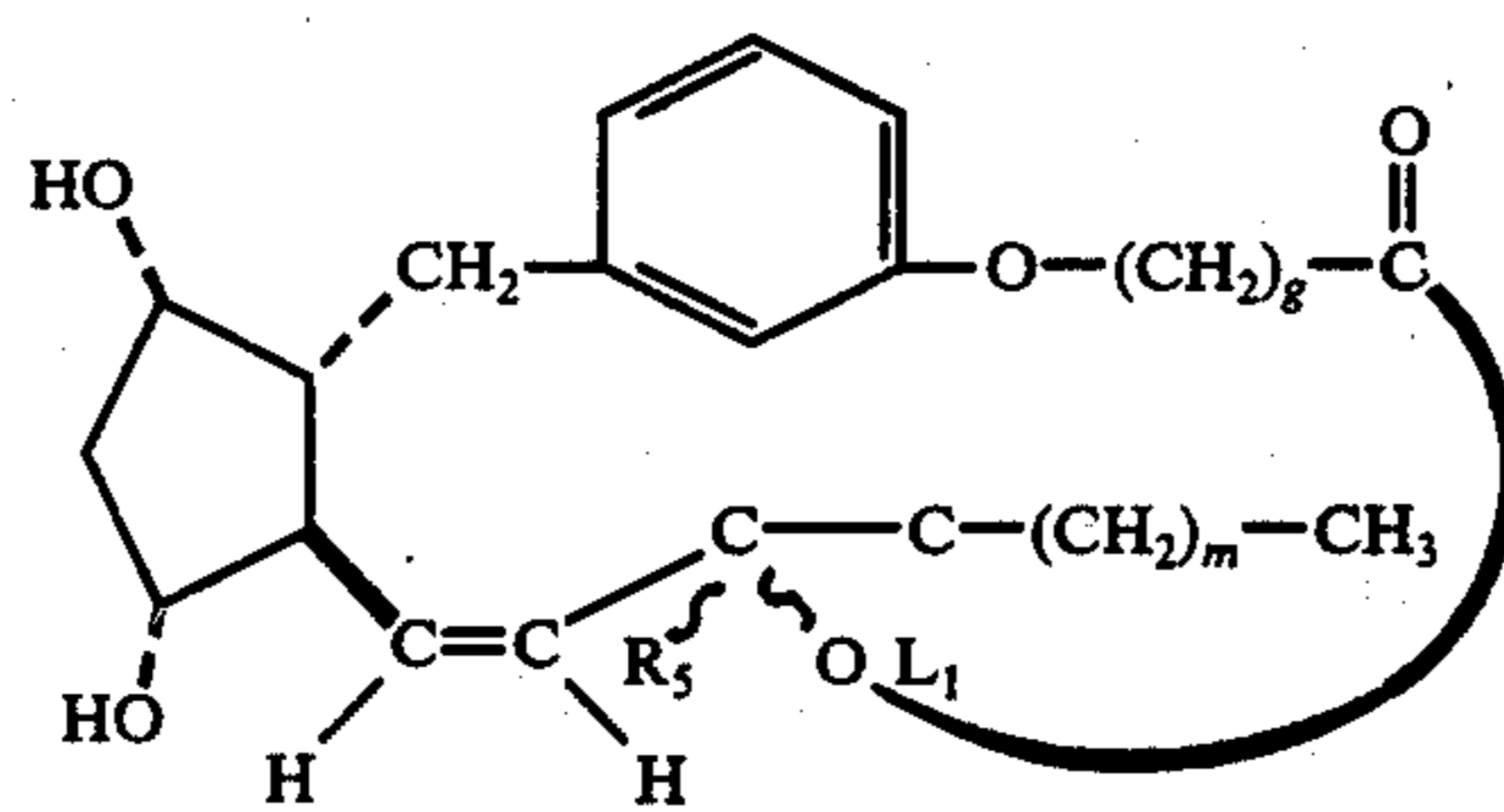
3,7-inter-m-phenylene-3-oxa-4,5,6-trinor-cis-13-PGD 1 -type, 1,15-lactones
