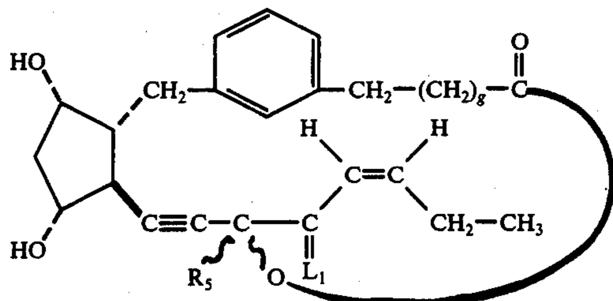
13,14-didehydro-3,7-inter-m-phenylene-4,5,6-trinor-cis-17,18-didehydro-PGF 1α -type, 1,15-lactones
