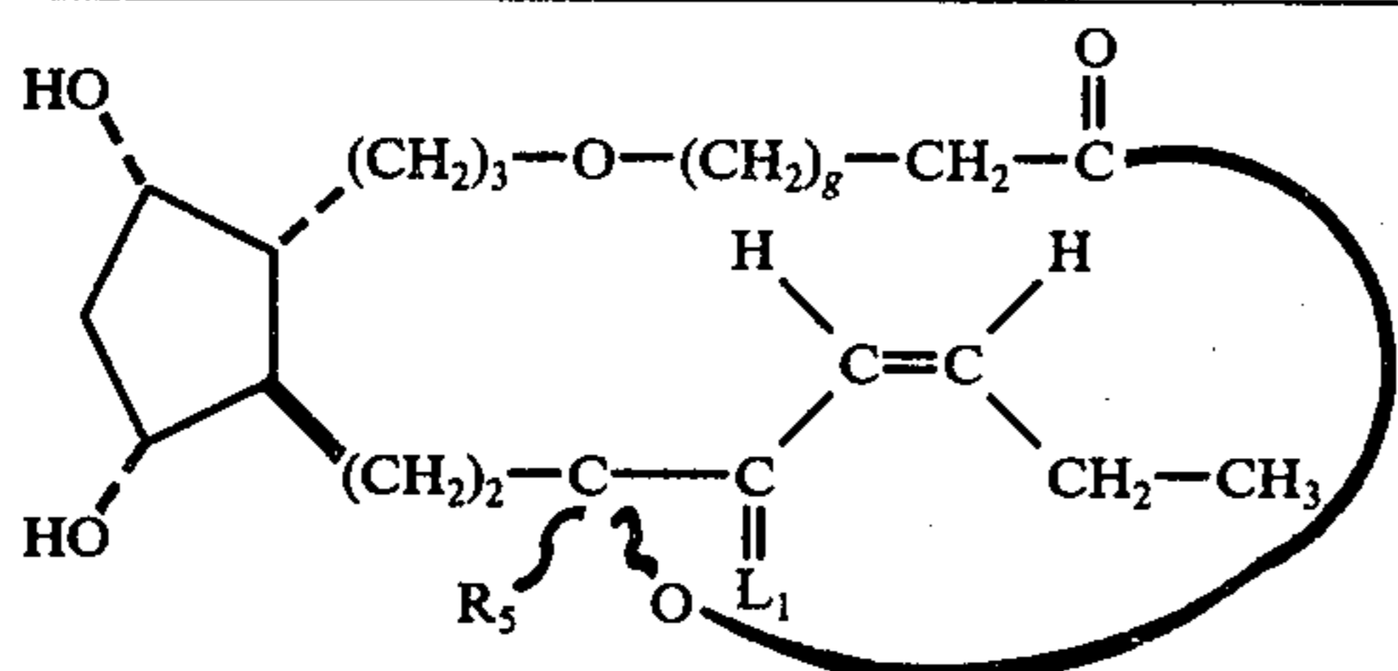
4-oxa-13,14-dihydro-17,18-didehydro-PGF 1α - type, 1,15-lactones
