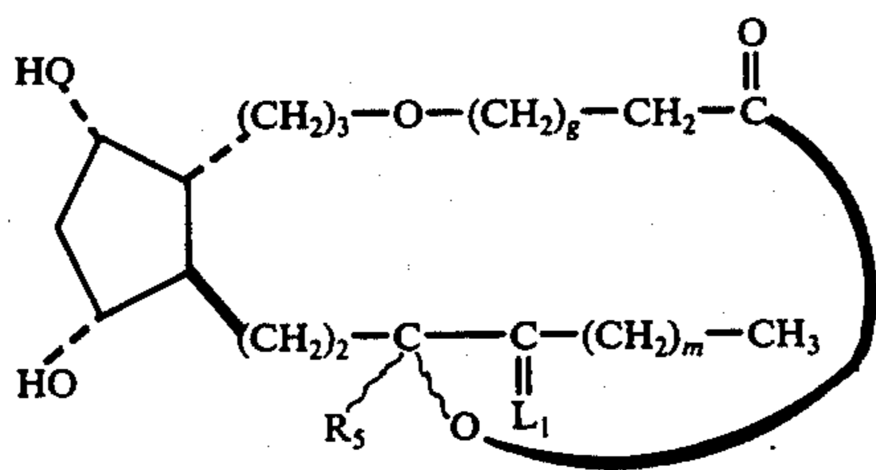
4-oxa-13,14-dihydro-PGF 1α -type, 1,15-lactones
