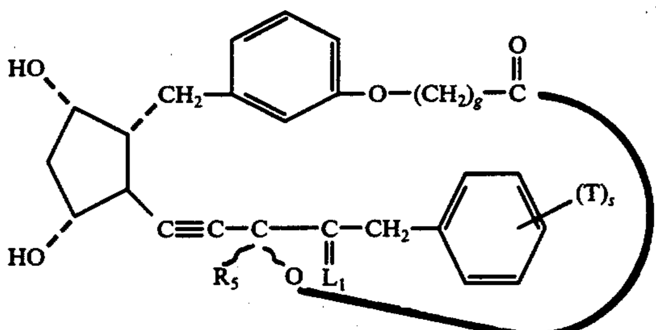
13,14-didehydro-3,7-inter-m-phenylene-3-oxa-4,5,6,18,19,20-hexanor-PGF 1α -type, 1,15-lactones
