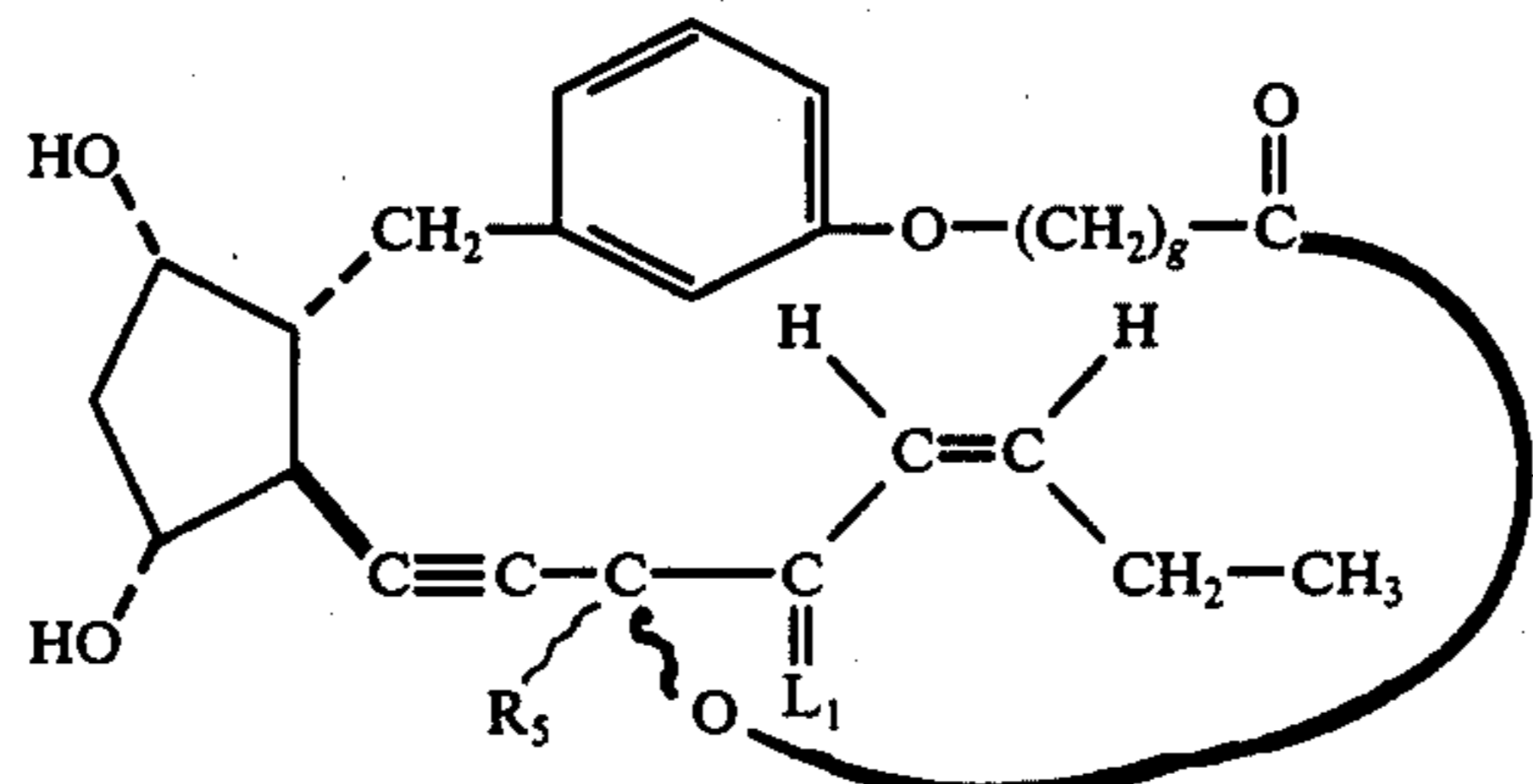
13,14-didehydro-3,7-inter-m-phenylene-3-oxa-4,5,6-trinor-cis-17,18-didehydro-PGF 1α -type, 1,15-lactones
