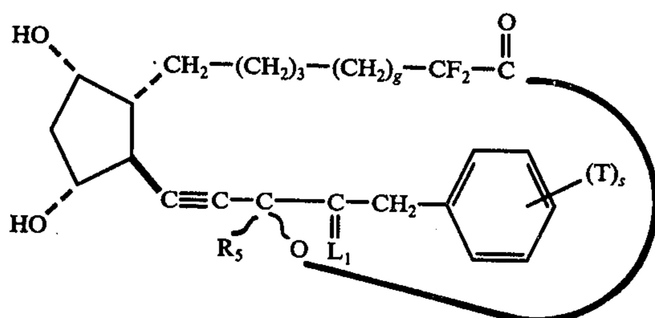
13,14-didehydro-18,19,20-trinor-2,2-difluoro- PGF 1α -type, 1,15-lactones
