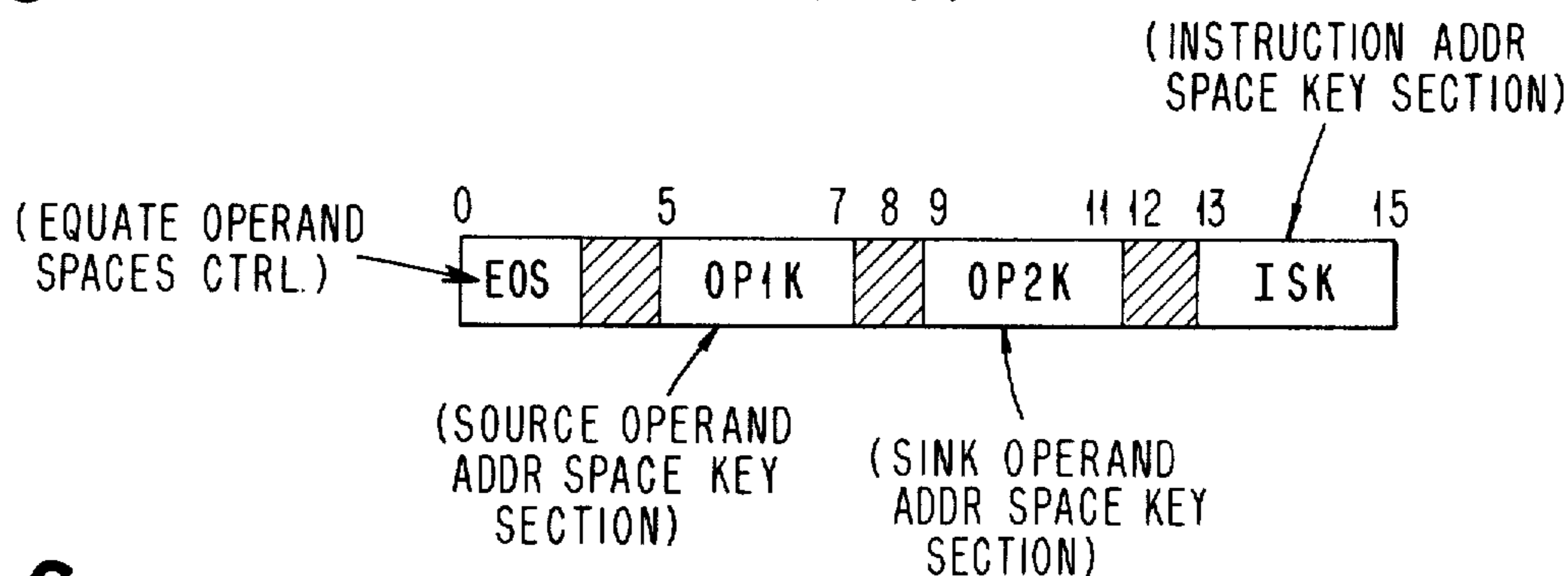
FIG. 5 (PROCESSOR ADDRESS KEY REG (AKR))
