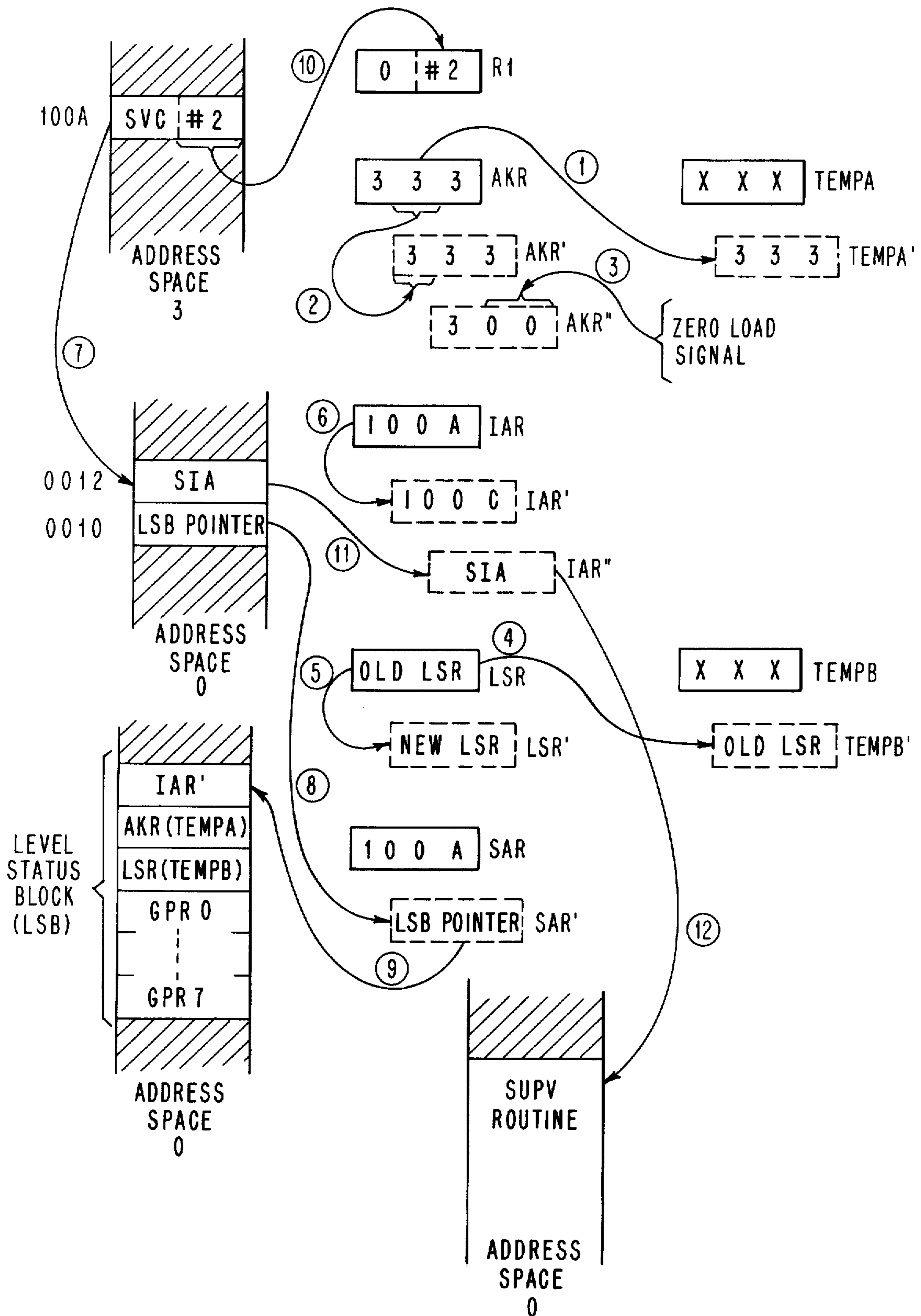
FIG. 18 (SVC EXECUTION EXAMPLE)
