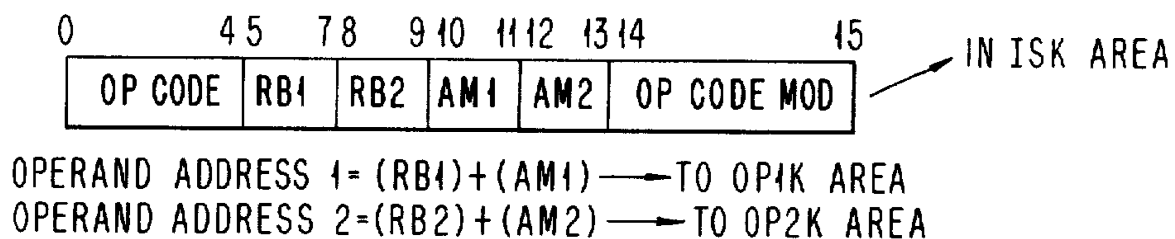
FIG. 12 INSTRUCTION OPERAND FORMAT
