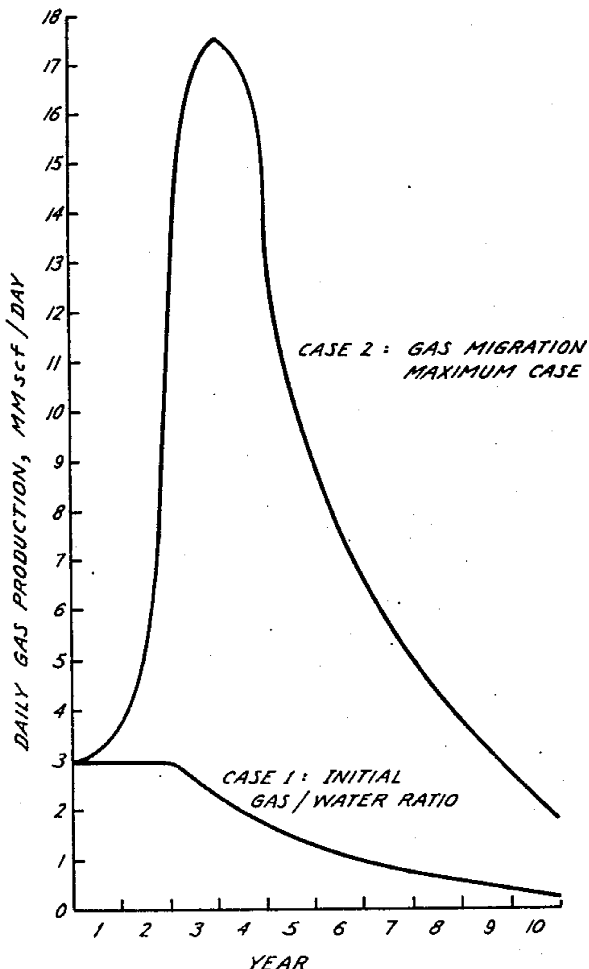
PRODUCTION HISTORY, 3 MILE RADIUS RESERVOIR
