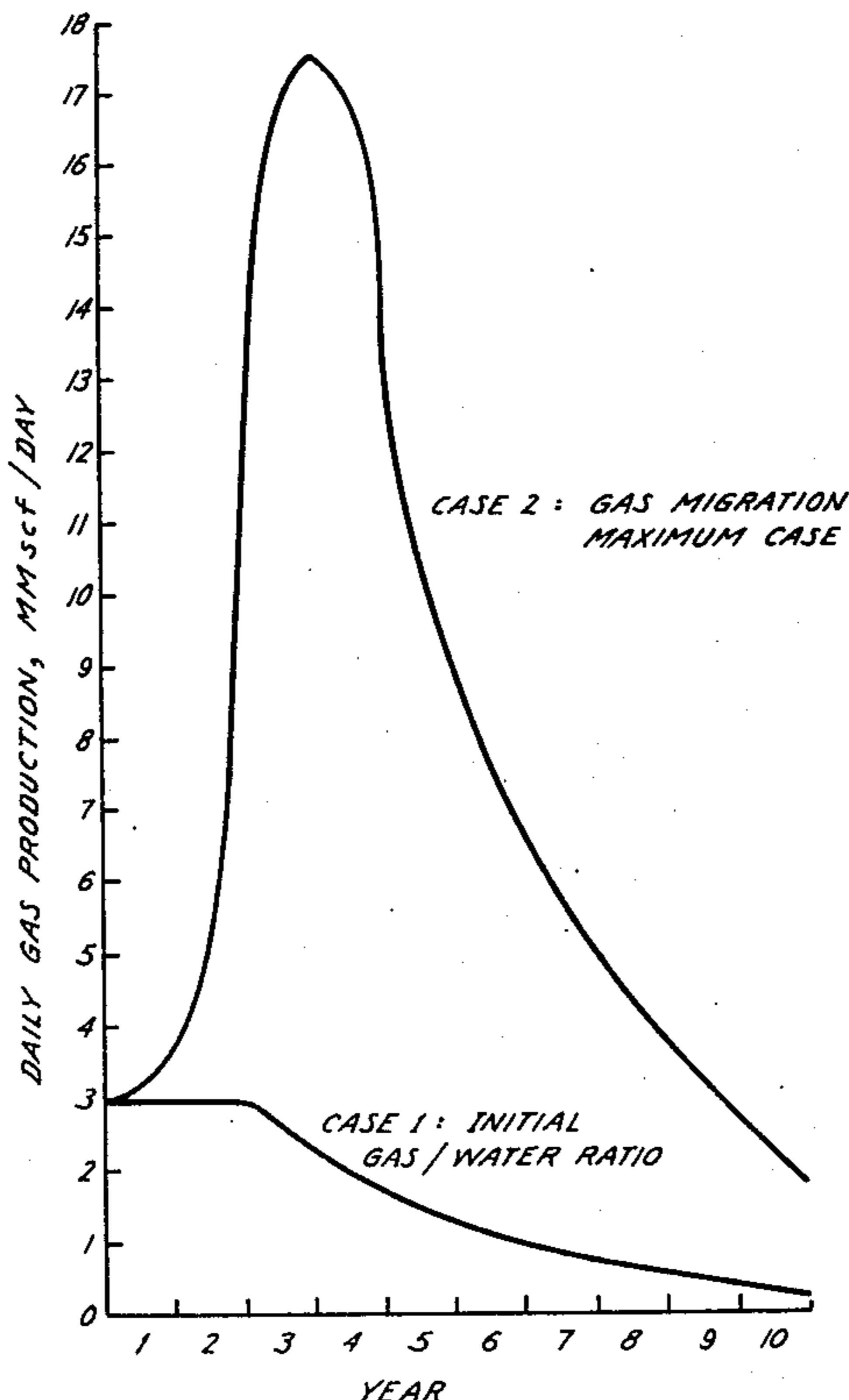
PRODUCTION HISTORY, 3 MILE RADIUS RESERVOIR
