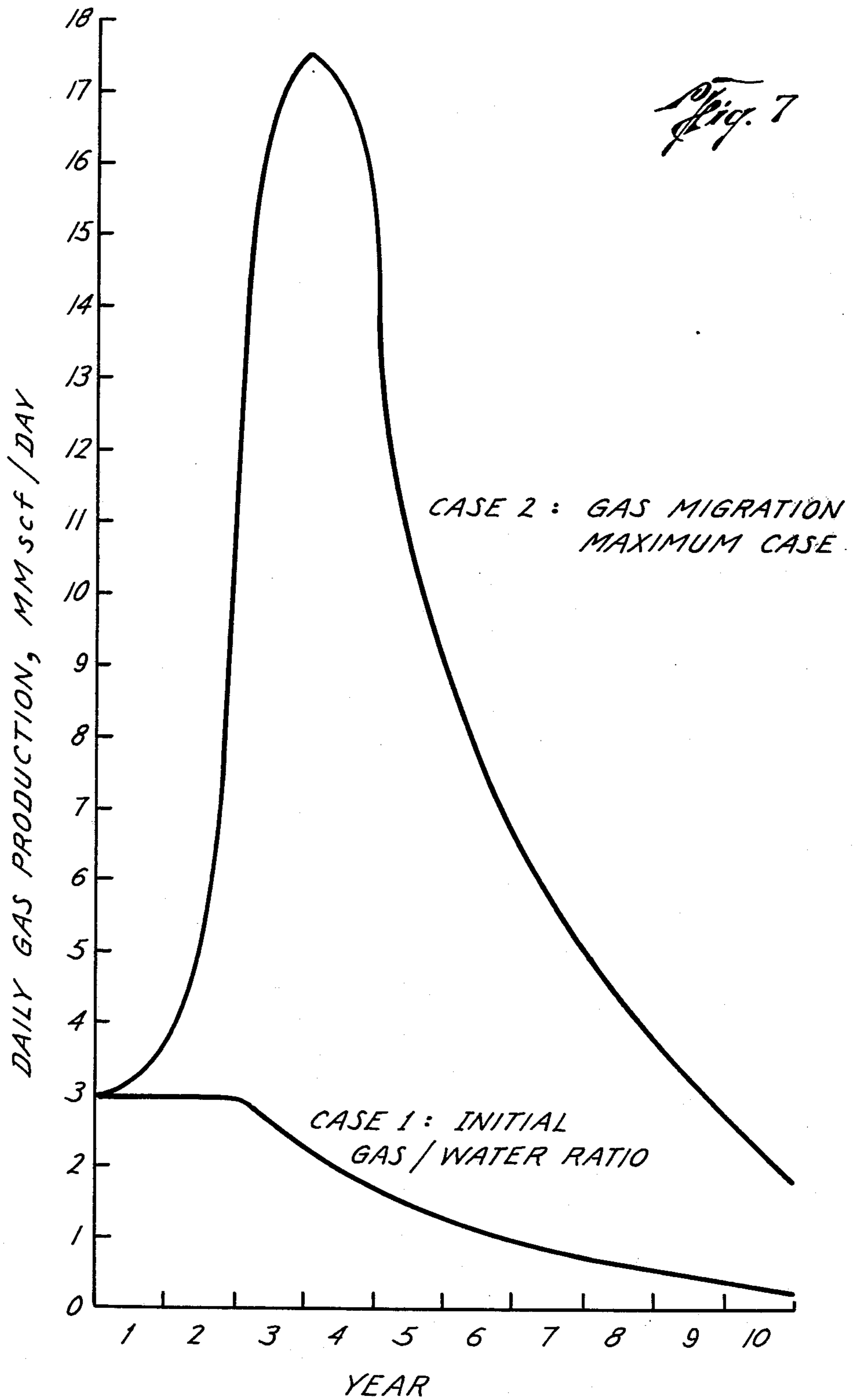
PRODUCTION HISTORY, 3 MILE RADIUS RESERVOIR
