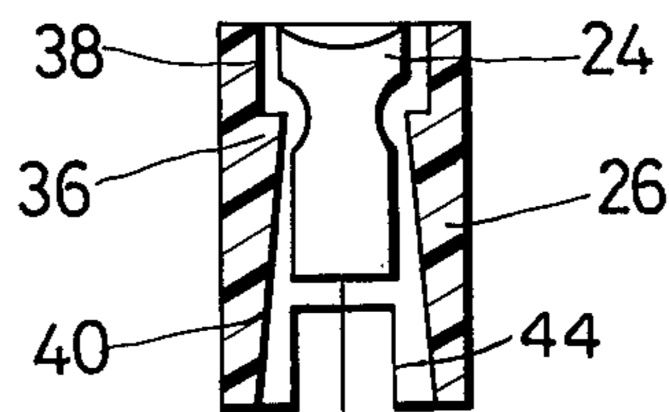
(PRIOR ART) Fig.1
