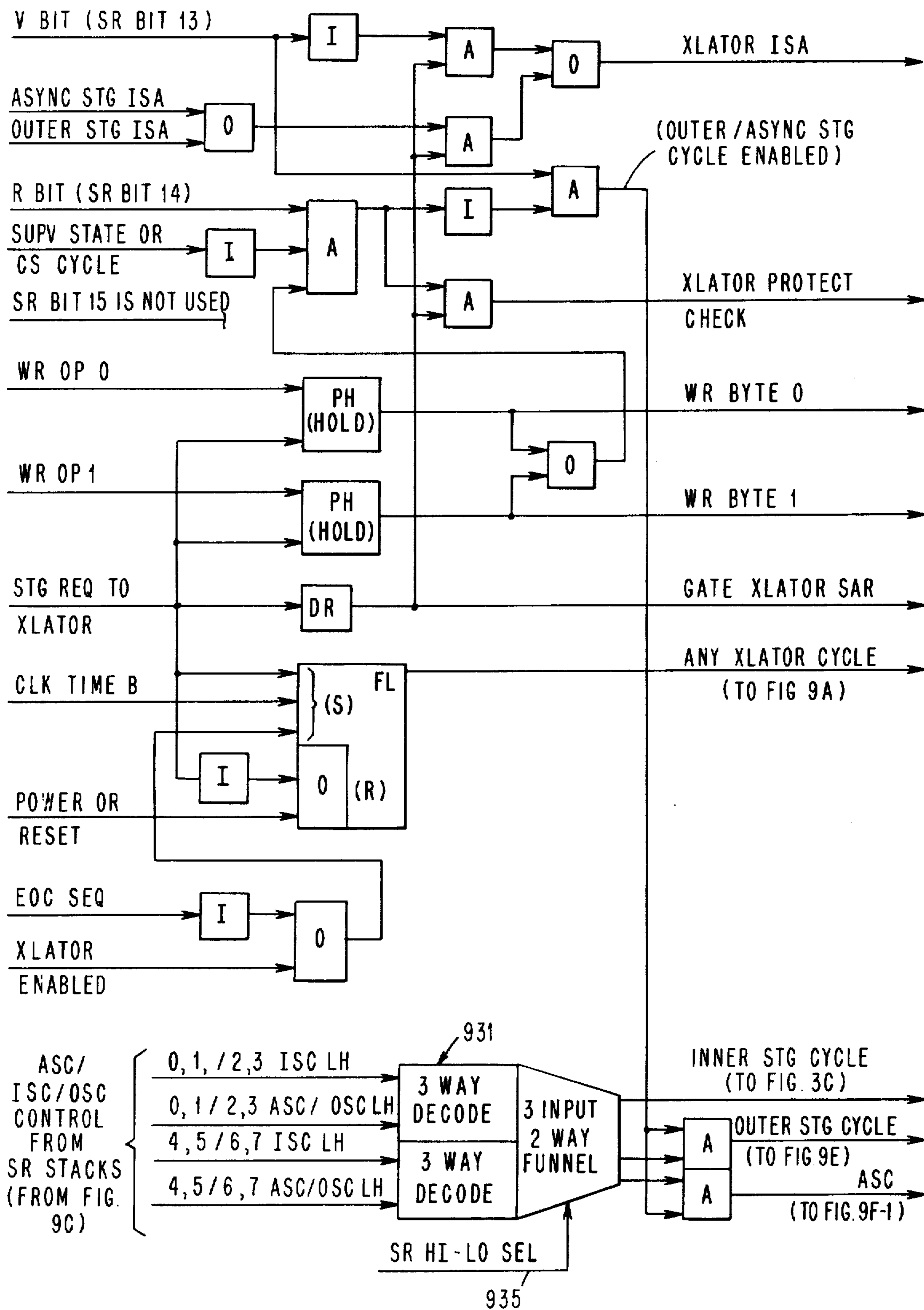
FIG. 9D-1 (BASIC CONTROLS FOR TRANSLATE CYCLE)
