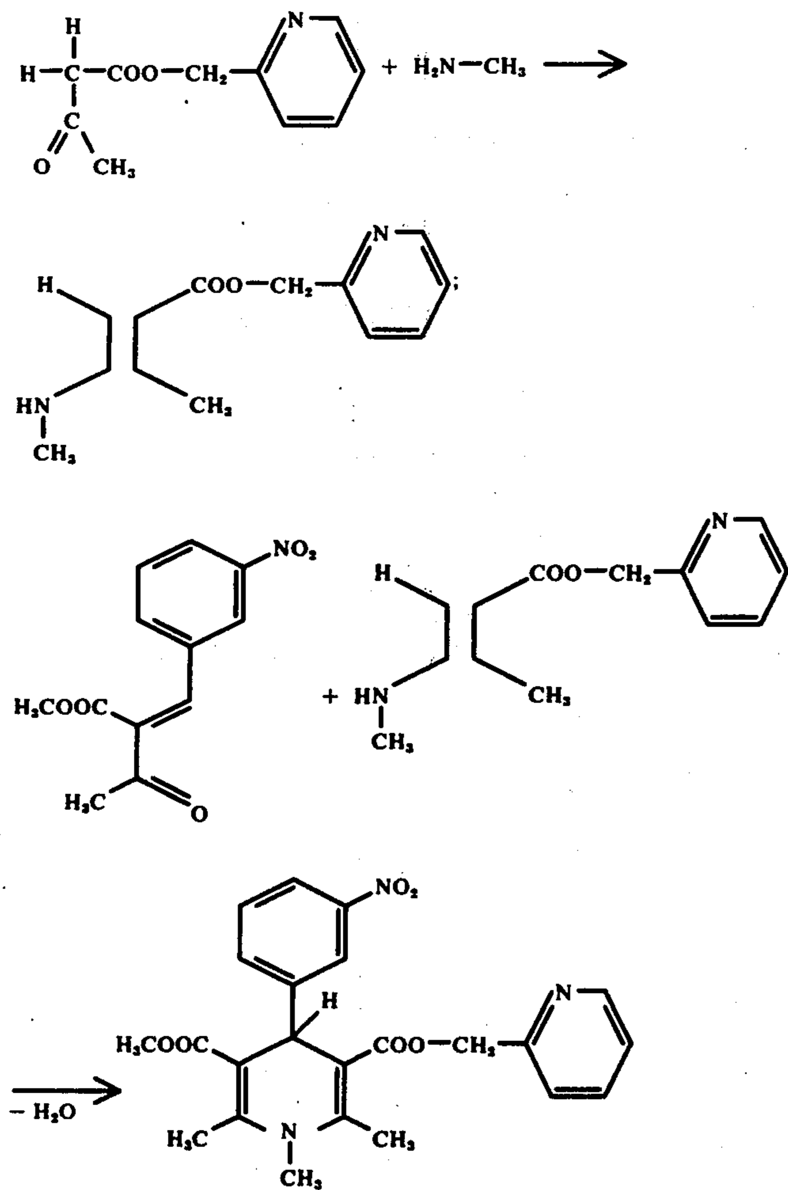
Scheme 1
