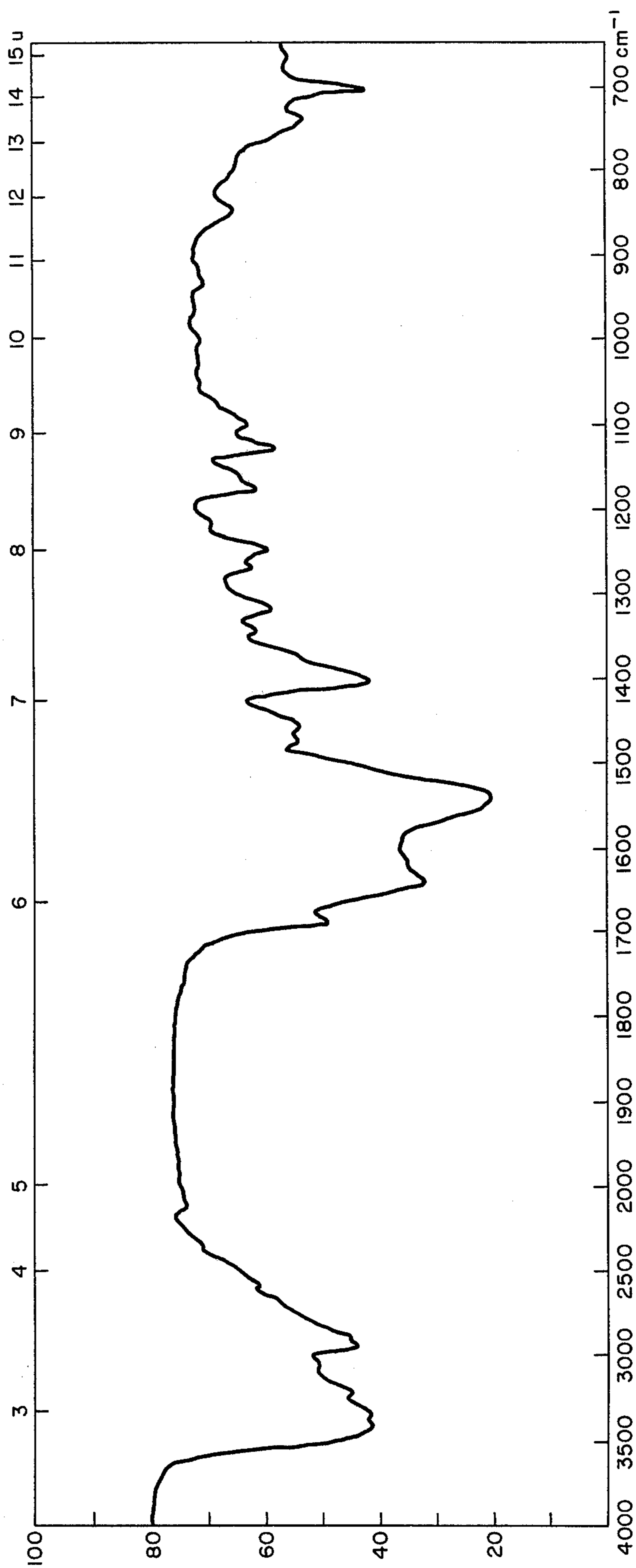
FIG. 2 INFRARED ABSORPTION SPECTRUM OF BESTATIN (KBr)
