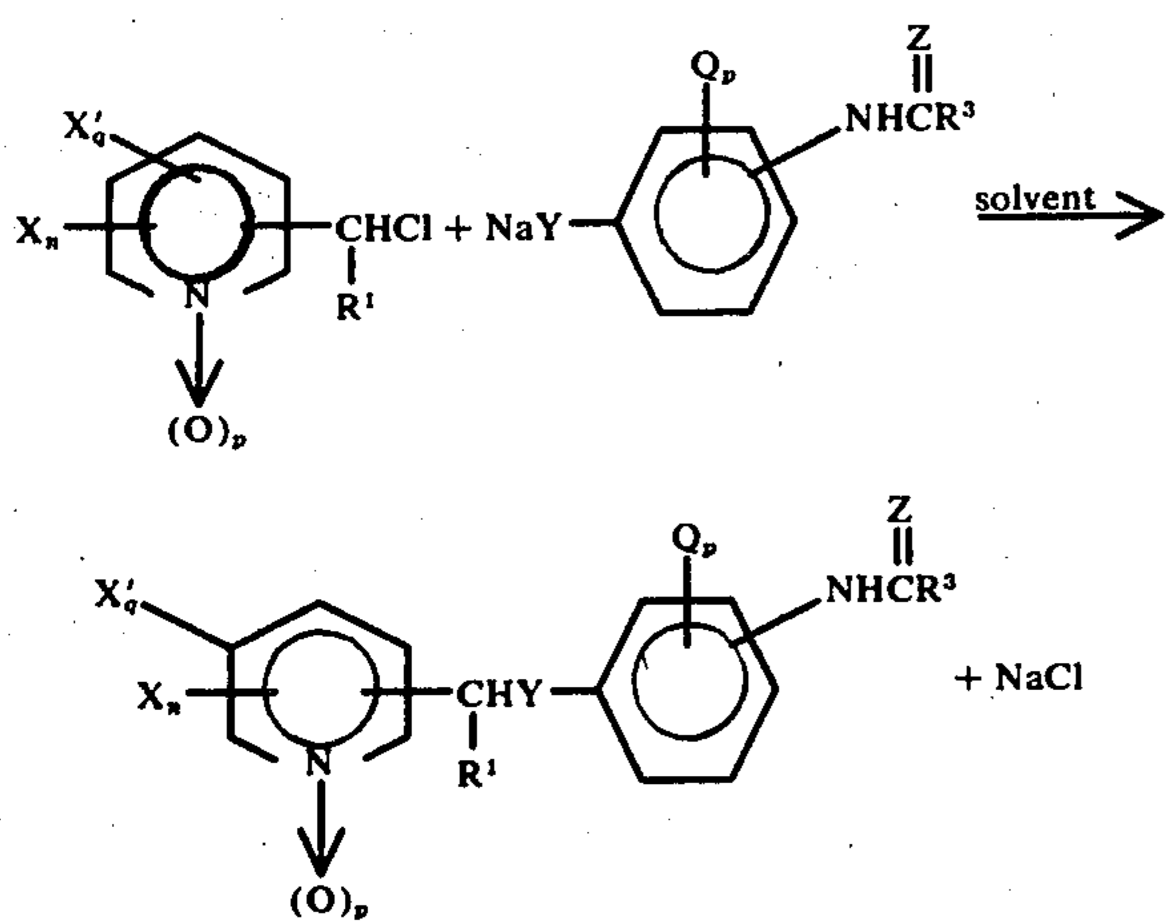
REACTION I
