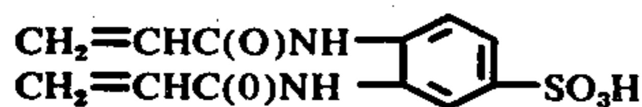
1,2-bis(acrylamido)-4-phenylsulfonic acid
