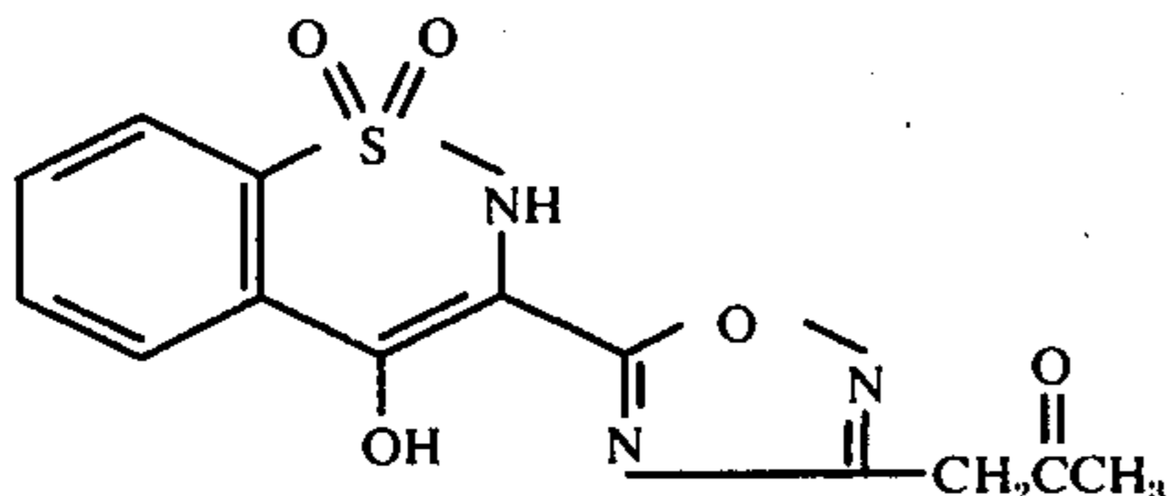
1-[[5-(4-Hydroxy-2H-1,2-benzothiazin-3-yl)-1,2,4-oxadiazol-3-yl]methyl]ethanone S,S-dioxide
