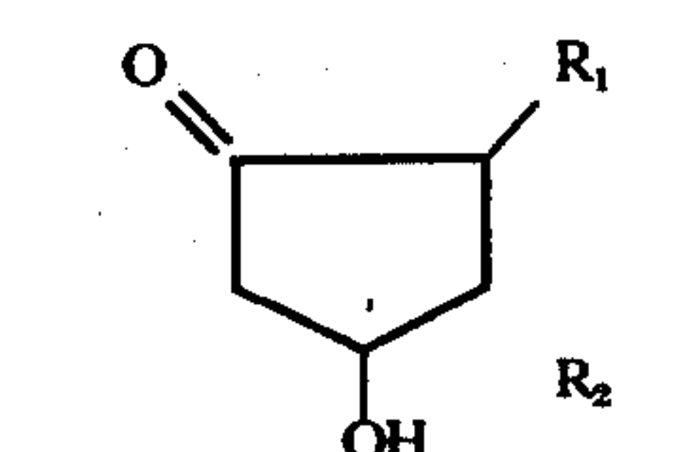
Nucleus of Prostaglandins E (II)
