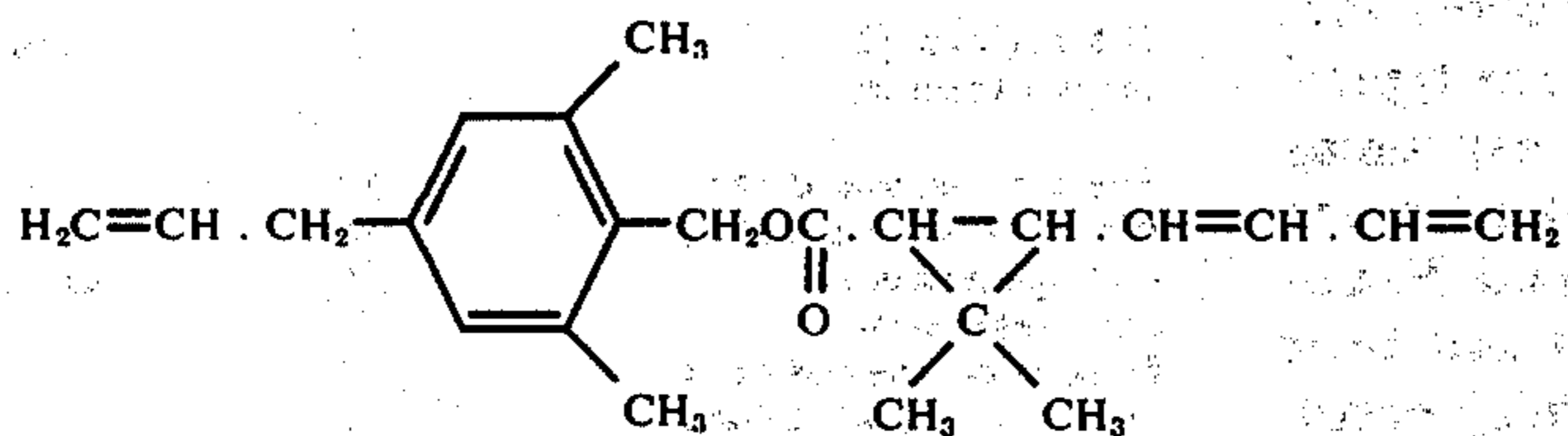
2,6-Dimethyl-4-allylbenzyl 2',2'- dimethyl-3'-(1'',3''-butadienyl)-cyclo- propanecarboxylate
