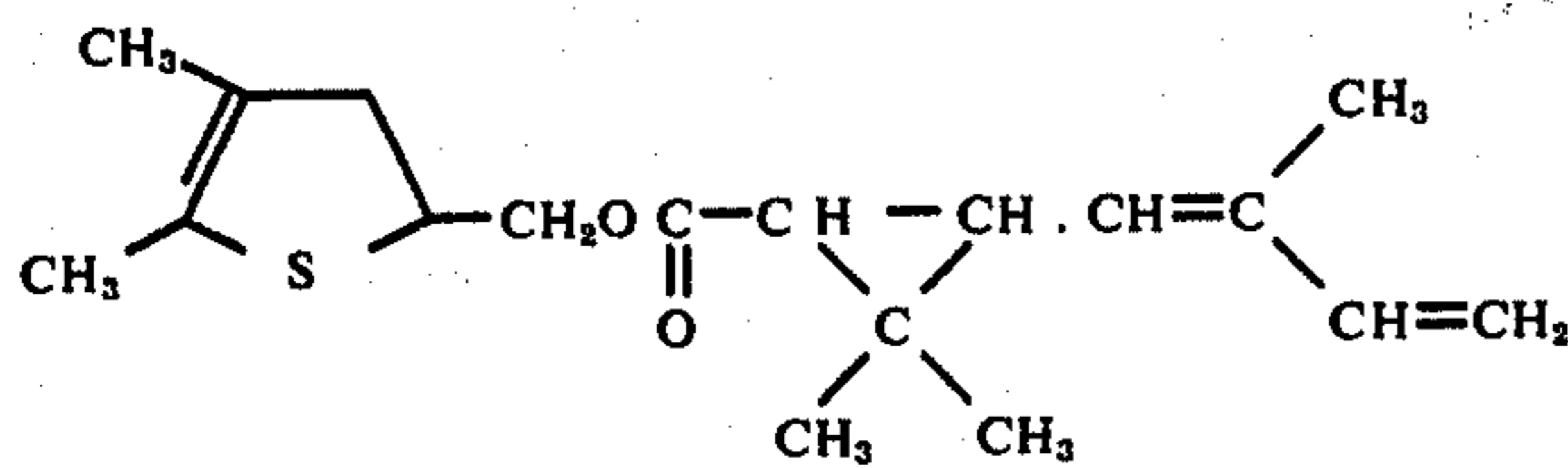
4,5-Dimethylfurfuryl 2',2'-dimethyl-3'-(2''-methyl-1'',3''-butadienyl)-cyclopropanecarboxylate
