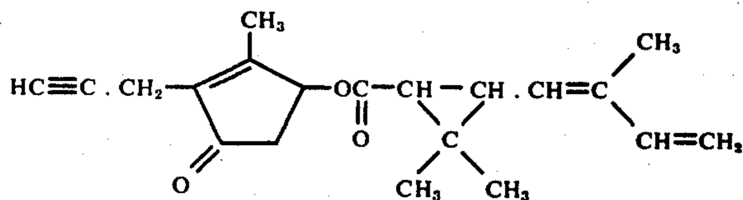
2-Propargyl-3-methyl-2-cyclopentene-1-one-4-yl 2',2'-dimethyl-3'-(2''-methyl-1'',3''-butadienyl)-cyclopropanecarboxylate
