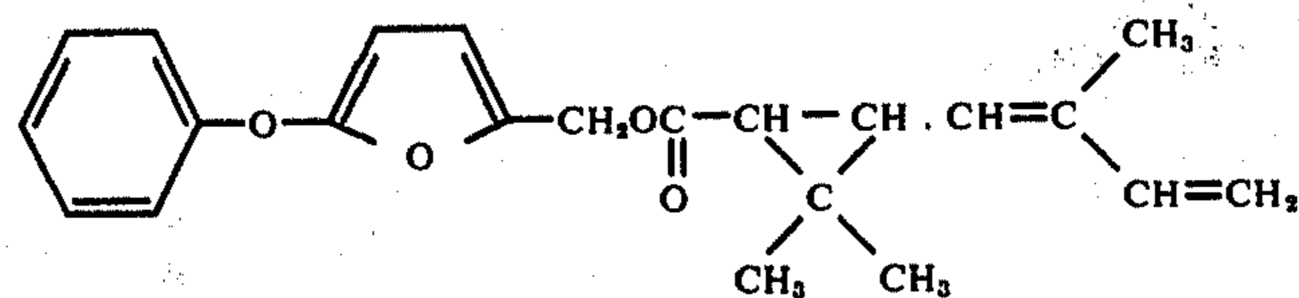
5-Oxa-4,5,6,7-tetrahydrobenzofurfuryl-2',2'-dimethyl-3'-(2''-methyl-1'',3''-butadienyl)-cyclopropanecarboxylate
