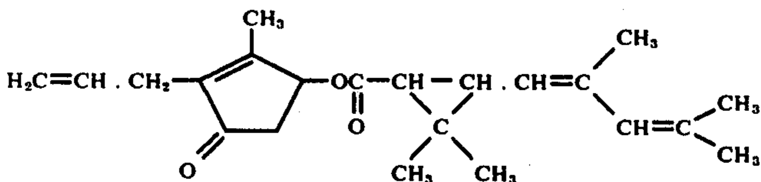
2-Allyl-3-methyl-2-cyclopentene-1-one-yl 2',2'-dimethyl-3'-(2'',4''-dimethyl-1'',3''- pentadienyl)-cyclopropanecarboxylate
