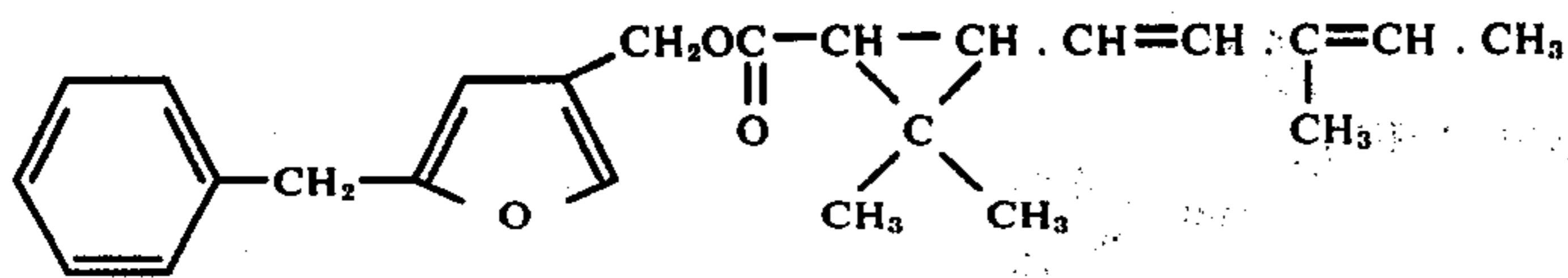
5-Benzyl-3-furymethyl 2',2'-dimethyl-3'-(3''-methyl-1'',3''-pentadienyl)-cyclopropanecarboxylate
