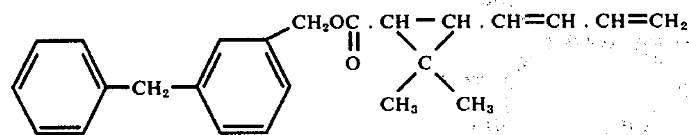
3-Benzylbenzyl 2',2'-dimethyl-3'-(1'',3''-butadienyl)-cyclopropanecarboxylate
