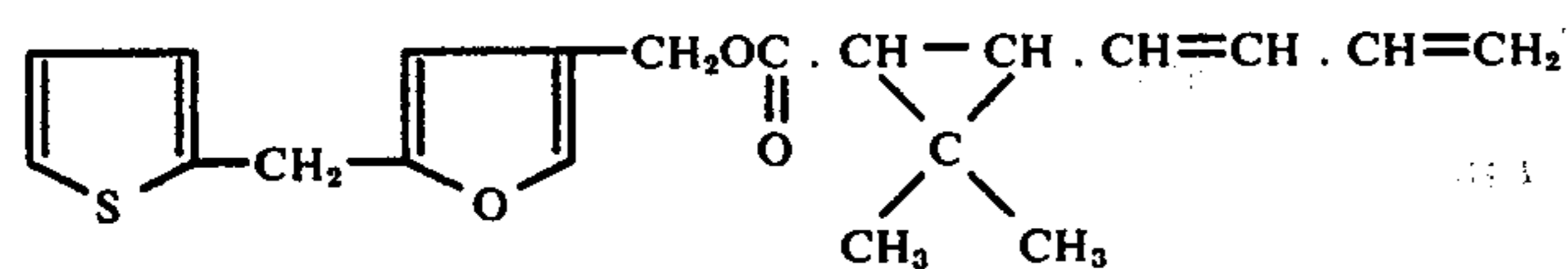
5-(2'-Thienyl)-3-furymethyl 2',2'-dimethyl-3'-(1'',3''-butadienyl)-cyclopropanecarboxylate
