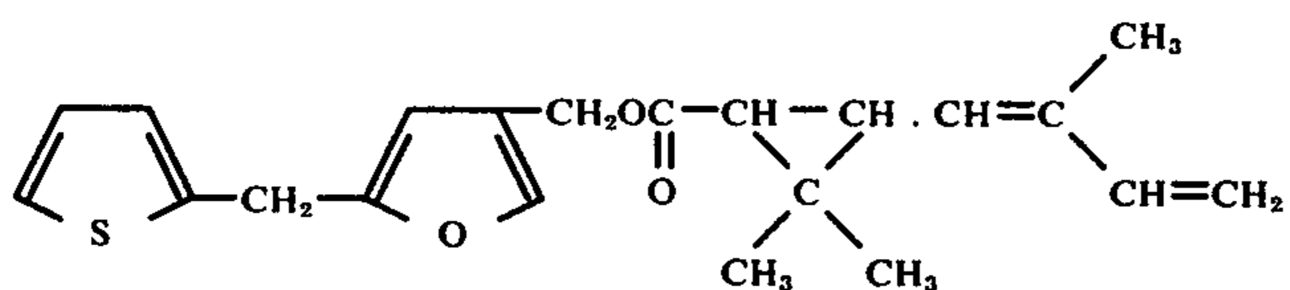
5-(2'-Thienyl)-3-furylmethyl 2',2'-dimethyl-3'-(2''-methyl-1'',3''-butadienyl)-cyclopropanecarboxylate
