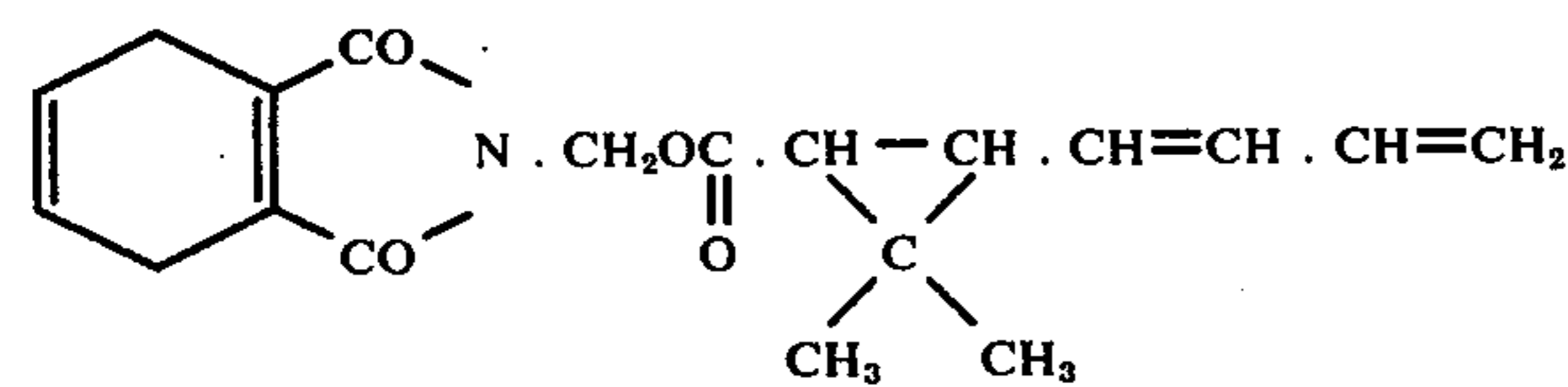
3,6-Dihydrophthalimidomethyl 2',2'- dimethyl-3'-(1'',3''-butadienyl)- cyclopropanecarboxylate
