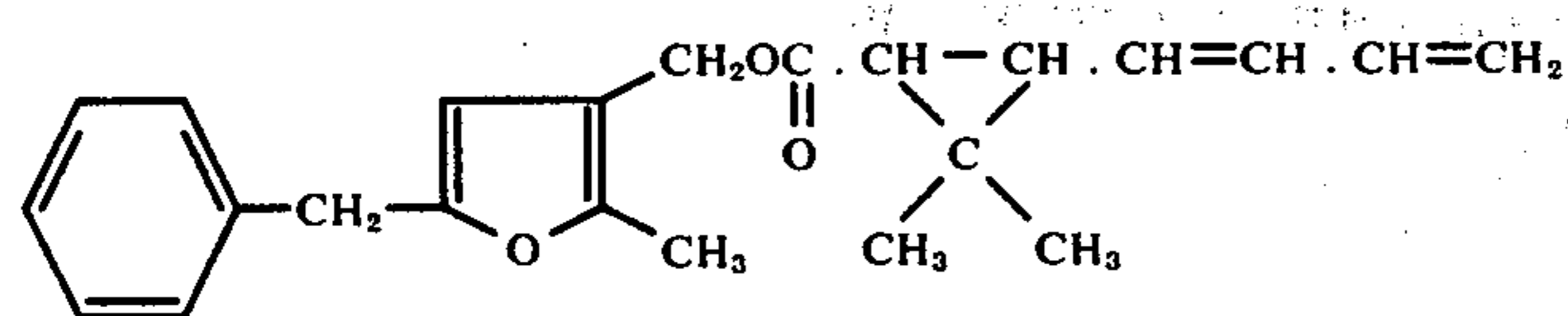
2-Methyl-5-benzyl-3-furymethyl-2',2'-dimethyl-3'-(1'',3''-butadienyl)-cyclopropanecarboxylate
