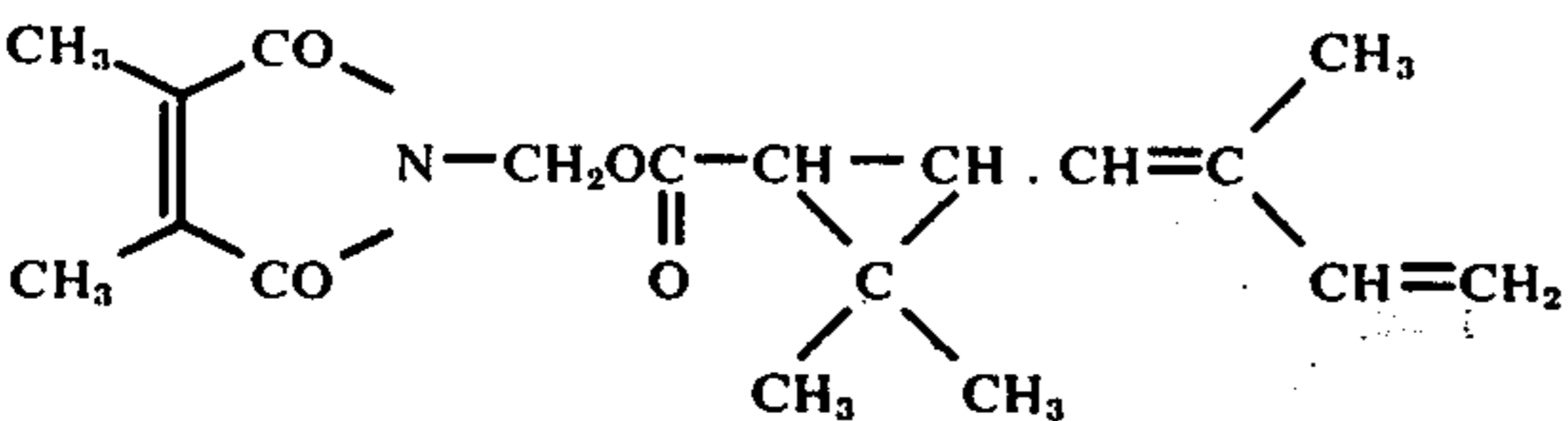
Dimethylmaleimidomethyl 2,2-dimethyl-3-(2'-methyl-1',3'-butadienyl)-cyclopropanecarboxylate
