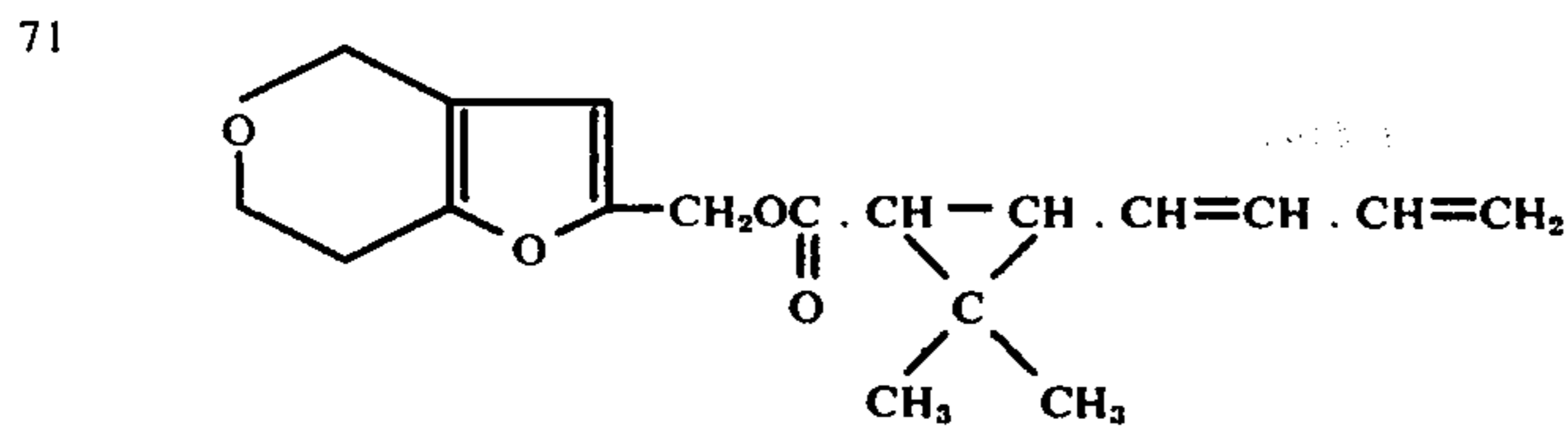
5-Oxa-4,5,6,7-tetrahydrobenzofurfuryl 2',2'-dimethyl-3'-(1'',3''-butadienyl)-cyclopropanecarboxylate
