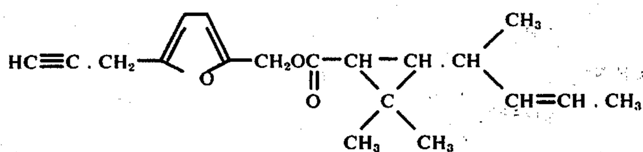
5-Propargylfurfuryl 2',2'-dimethyl-3'-(2''-methyl-1'',3''-pentadienyl)-cyclopropanecarboxylate
