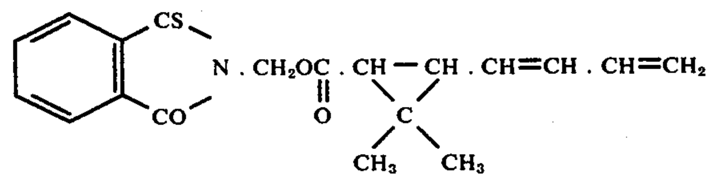
Monothiophthalimidomethyl 2',2'-dimethyl- 3'-(1'',3''-butadienyl)-cyclopropanecarboxylate
