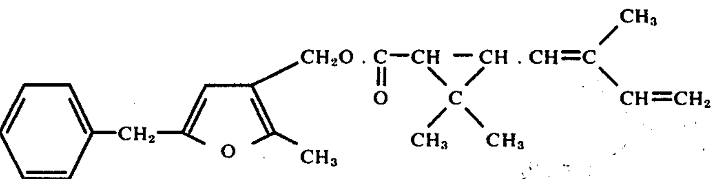
2-Methyl-5-benzyl-3-furylmethyl 2',2'-dimethyl-3'-(2''-methyl-1'',3''-butadienyl)-cyclopropanecarboxylate
