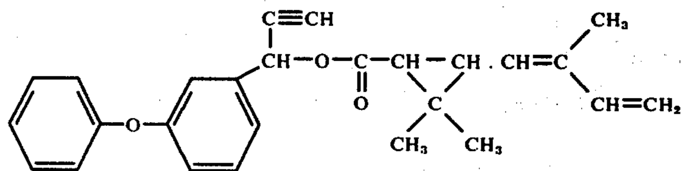
3-Phenoxy- \alpha -ethynylbenzyl 2',2'-dimethyl-3'-(2''-methyl-1'',3''-butadienyl)-cyclopropanecarboxylate
