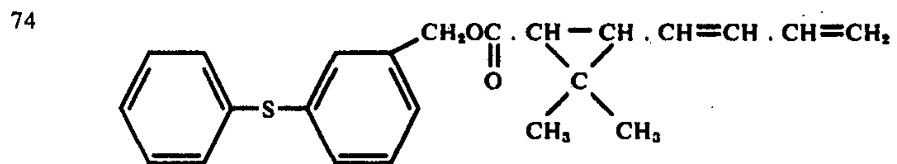
3-Phenylthiobenzyl 2',2'-dimethyl-3'-(1'',3''-butadienyl)-cyclopropanecarboxylate
