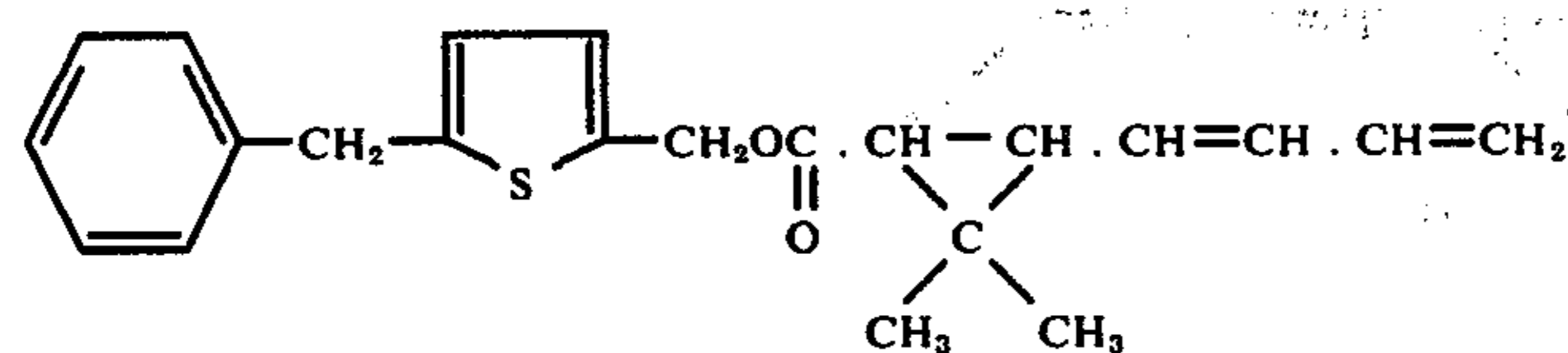
5-Benzyl-2-thienyl 2',2'-dimethyl-3'-(1'',3''-butadienyl)-cyclopropanecarboxylate
