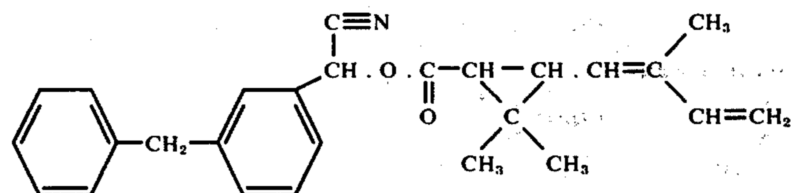
3-Benzyl-α-cyanobenzyl 2',2'-dimethyl-3'-(2''-methyl-1'',3''-butadienyl)-cyclopropanecarboxylate
