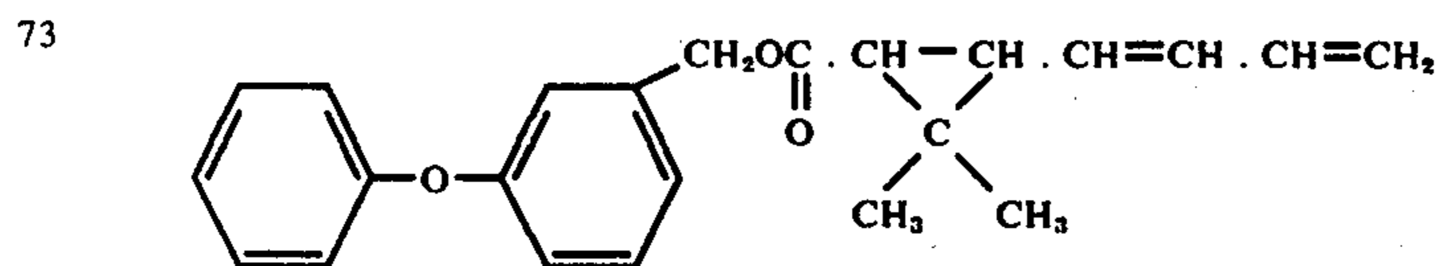
3-Phenoxybenzyl 2',2'-dimethyl-3'-(1'',3''-butadienyl)-cyclopropanecarboxylate
