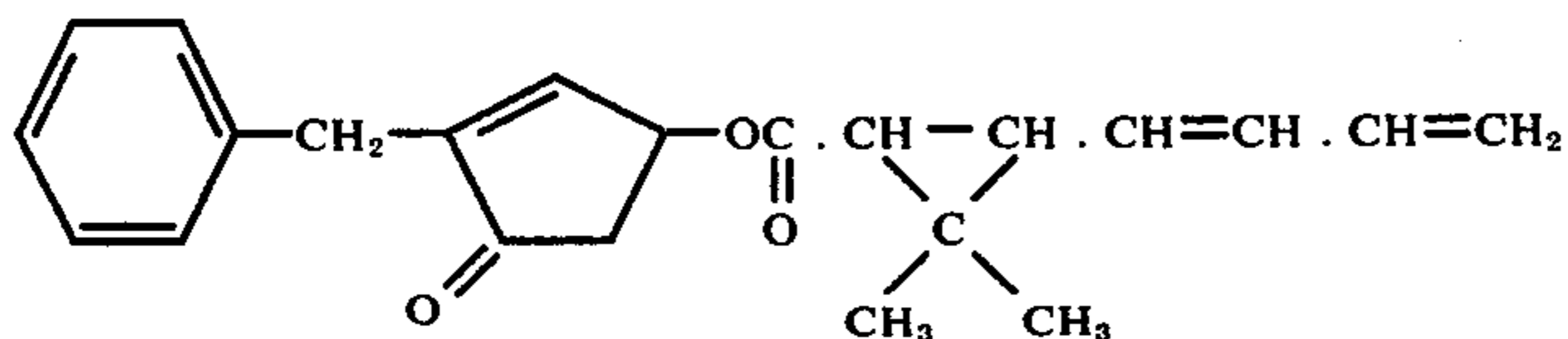
2-Benzyl-2-cyclopentene-1-one-4-yl 2',2'-dimethyl-3'-(1'',3''-butadienyl)- cyclopropanecarboxylate
