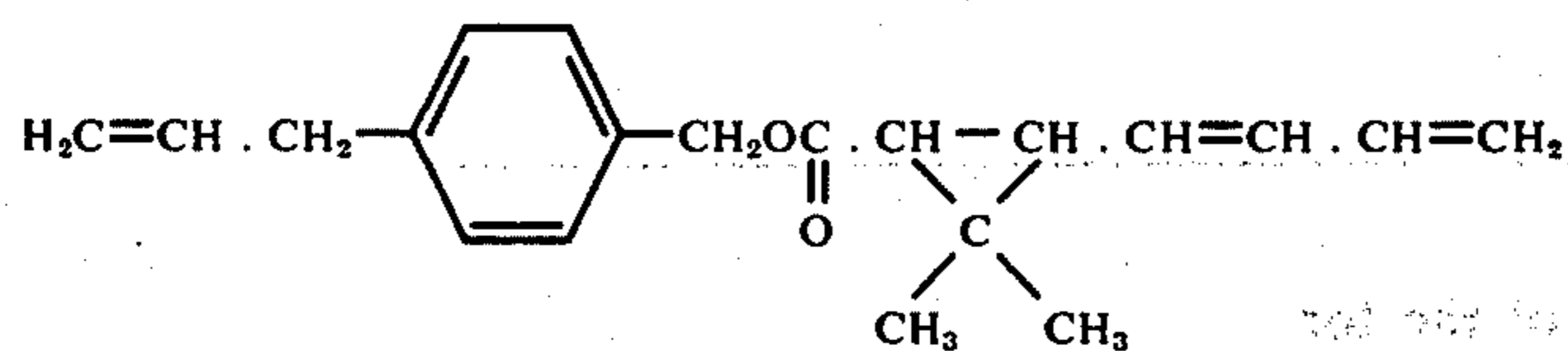
4-Allylbenzyl 2',2'-dimethyl-3'- (1'',3''-butadienyl)-cyclopropane- carboxylate
