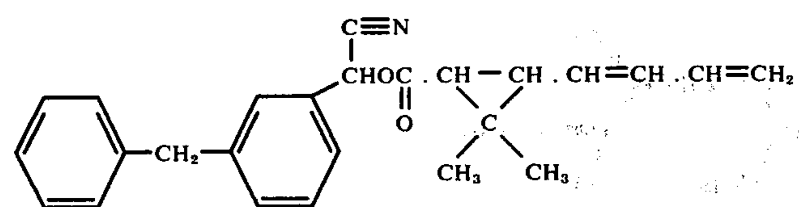
3-Benzyl-α-cyanobenzyl 2',2'-dimethyl-3'-(1'',3''-butadienyl)-cyclopropanecarboxylate
