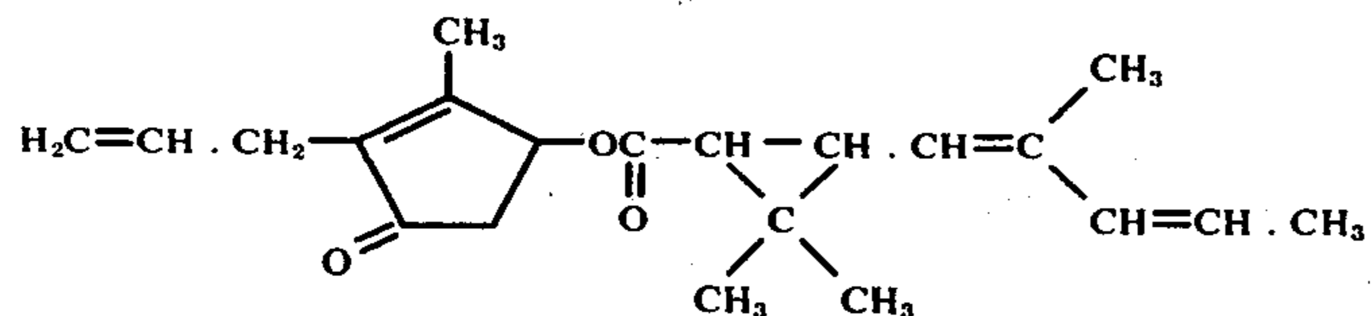
2-Allyl-3-methyl-2-cyclopentene-1-one-4-yl 2',2'-dimethyl-3'-(2''-methyl-1'',3''- pentadienyl)-cyclopropanecarboxylate
