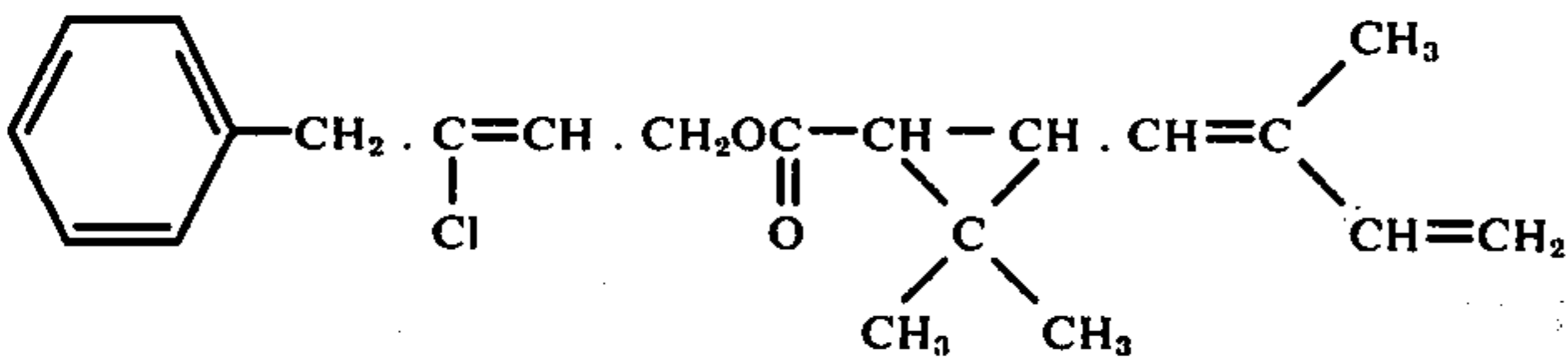
3-Chloro-4-phenyl-2-butene-1-yl 2,2'-dimethyl-3'-(2''-methyl-1'',3''-butadienyl)-cyclopropanecarboxylate
