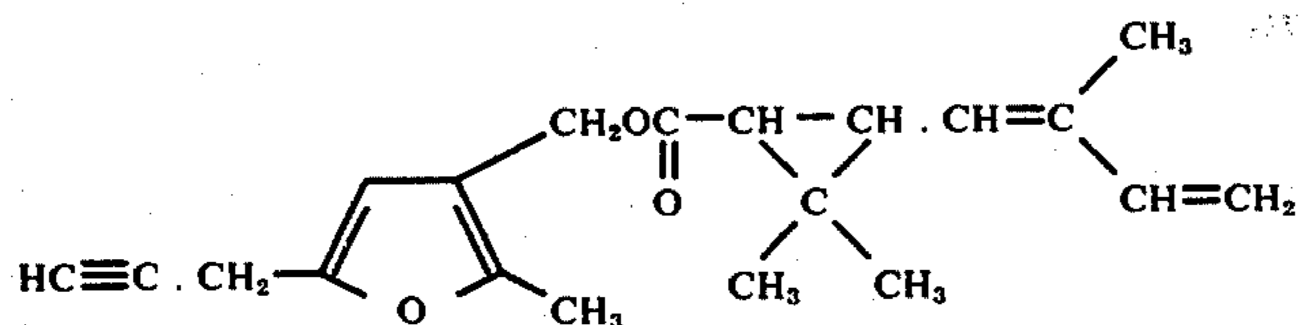
2-Methyl-5-propargyl-3-furylmethyl 2',2'-dimethyl-3'-(2''-methyl-1'',3''-butadienyl)-cyclopropanecarboxylate
