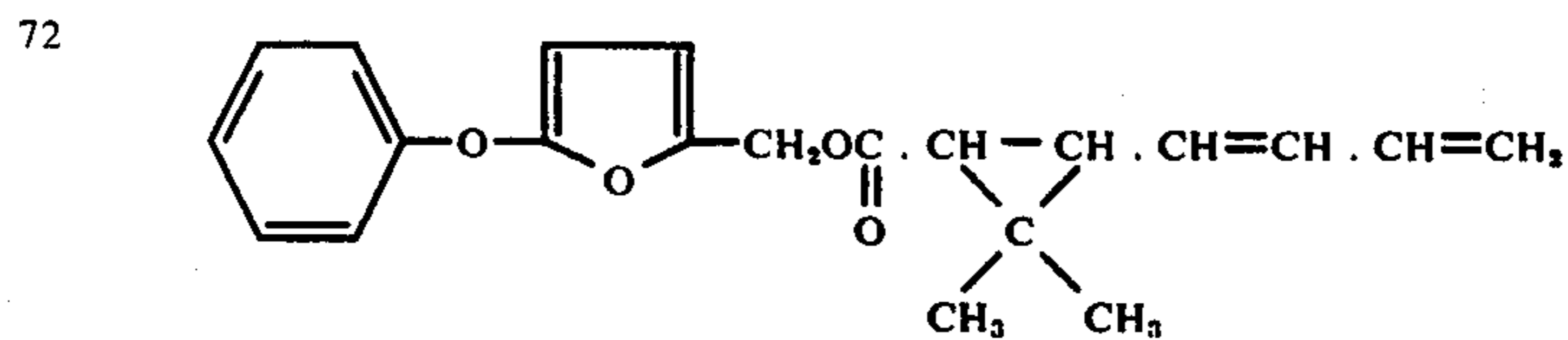
5-Phenoxyfurfuryl 2',2'-dimethyl-3'-(1'',3''-butadienyl)-cyclopropanecarboxylate
