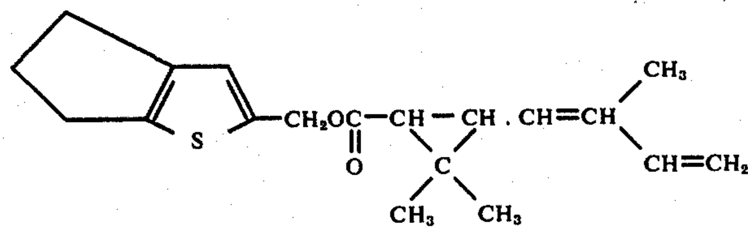
4,5-Trimethylene-2-thienyl 2',2'-dimethyl-3'-(2''-methyl-1'',3''-butadienyl)-cyclopropanecarboxylate
