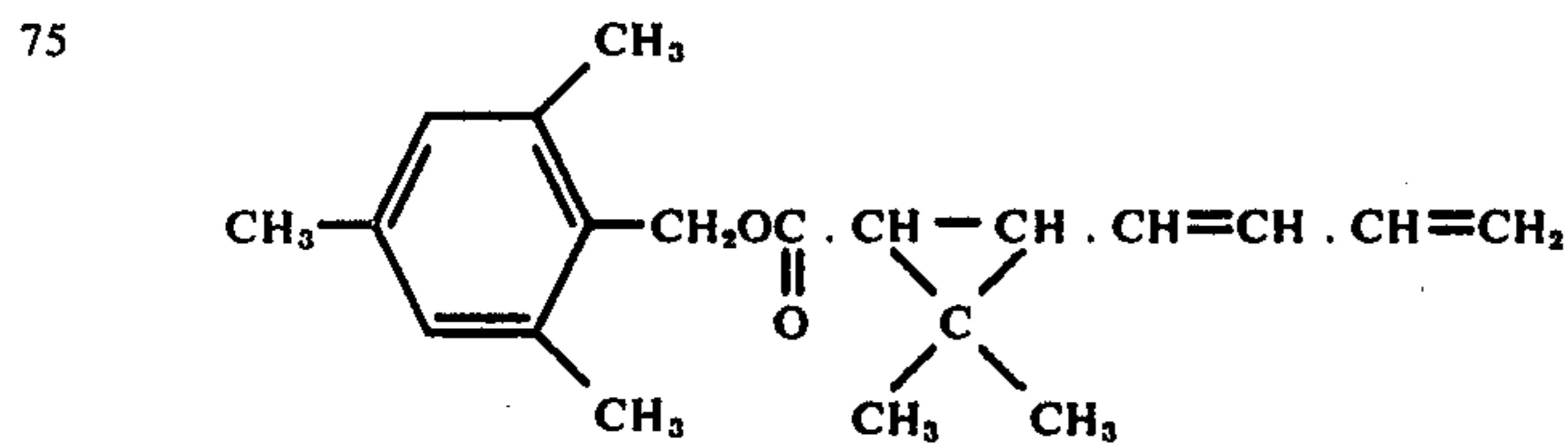
2,4,6-Trimethylbenzyl 2',2'-dimethyl-3'-(1'',3''-butadienyl)-cyclopropanecarboxylate
