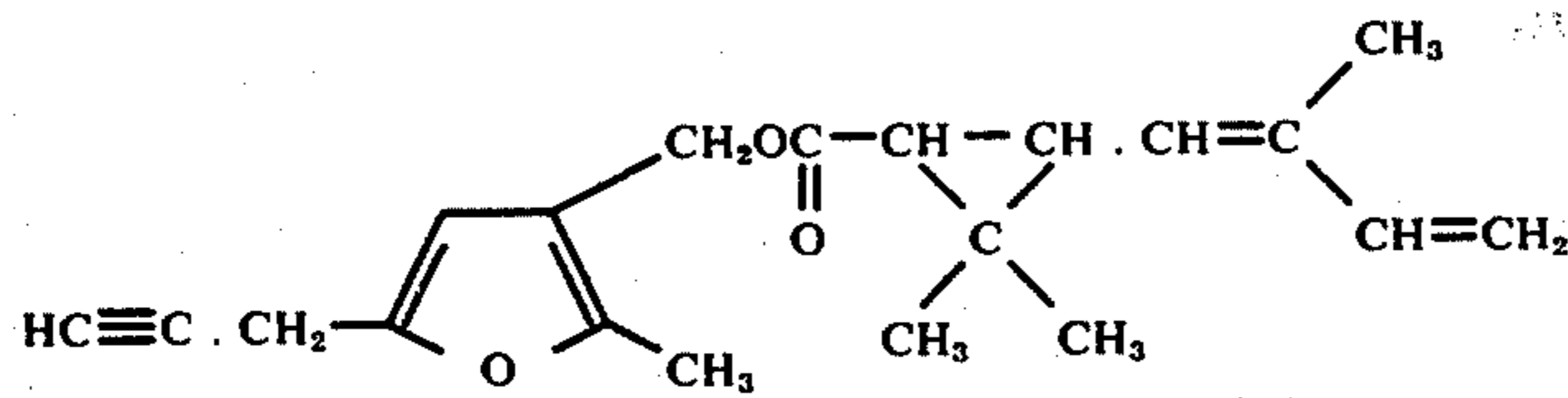
2-Methyl-5-propargyl-3-furylmethyl 2',2'-dimethyl-3'-(2''-methyl-1'',3''-butadienyl)-cyclopropanecarboxylate
