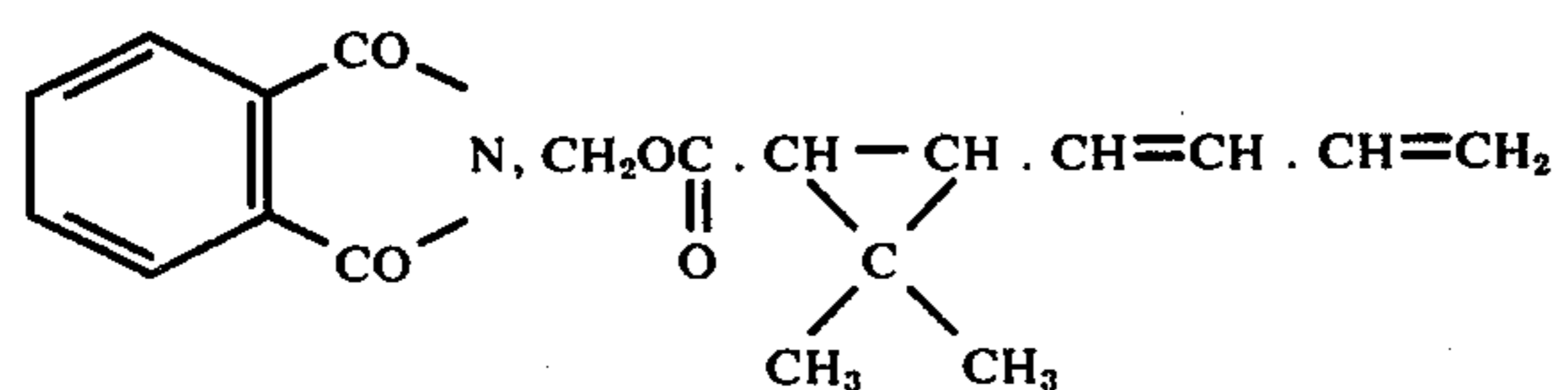
Phthalimidomethyl 2', 2'-dimethyl-3'- (1'',3''-butadienyl)-cyclopropanecarboxylate
