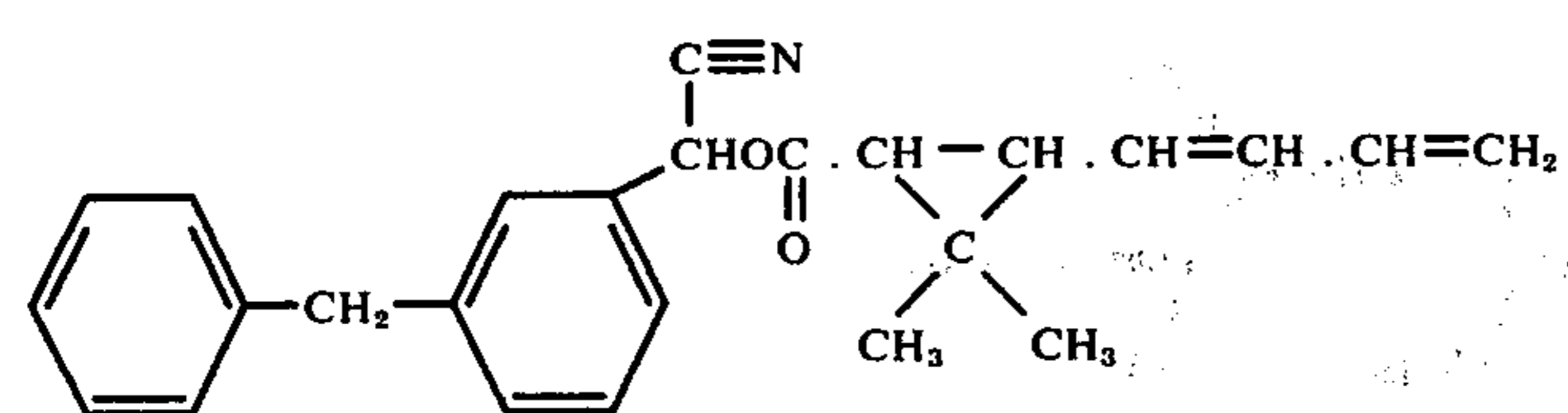
3-Benzyl-α-cyanobenzyl 2',2'-dimethyl-3'-(1'',3'''-butadienyl)-cyclopropanecarboxylate
