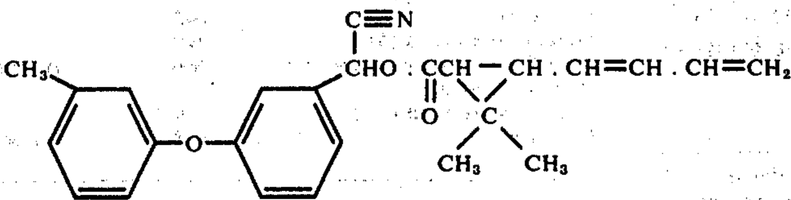
3-(m-Tolyloxy)-alpha-cyanobenzyl 2',2'- dimethyl-3'-(1'',3''-butadienyl)-cyclo- propanecarboxylate
