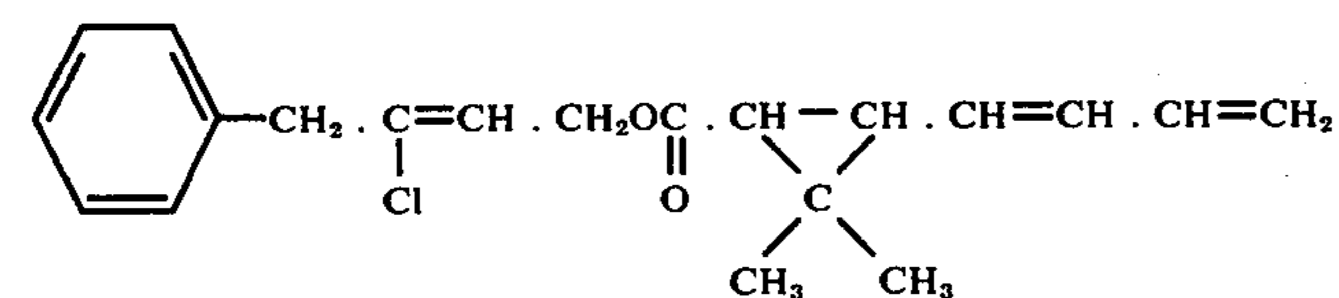
3-Chloro-4-phenyl-2-butene-1-yl 2',2'- dimethyl-3'-(1'',3''-butadienyl)-cyclo- propanecarboxylate
