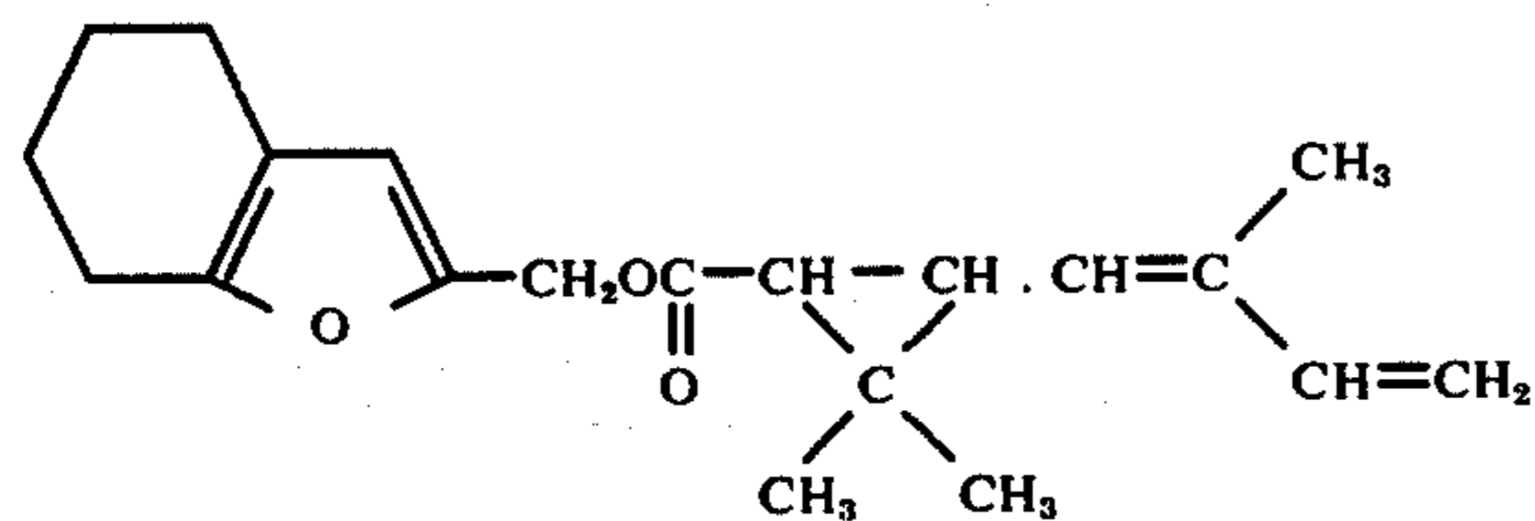
4,5-Tetramethylenefurfuryl 2',2'-dimethyl-3'-(2''-methyl-1'',3''-butadienyl)-cyclopropanecarboxylate
