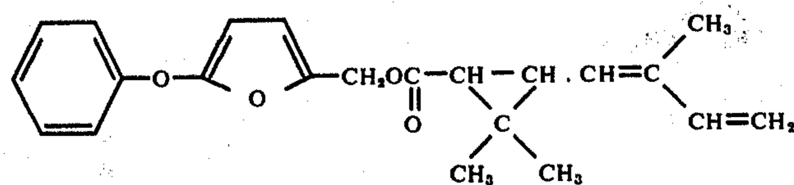
5-Oxa-4,5,6,7-tetrahydrobenzofurfuryl-2',2'-dimethyl-3'-(2''-methyl-1'',3''-butadienyl)-cyclopropanecarboxylate
