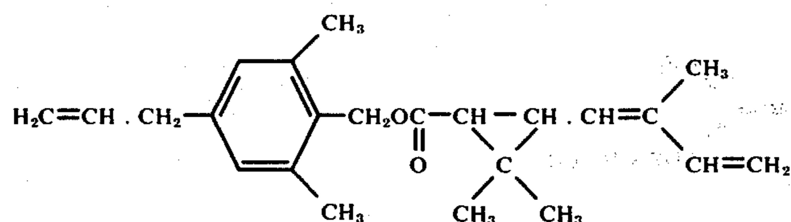
2,6-Dimethyl-4-allylbenzyl 2',2'-dimethyl-3'-(2''-methyl-1'',3''-butadienyl)-cyclopropanecarboxylate
