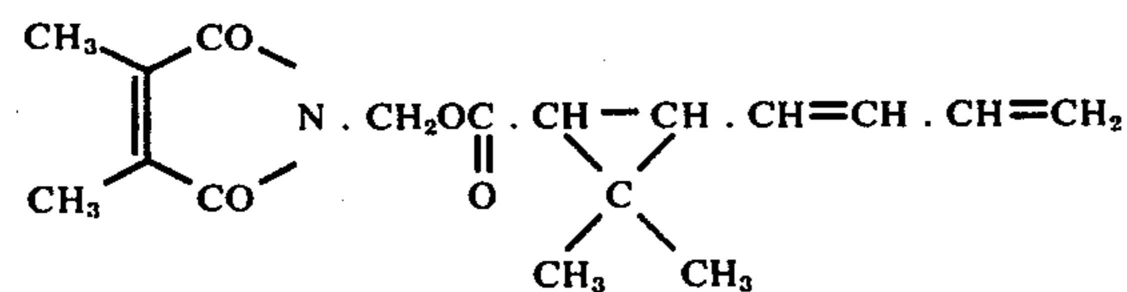
Dimethylmaleimidomethyl 2,2-dimethyl- 3-(1'',3''-butadienyl)-cyclopropane- carboxylate
