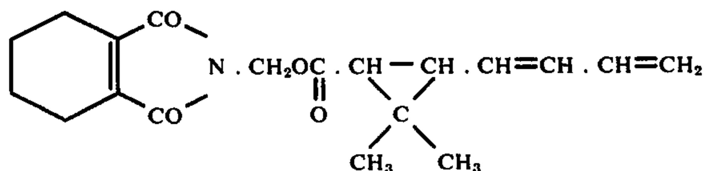
3,4,5,6-Tetrahydrophthalimidomethyl 2',2'-dimethyl-3'-(1'',3''-butadienyl)- cyclopropanecarboxylate
