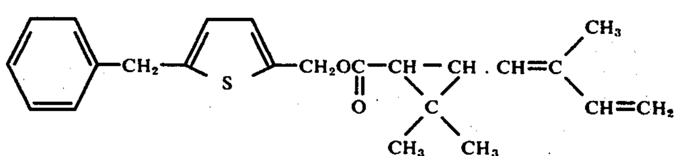
5-Benzyl-2-thienyl 2',2'-dimethyl-3'-(2''-methyl-1'',3''-butadienyl)-cyclopropanecarboxylate
