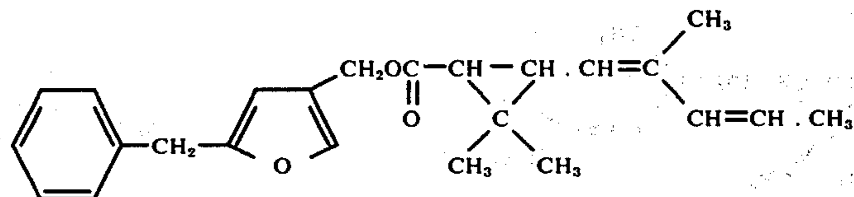
5-Benzyl-3-furylmethyl 2',2'-dimethyl-3'-(2''-methyl-1'',3''-pentadienyl)-cyclopropanecarboxylate
