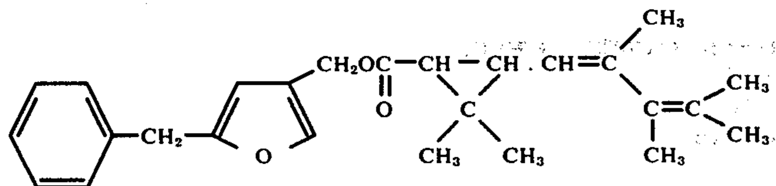
5-Benzyl-3-furymethyl 2',2'-dimethyl-3'-(2'',3'',4'''-trimethyl-1'',3'''-pentadienyl)-cyclopropanecarboxylate
