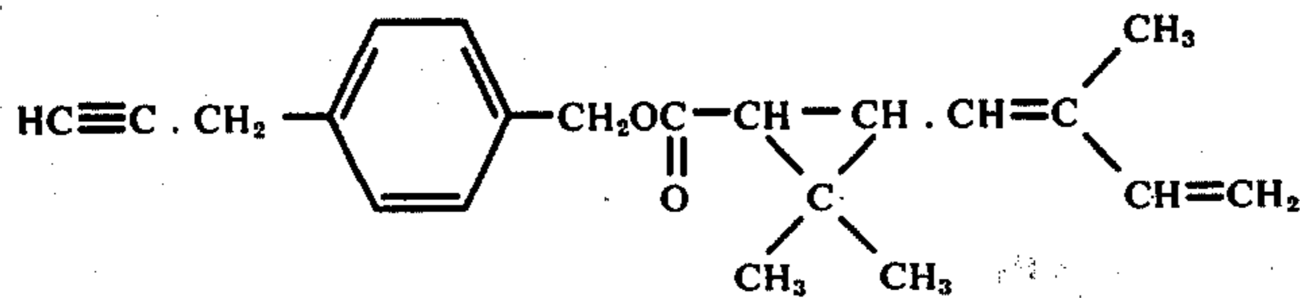
4-Propargylbenzyl 2',2'-dimethyl-3'-(2''-methyl-1'',3''-butadienyl)-cyclopropanecarboxylate
