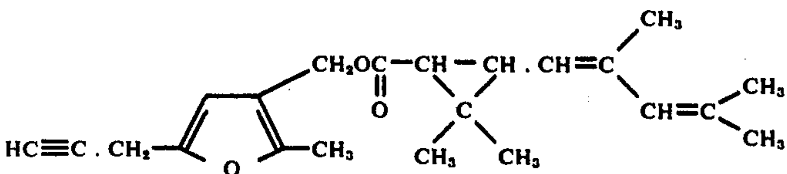
2-Methyl-5-propargyl-3-furymethyl 2',2'- dimethyl-3'-(2'',4''-dimethyl-1'',3''- pentadienyl)-cyclopropanecarboxylate
