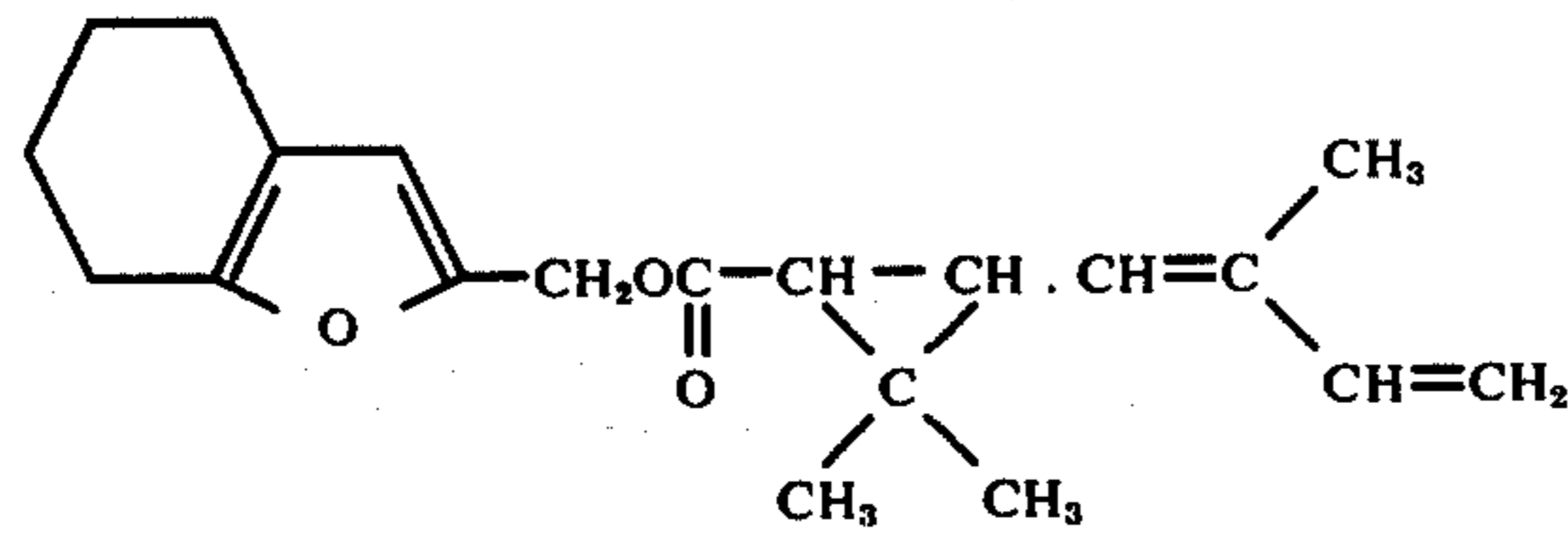
4,5-Tetramethylenefurfuryl 2',2'-dimethyl-3'-(2''-methyl-1'',3''-butadienyl)-cyclopropanecarboxylate
