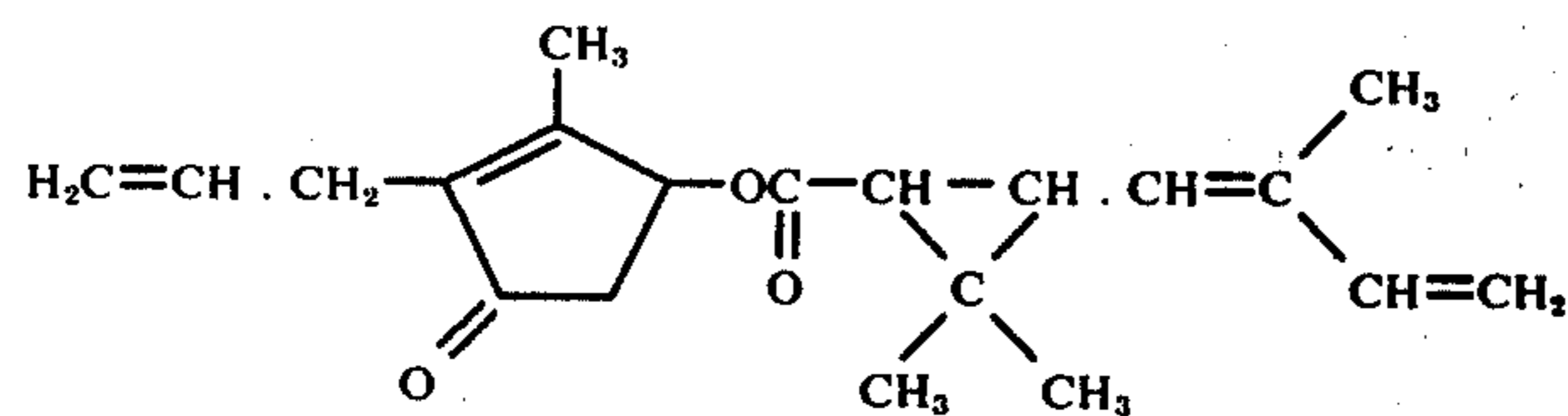
2-Allyl-3-methyl-2-cyclopentene-1-one-4-yl 2',2'-dimethyl-3'-(2''-methyl-1'',3''-butadienyl)-cyclopropanecarboxylate
