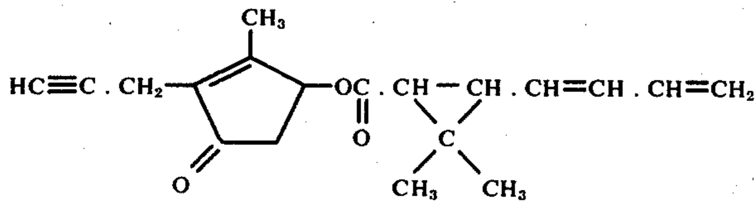
2-Propargyl-3-methyl-2-cyclopentene-1- one-4-yl 2',2'-dimethyl-3'-(1'',3''- butadienyl)-cyclopropanecarboxylate
