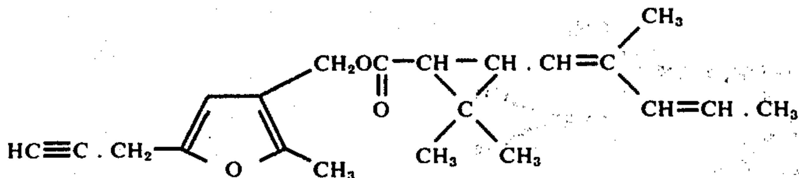
2-Methyl-5-propargyl-3-furylmethyl 2',2'-dimethyl-3'-(2''-methyl-1'',3''-pentadienyl)-cyclopropanecarboxylate
