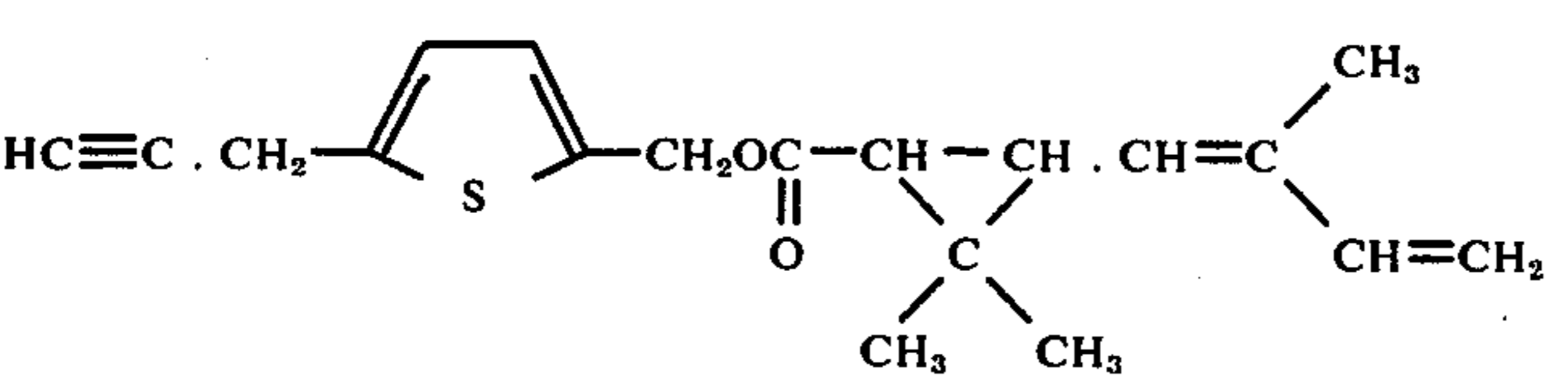
5-Propargyl-2-thienyl 2',2'-dimethyl-3'-(2''-methyl-1'',3''-butadienyl)-cyclopropanecarboxylate
