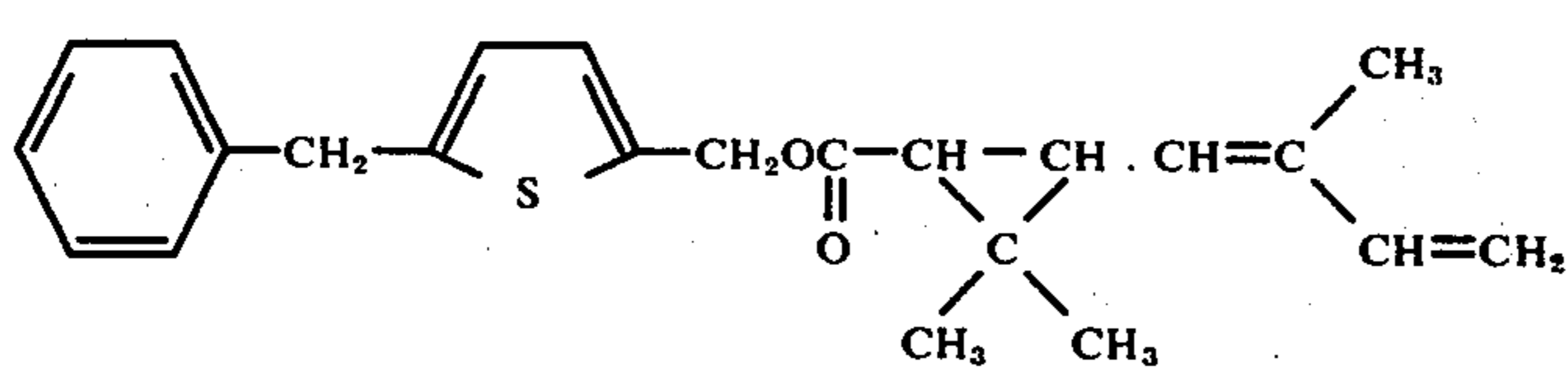
5-Benzyl-2-thenyl 2',2'-dimethyl-3'-(2''-methyl-1'',3''-butadienyl)-cyclopropanecarboxylate
