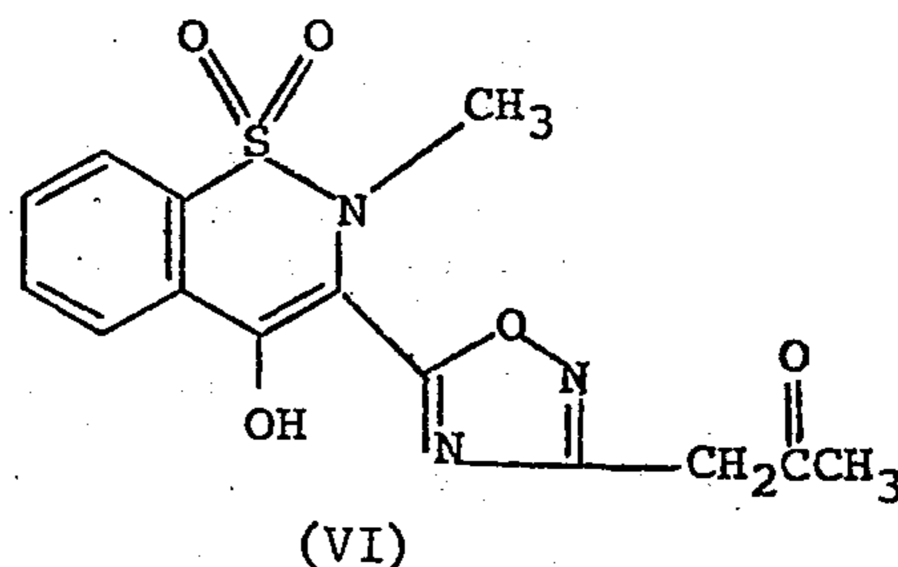
1-[[5-(4-Hydroxy-2-methyl-2H-1,2-benzothiazin-3-yl)-1,2,4-oxadiazol-3-yl]methyl]ethanone S,S-dioxide
