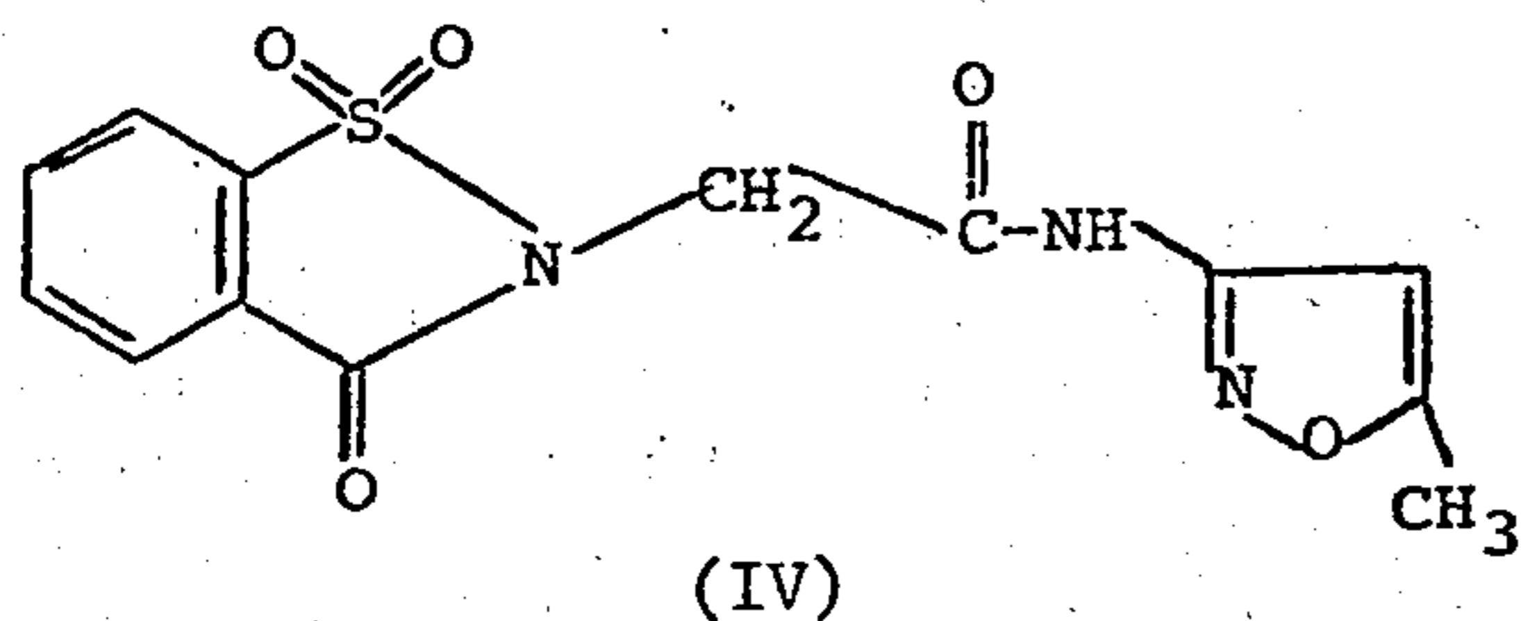
2,3-Dihydro-N-(5-methyl-3-isoxazolyl)-3-oxo-1,2-benzisothiazole-2-acetamide 1,1-dioxide
