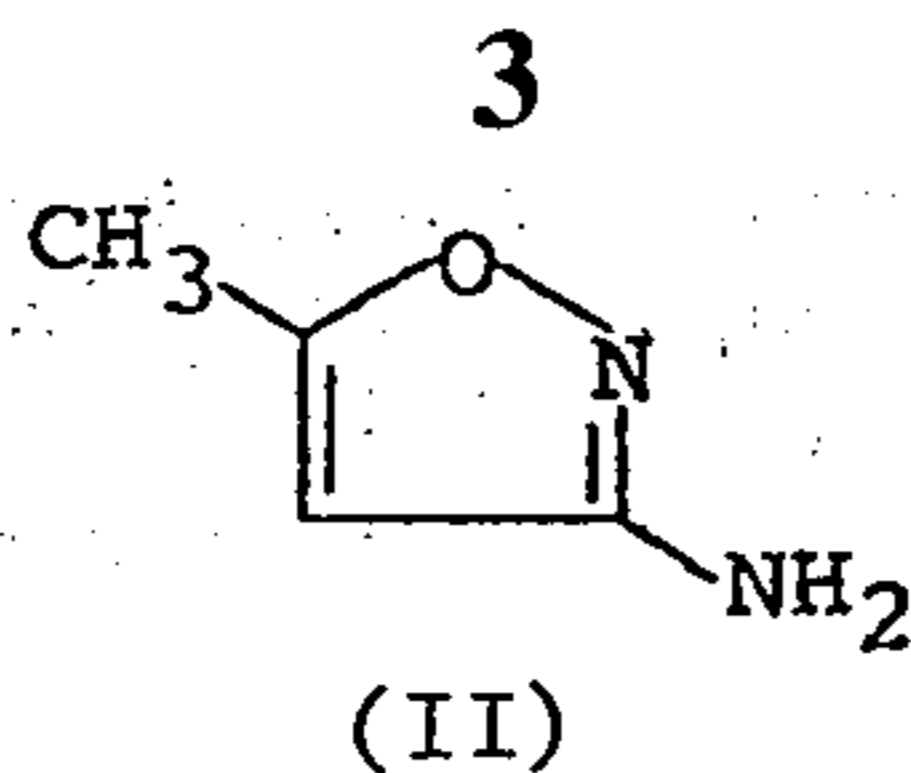
3-Amino-5-methylisoxazole
