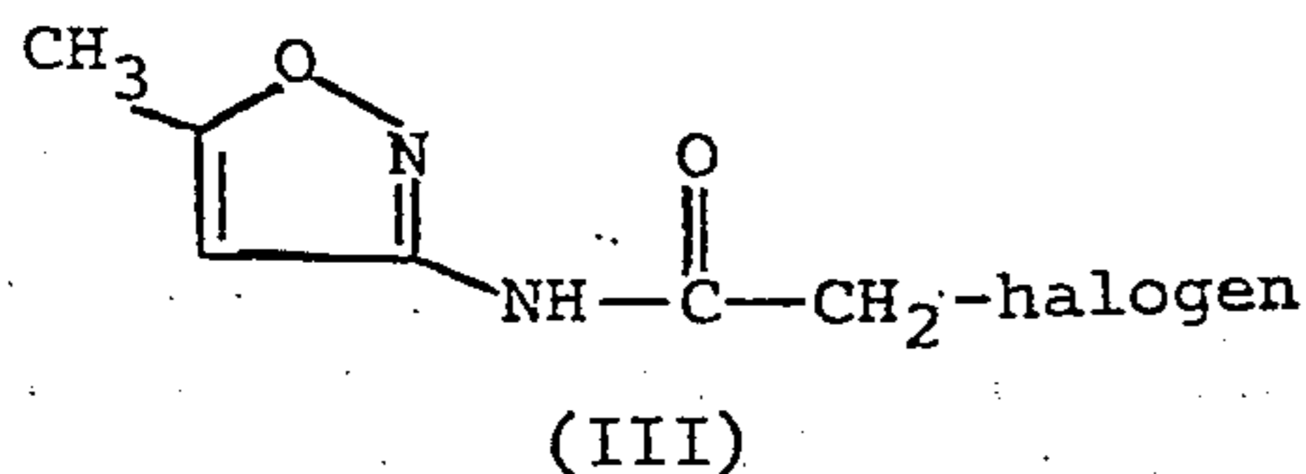
3-(Haloacetamido)-5-methylisoxazole
