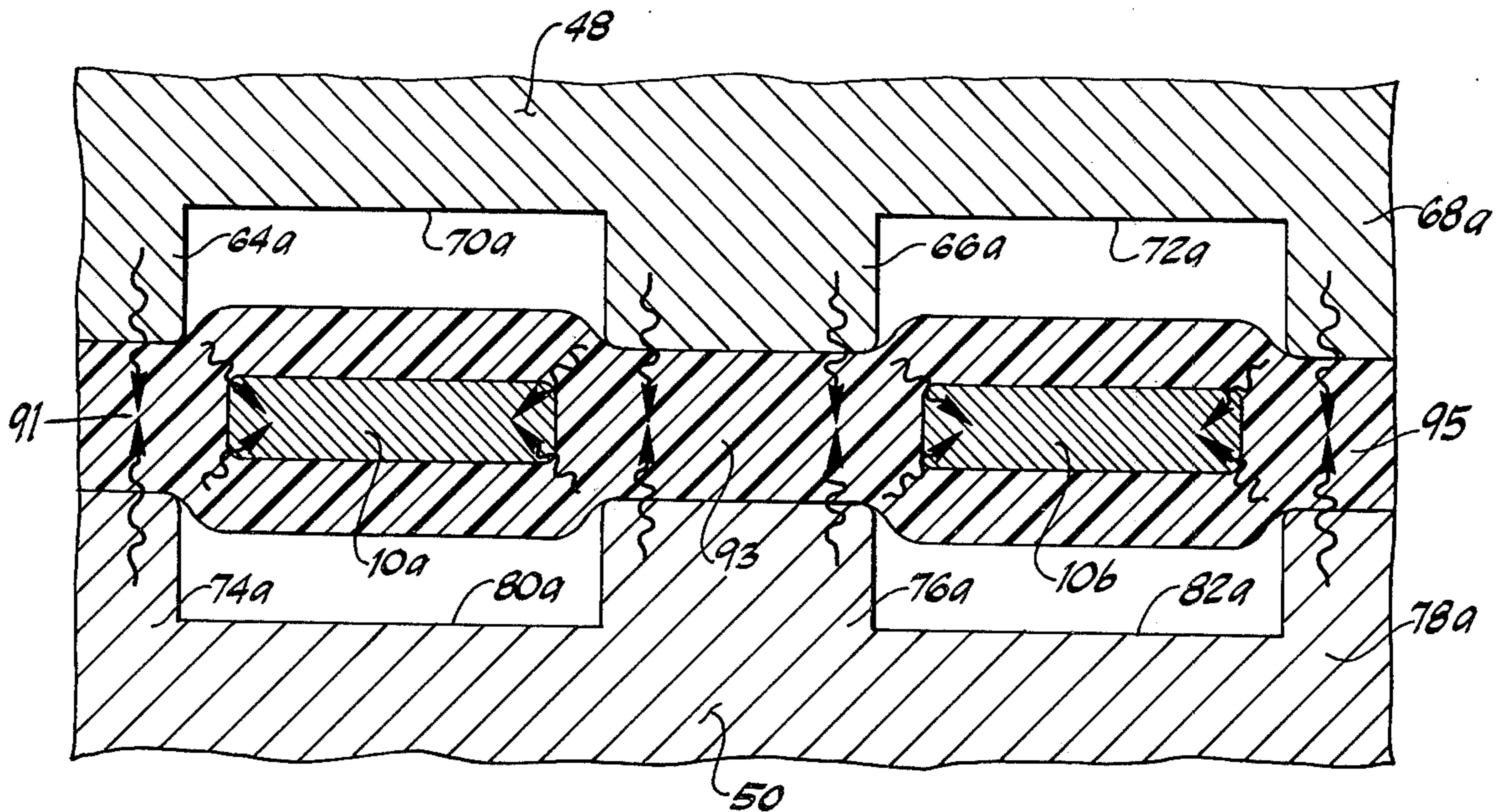
Fig. 5 (BONDING)
