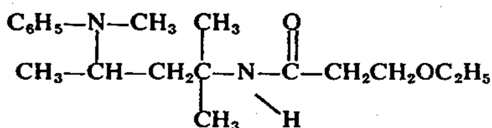
N-(1,1-dimethyl-3-piperidinopropyl)-3-phenoxy-2-methylpropionamide
