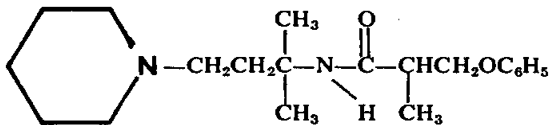
Trimethyl-3-[1-(3-methoxypropionamido)-1-methyl-1,3-diphenylpropyl]ammonium iodide
