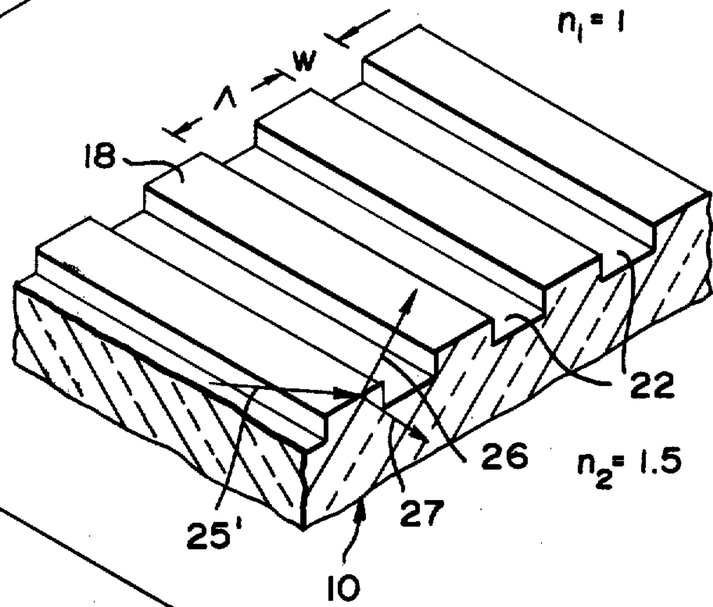
FIG. 2 PRIOR ART
