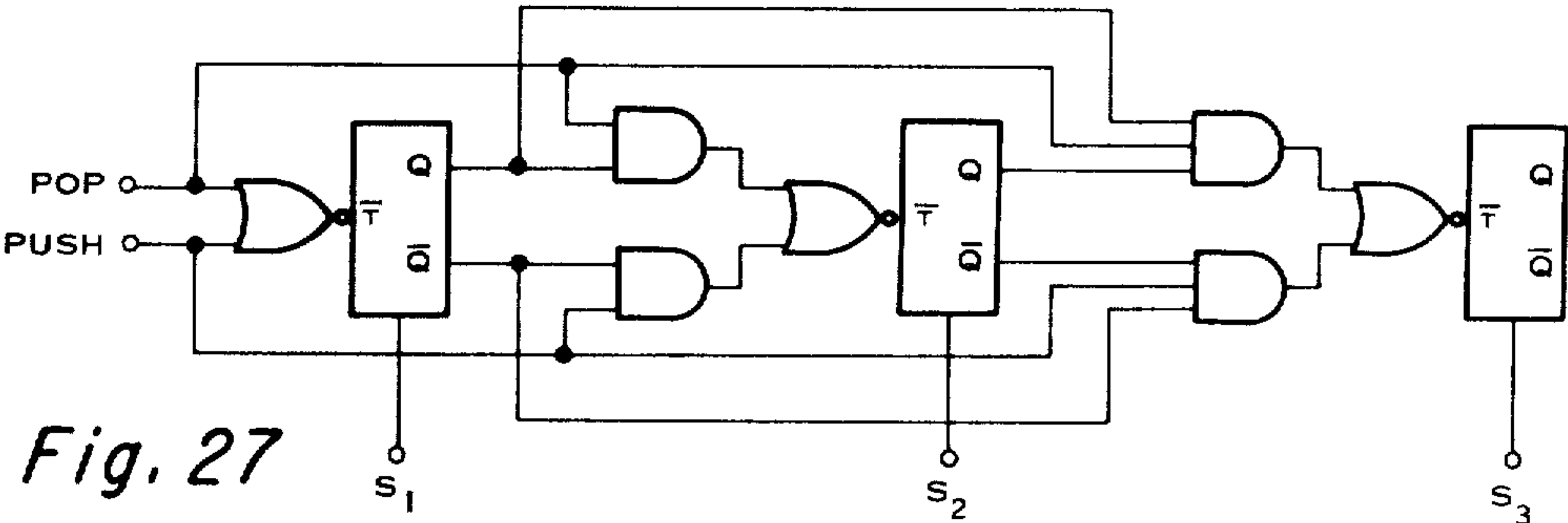
STACK POINTER
