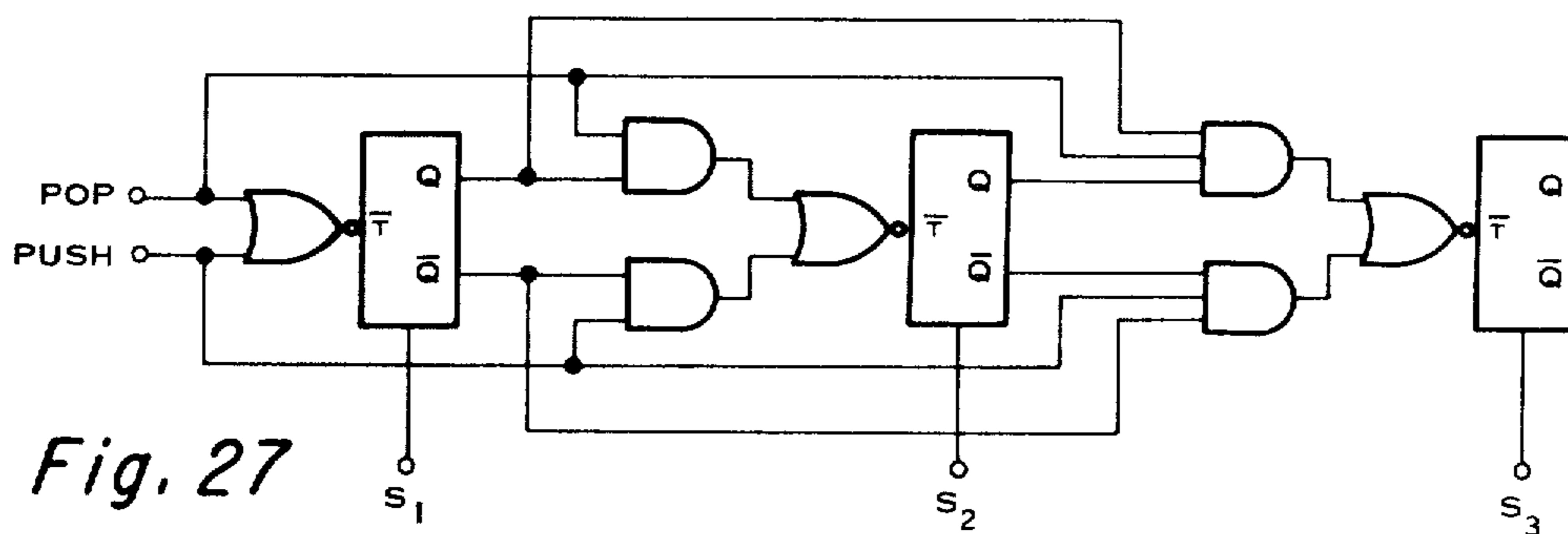
STACK POINTER
