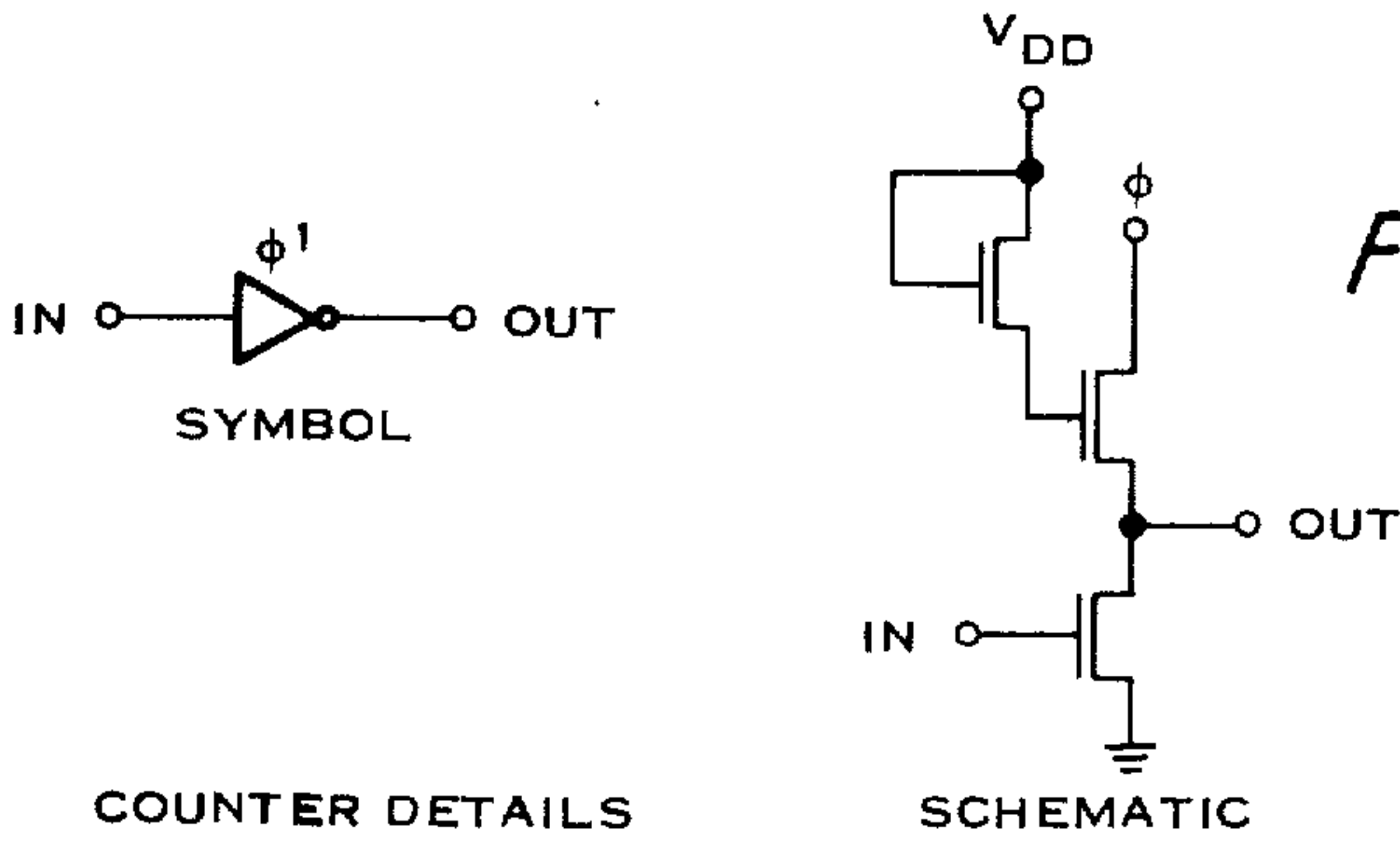
CLOCKED INVERTER DETAIL
