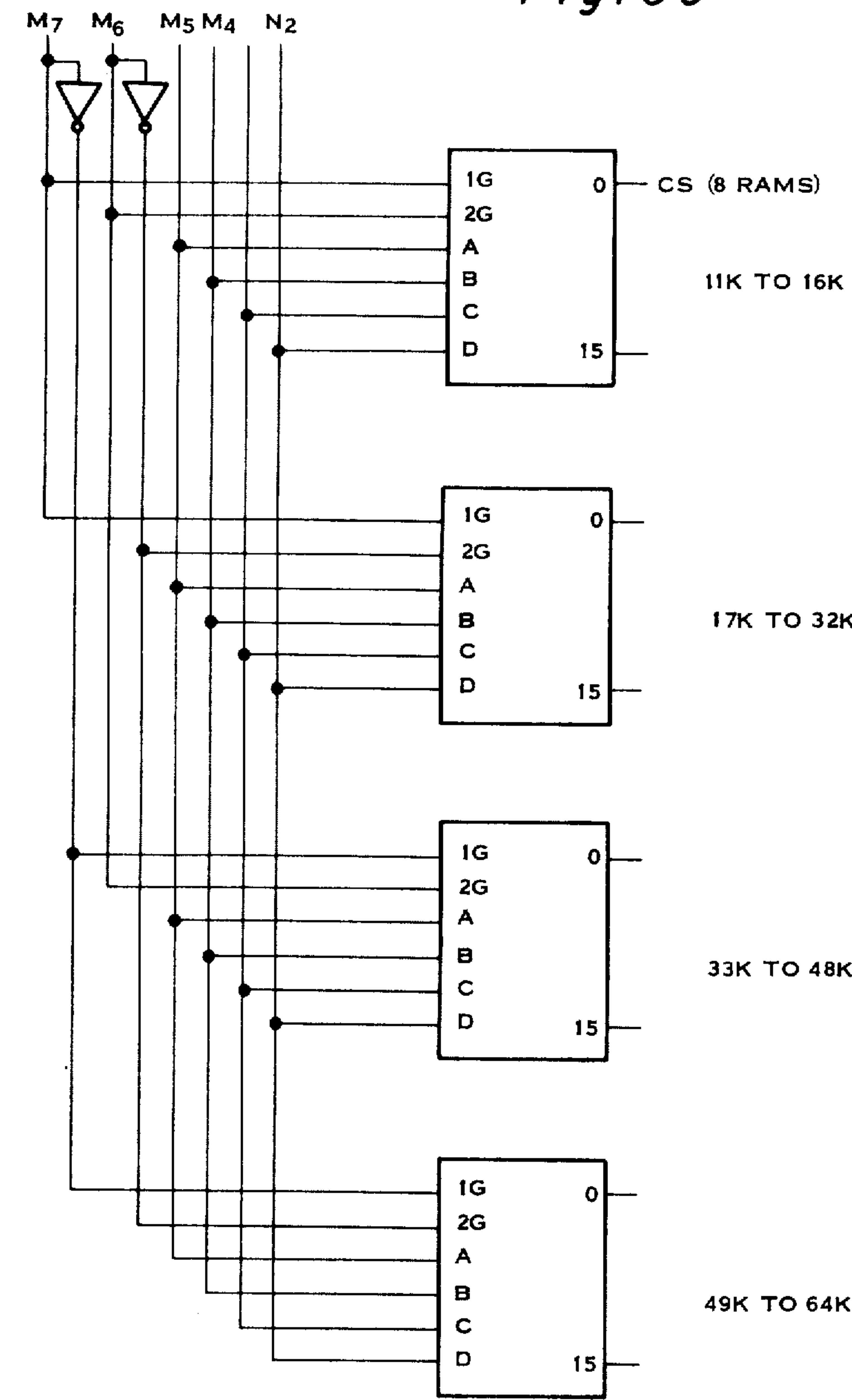
INTERFACE LOGIC
