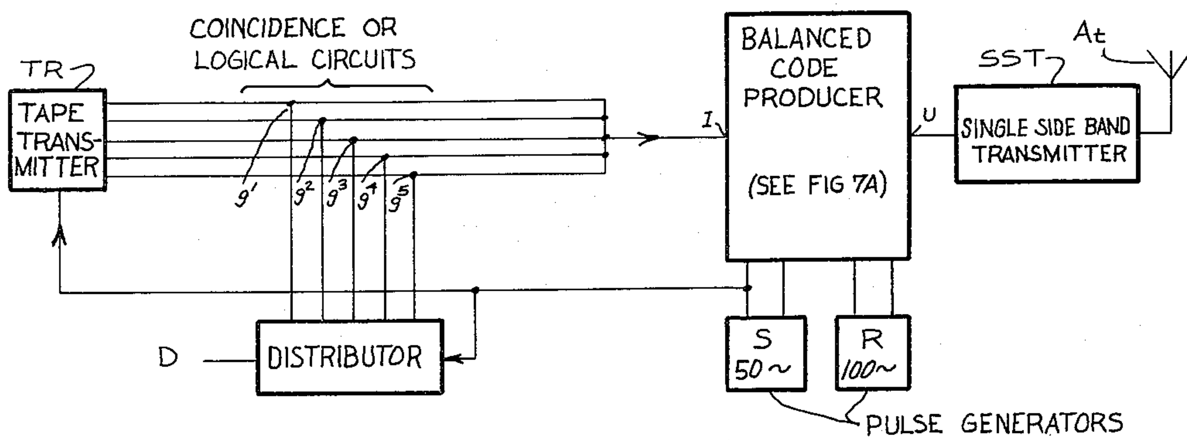
TRANSMITTER Fig. 7
