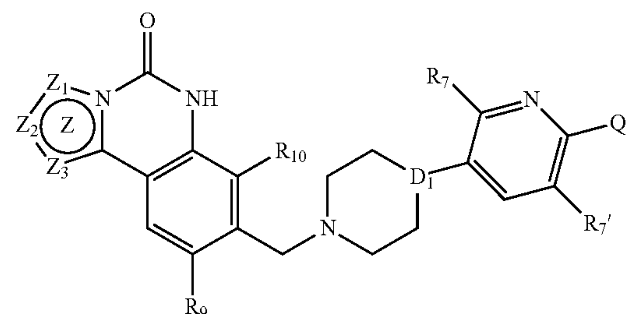
(VIc)
