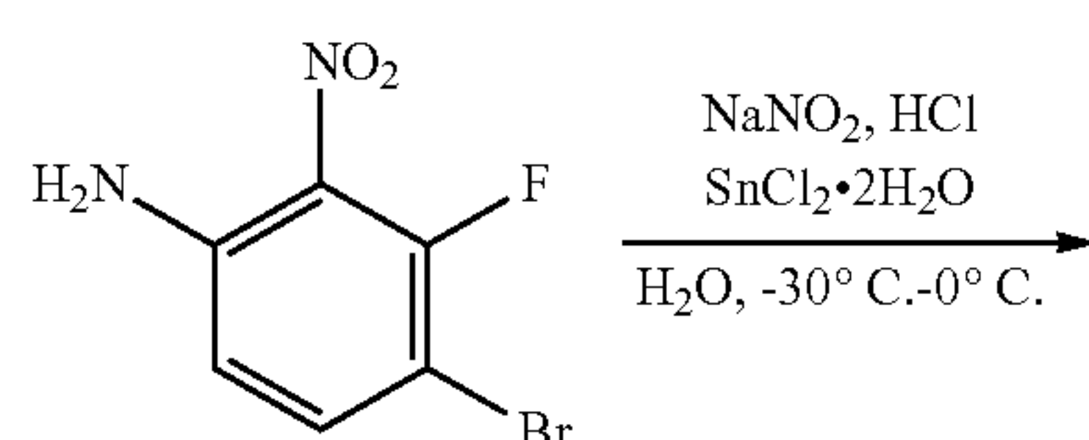
Scheme 9
