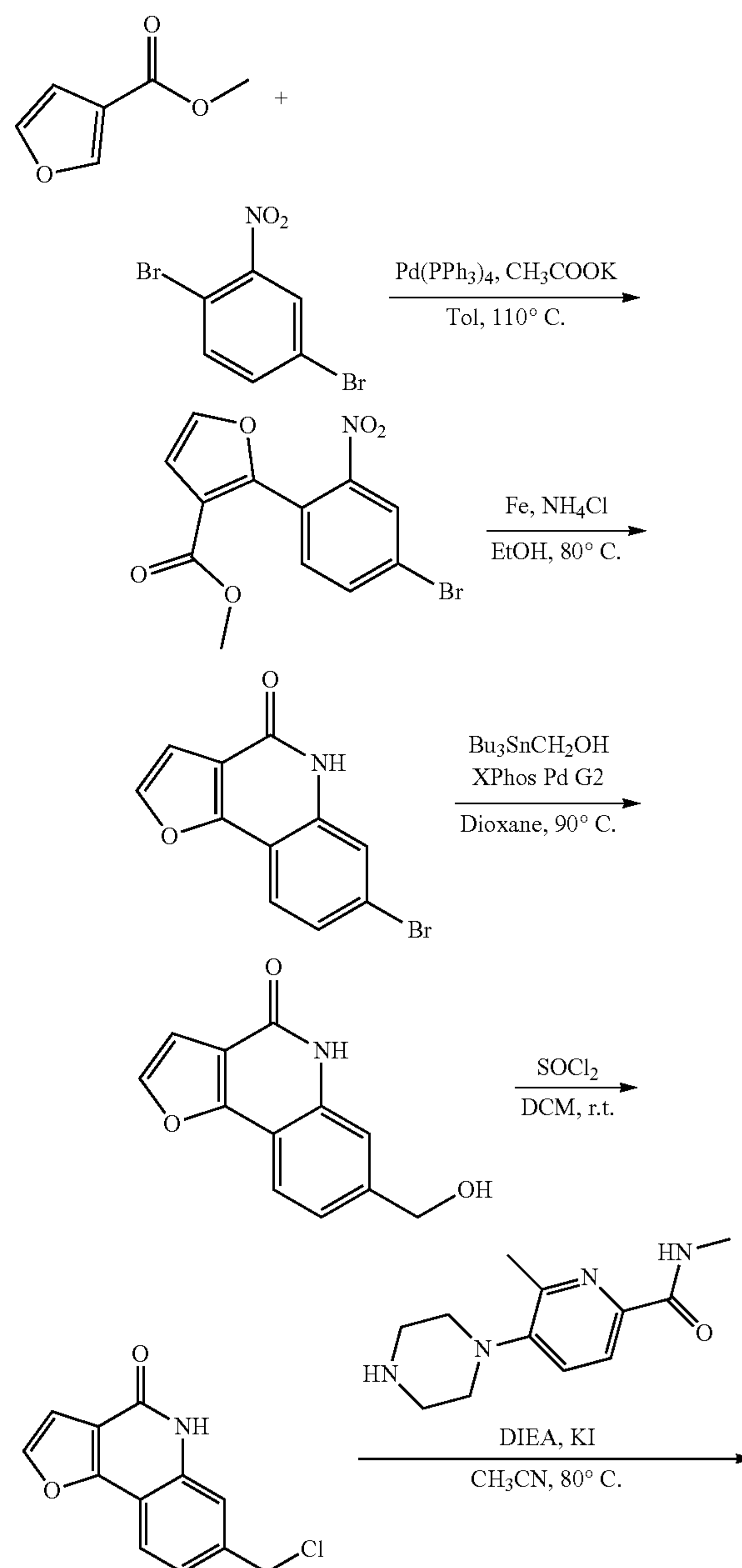
Scheme 2
