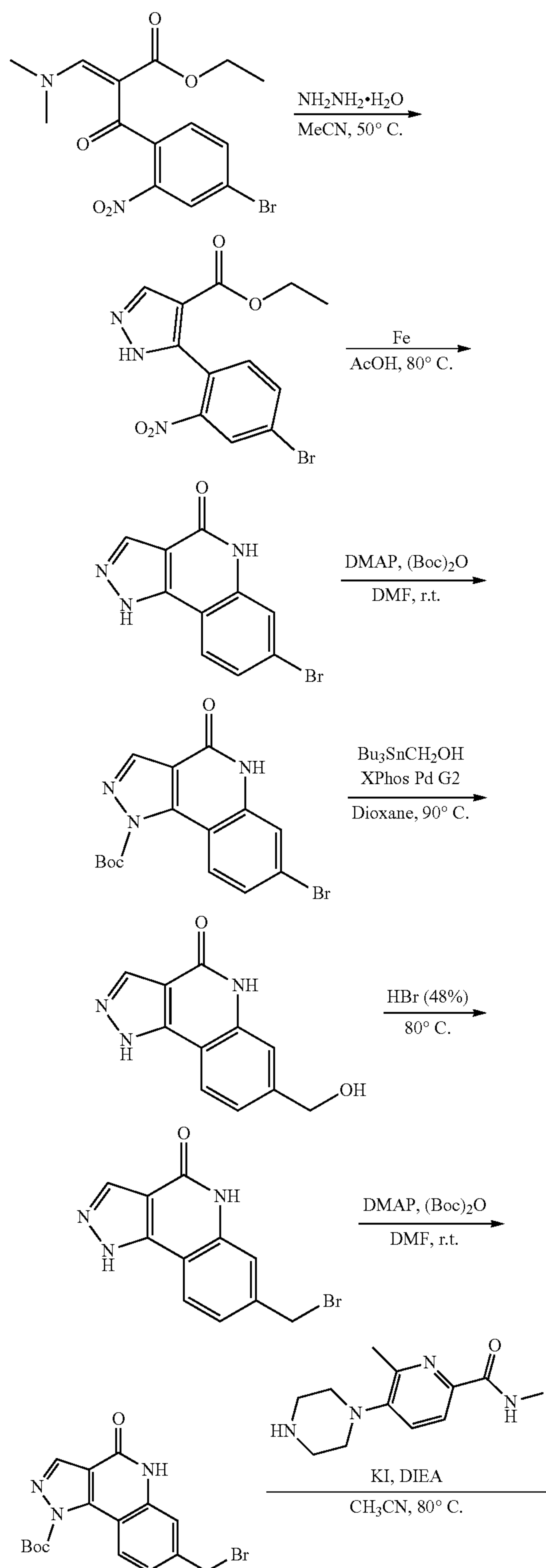
Scheme 3
