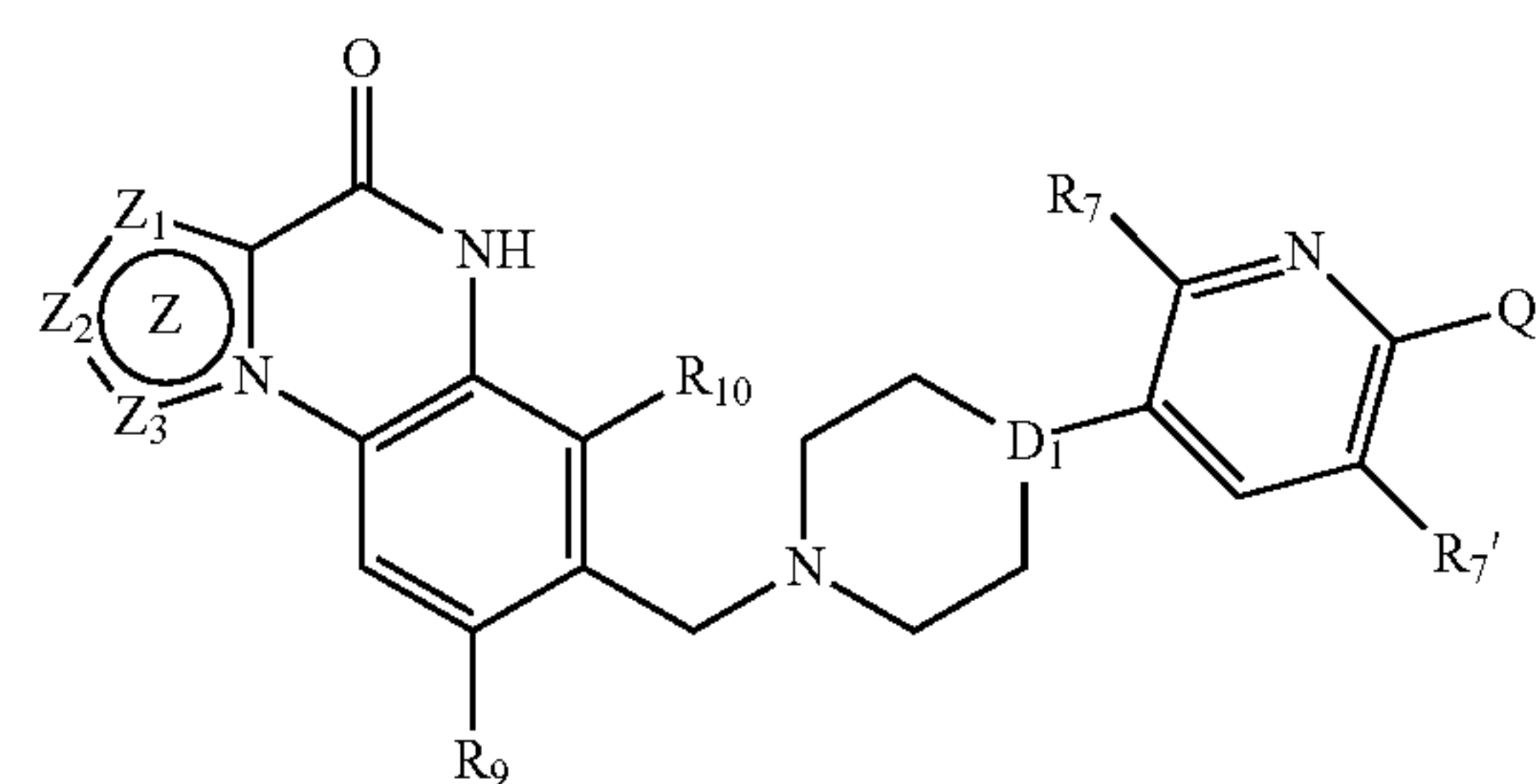
(VIc)
