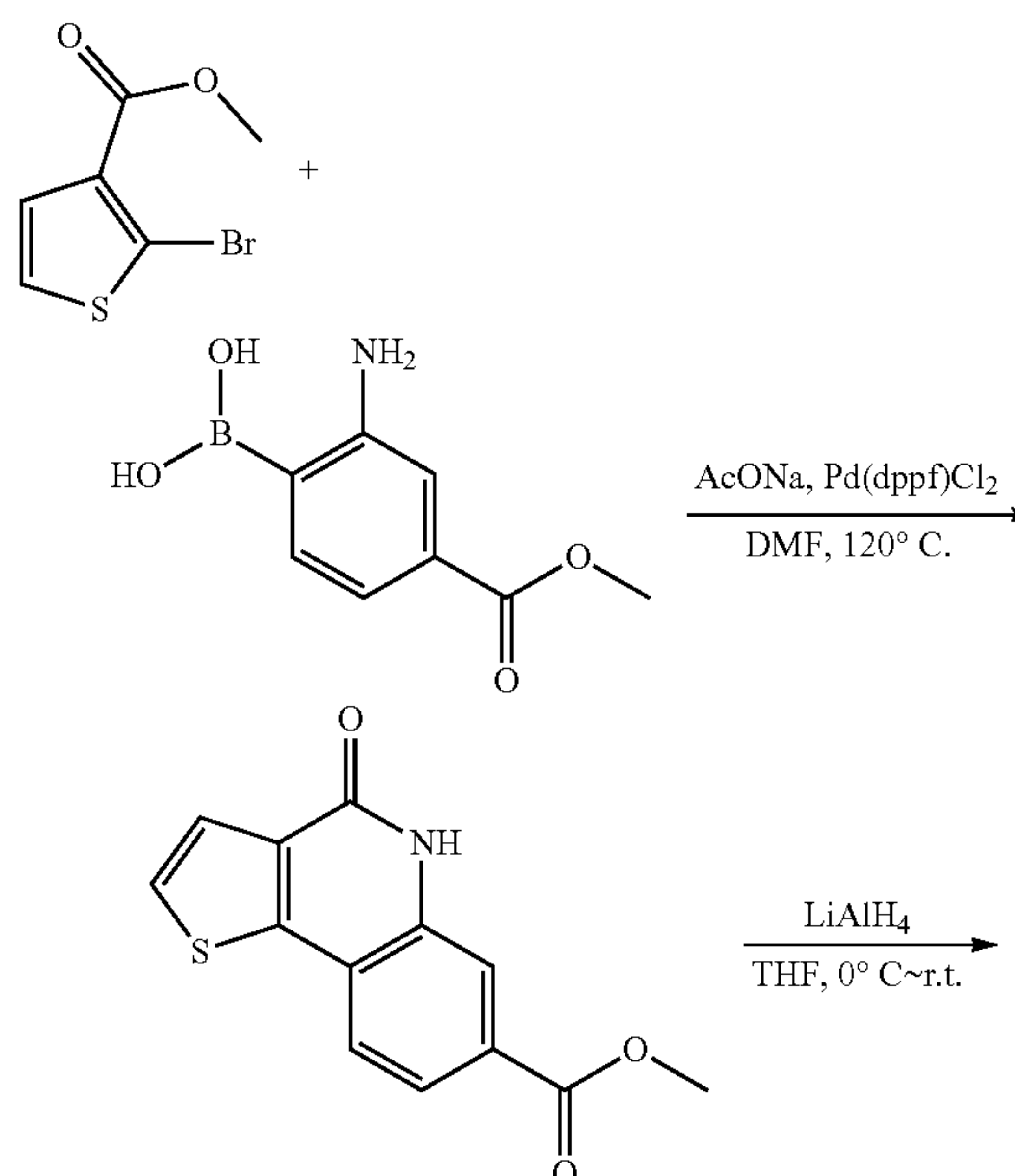
Scheme 1
