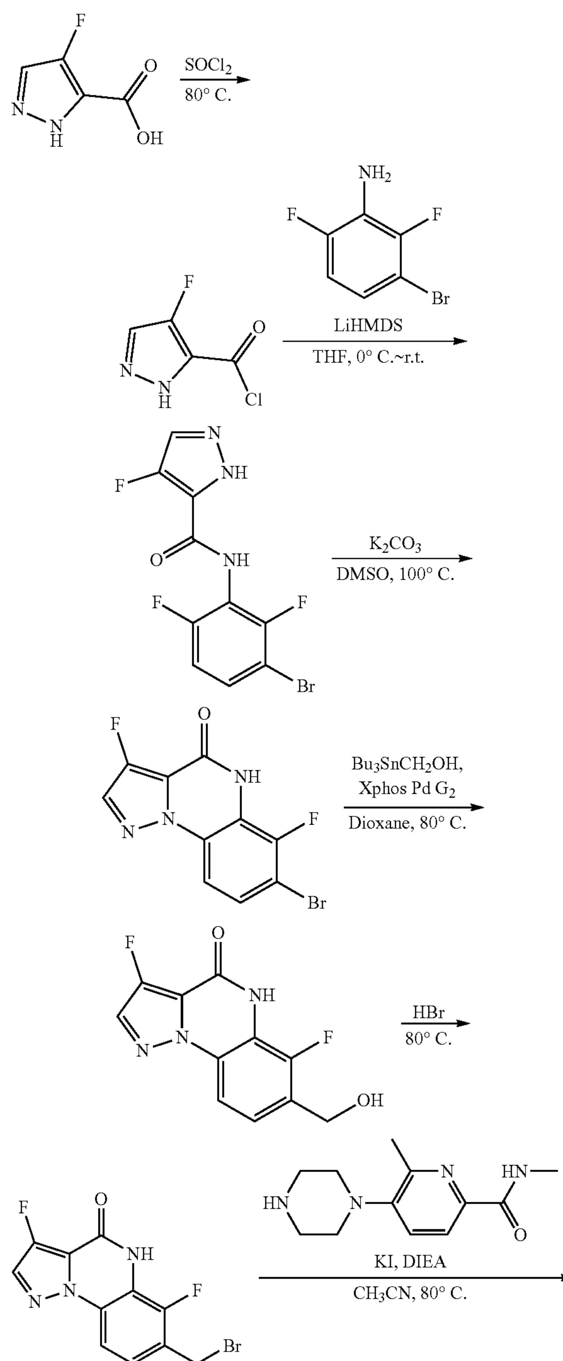
Scheme 8
