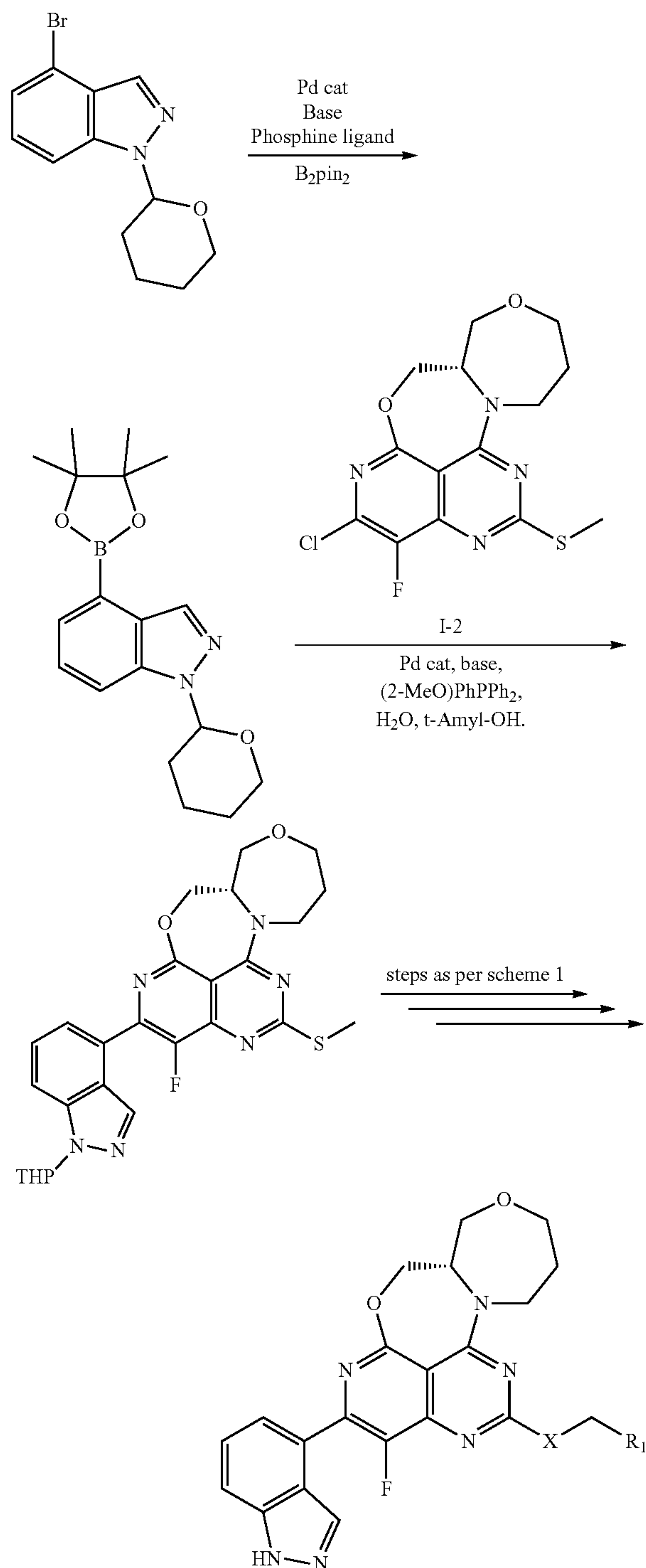
Scheme 3: General Method C
