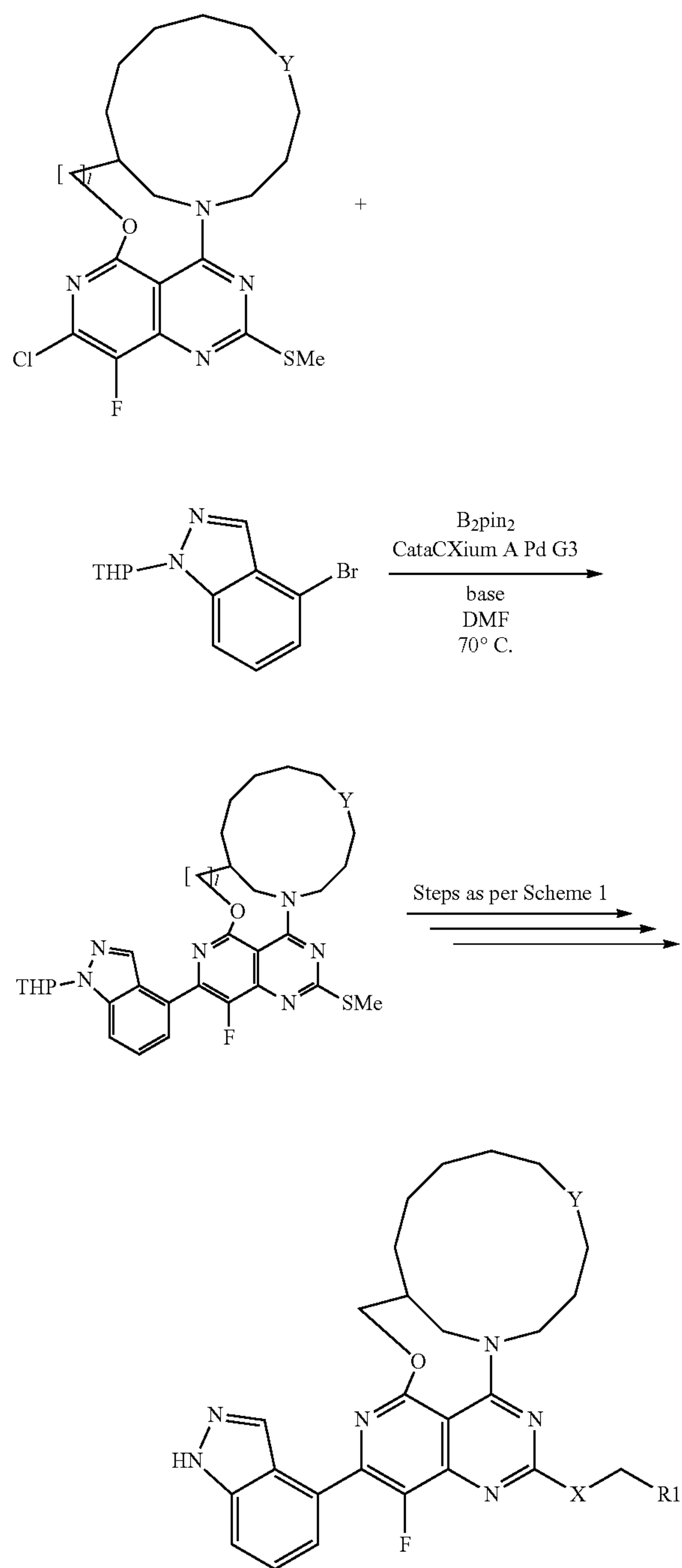
Scheme 2: General Method B
