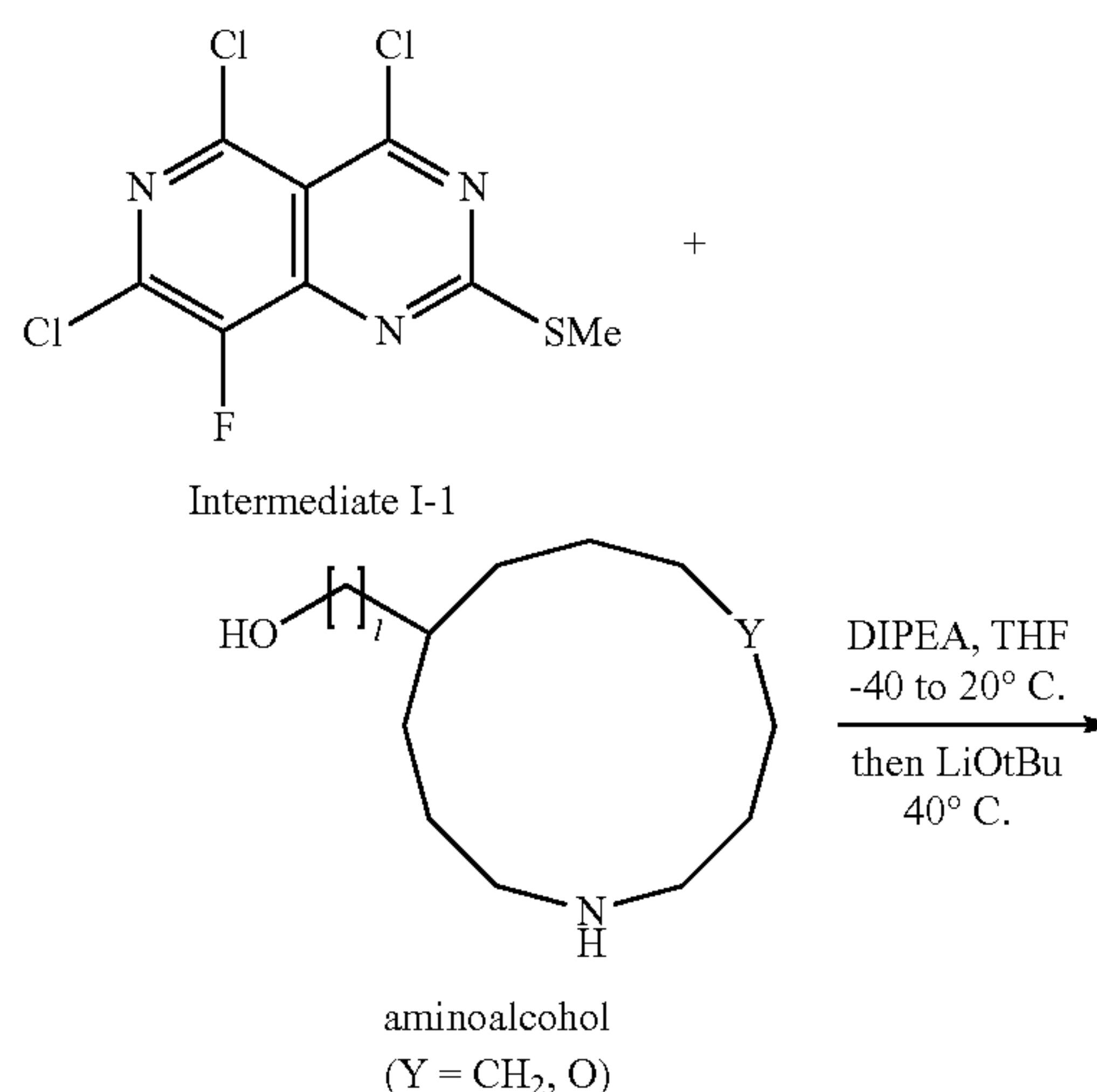
Scheme 1: General Method A
