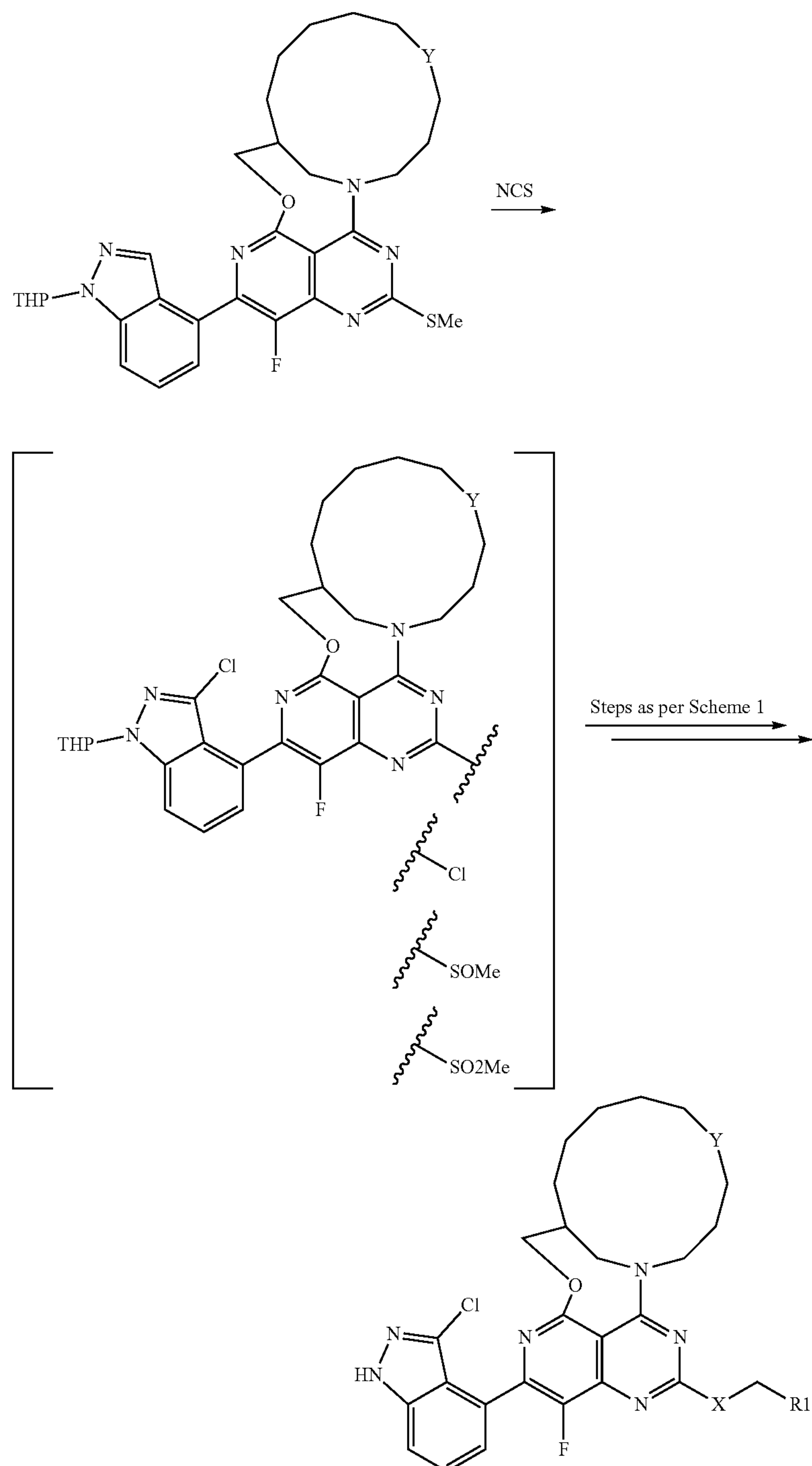
Scheme 4: General Method D
