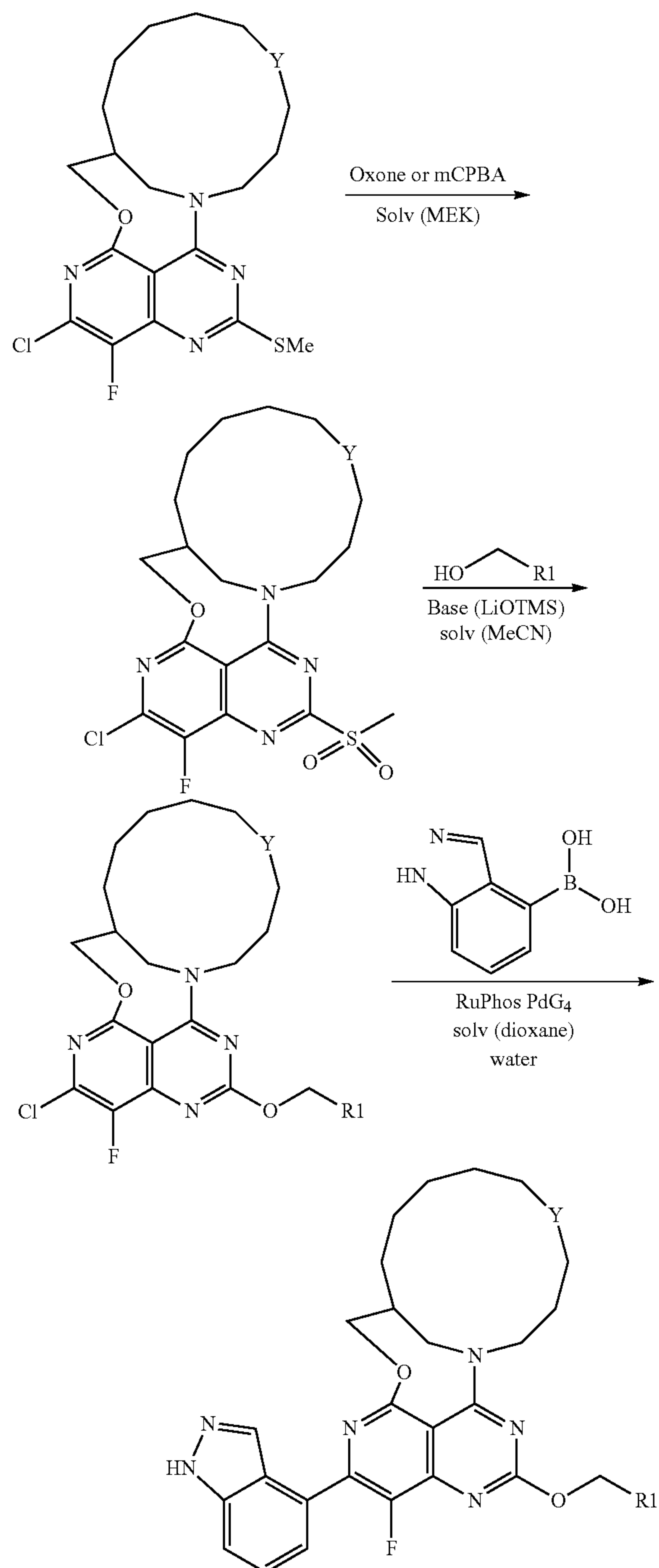
Scheme 5: General Method E
