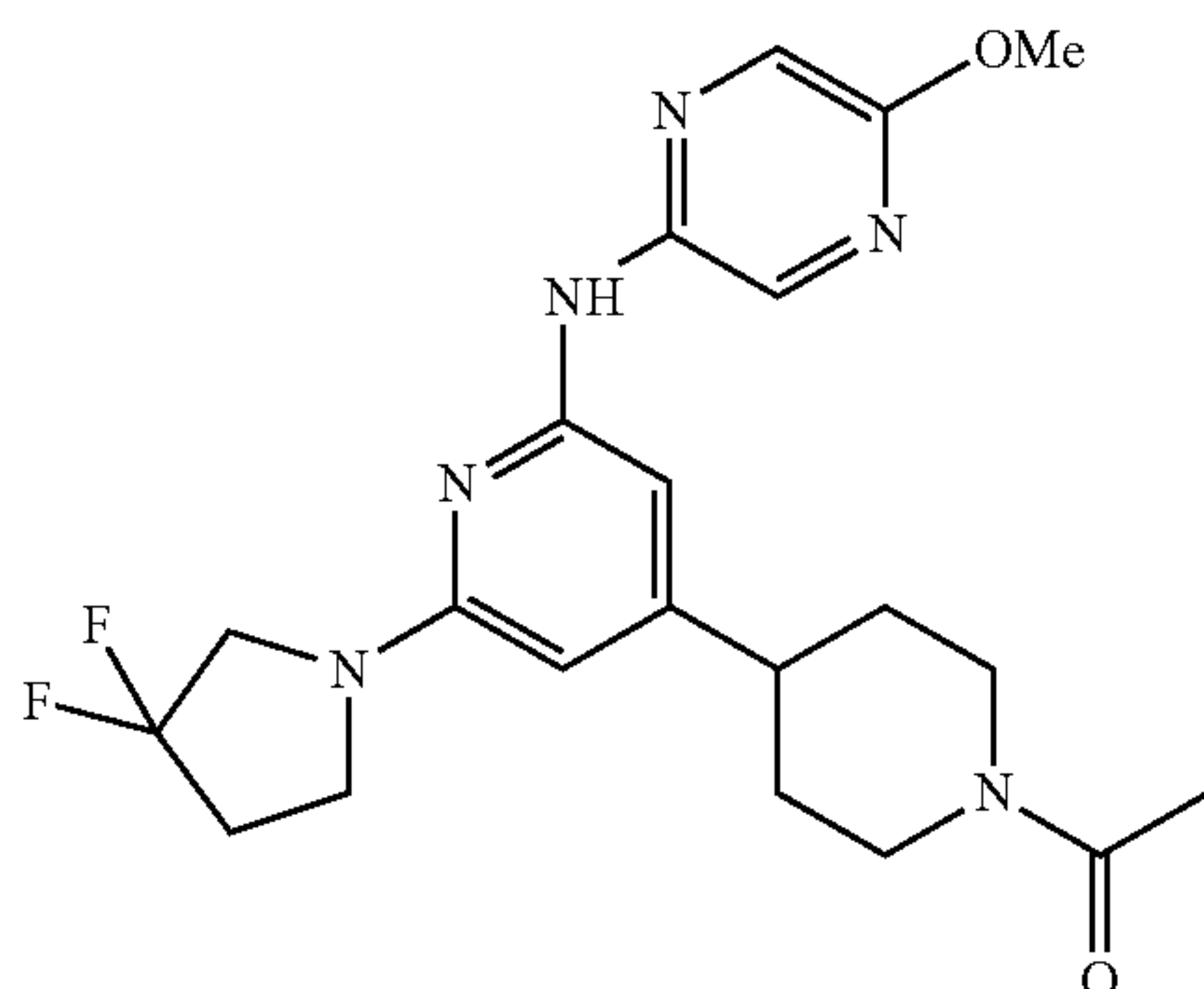
Compound 115
