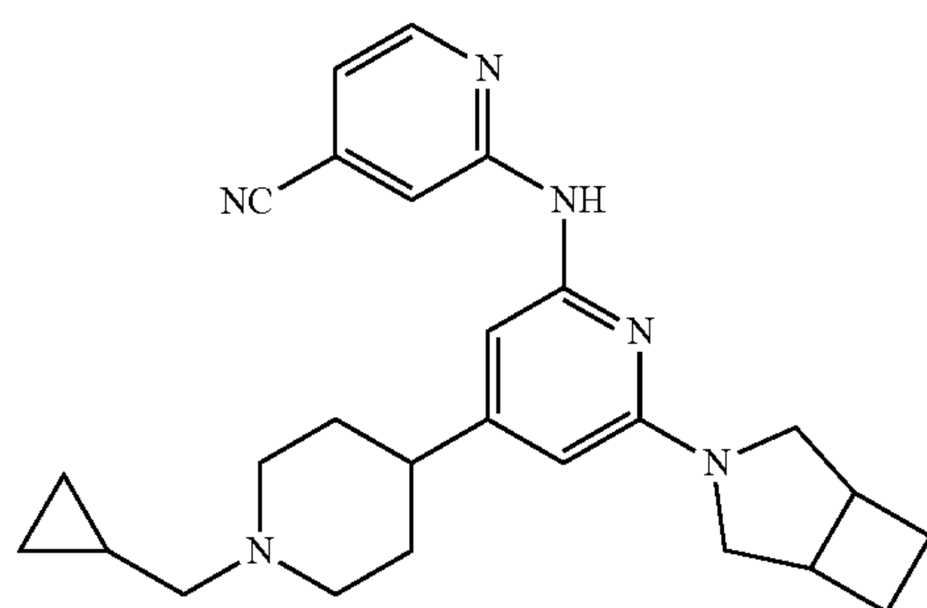
Compound 231
