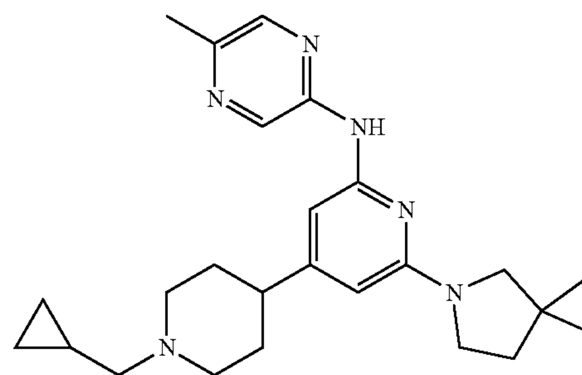
Compound 221
