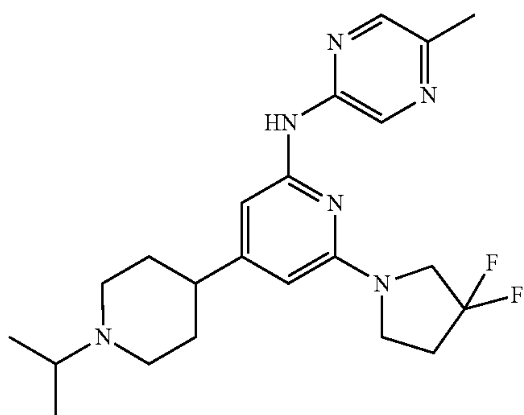
Compound 160
