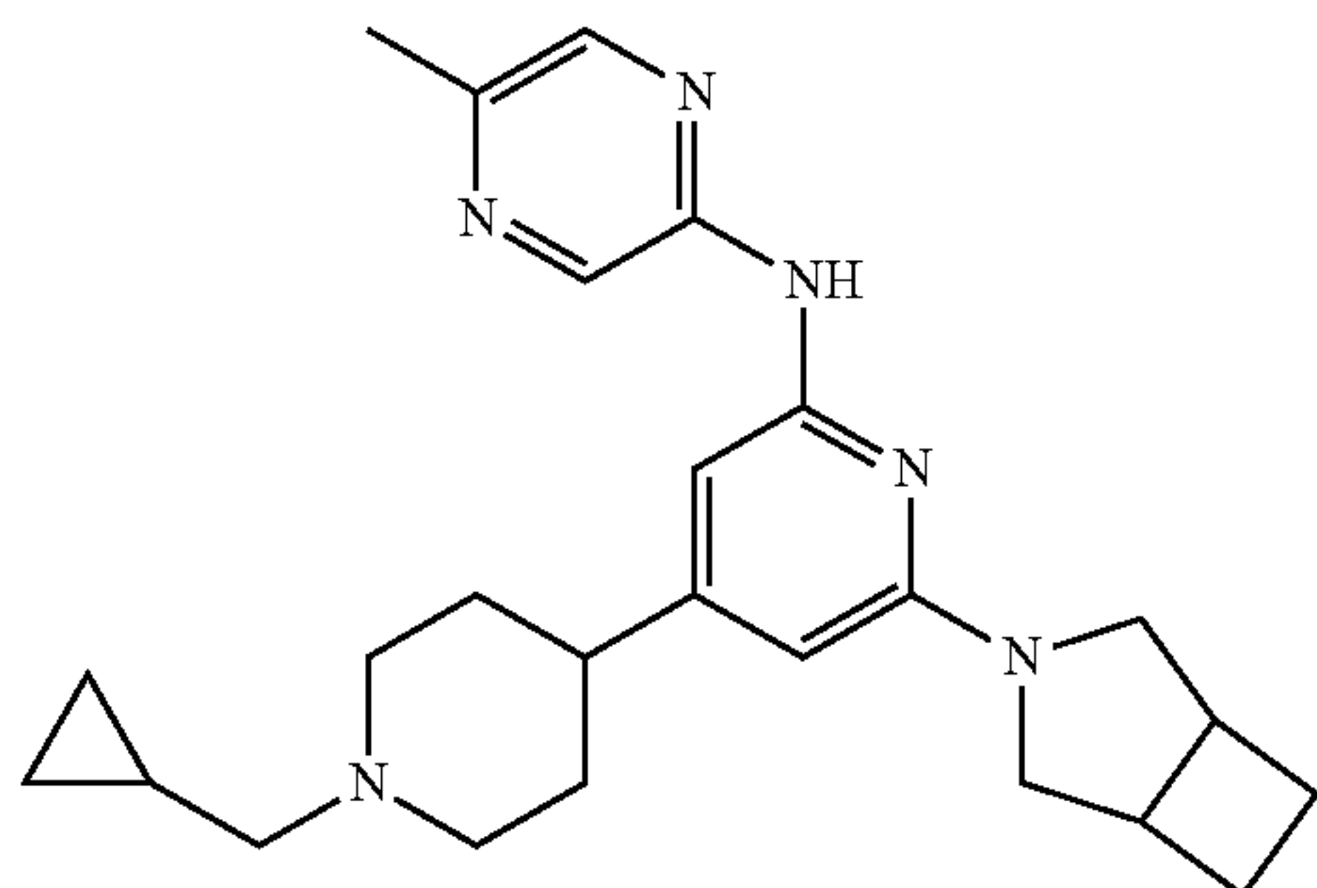
Compound 222
