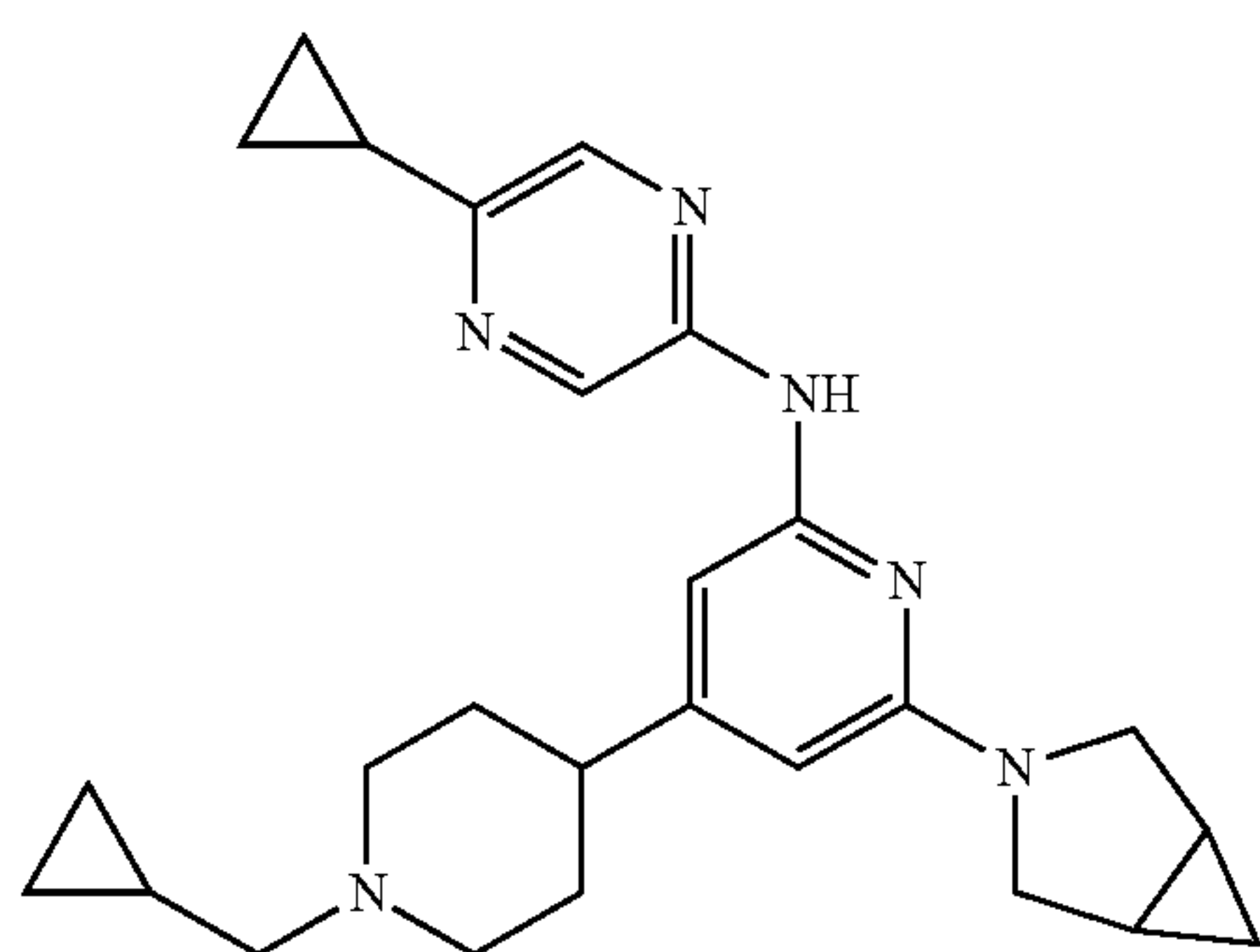
Compound 216
