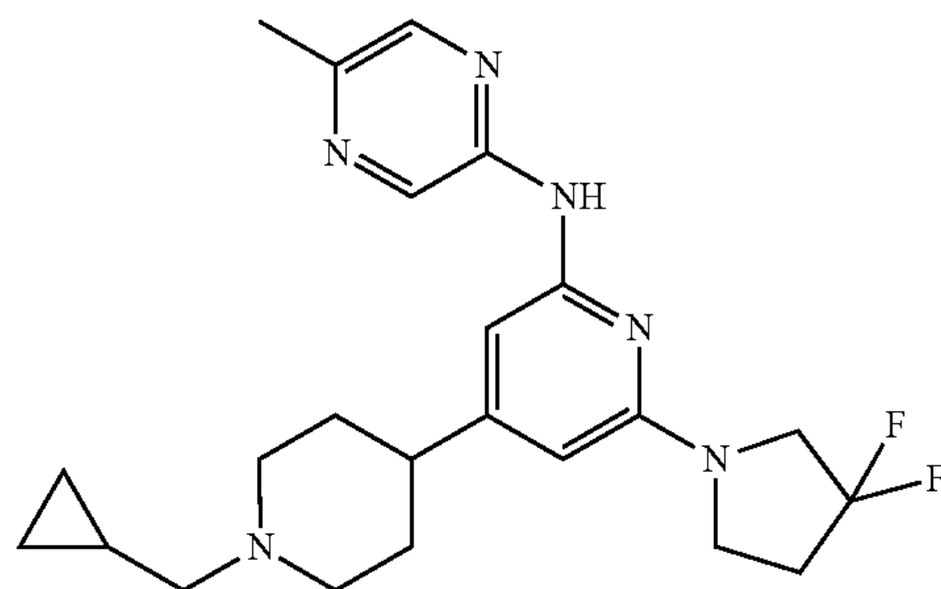
Compound 161
