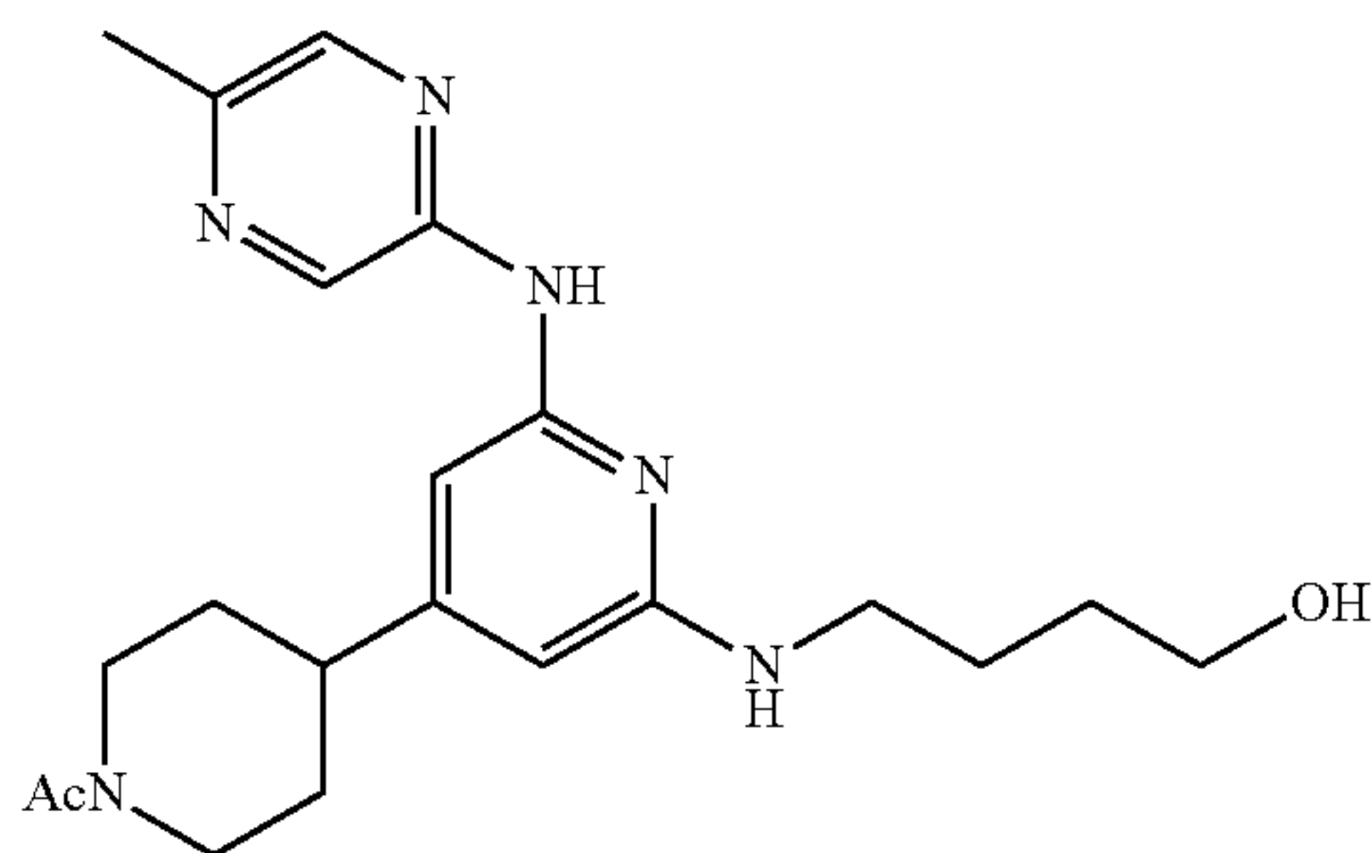
Compound 184
