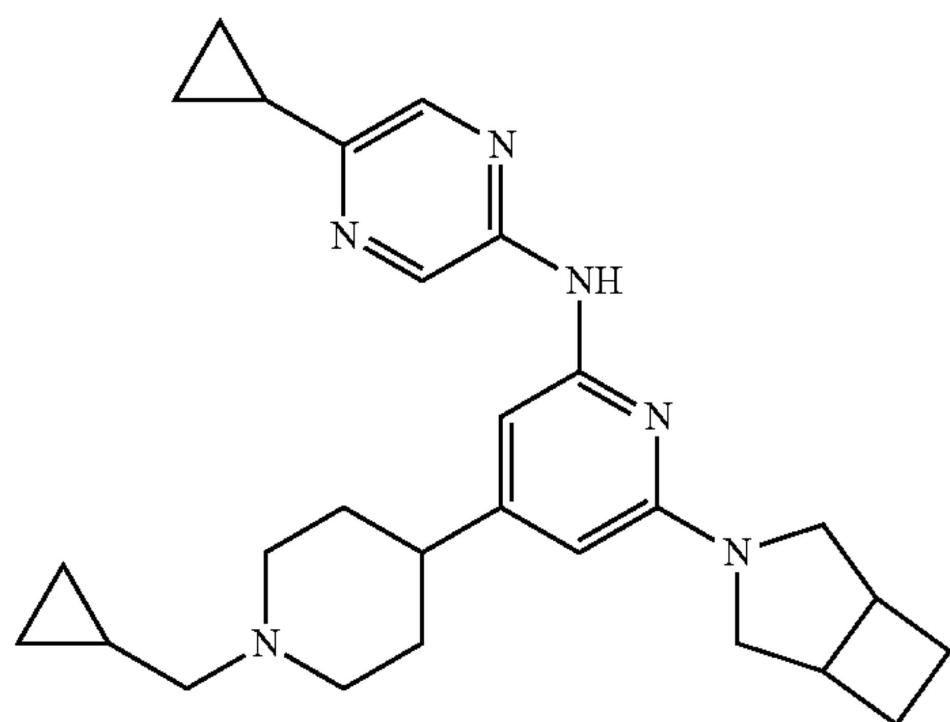
Compound 225
