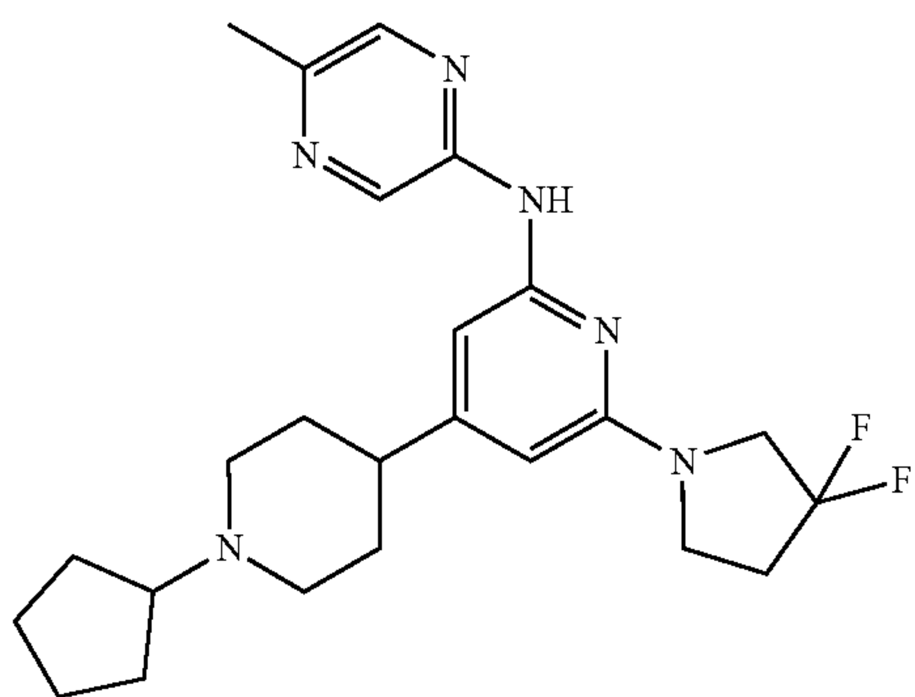
Compound 164
