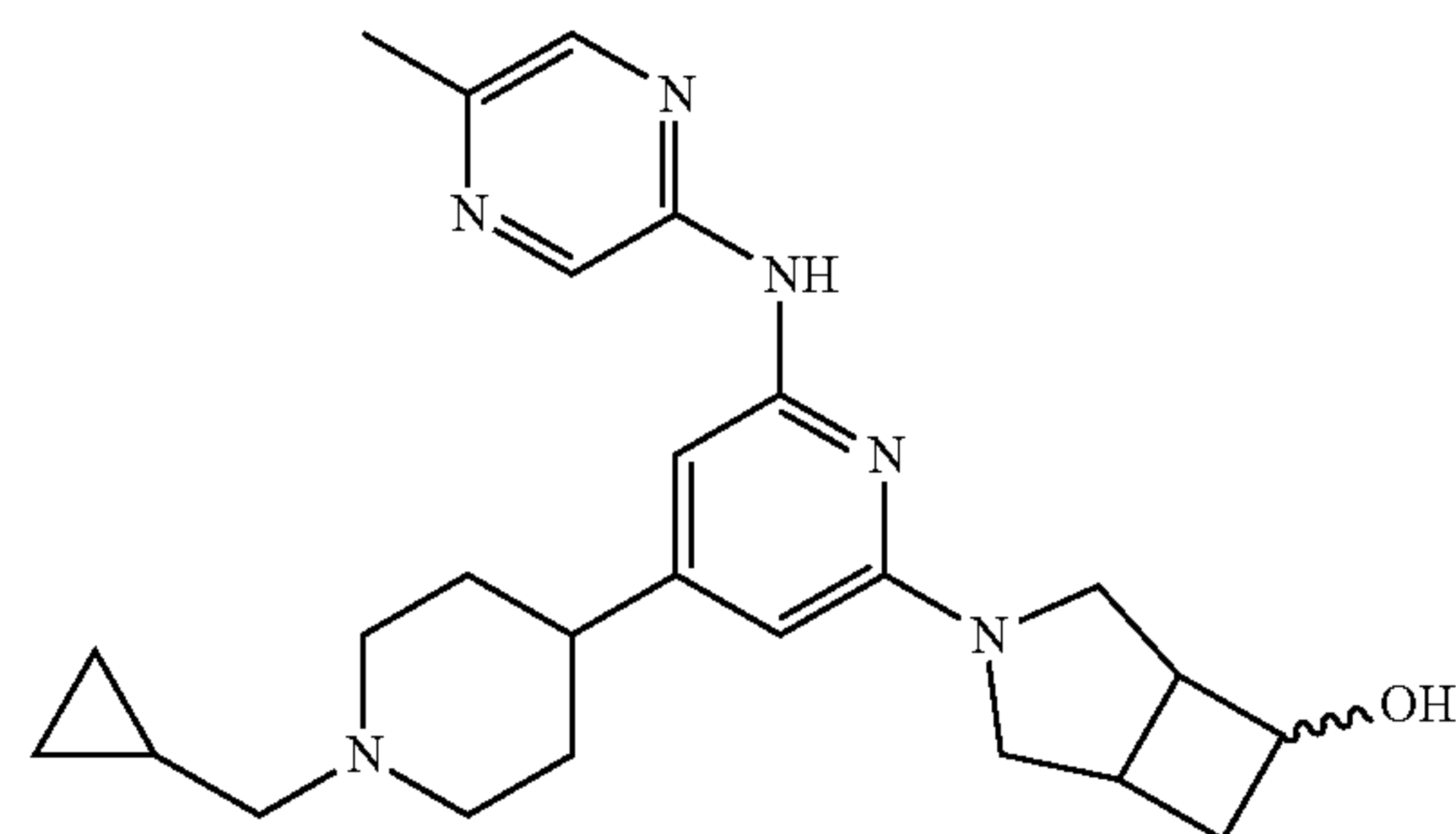
Compound 232
