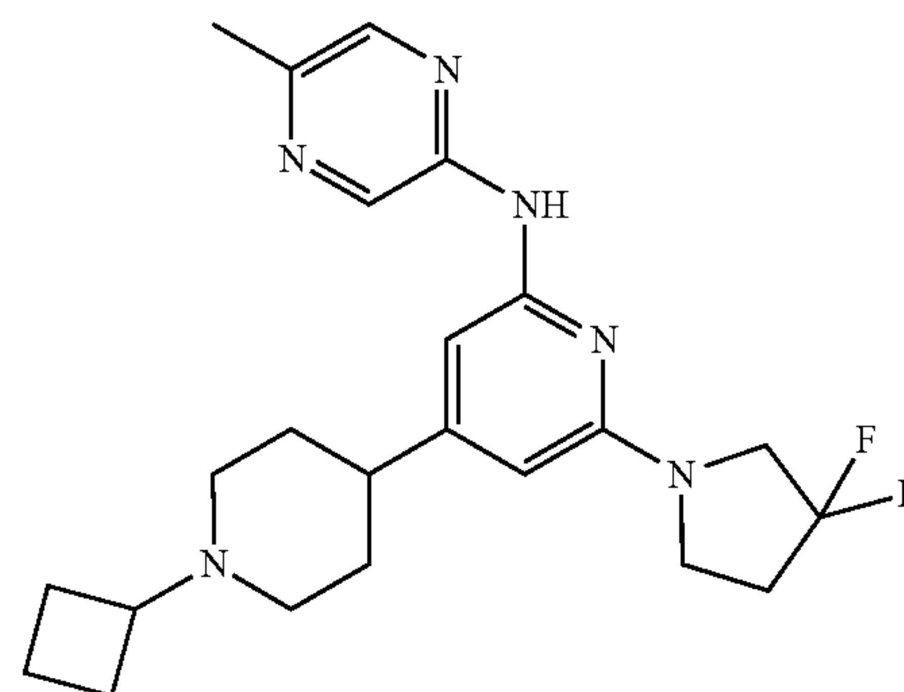
Compound 162
