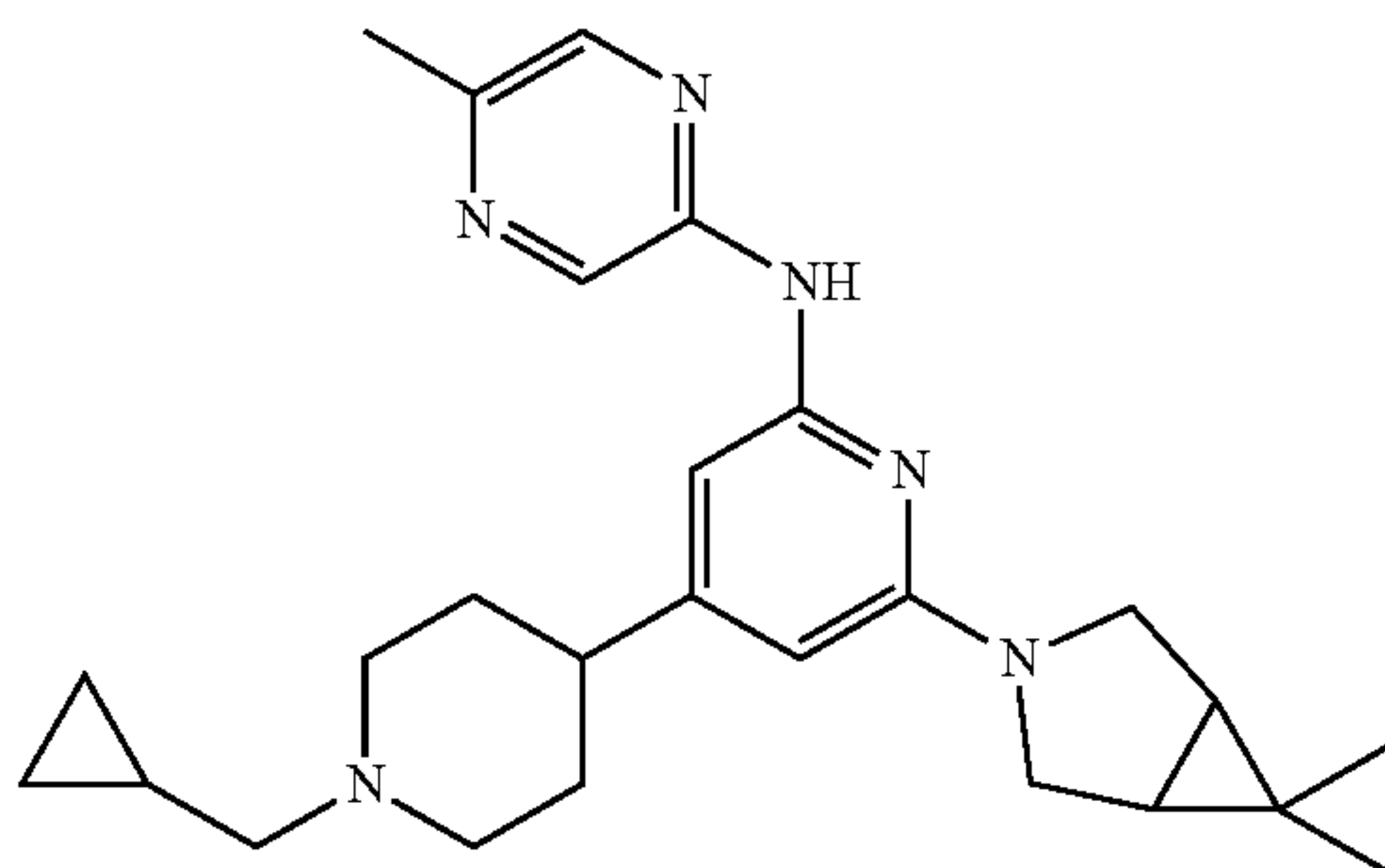
Compound 214
