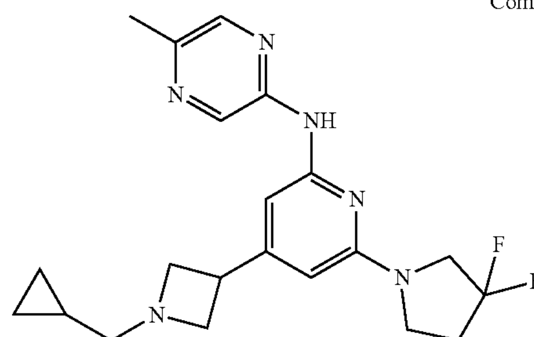
Compound 167
