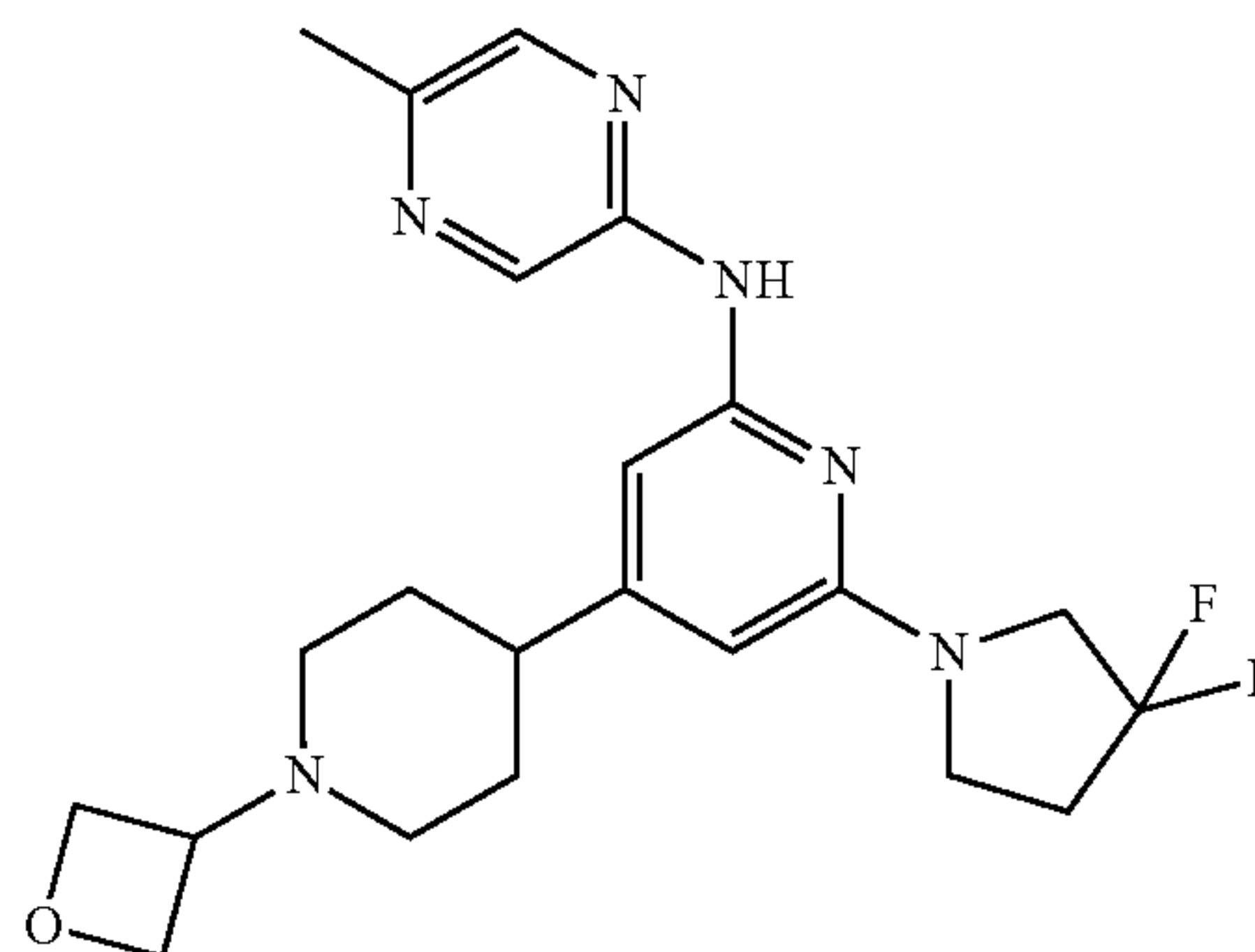
Compound 163
