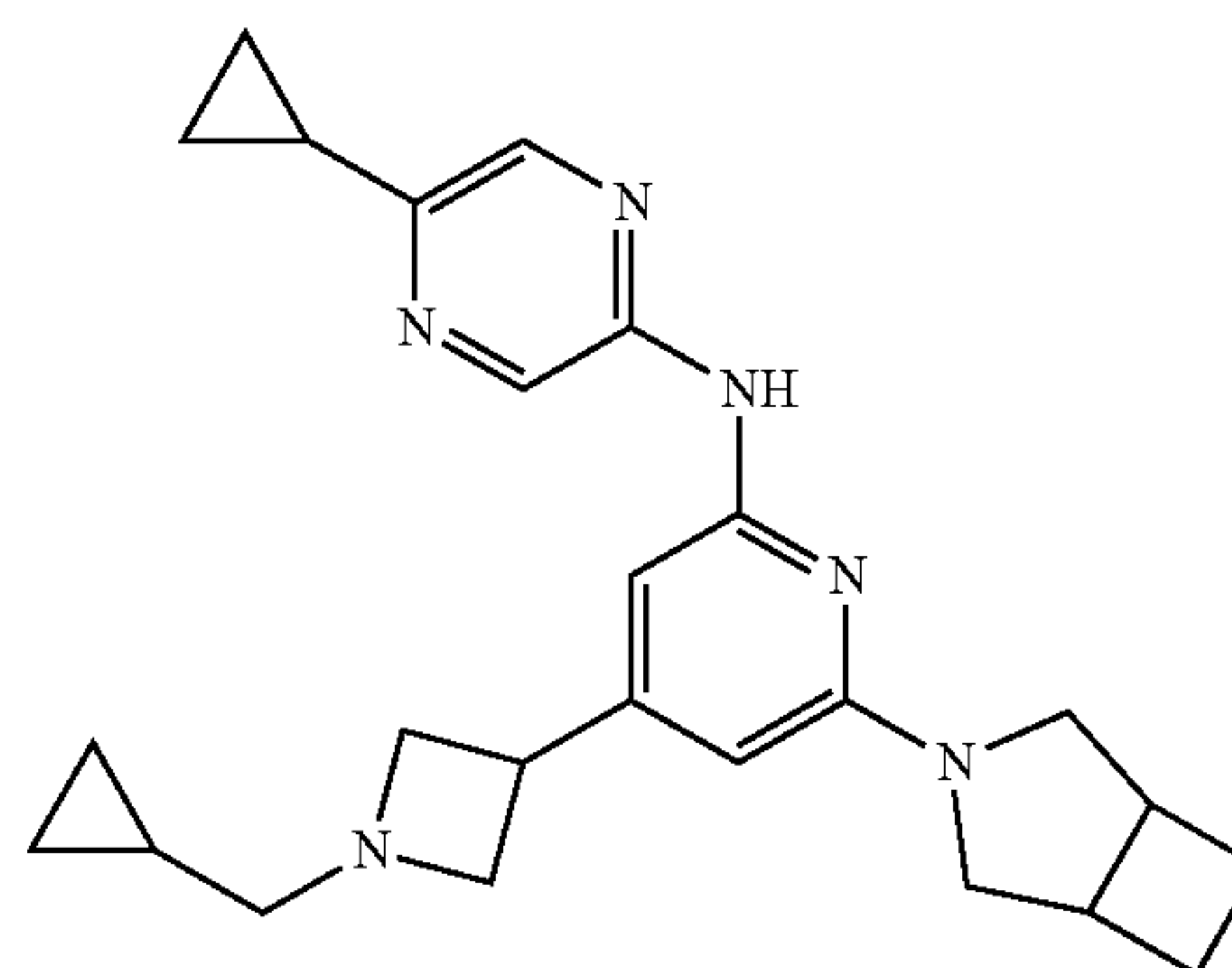
Compound 228
