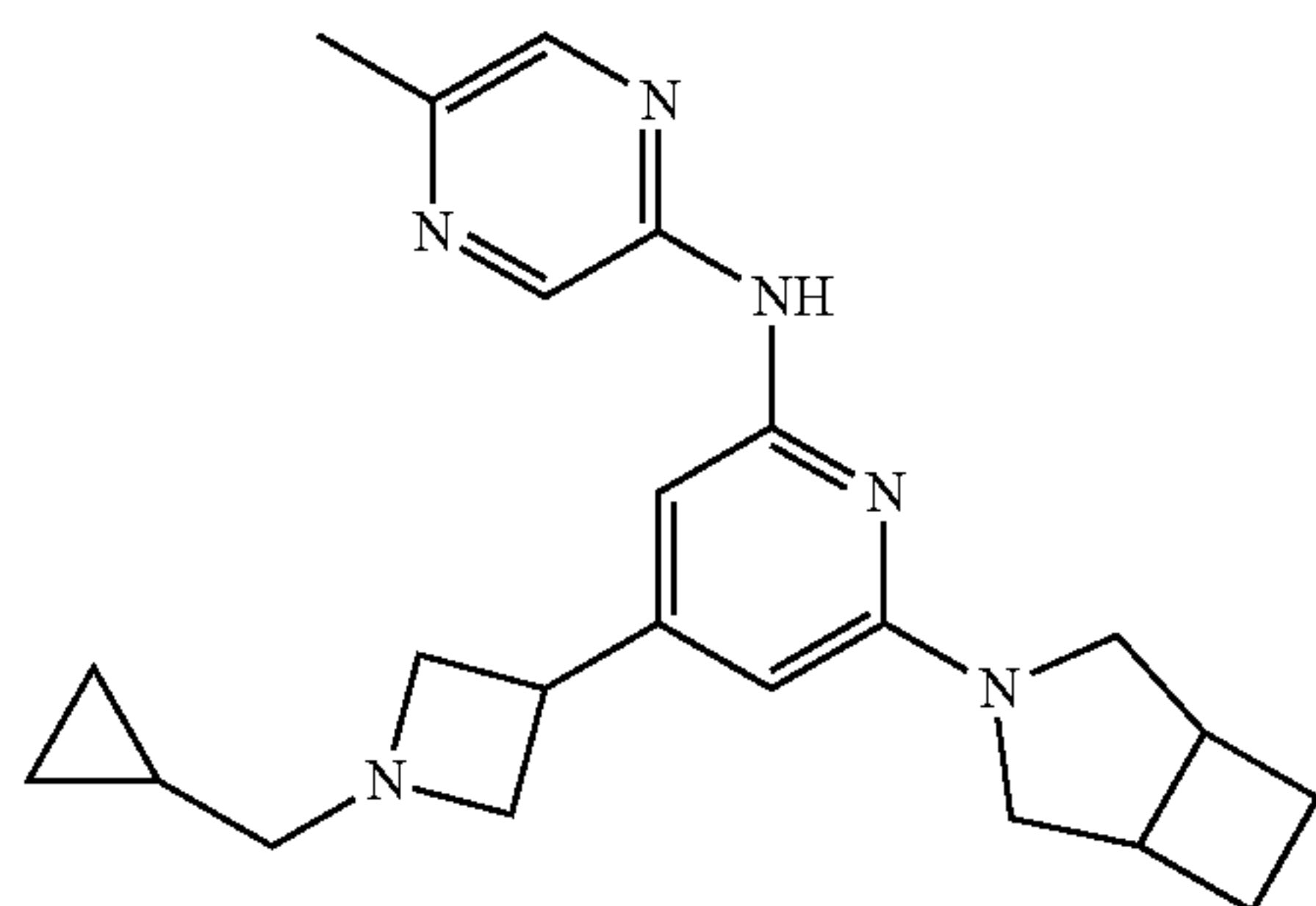
Compound 223
