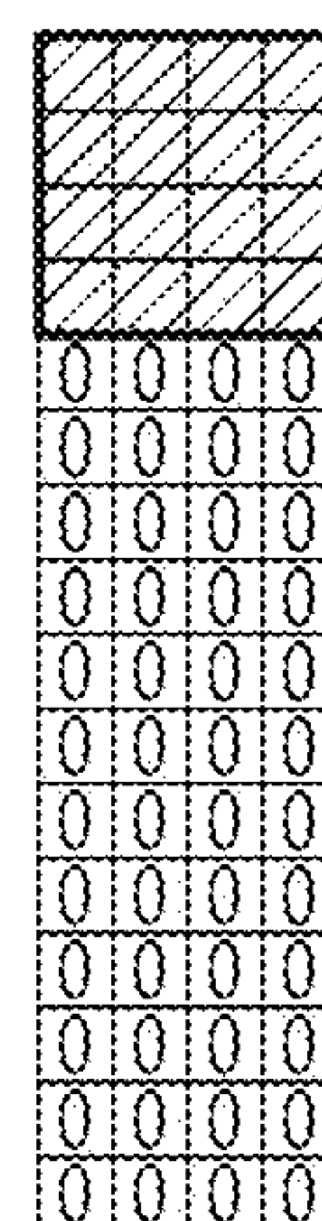
4 \times N / N \times 4 , when N \geq 16
