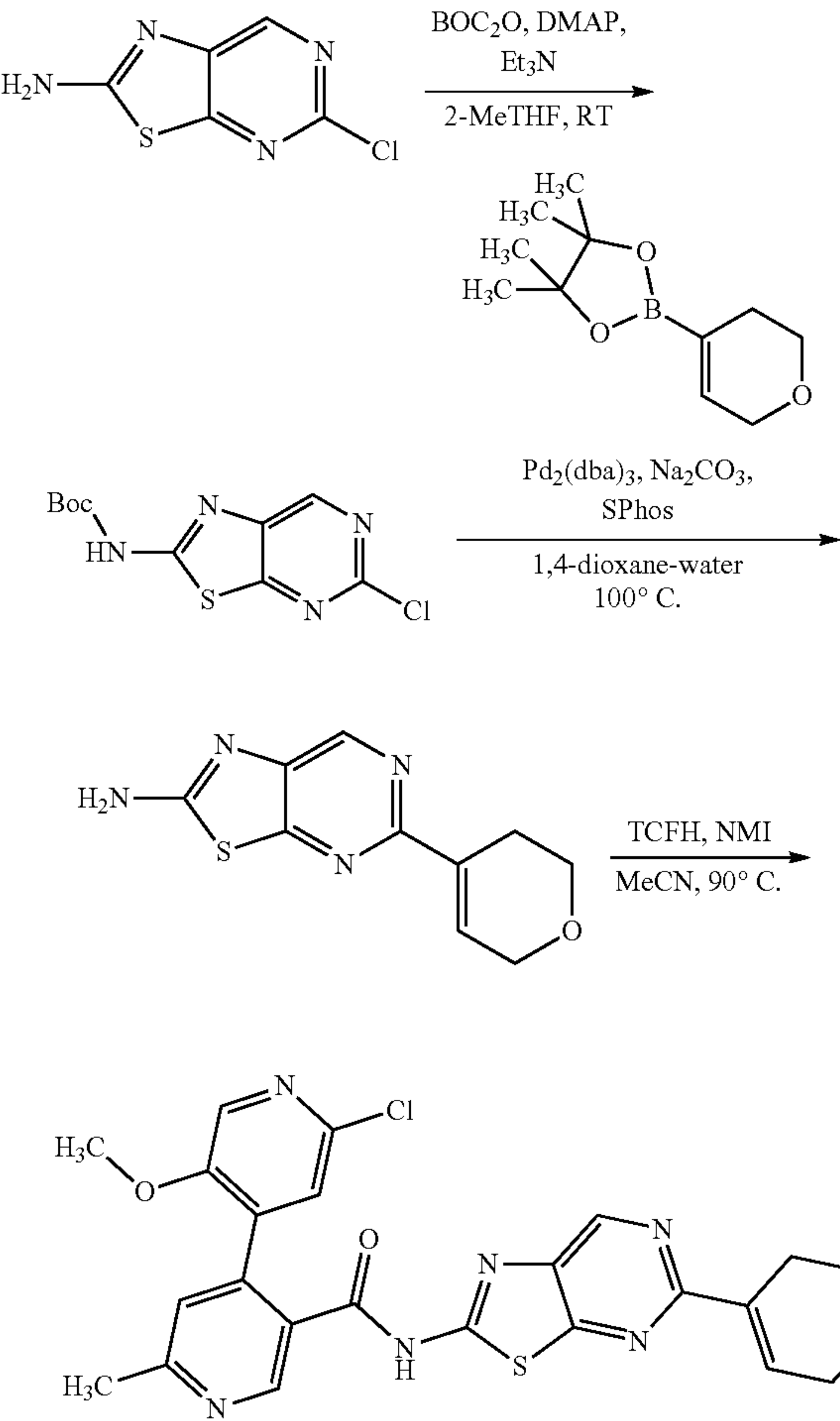
Scheme 2 Synthesis of Example 87
