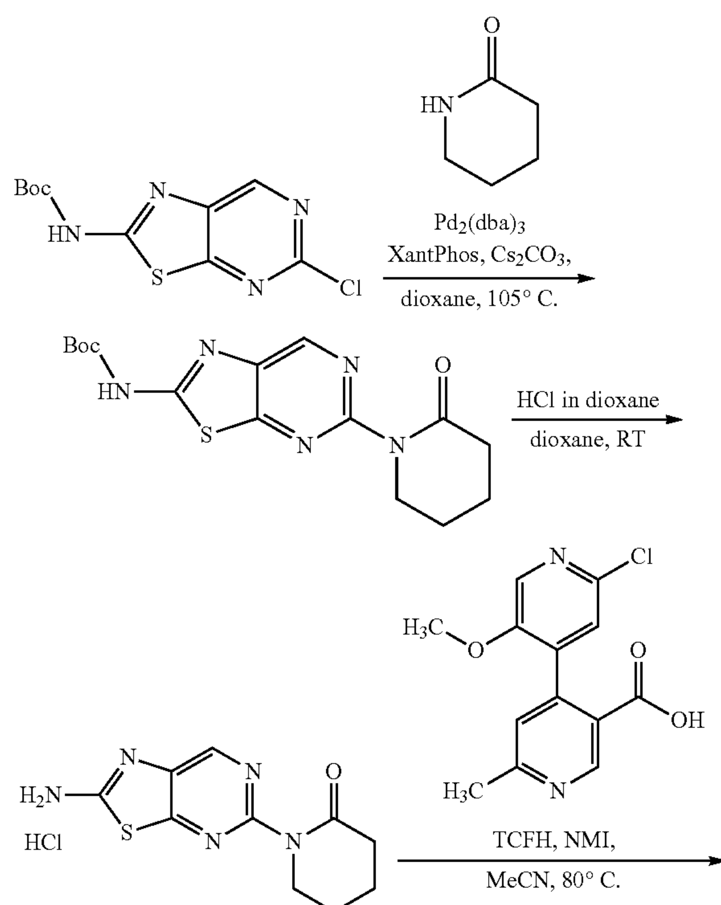
Scheme 9 Synthesis of Example 94
