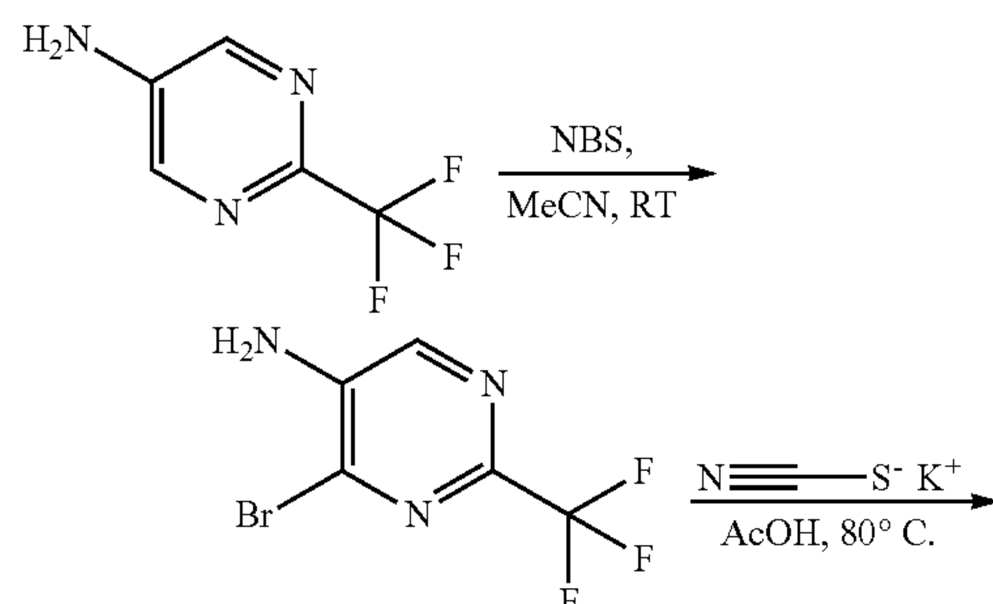
Scheme 5 Synthesis of Example 90
