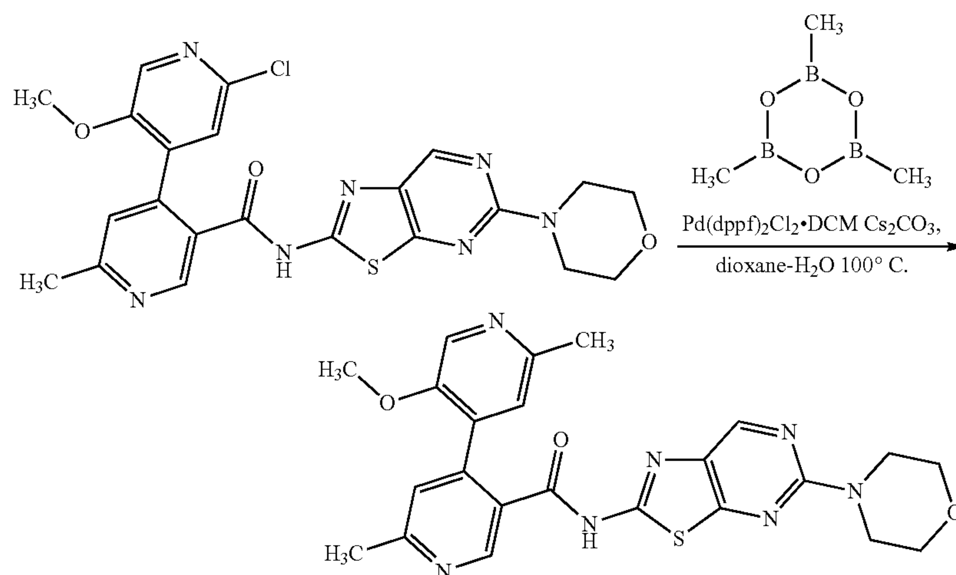
Scheme 7 Synthesis of Example 92
