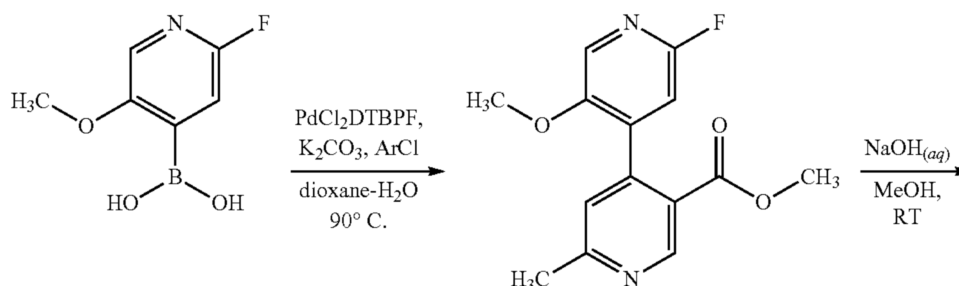
Scheme 8 Synthesis of Example 93
