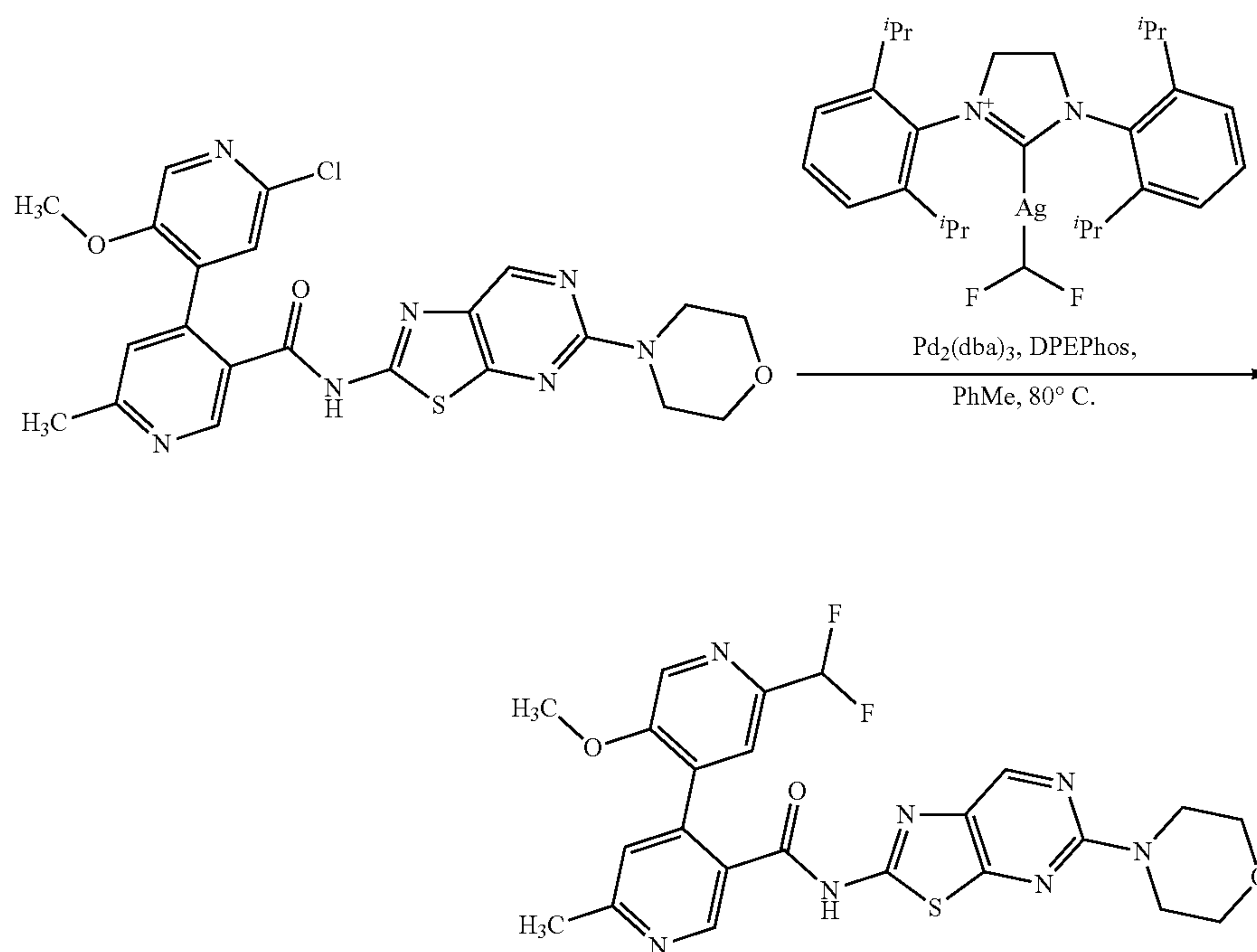
Scheme 4 Synthesis of Example 89
