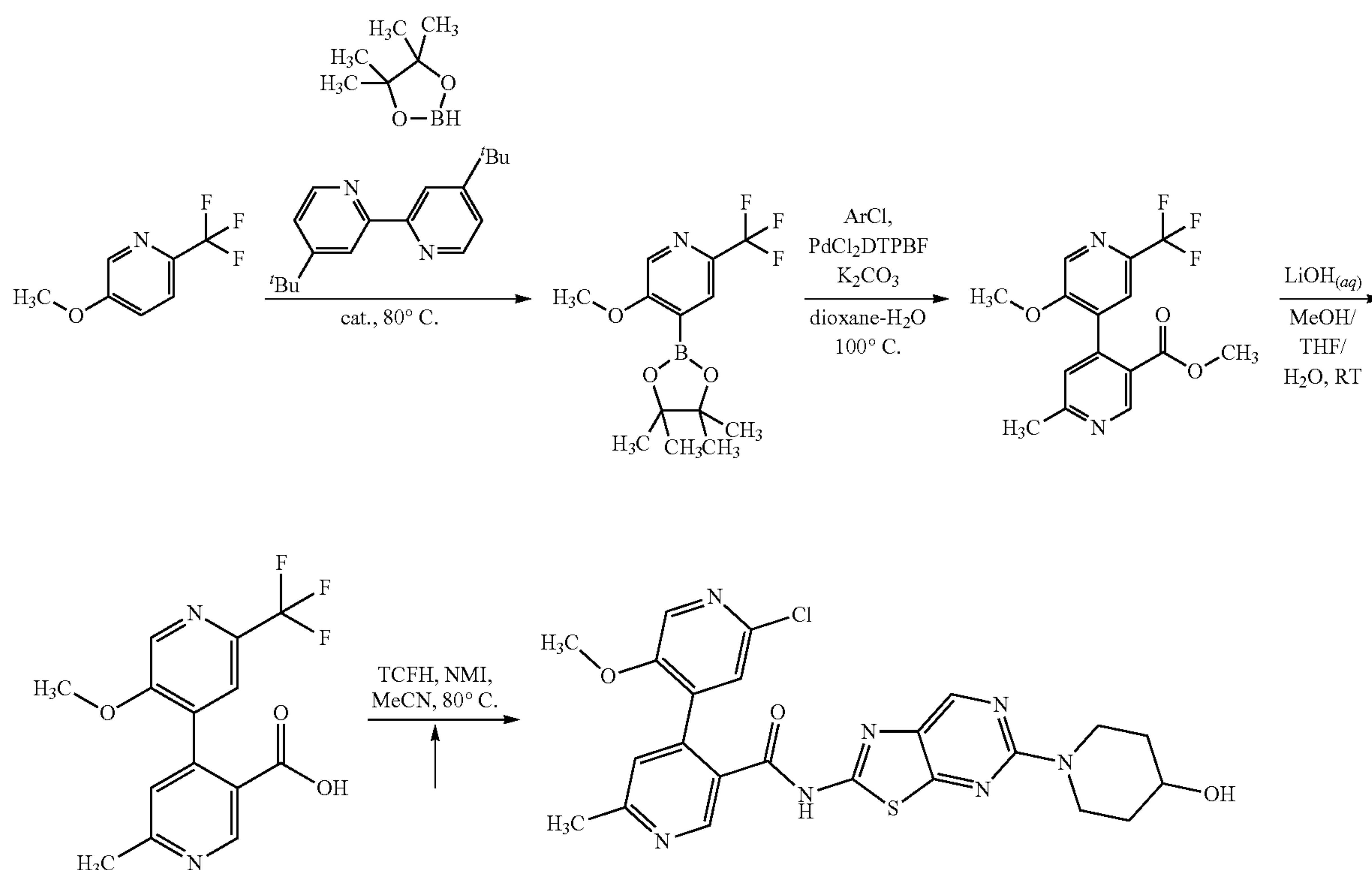
Scheme 3 Synthesis of Example 88
