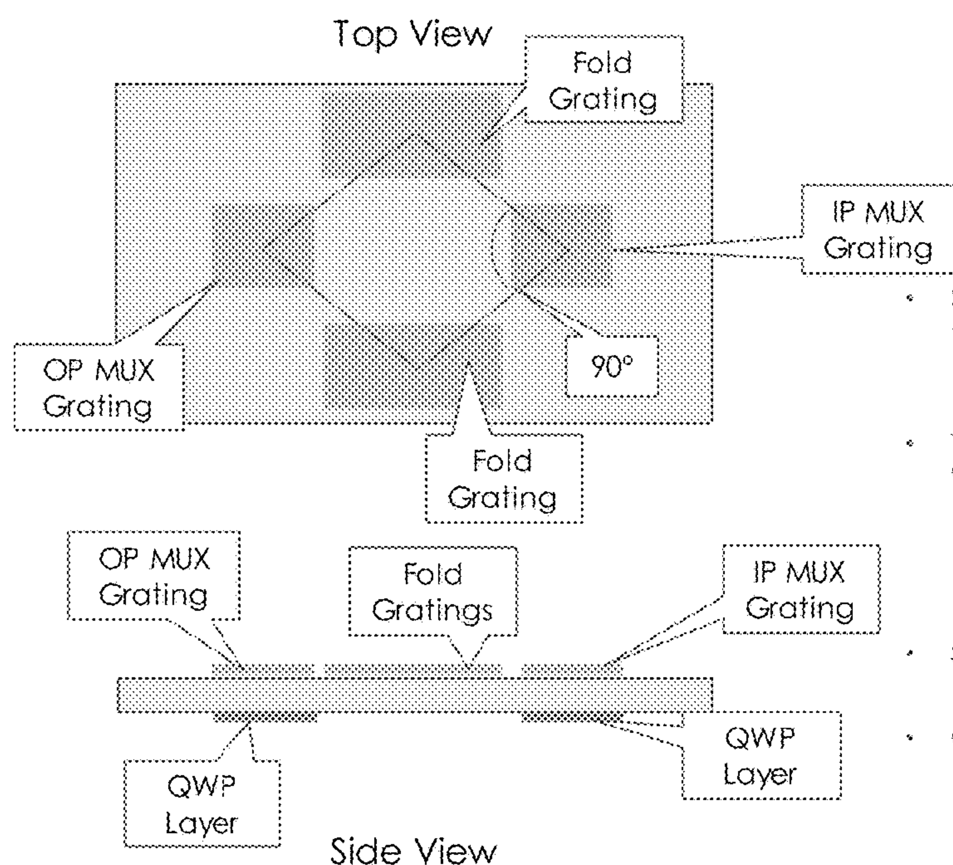
FIG. 65F Top View
