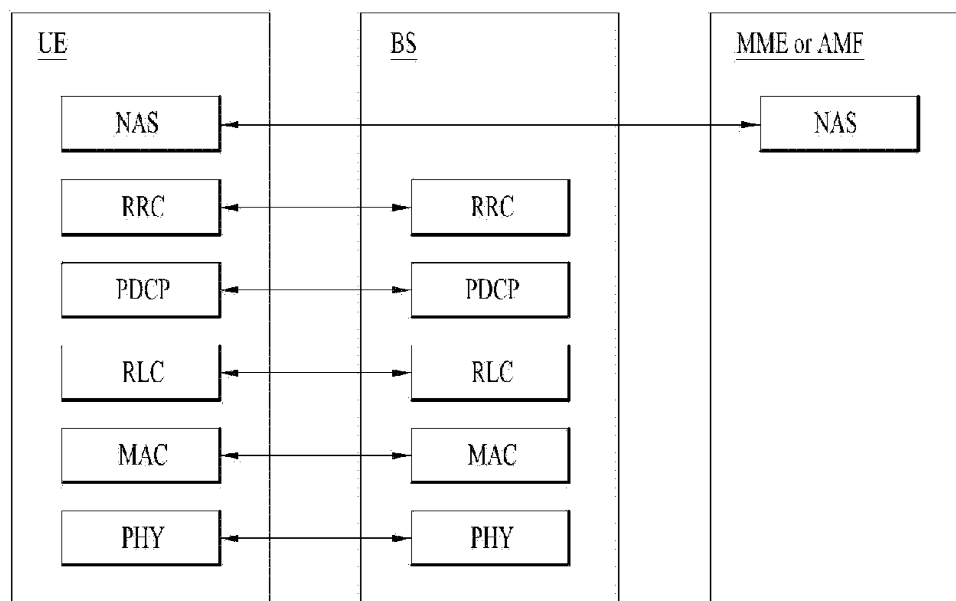
(b) Control Plane Protocol Stack
