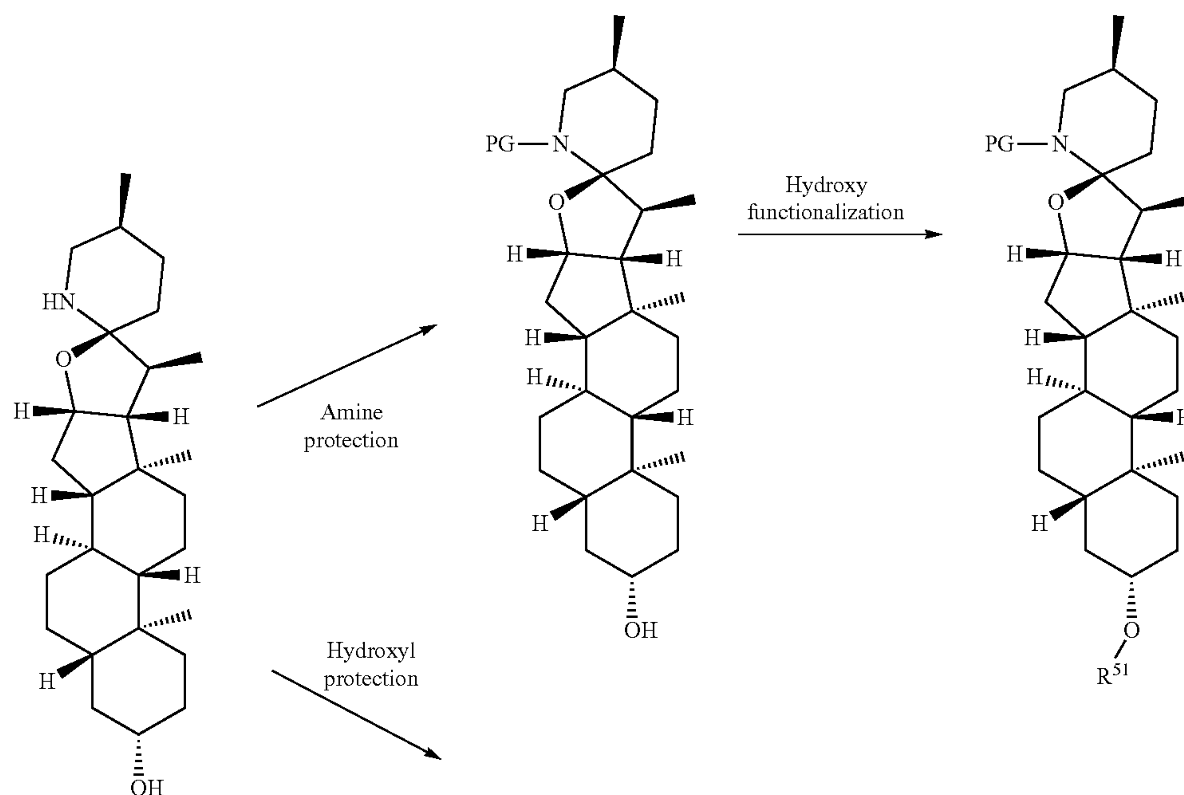
SCHEME 5A
