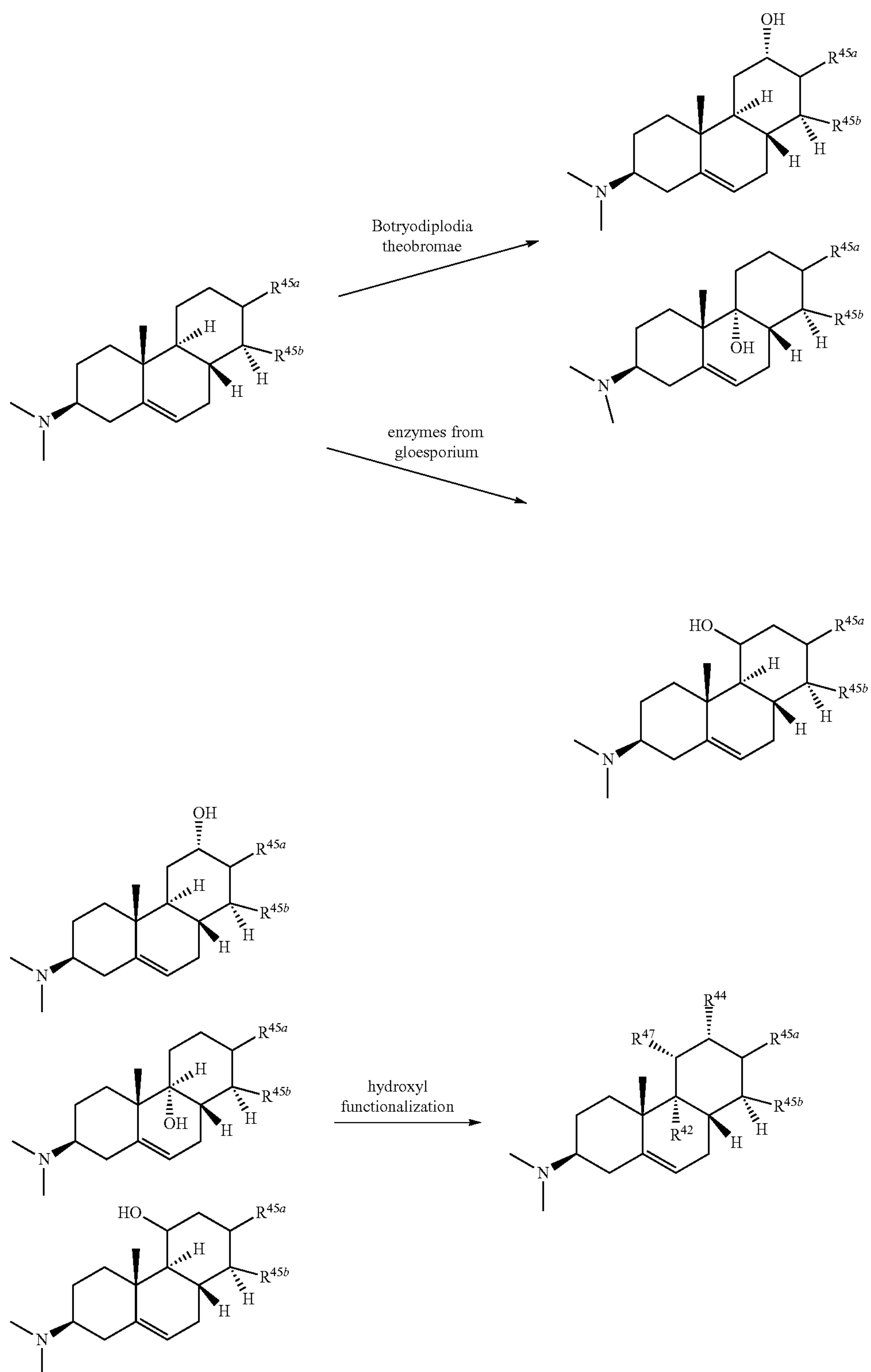
SCHEME 4A
