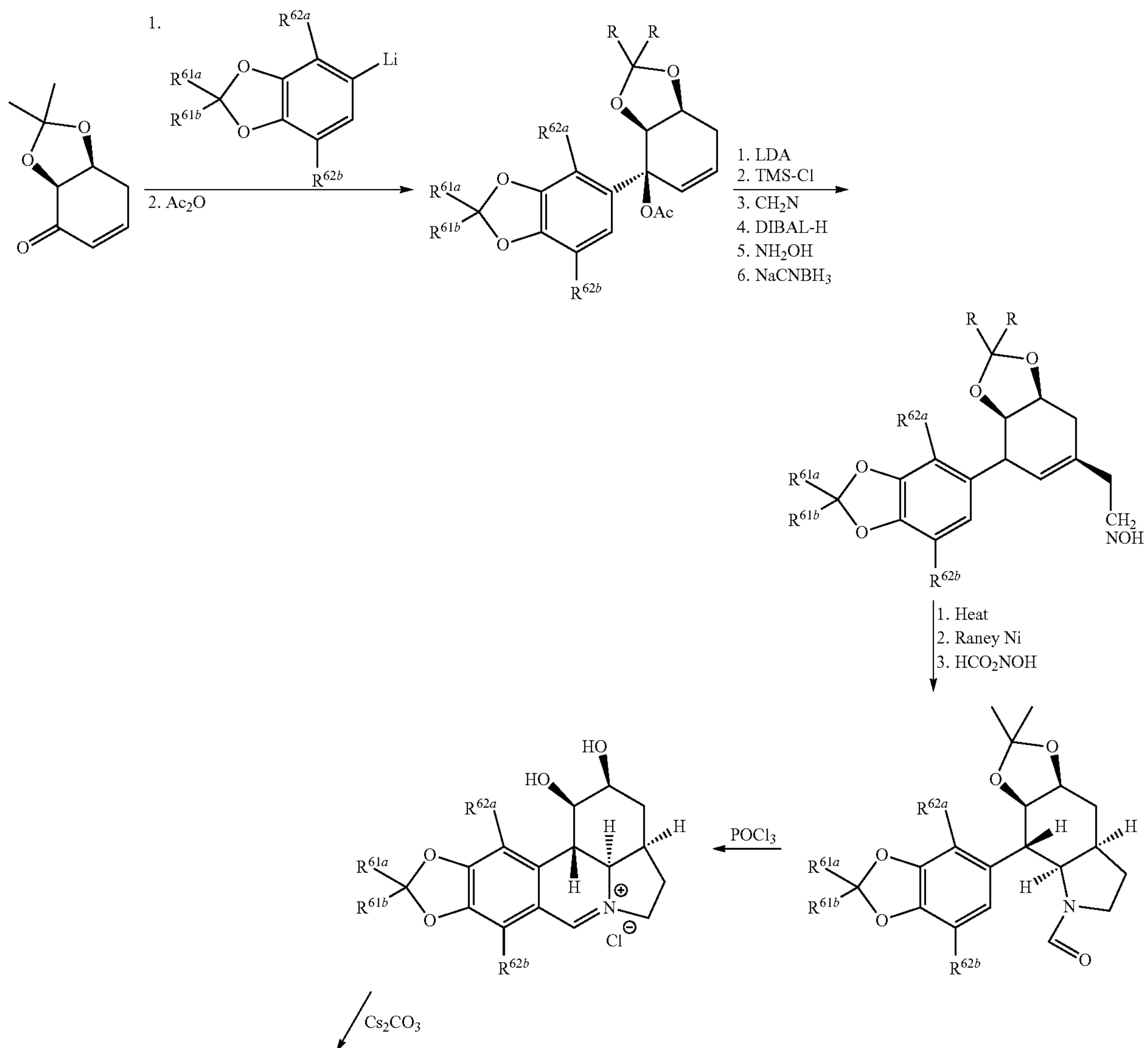
SCHEME 6B
