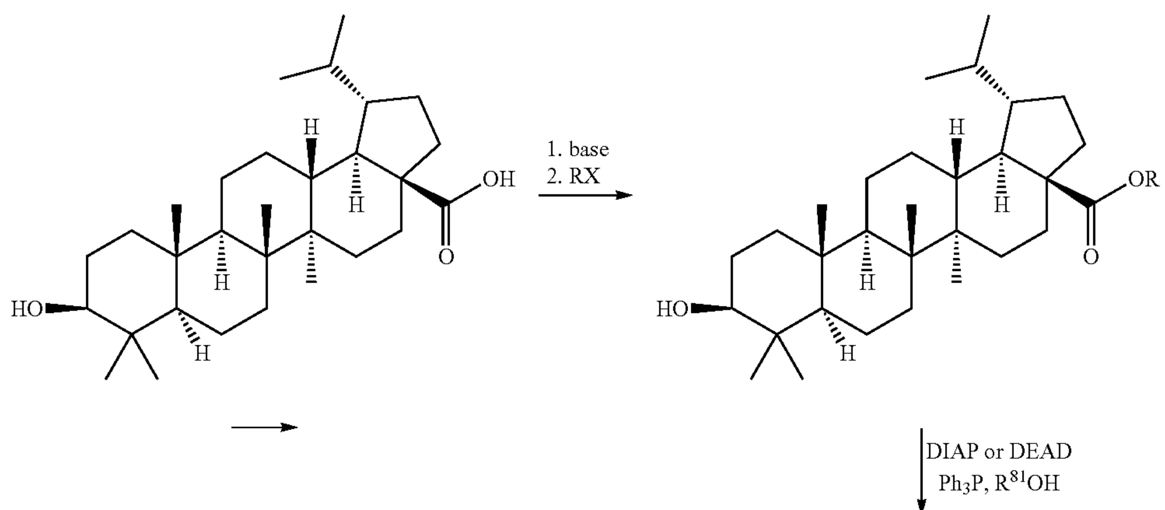
SCHEME 7B
