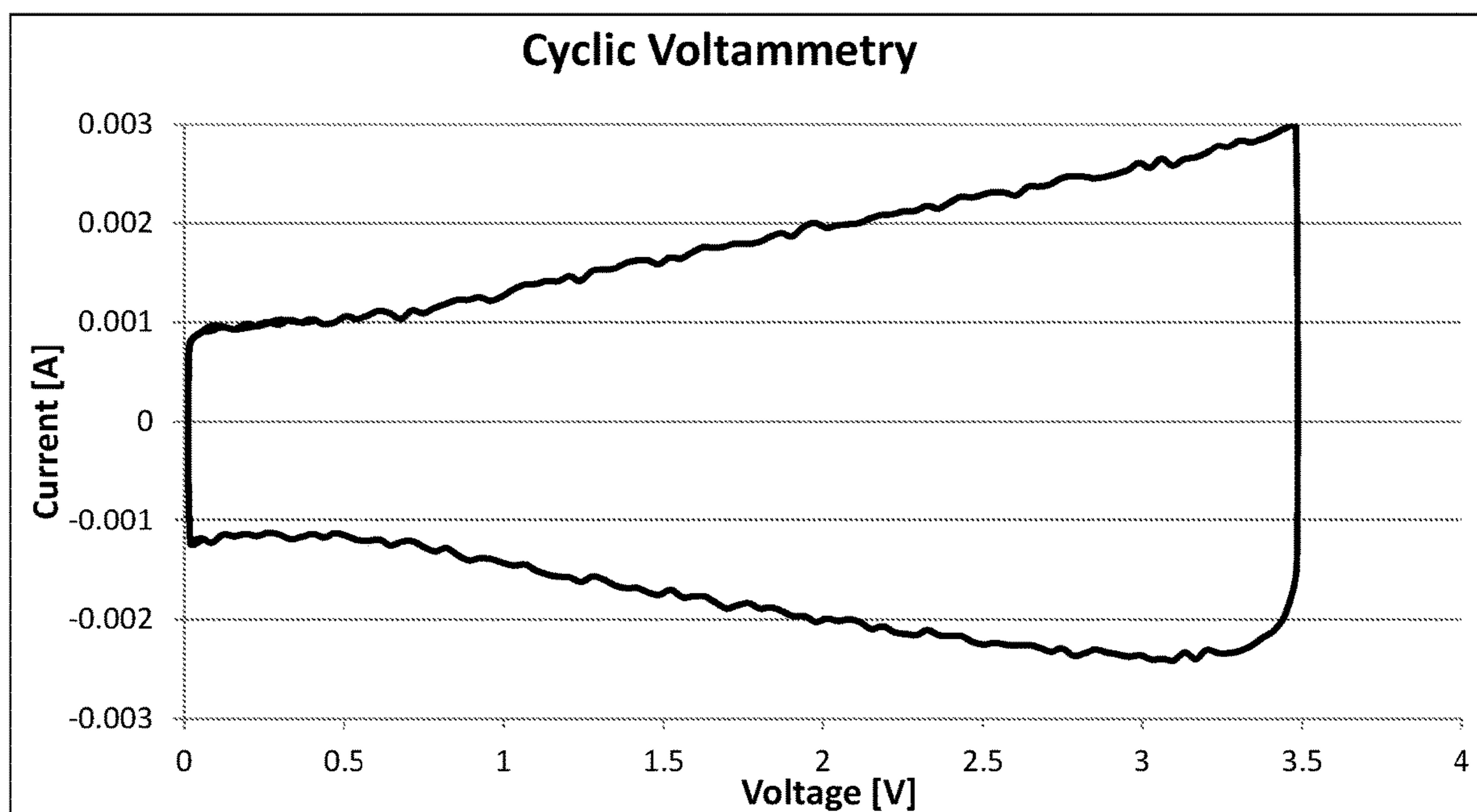
Cyclic voltametry of 1 layer of CNTs on Al_4C_3 on 50 \mu m aluminum foil.
