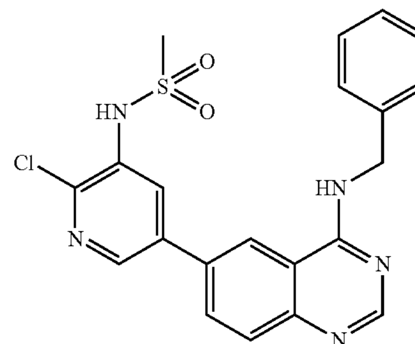
Comparative Compound 1
