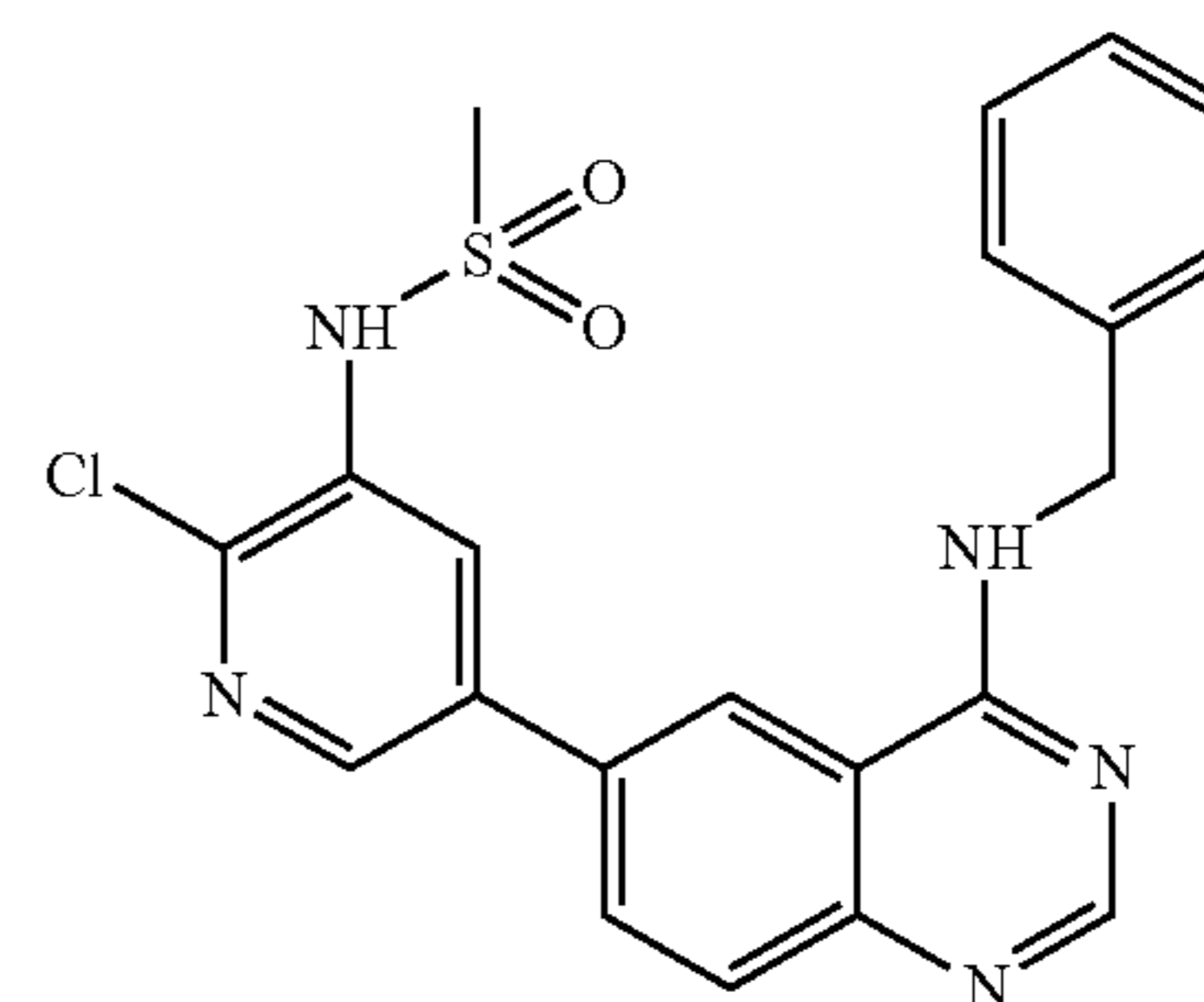
Comparative Compound 1
