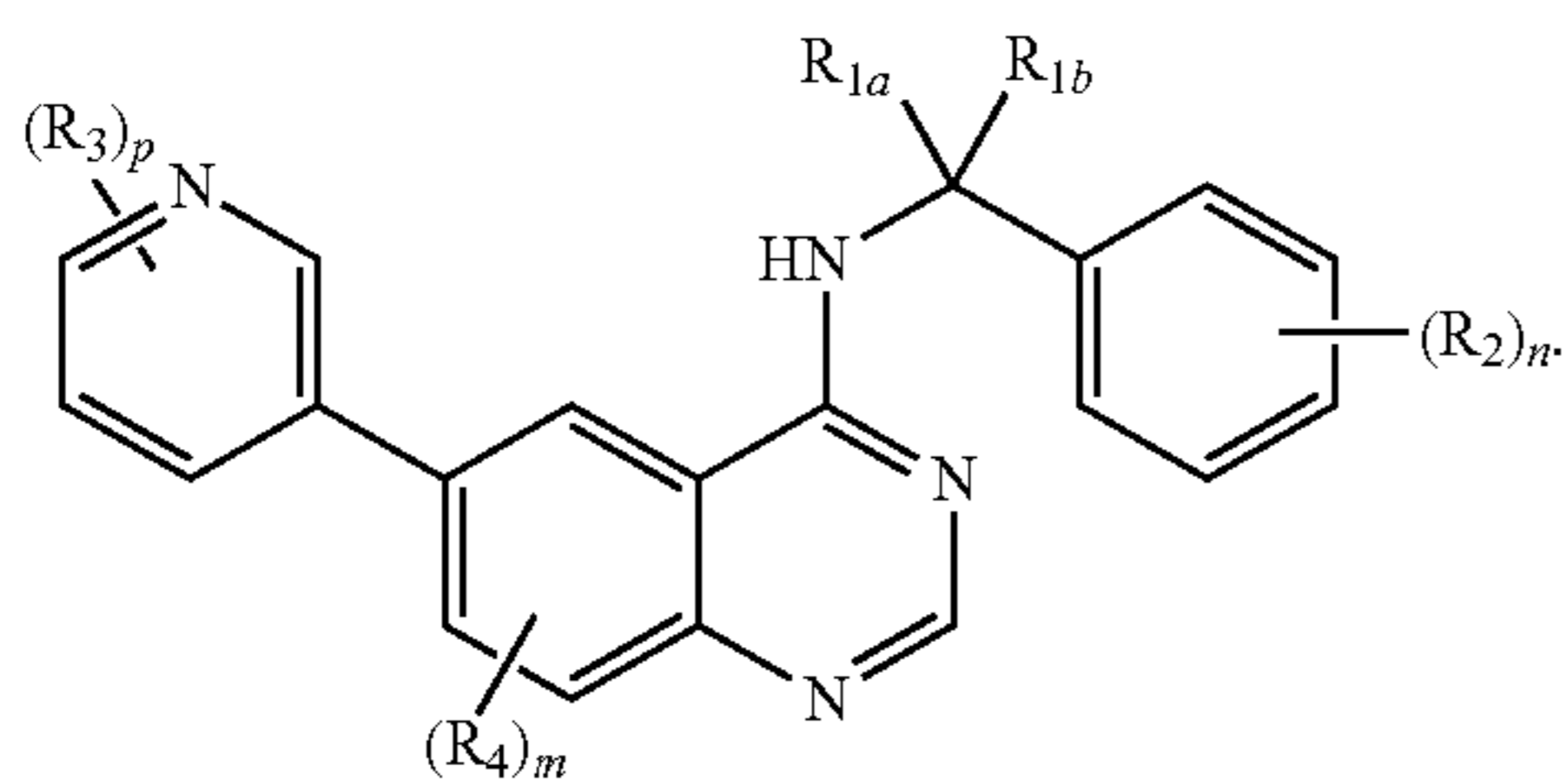
Formula Ia-2
