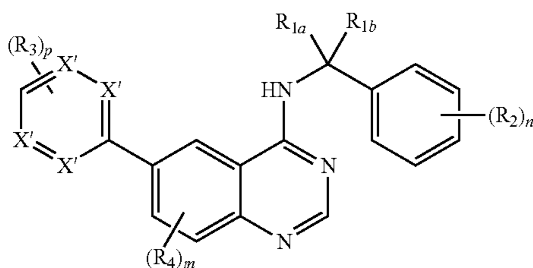
Formula Ia-1
