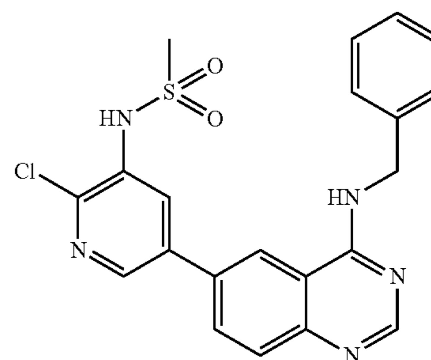
Comparative Compound 1
