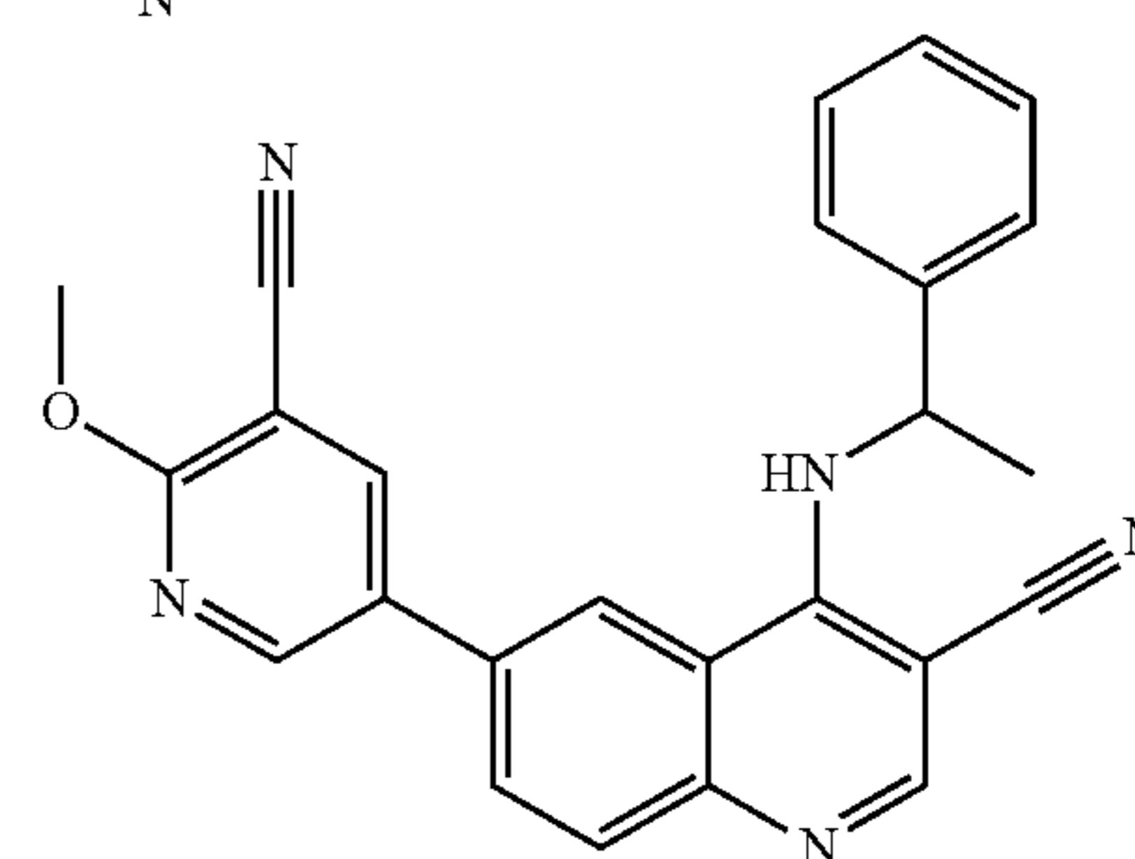
Compound 126
