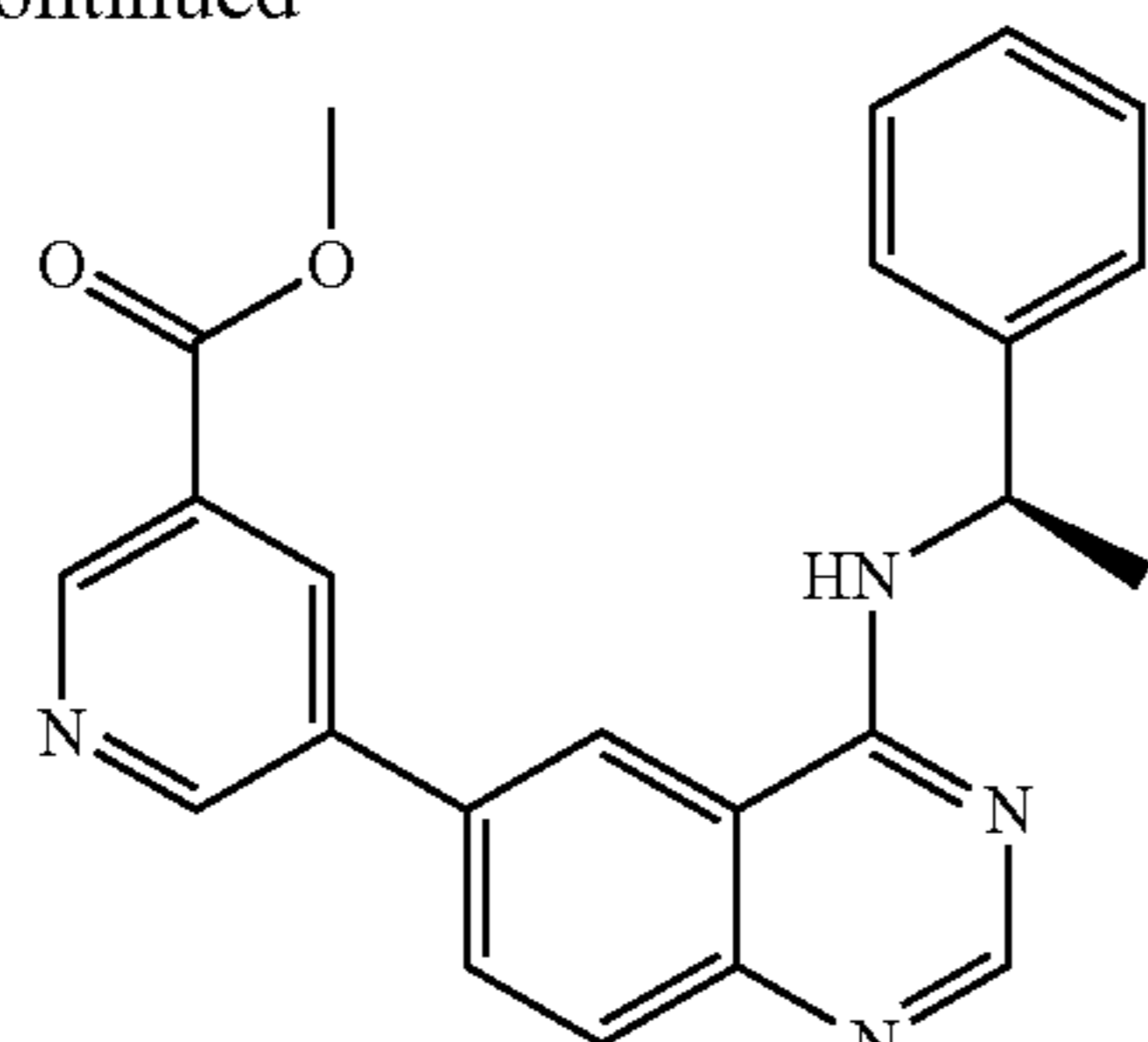
Compound 135
