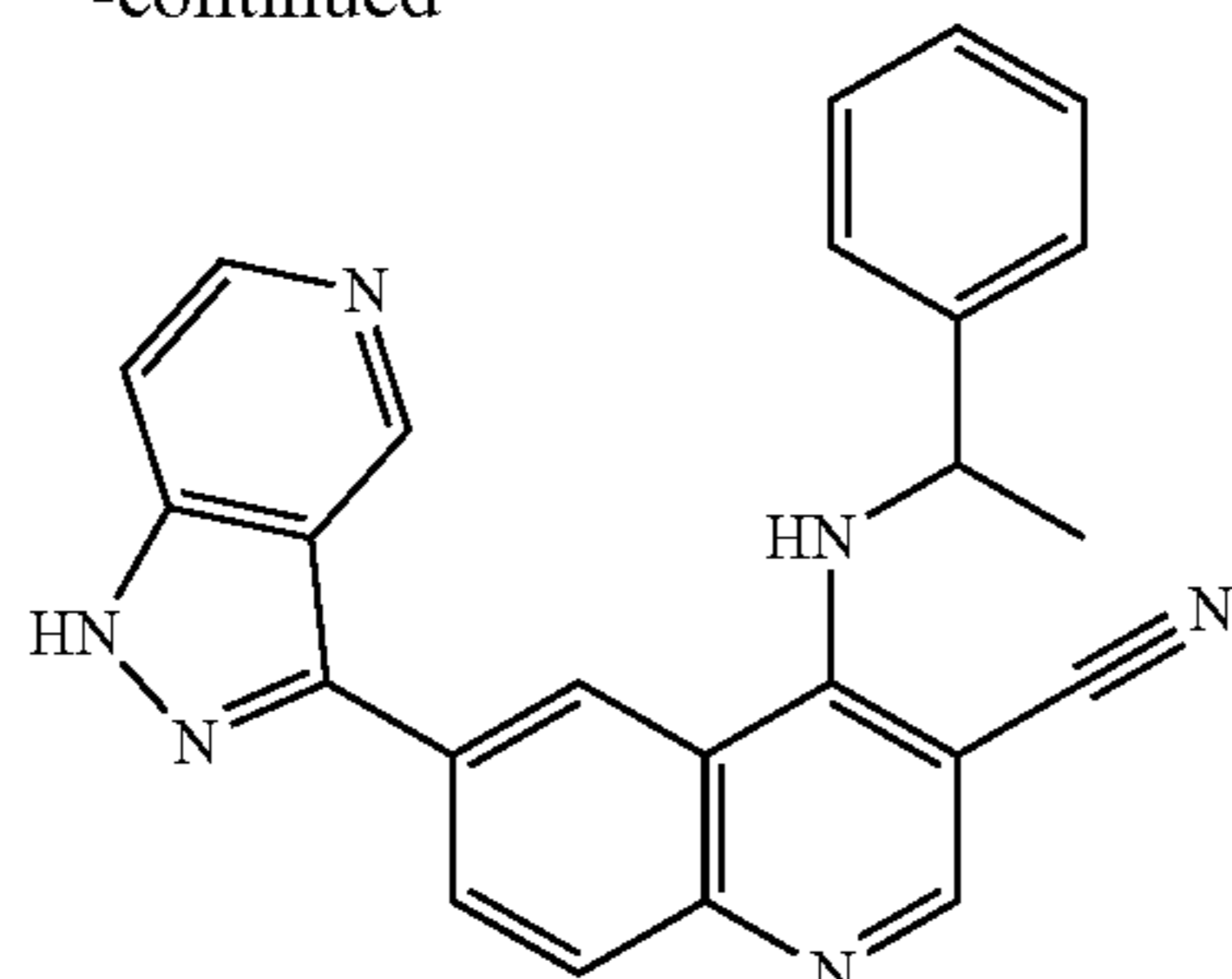
Compound 124
