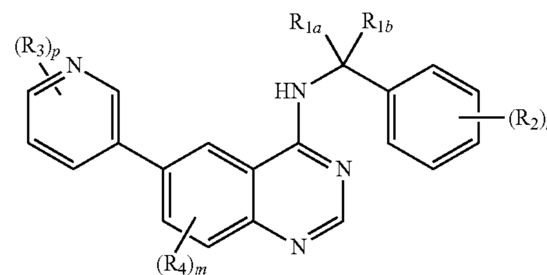
Formula Ia-2
