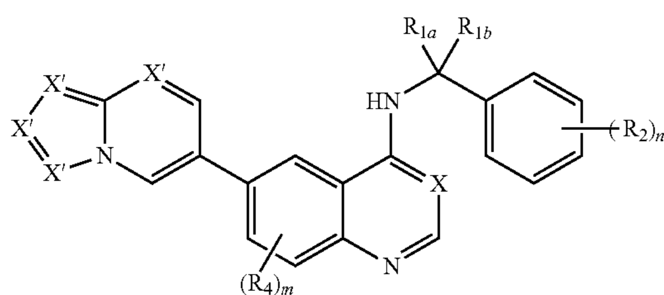
Formula Ic-2
