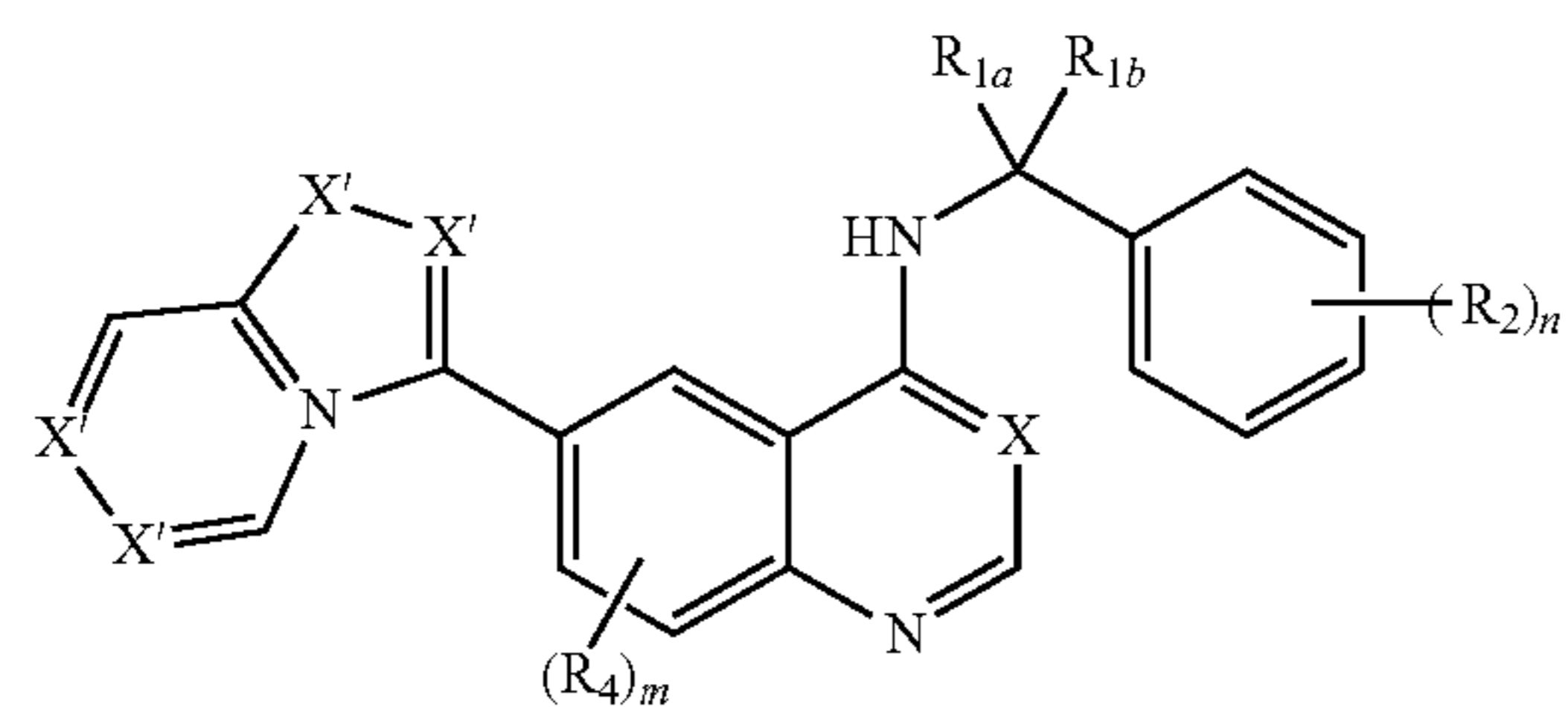
Formula Ic-3
