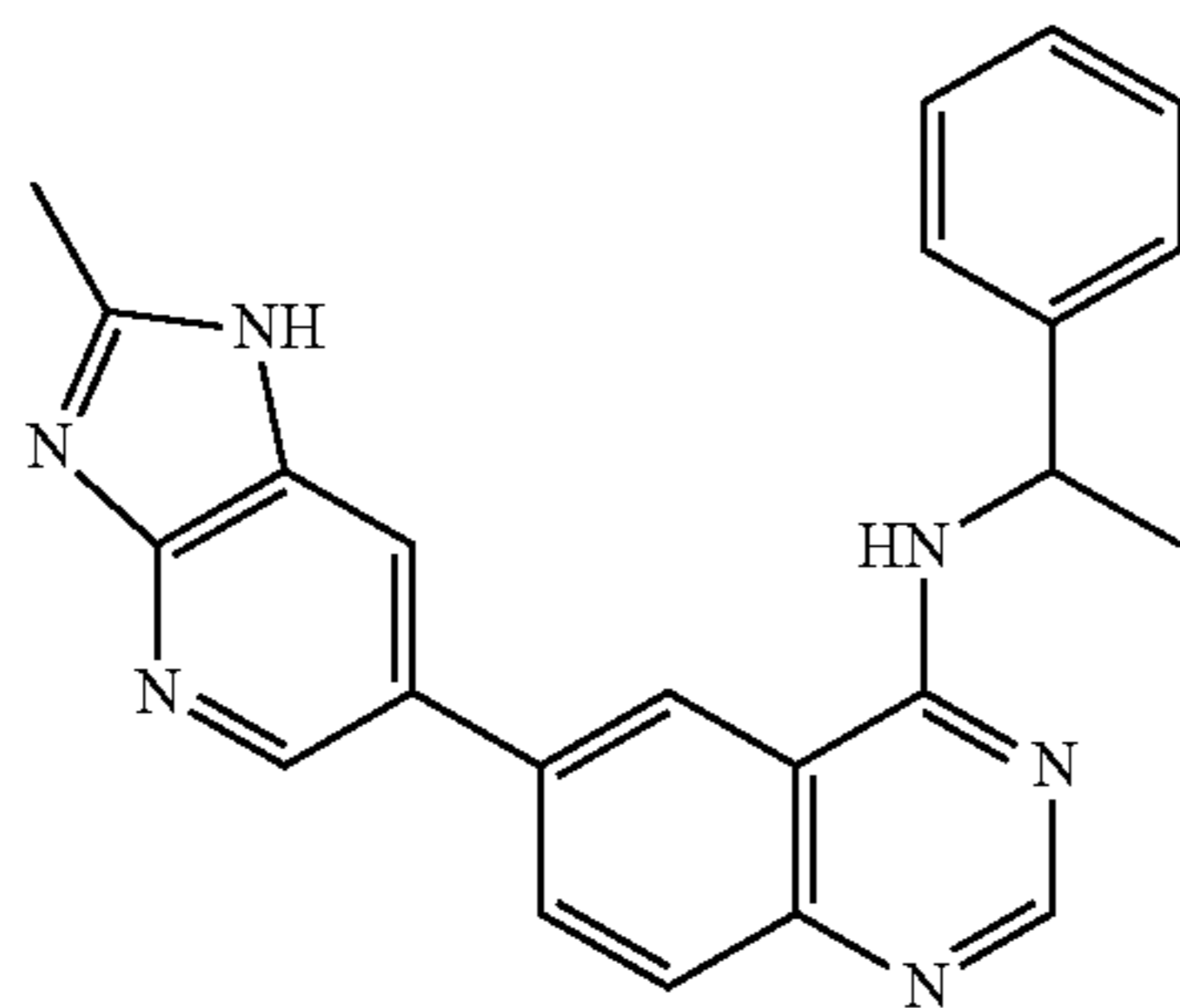
Compound 10
