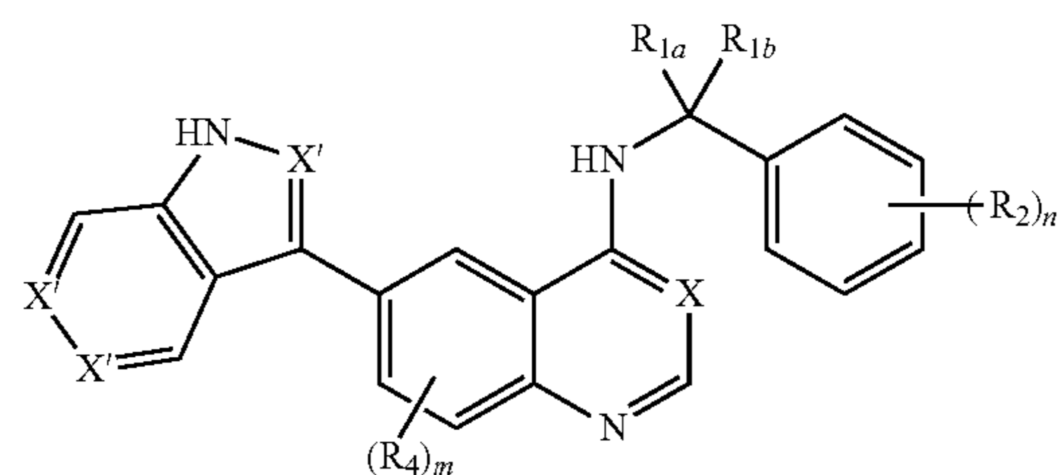
Formula Ic-3
