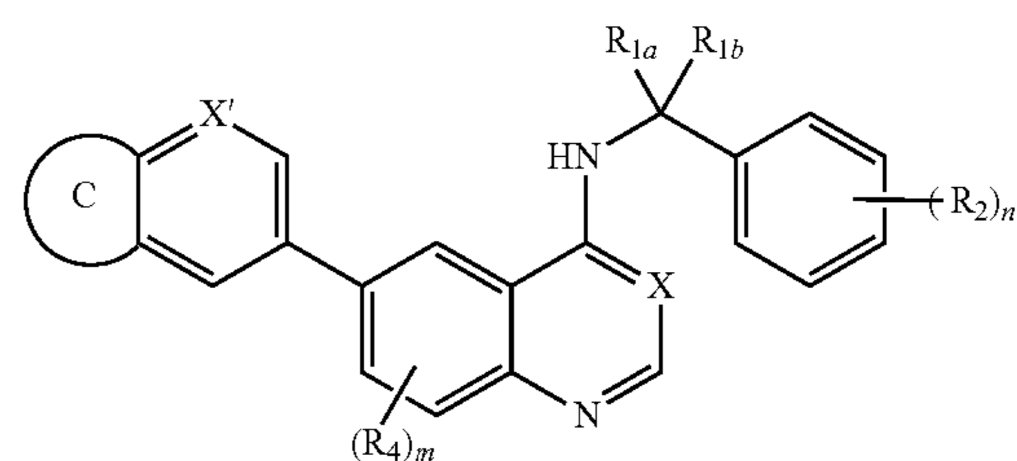
Formula Ib
