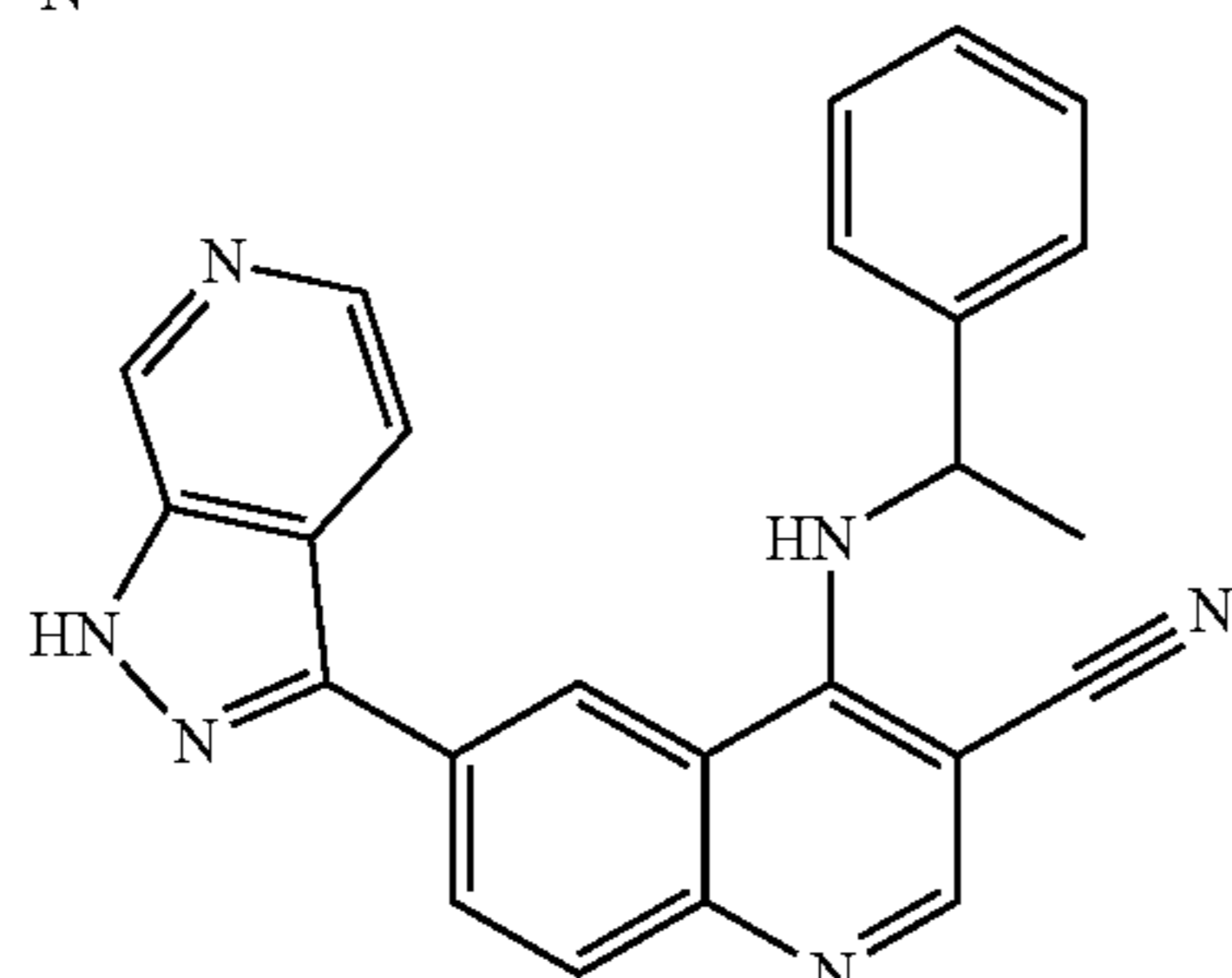
Compound 125
