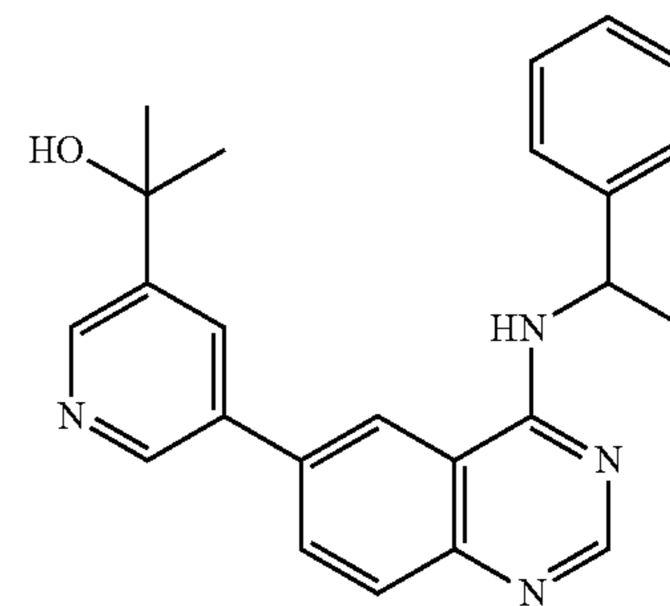
Compound 21
