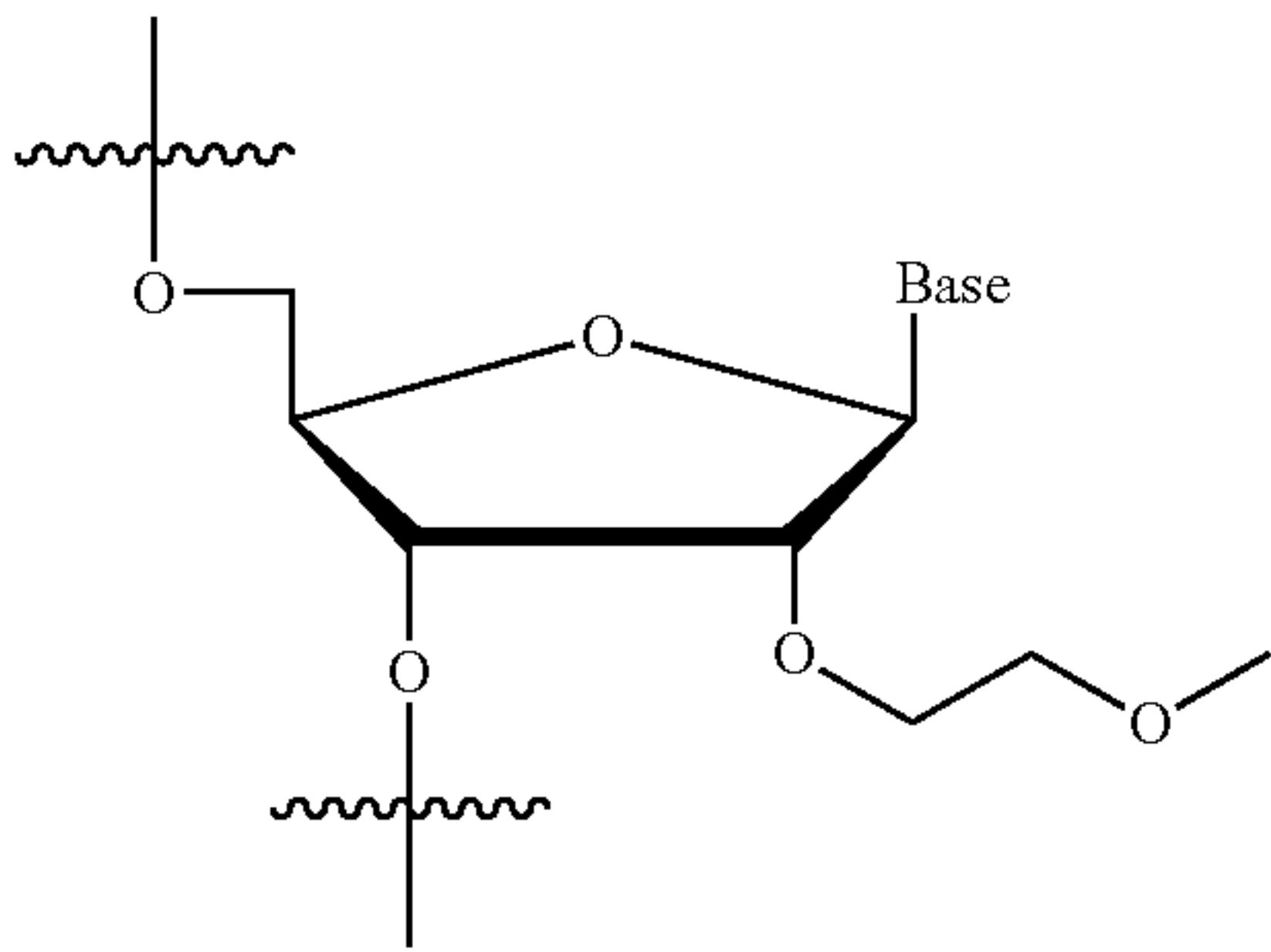
2'-O-methoxyethyl (2'-O-ME)
