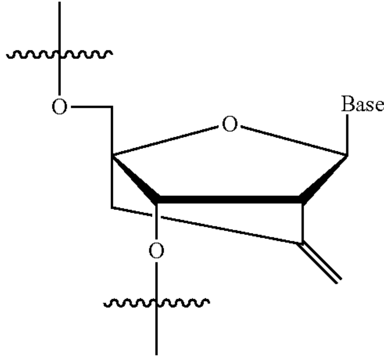
Methylene-cLAN
