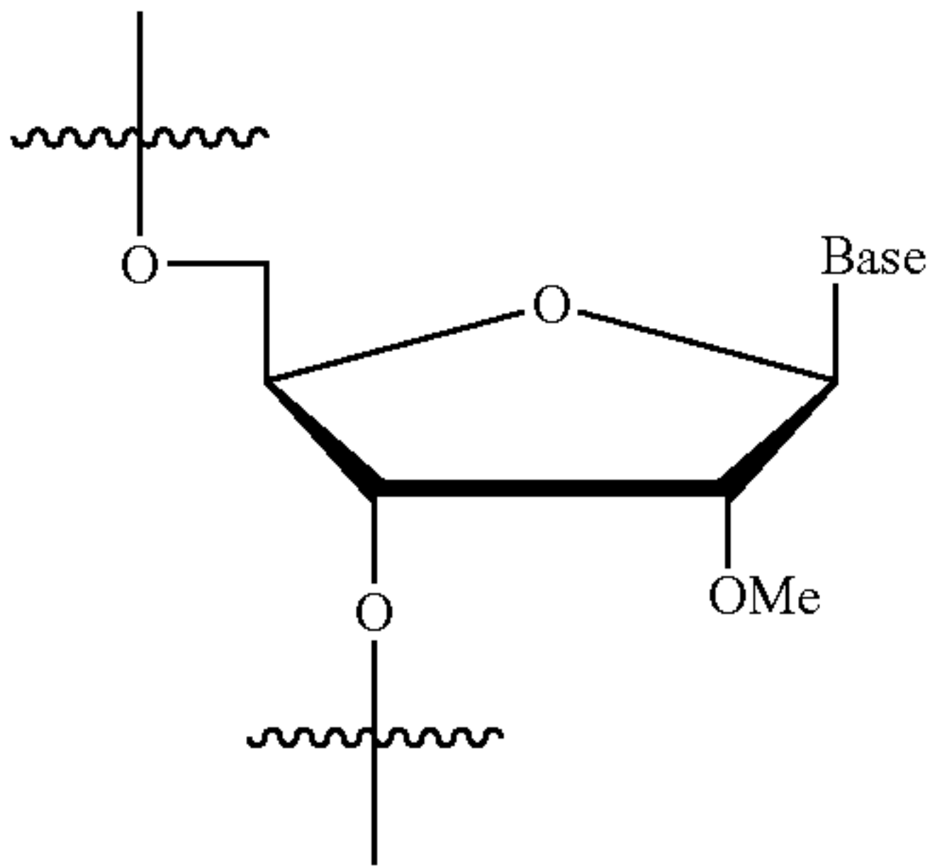
2'-O-methyl (2'-O-Me)
