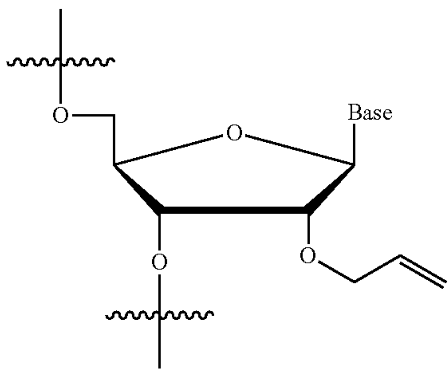
2'-O-Allyl
