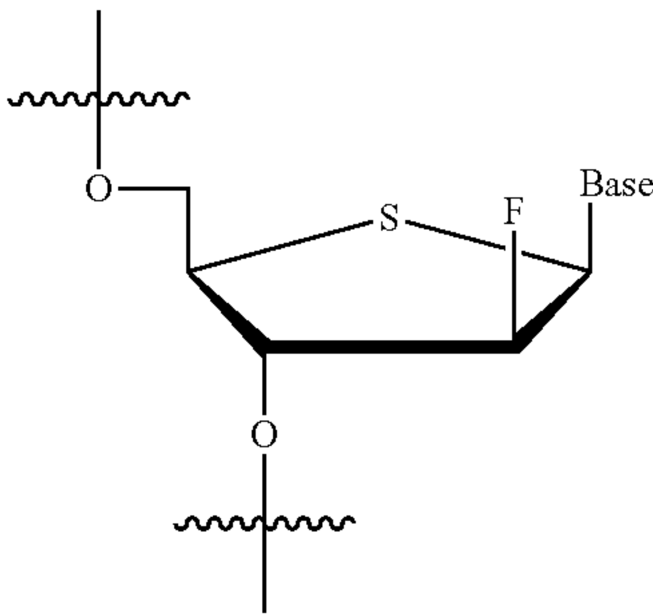
4'-SFANA
