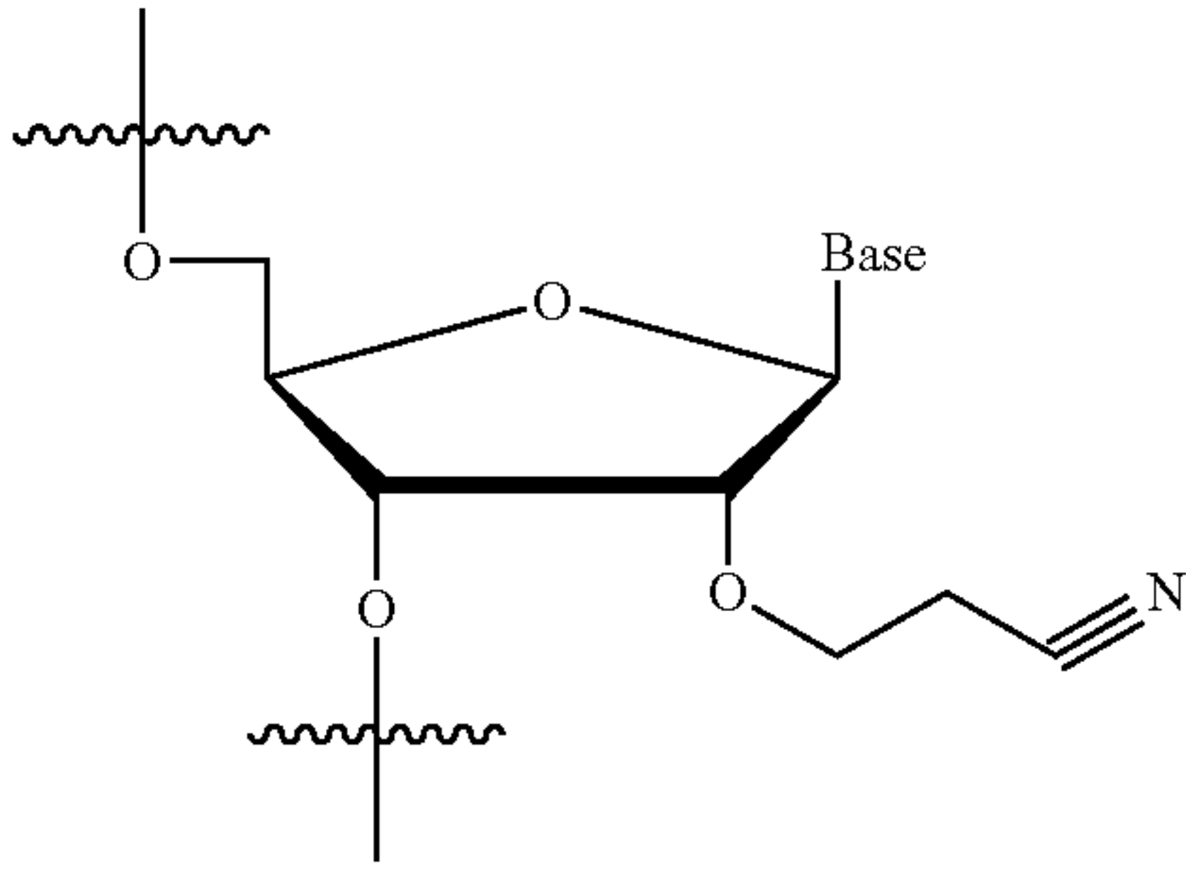
2'-O-Cyanoethyl
