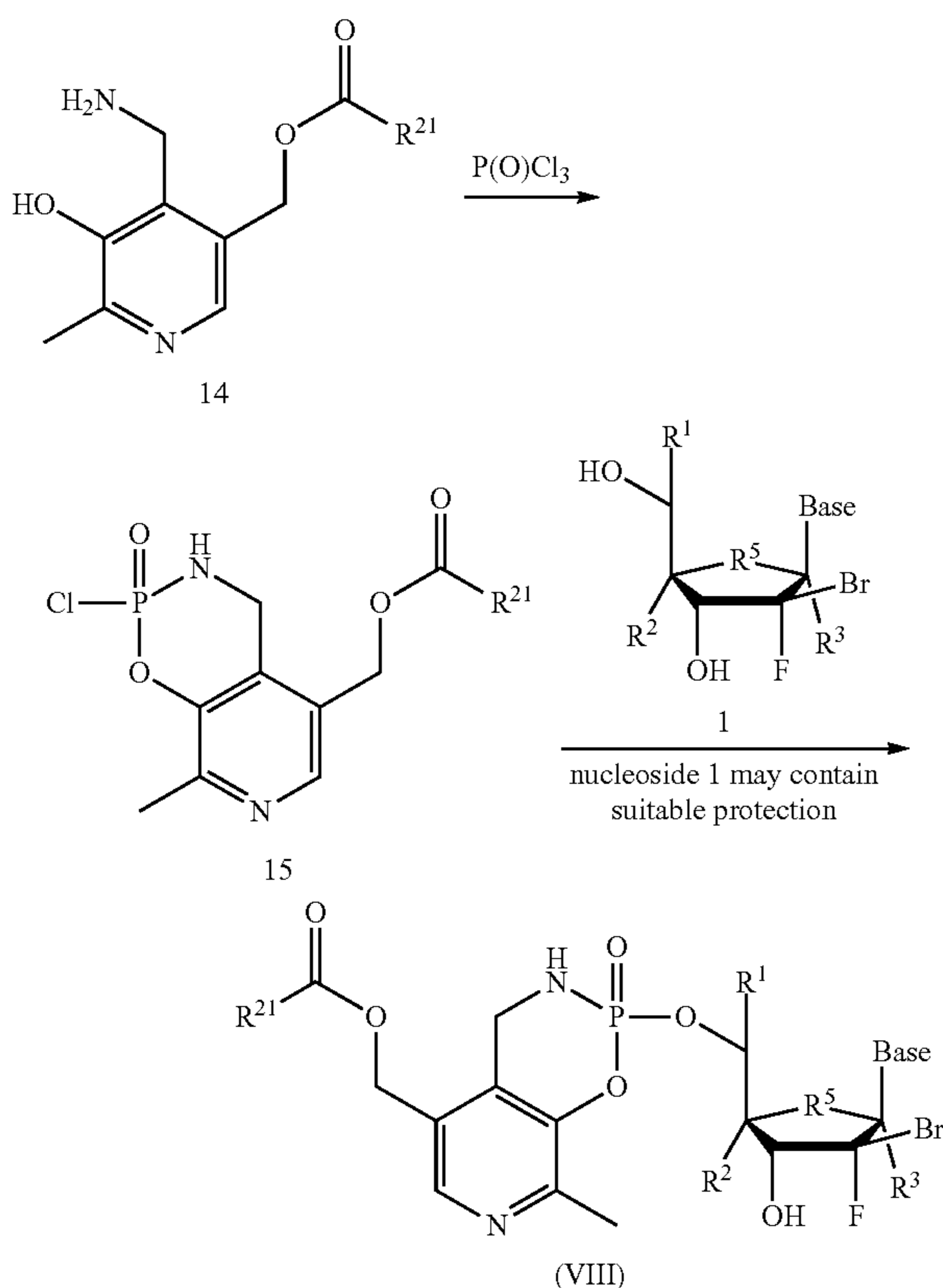
Scheme 35 A synthetic approach to monophosphate prodrugs VIII. (Base, R 1 , R 2 , R 3 , R 5 , and R 21 are as defined in active compound section).
