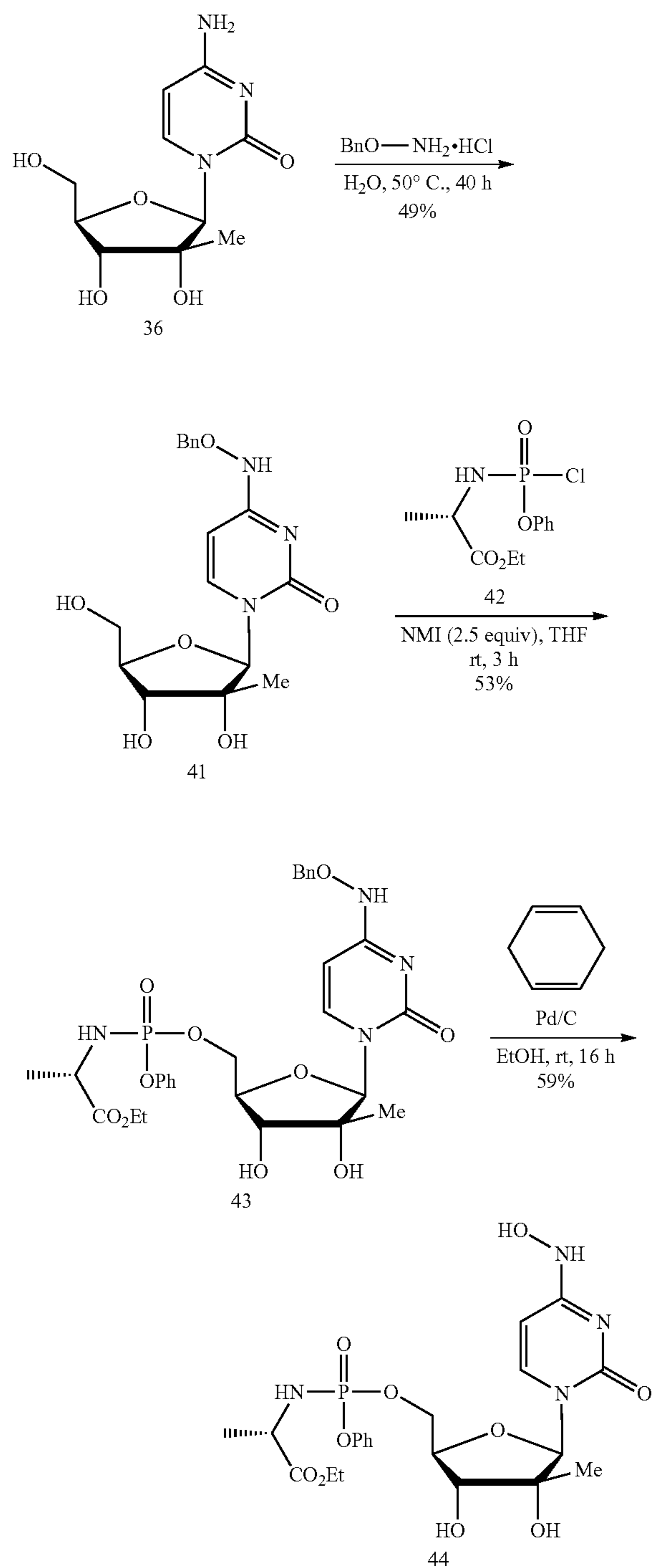
Scheme 17. Synthesis of N 4 -hydroxycytidine 2'-C-Me nucleoside prodrug 44
