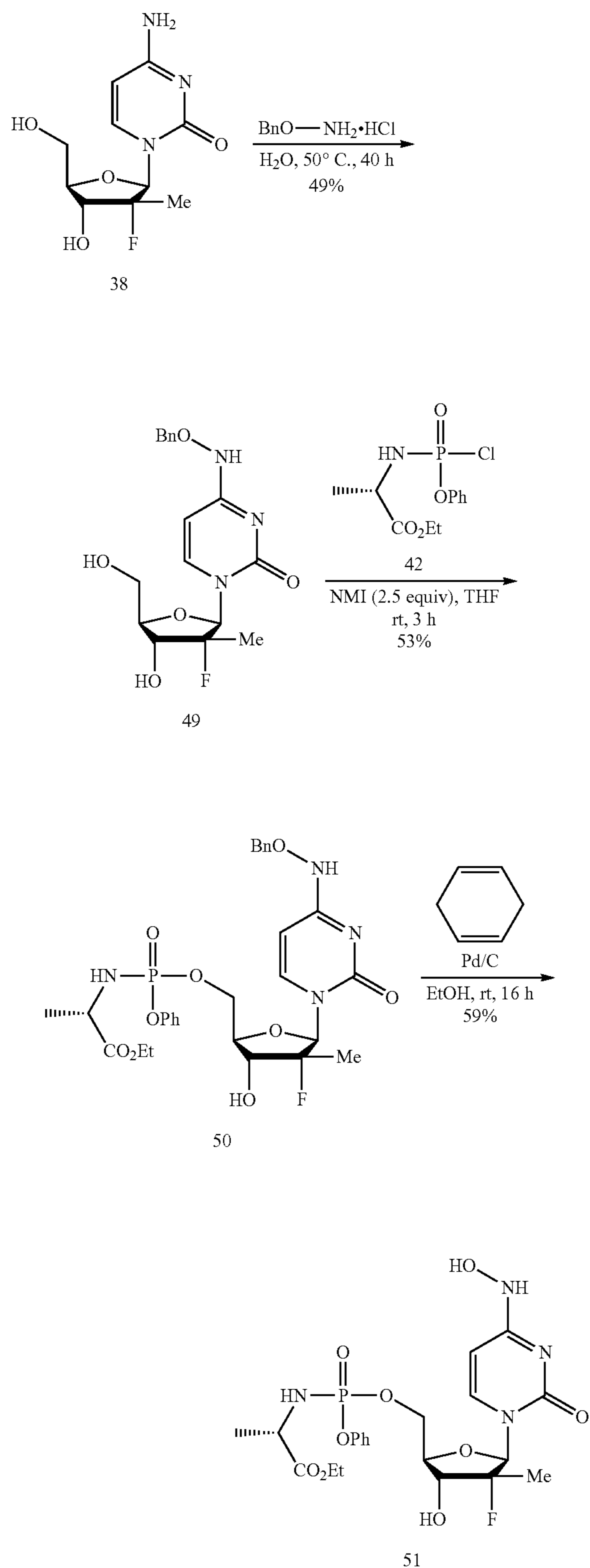
Scheme 19. Synthesis of N 4 -hydroxycytidine 2'-deoxy-2'- \alpha -fluoro-2'- \beta -C-Me nucleoside prodrug 51
