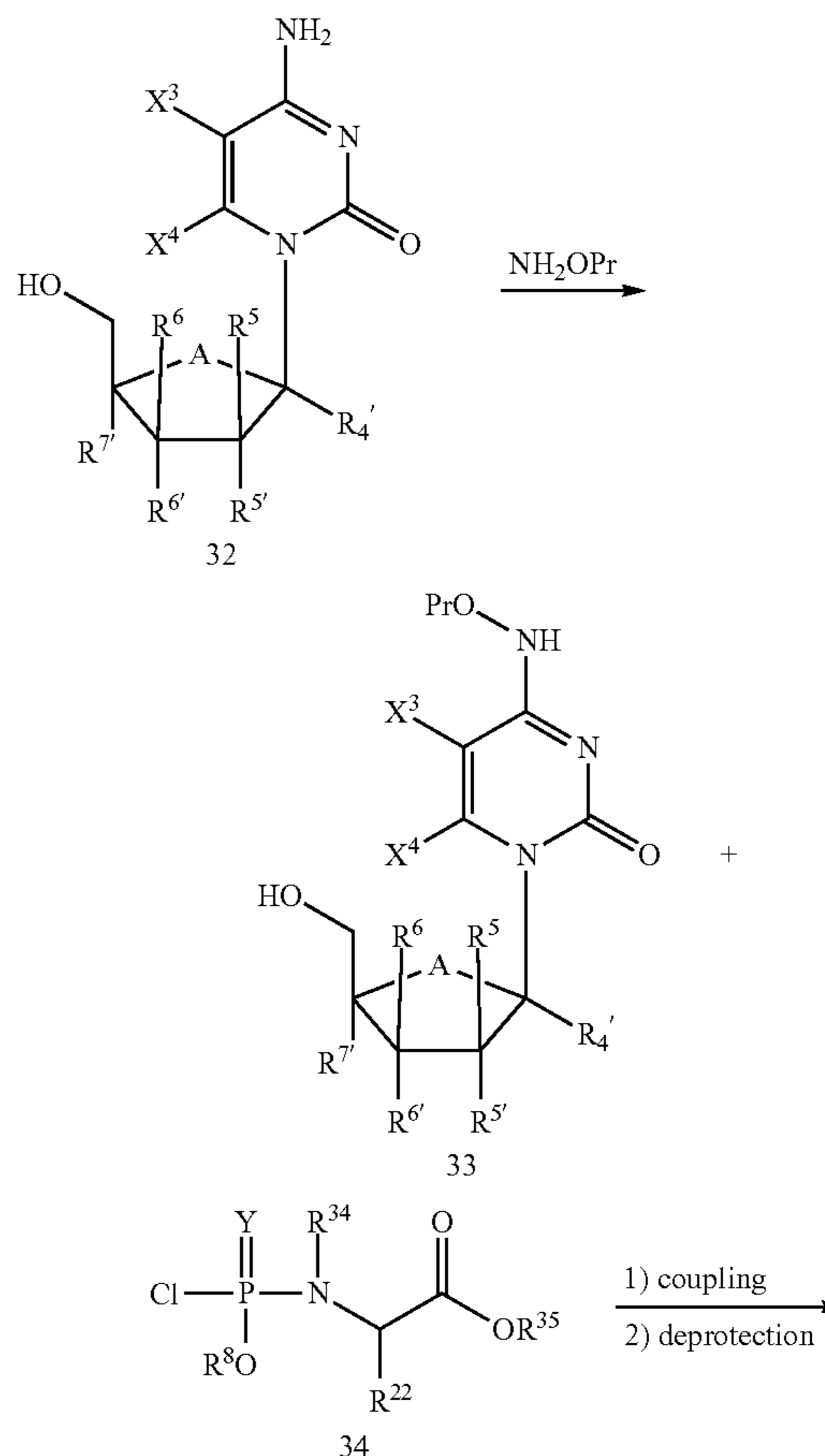
Scheme 13 Approach to monophosphate prodrug 35. ( X^3 , X^4 , Y , R^4 , R^5 , R^6 , Y , R^34 , R^35 , R^22 , and R^7 are as defined in active compound section)
