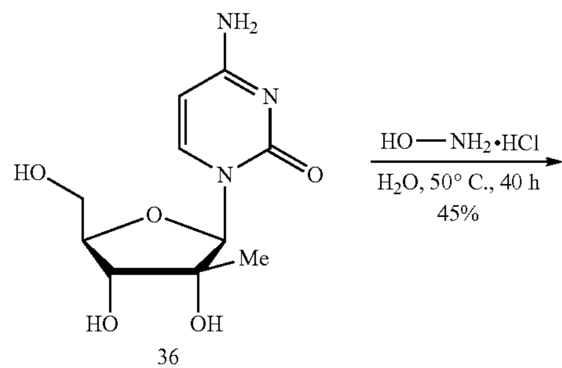
Scheme 14. Synthesis of N 4 -hydroxycytidine 2'-C-Me nucleoside 37
