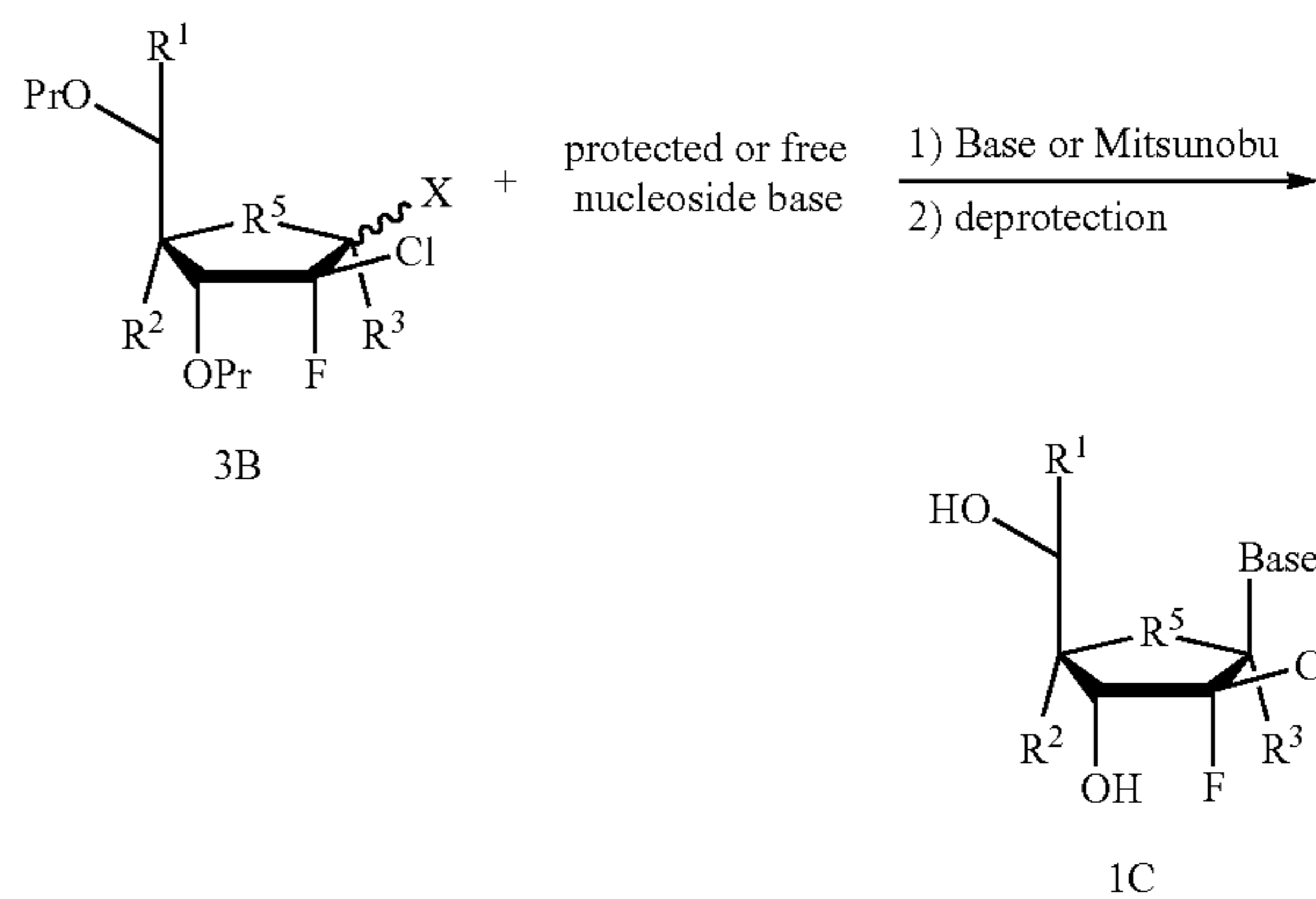
Scheme 22 An alternate synthetic approach to nucleosides 1C. (Base is defined in active compound section)
