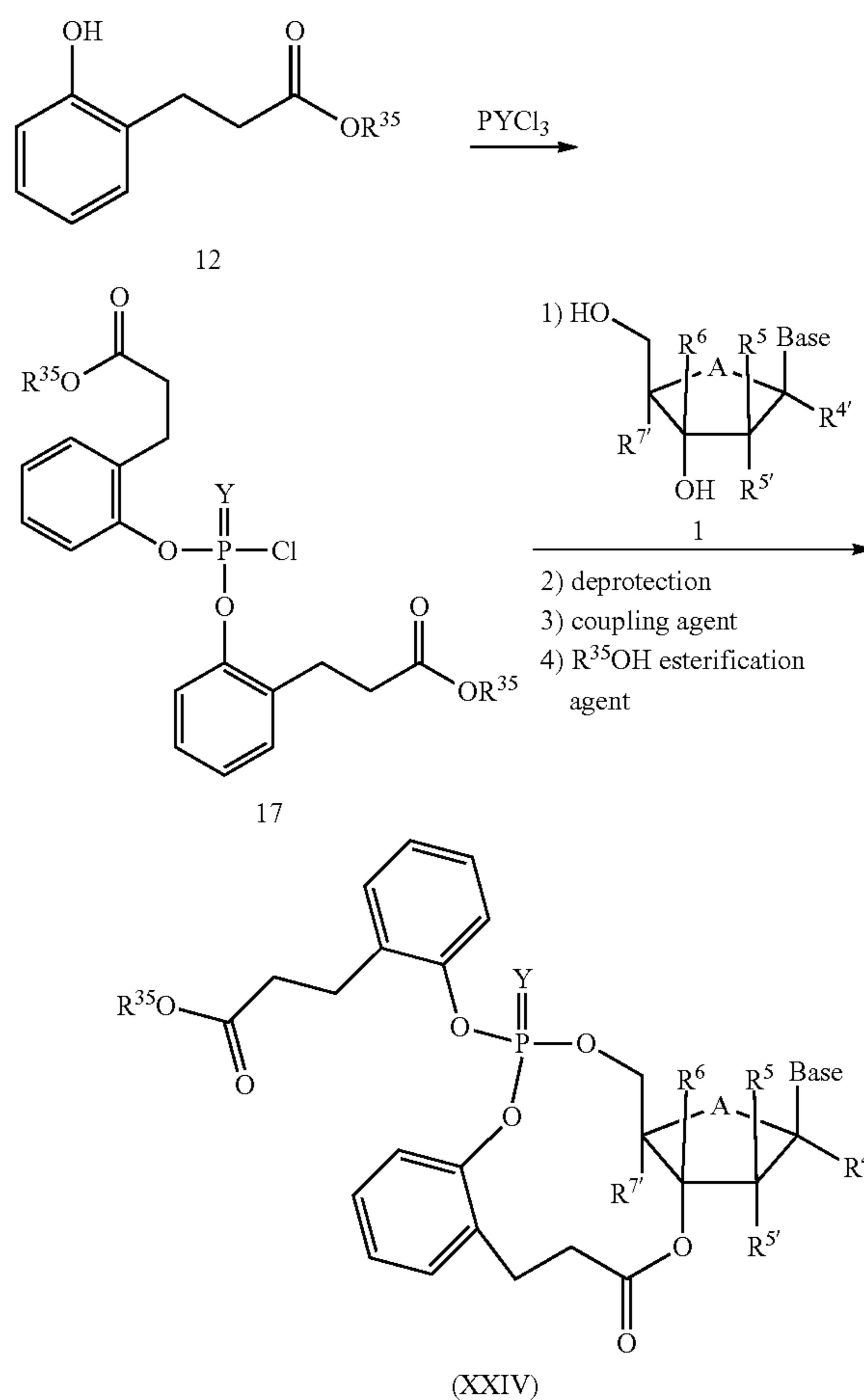
Scheme 4 A synthetic approach to monophosphate prodrug XXIV. (Base is a natural or unnatural nucleoside base; R 4' , R 5 , R 5' , R 6 , Y, R 35 , and R 7' are as defined in active compound section)
