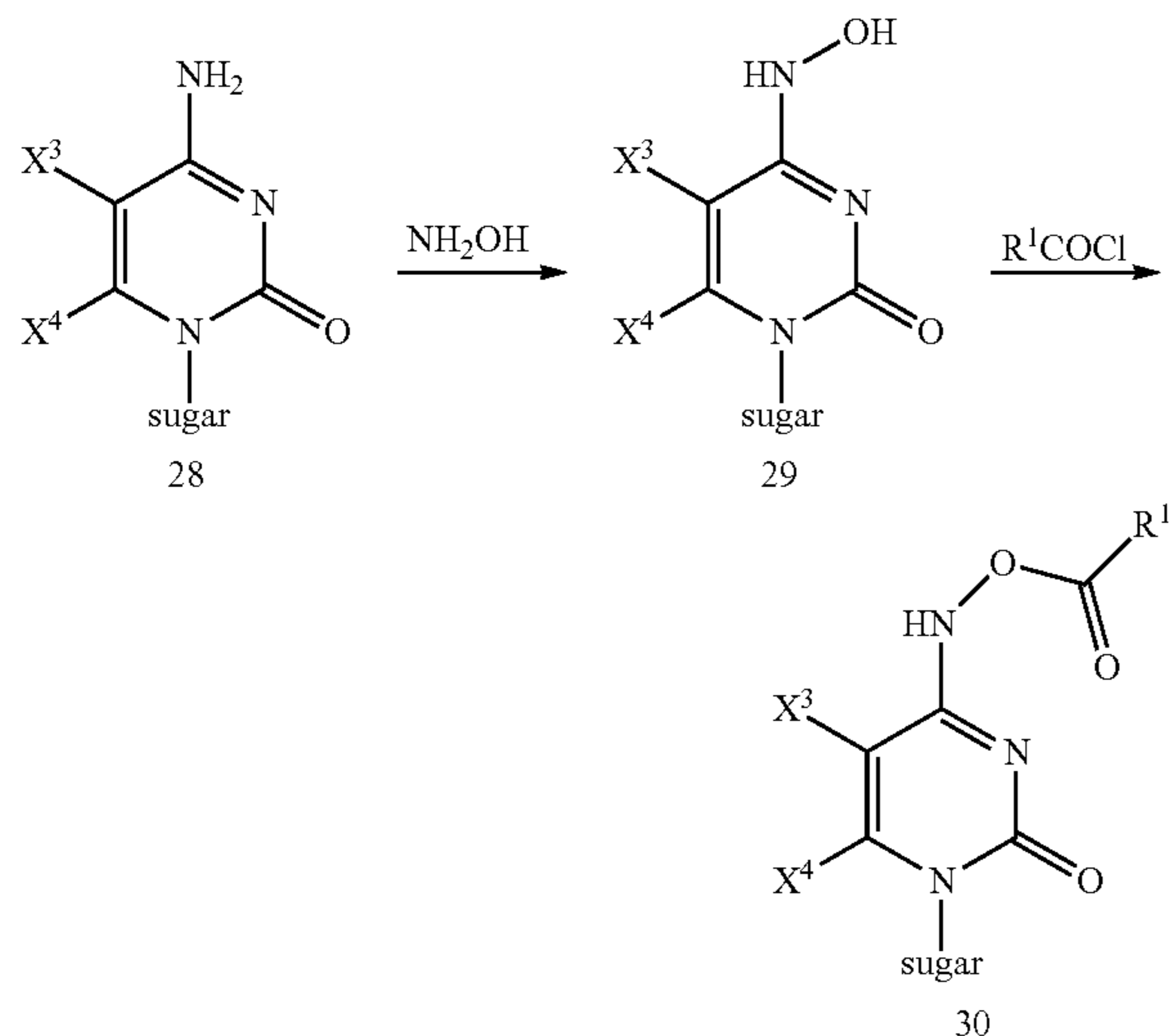
Scheme 11 Synthetic approach to nucleosides 29 and 30. ( X^3 , X^4 , R^1 and sugar are as defined in active compound section)
