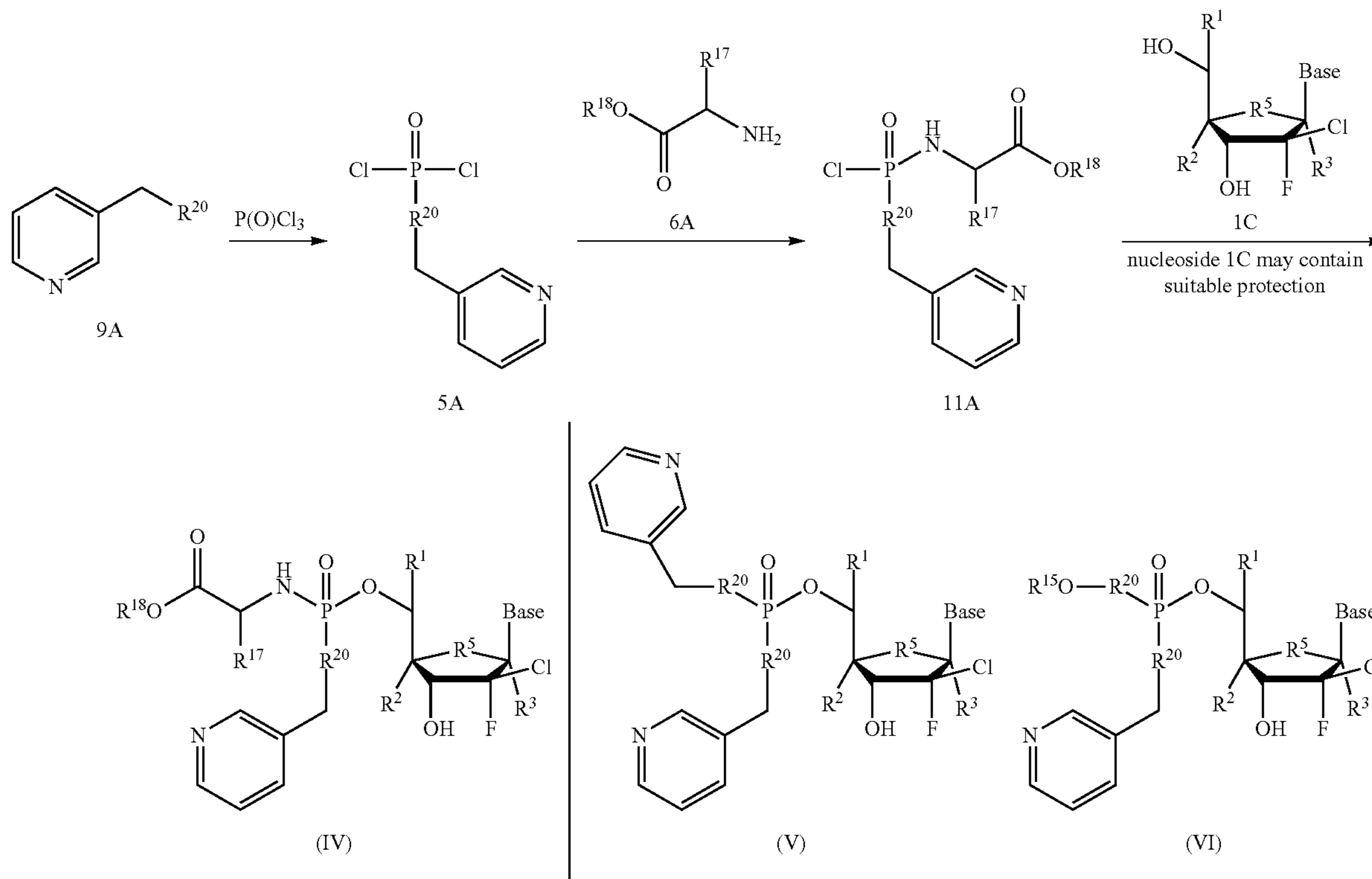
Scheme 24 A synthetic approach to monophosphate prodrugs IV-VI. (Base, R 1 , R 2 , R 3 , R 5 , R 16 , R 17 , and R 18 are as defined in active compound section).
