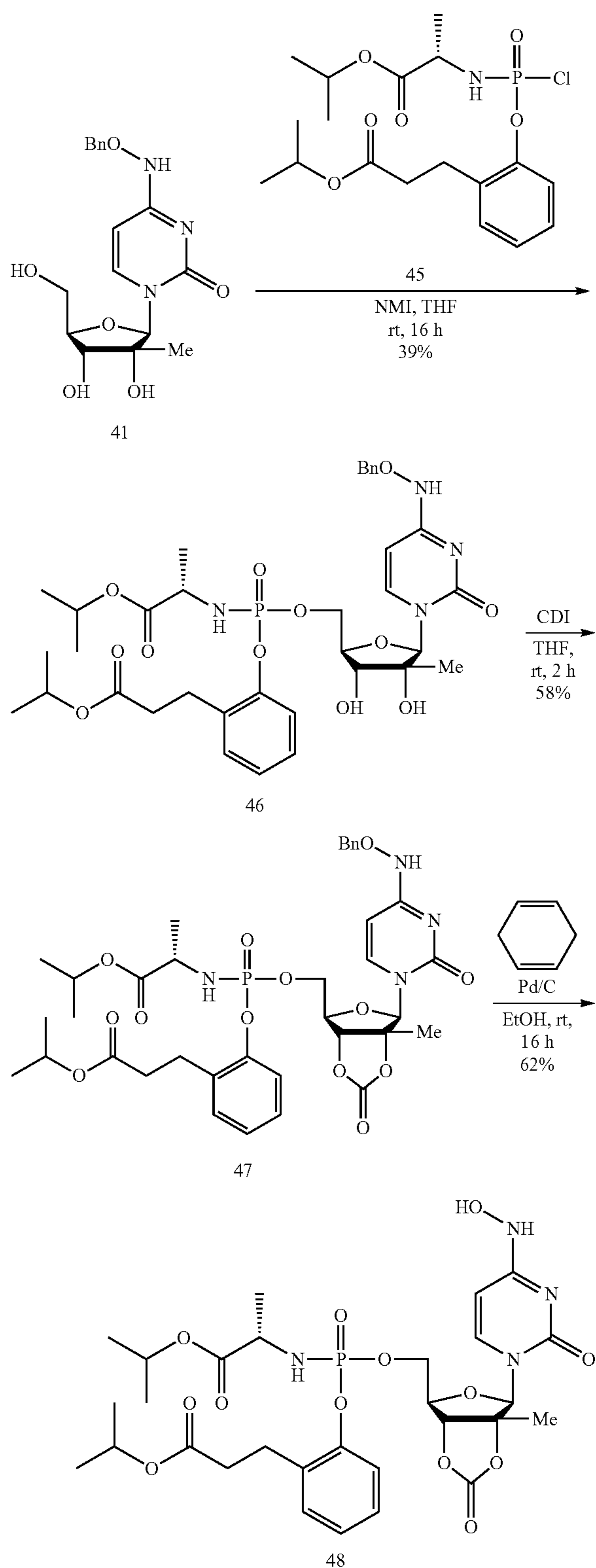
Scheme 18. Synthesis of N 4 -hydroxycytidine 2'-C-Me nucleoside prodrug 48
