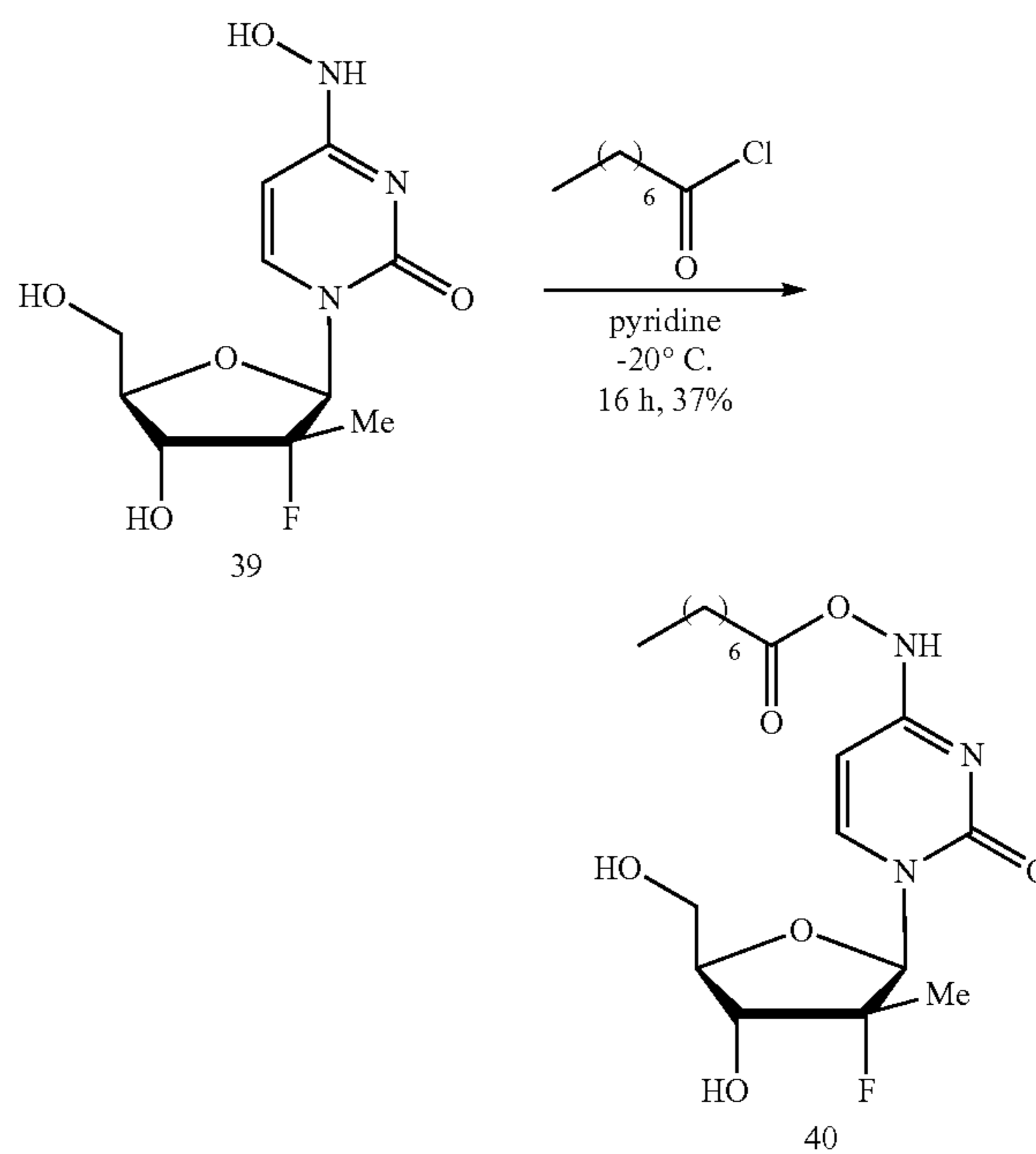
Scheme 16. Synthesis of N 4 -(Octanoloxy)cytidine 2'-deoxy-2'-alpha-fluoro-2'-beta-C-Me nucleoside 40
