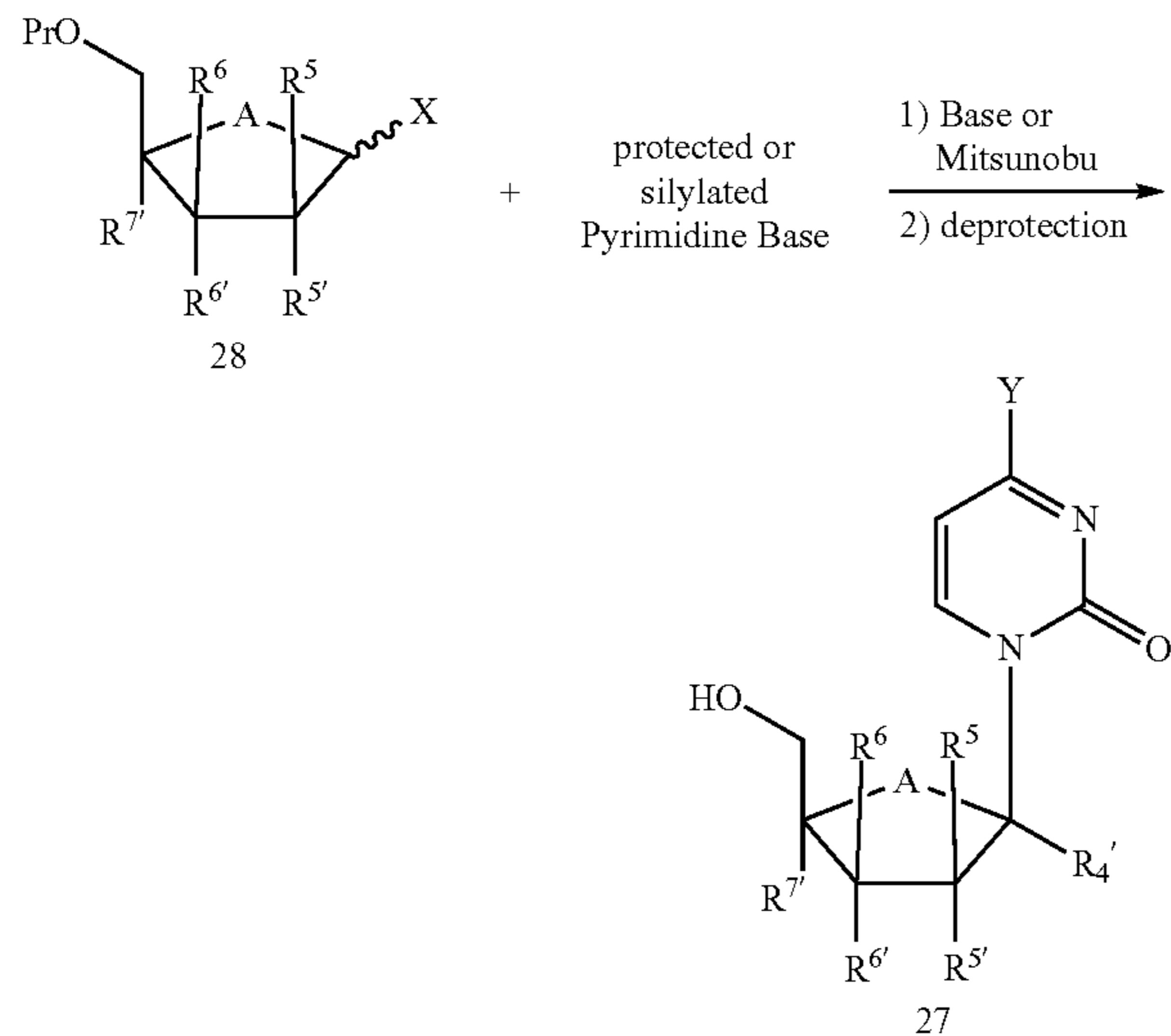
Scheme 10 An alternate synthetic approach to nucleosides 27. ( R^4 , R^5 , R^6 , R^7 , Y , R^6' and R^5' are as defined in active compound section)
