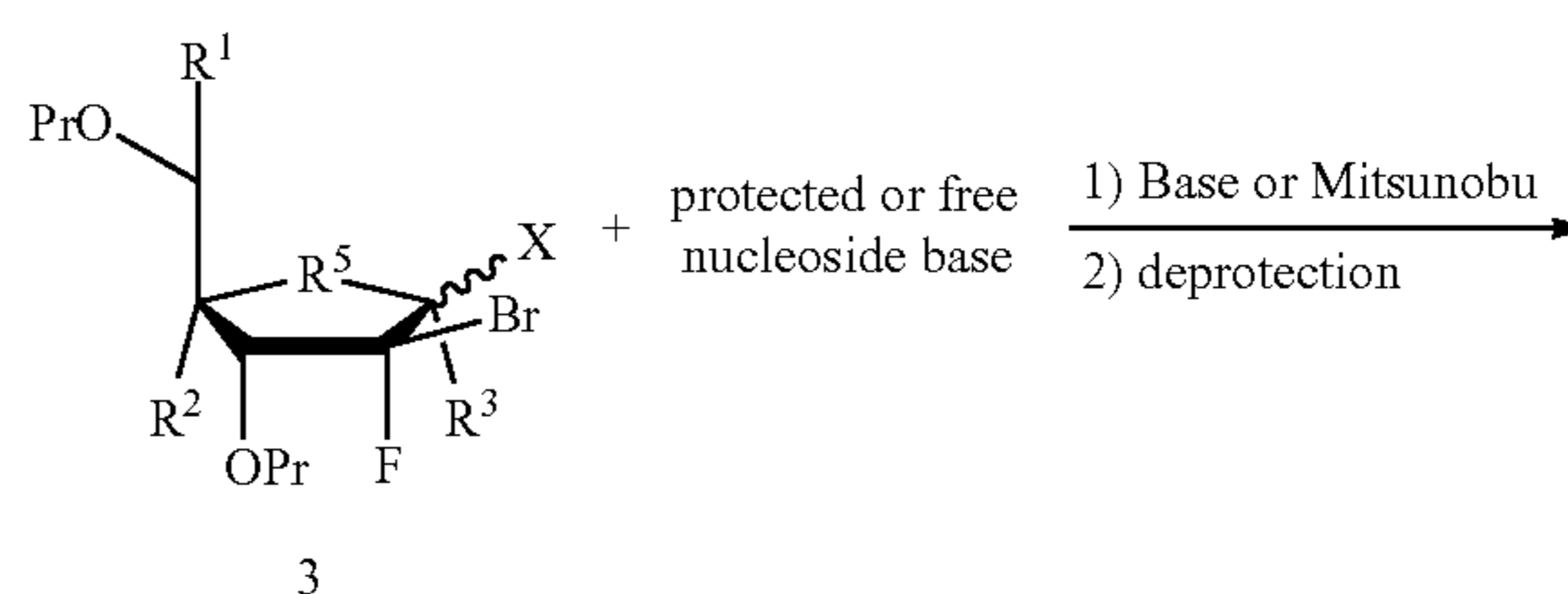
Scheme 31 An alternate synthetic approach to nucleosides 1. (Base are as defined in active compound section)
