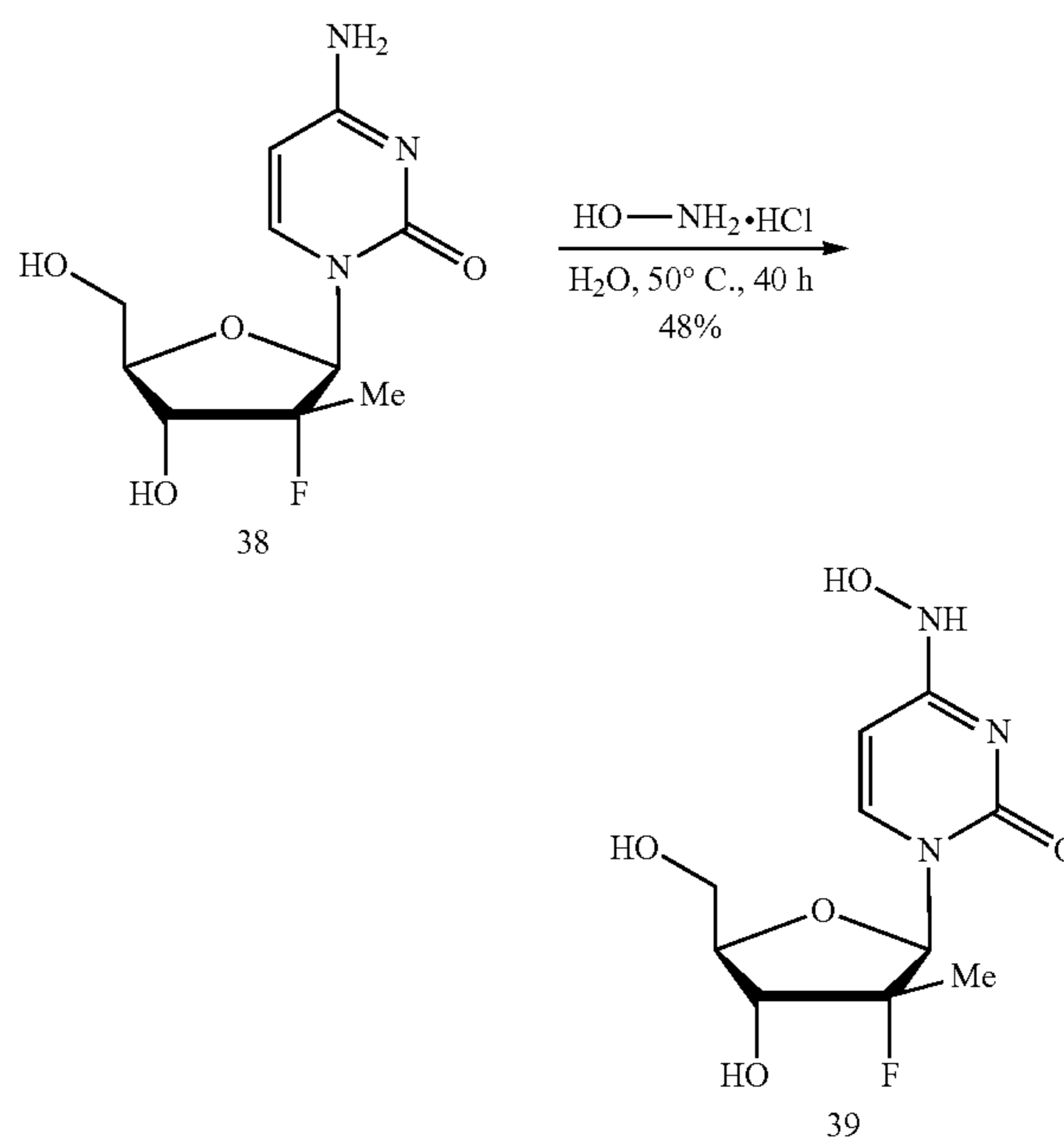
Scheme 15. Synthesis of N 4 -hydroxycytidine 2'-deoxy-2'-alpha-fluoro-2'-beta-C-Me nucleoside 39
