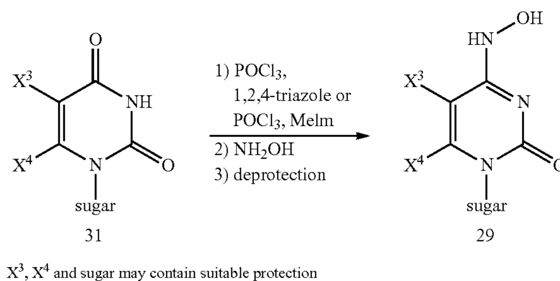
Scheme 12 An alternate synthetic approach to nucleosides 29. ( X^3 , X^4 , R^1 and sugar are as defined in active compound section)
