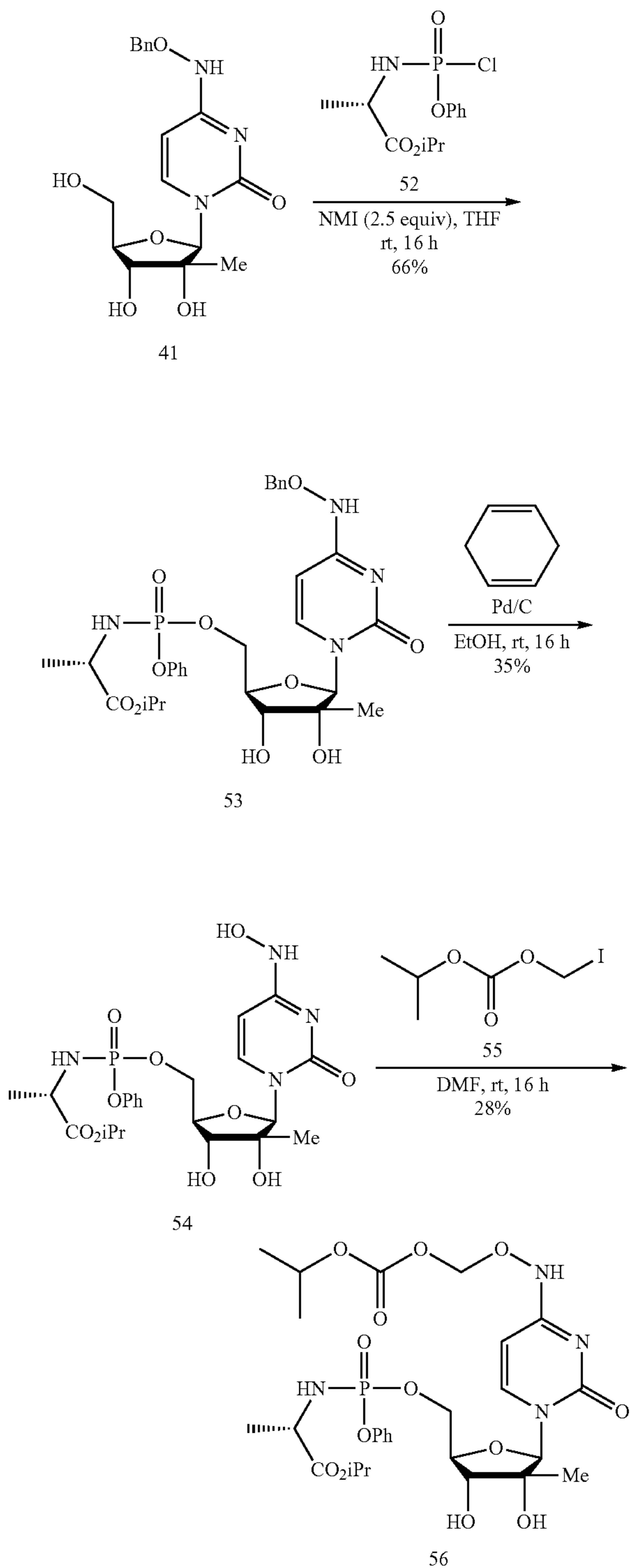
Scheme 20. Synthesis of N 4 -hydroxycytidine 2'-C-Me nucleoside prodrugs 54 and 56
