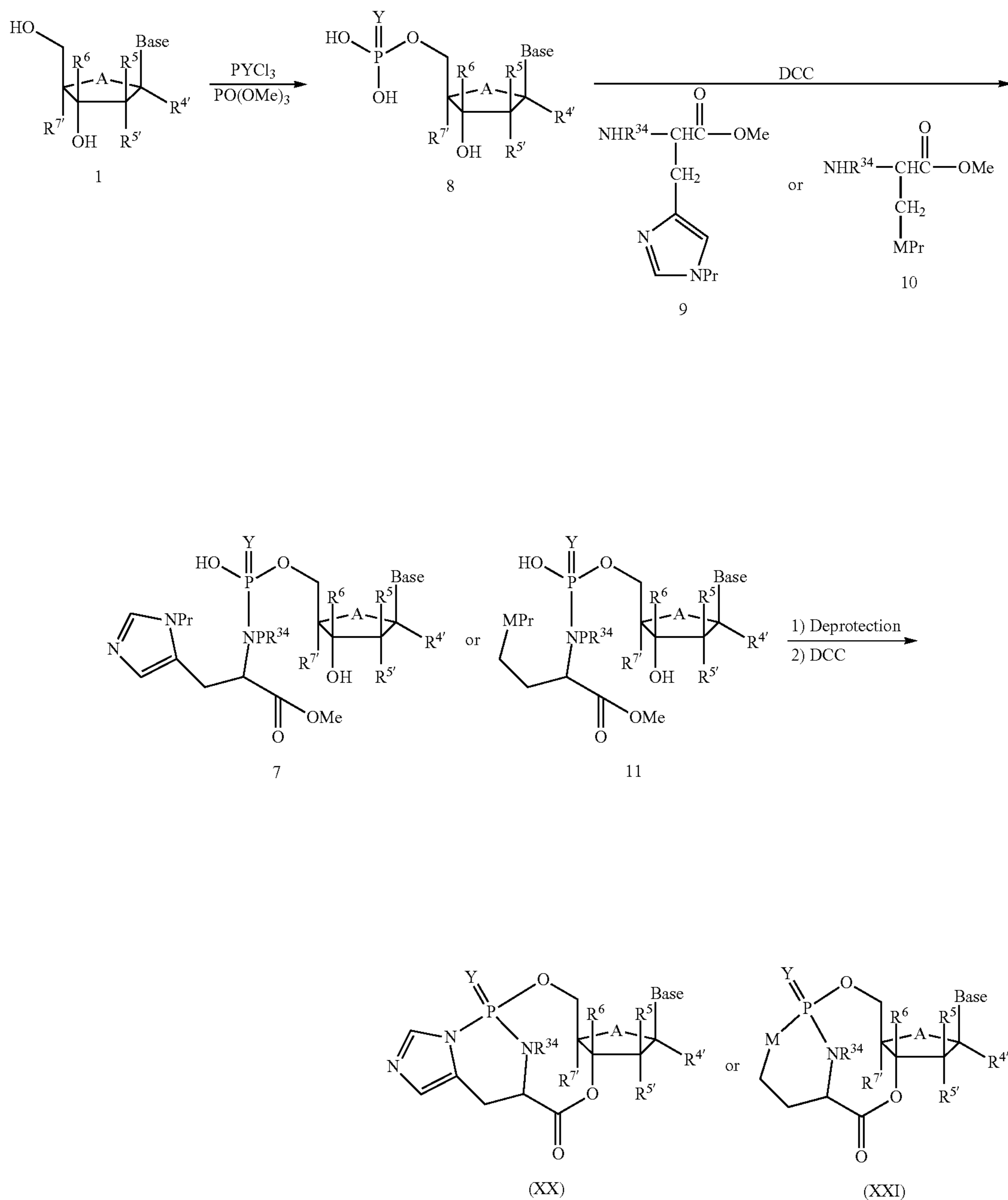
Scheme 2 An alternate synthetic approach to monophosphate prodrugs XX, XXI, XXII. (Base is a natural or unnatural nucleoside base; R 4' , R 5' , R 6' , Y, M, R 34 , and R 7' are as defined in active compound section)
