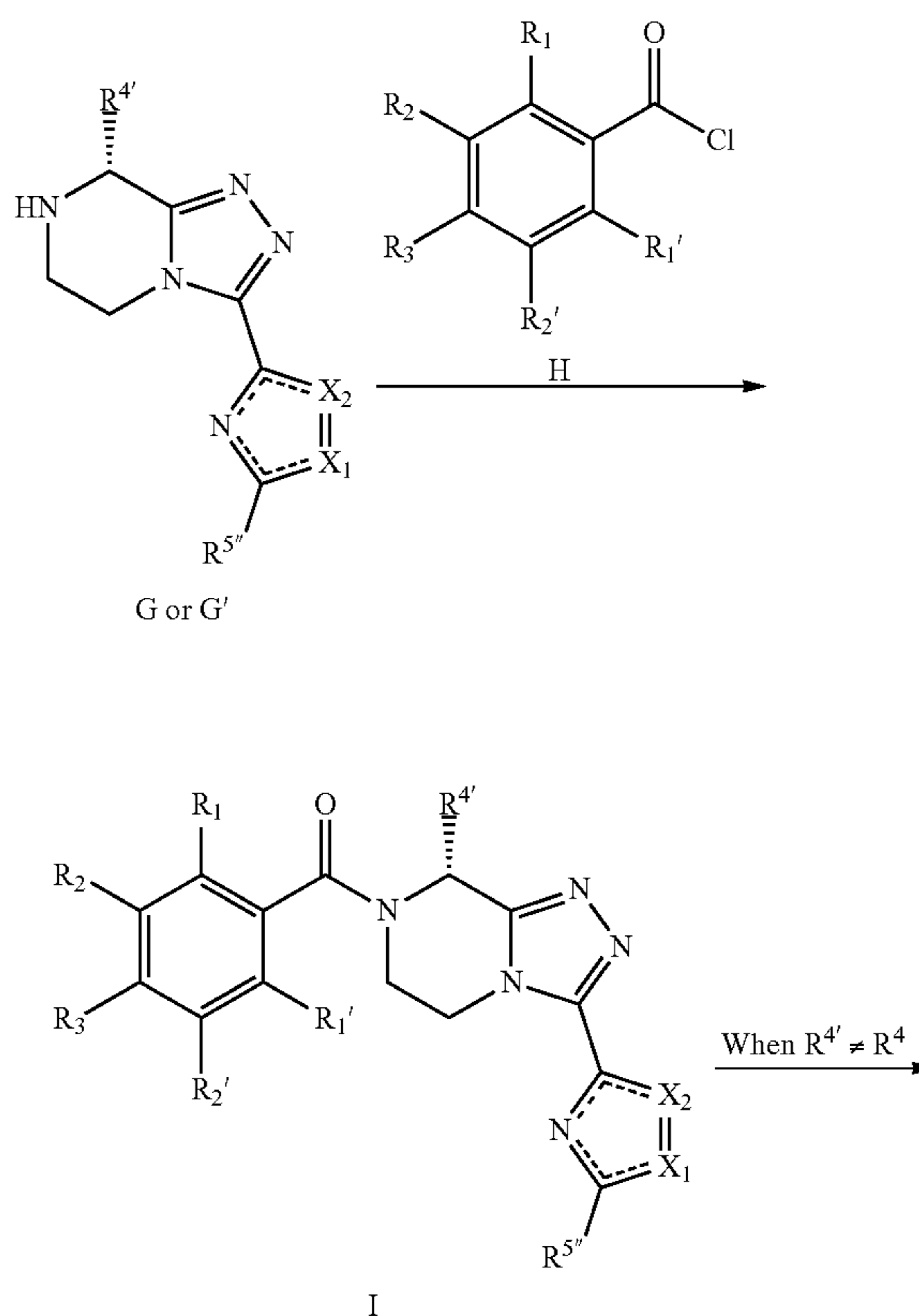
Scheme 16 Acylation.
