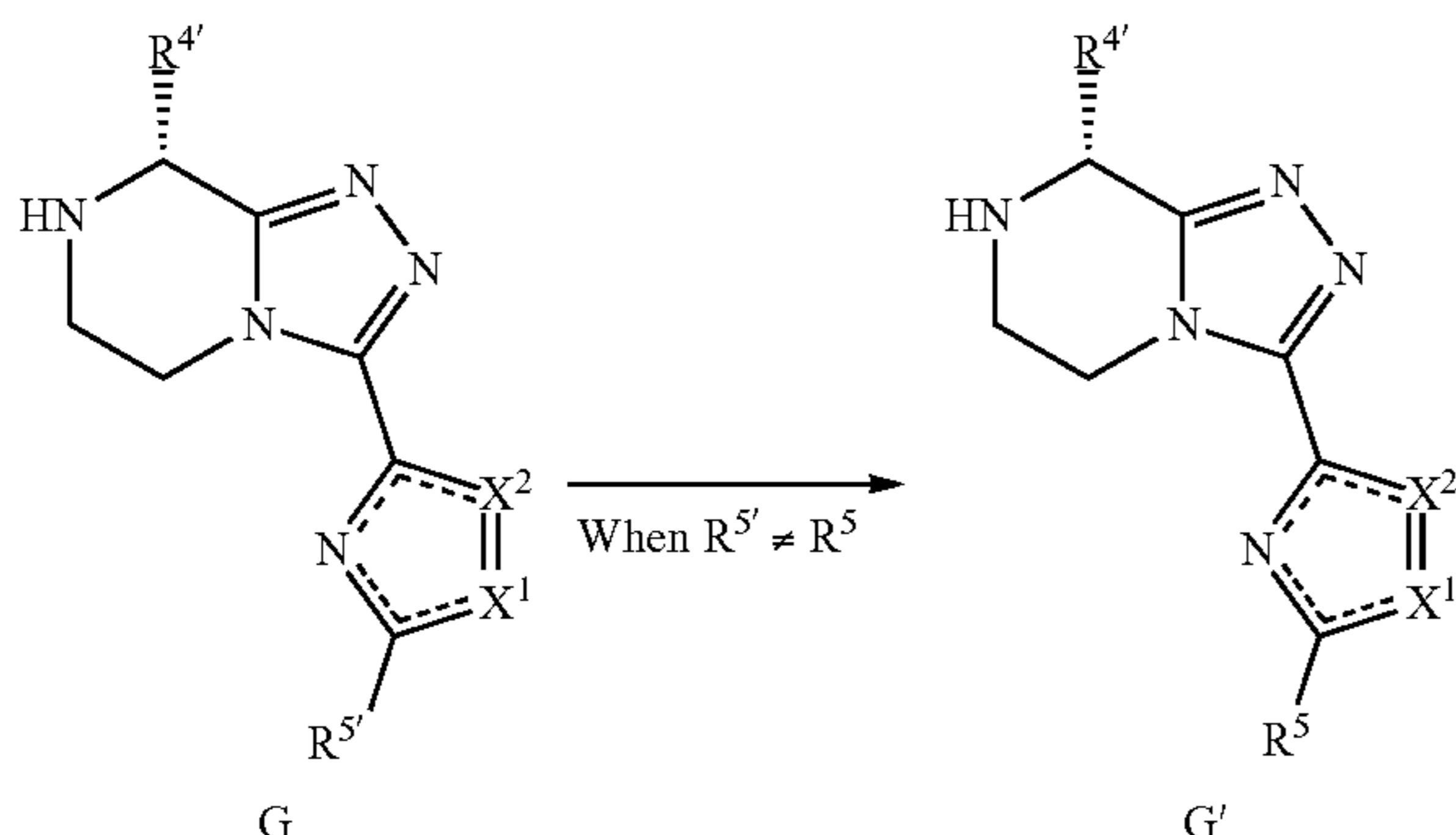
Scheme 15 conversion of R 5' to R 5 in triazolopiperazine G leading to G'.
