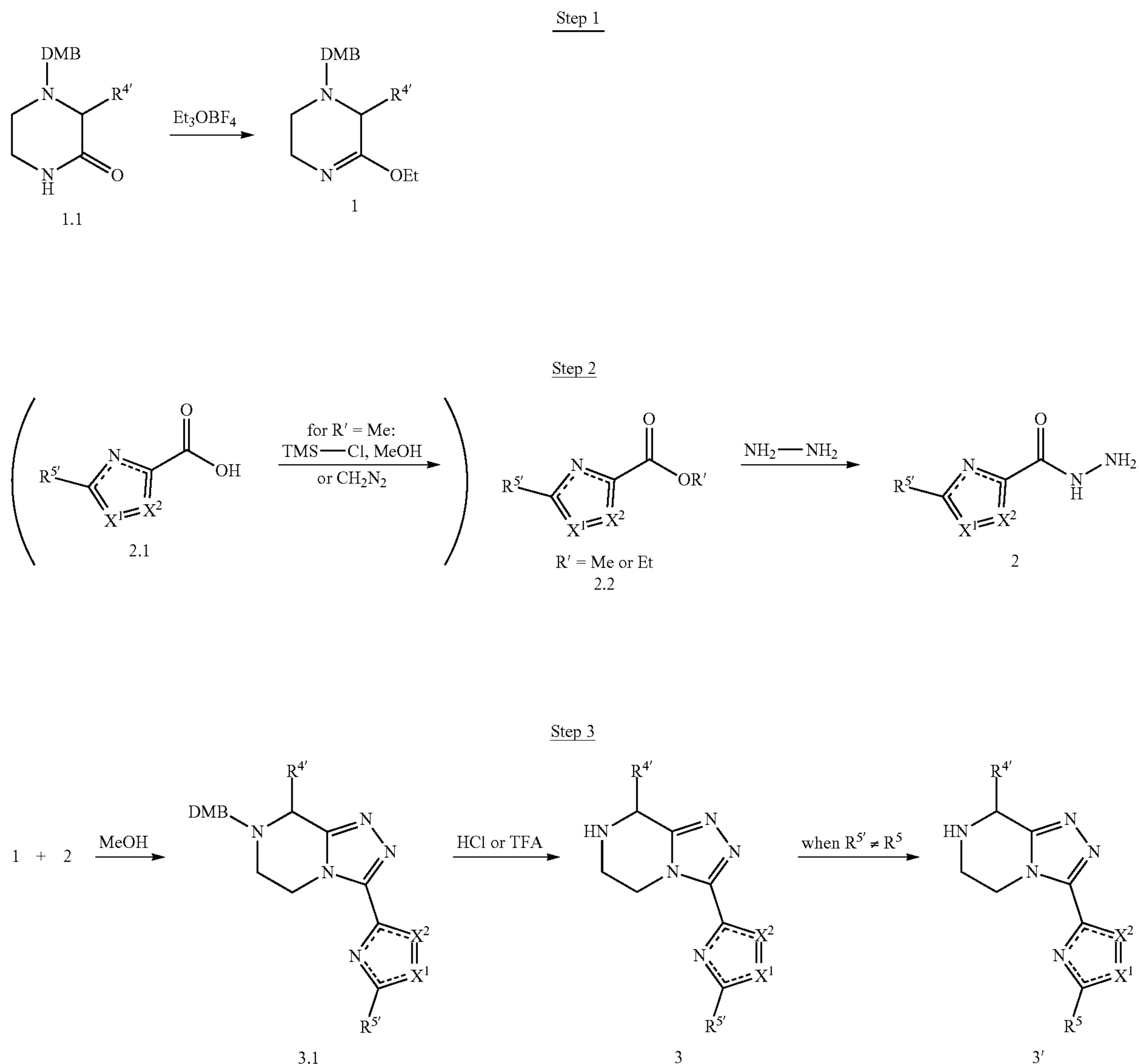
Scheme 1: General racemic synthetic scheme for the preparation of the compounds of the invention.
