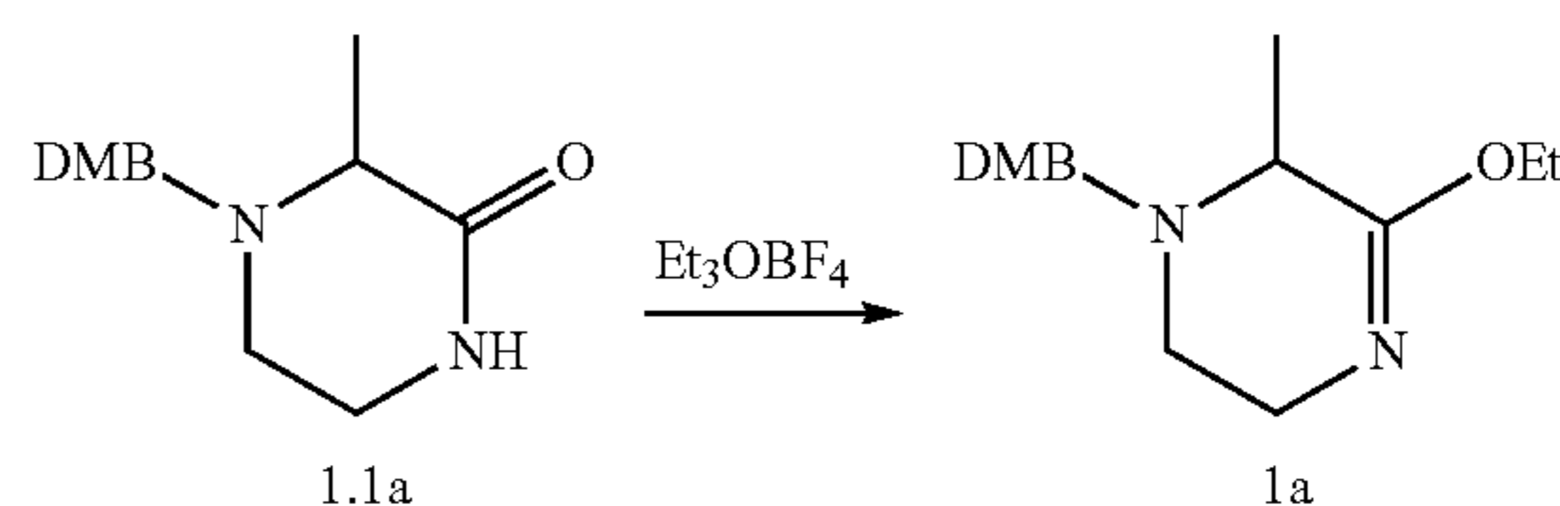
Scheme 3 Synthesis of 1-(2,4-dimethoxybenzyl)-5-ethoxy-6-methyl-1,2,3,6-tetrahydropyrazine 1a.
