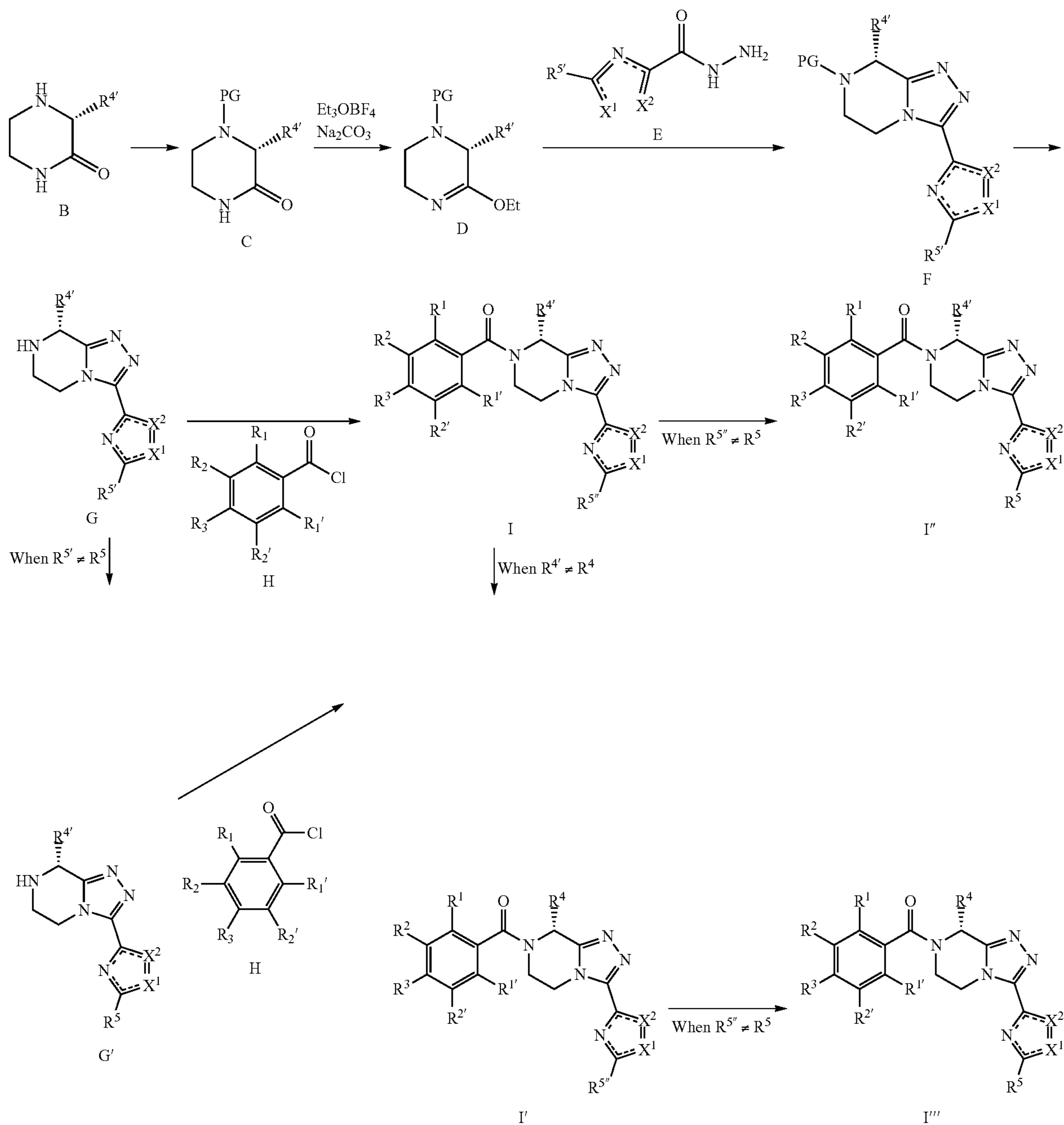
Scheme 7 General synthetic scheme for the preparation of chiral compounds of the invention.
