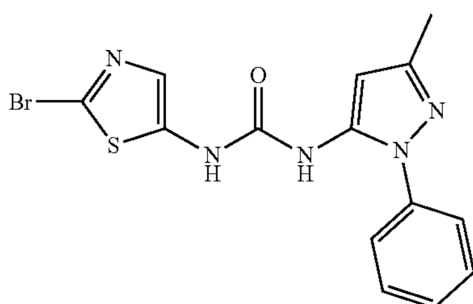
Molecular Weight: 378.25
