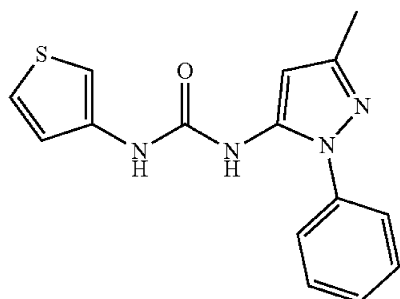
Molecular Weight: 298.36
