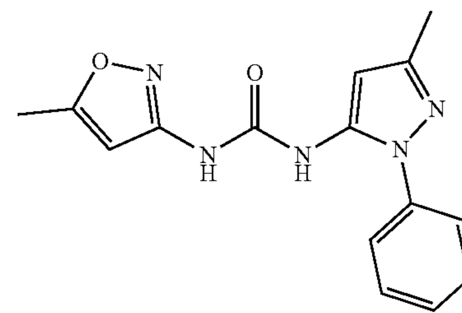
Molecular Weight: 297.32
