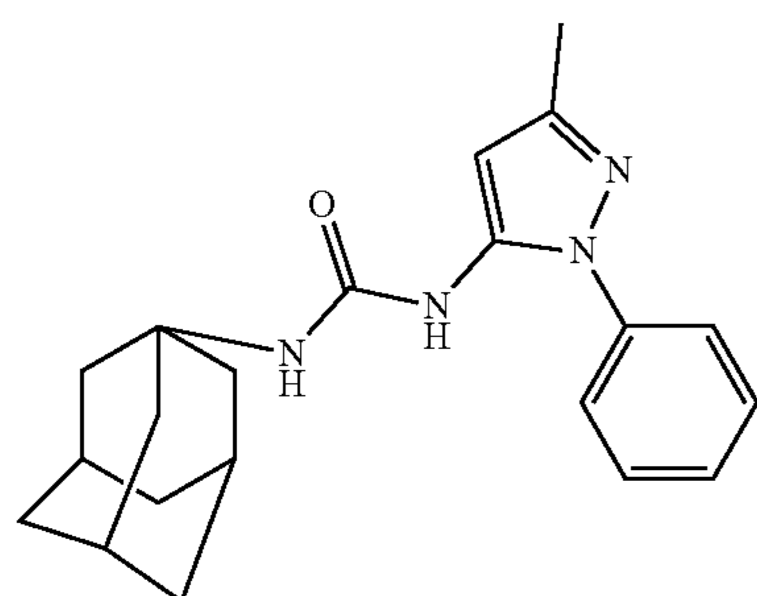
Molecular Weight: 350.47
