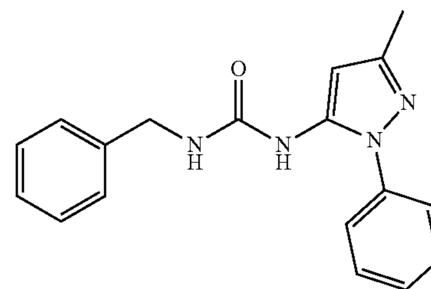
Molecular Weight: 306.37
