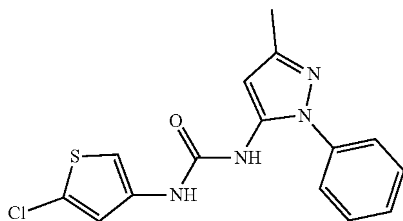
Molecular Weight: 332.81
