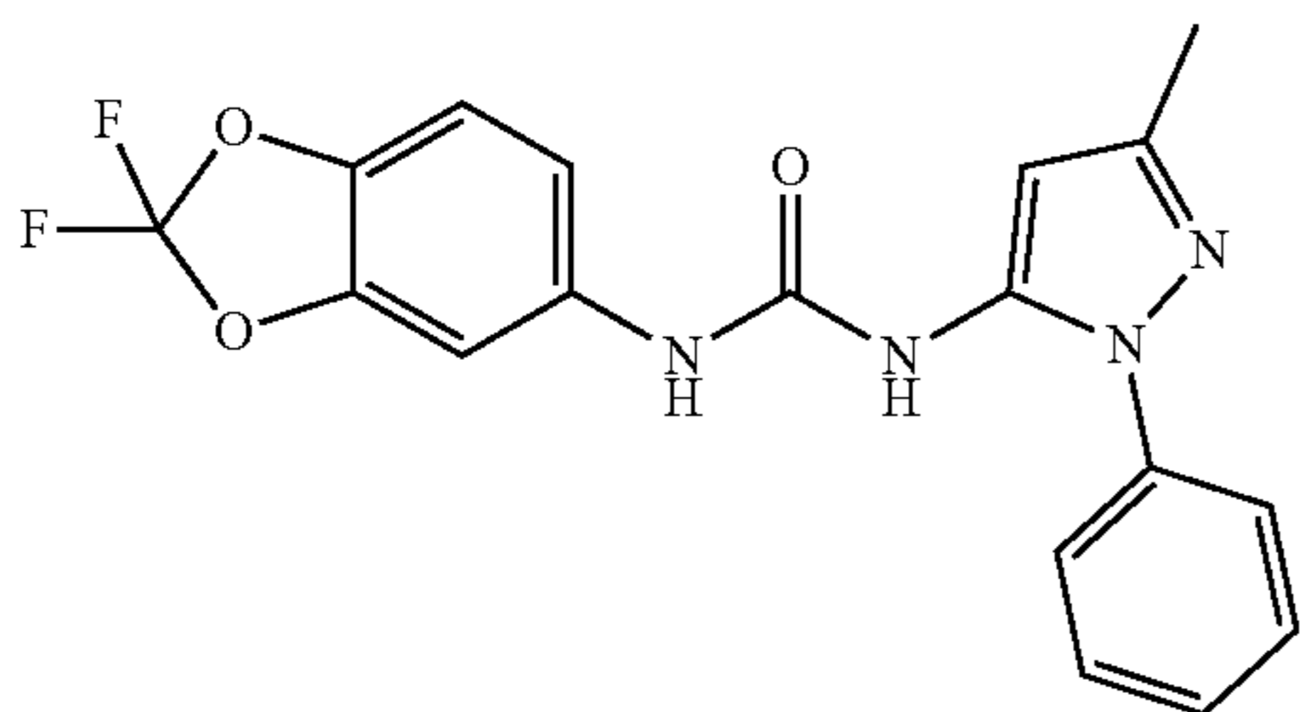
Molecular Weight: 372.33
