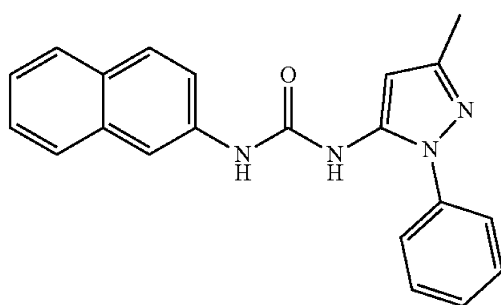
Molecular Weight: 342.40
