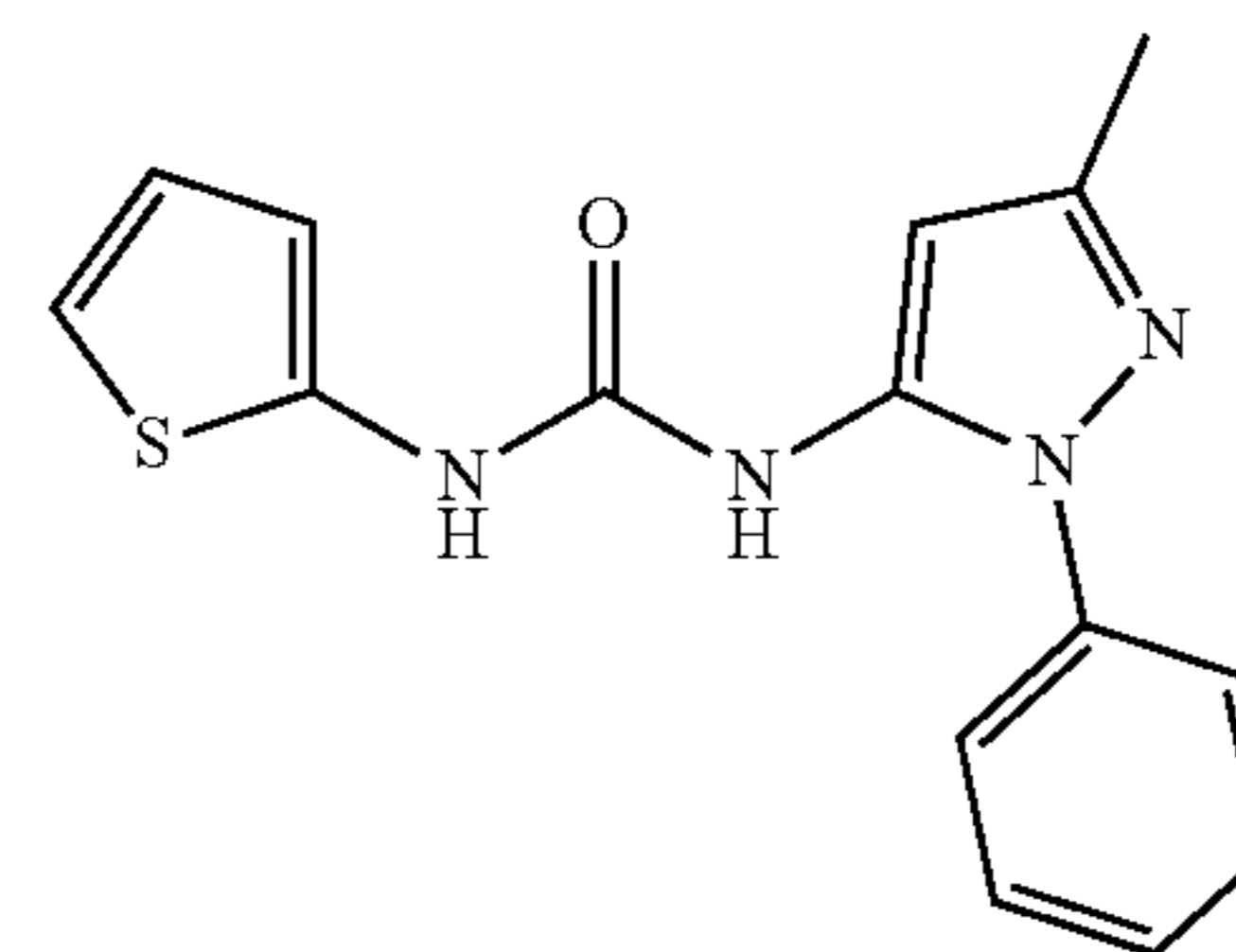
Molecular Weight: 298.36
