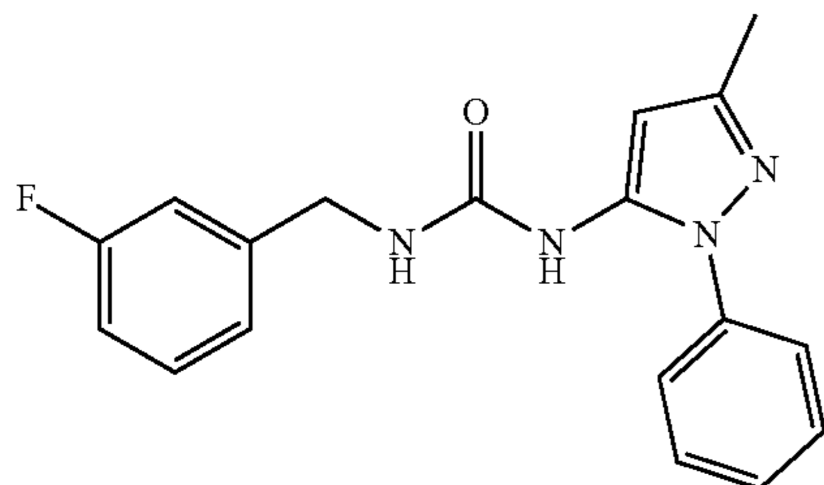
Molecular Weight: 324.36
