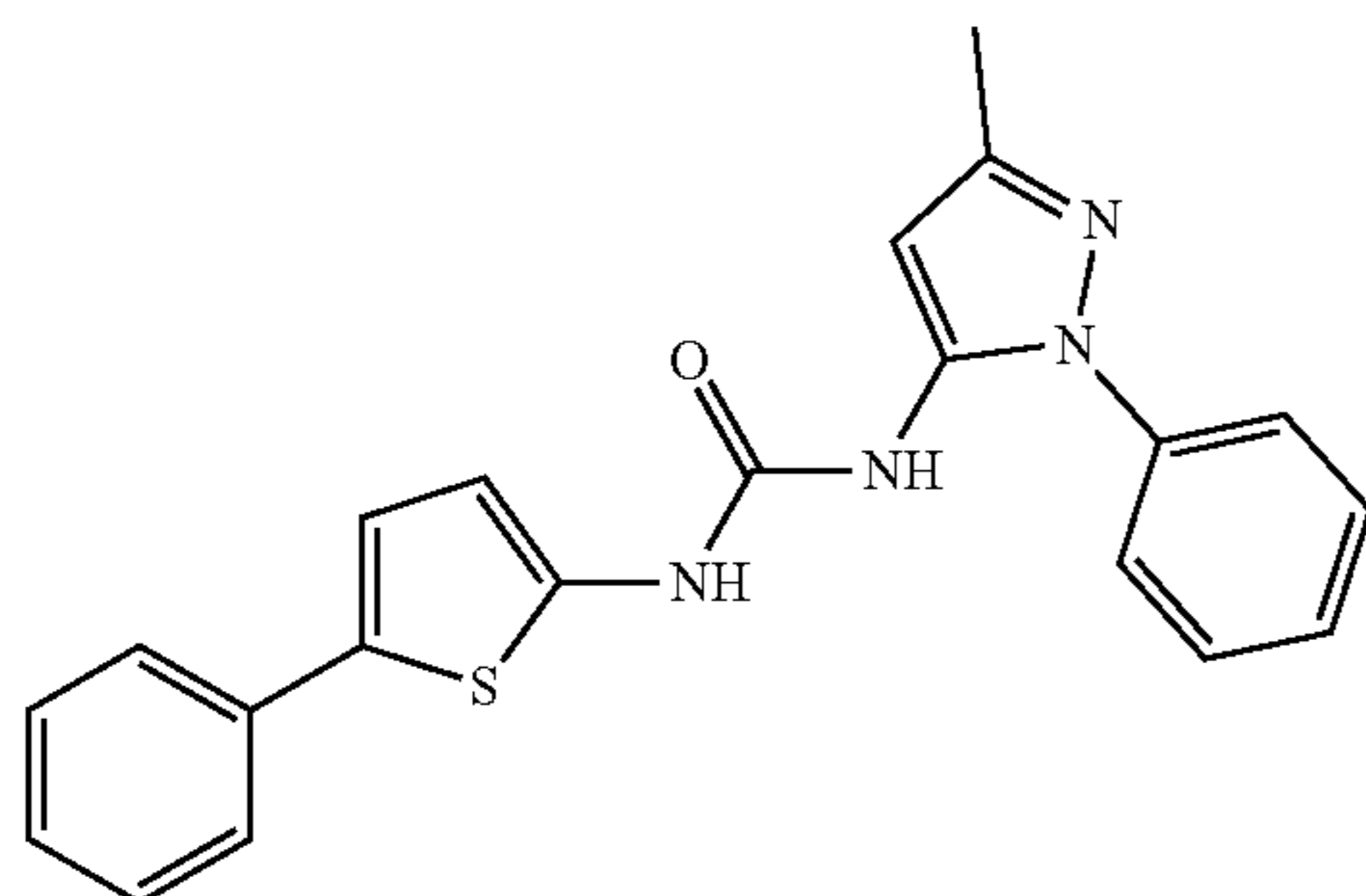
Molecular Weight: 374.46
