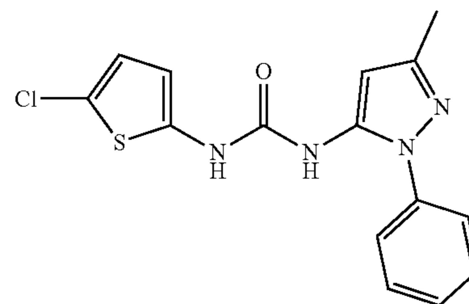
Molecular Weight: 332.81
