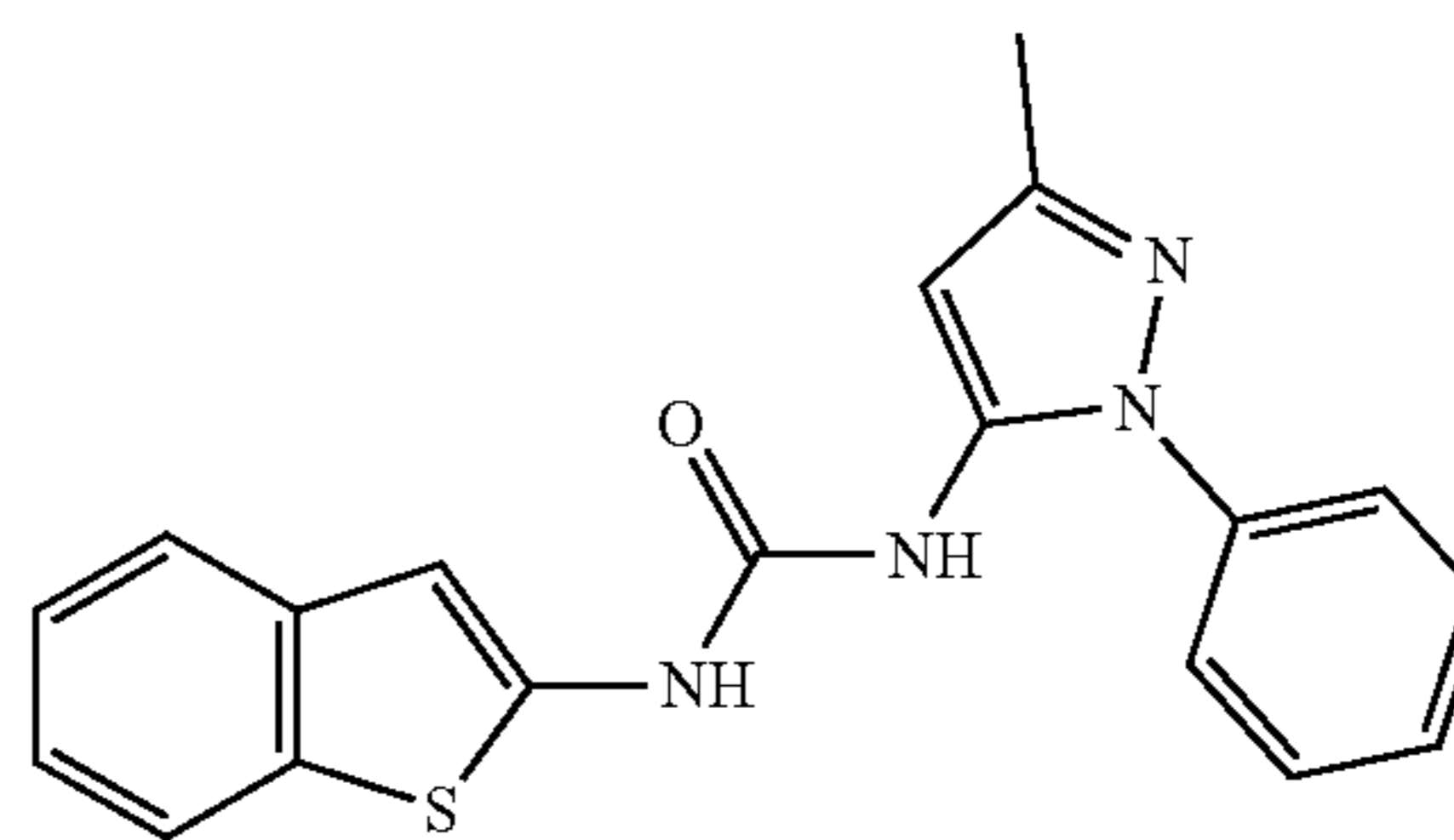
Molecular Weight: 348.42
