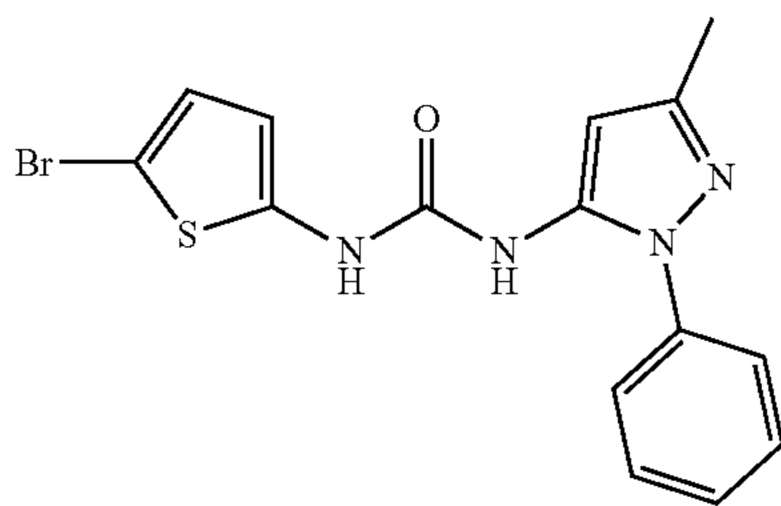
Molecular Weight: 377.26
