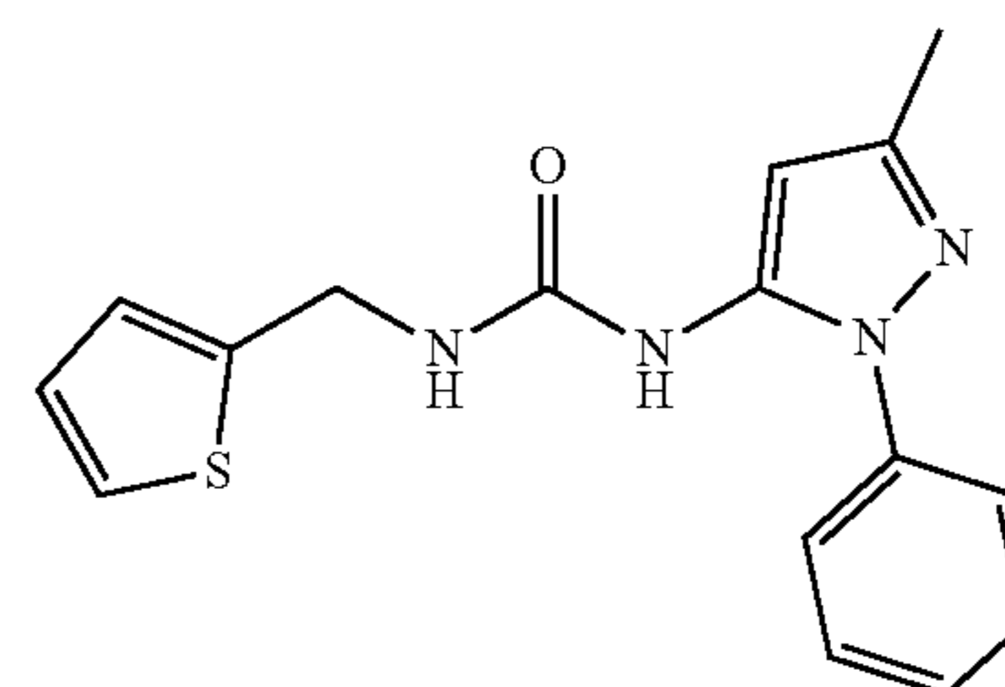
Molecular Weight: 312.39
