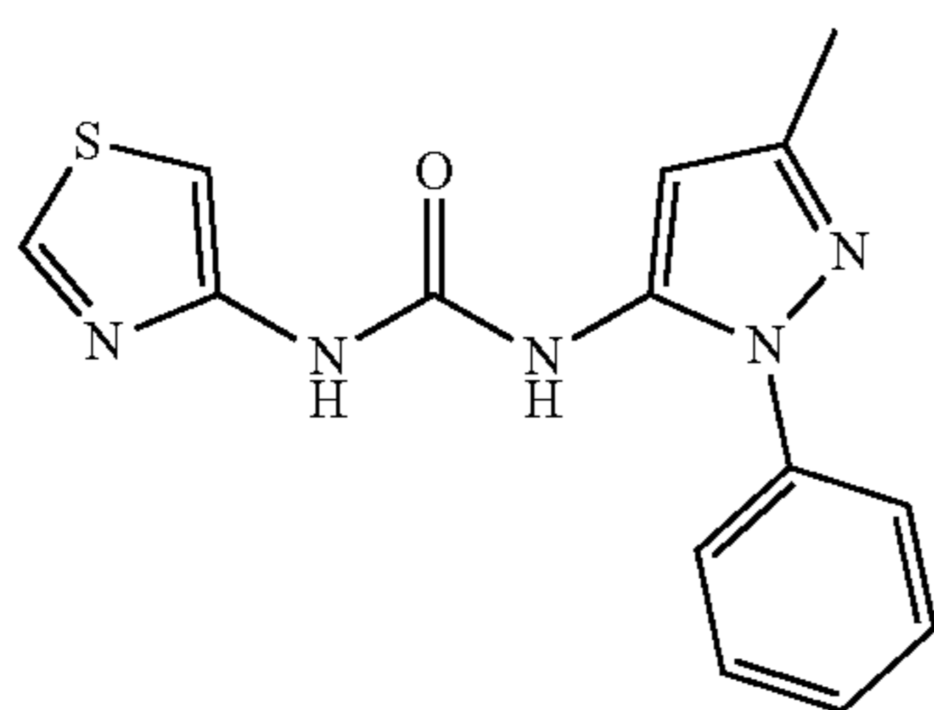
Molecular Weight: 299.35
