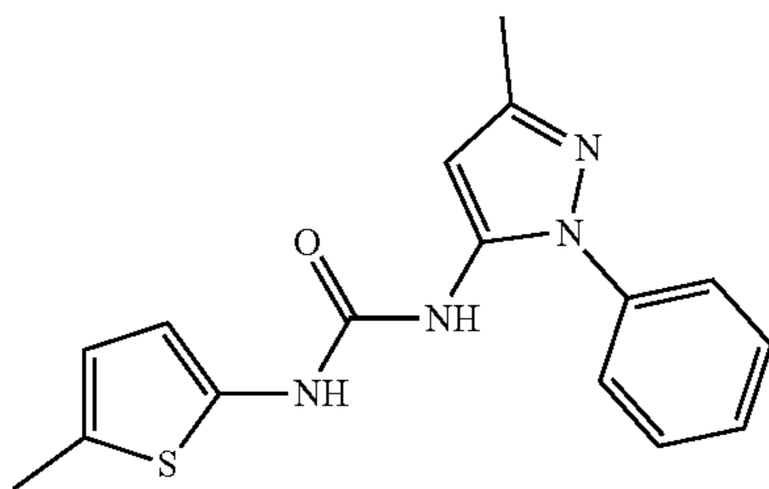
Molecular Weight: 312.39
