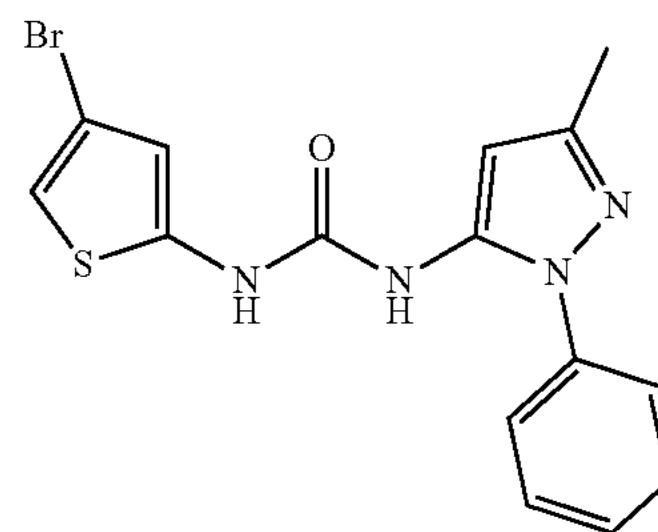
Molecular Weight: 377.26
