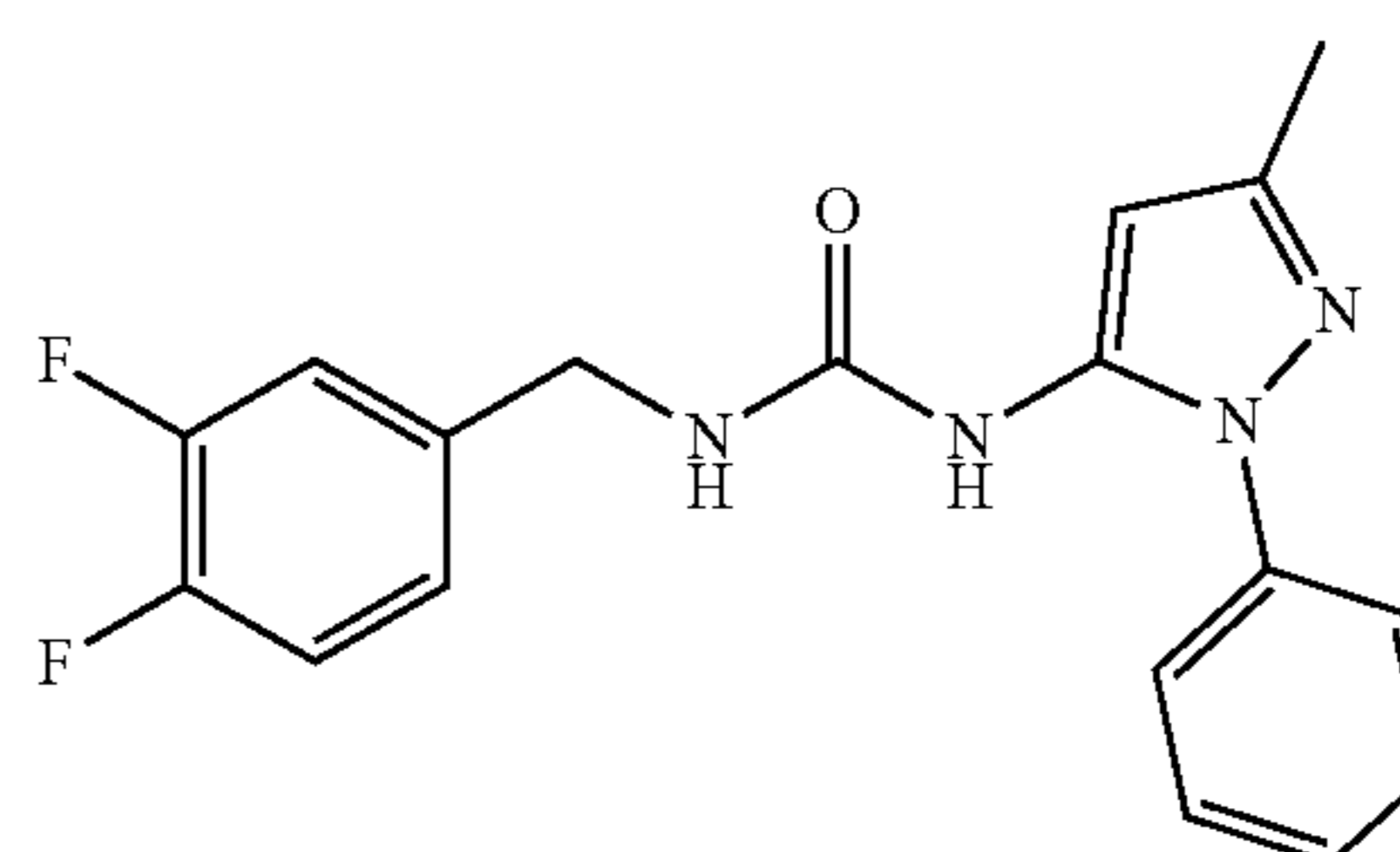
Molecular Weight: 342.35
