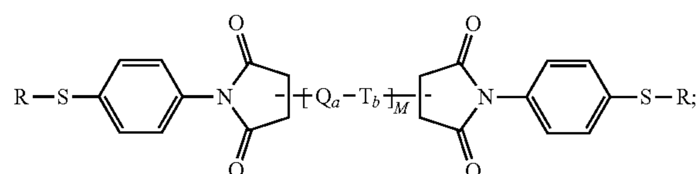
Structure XVII
