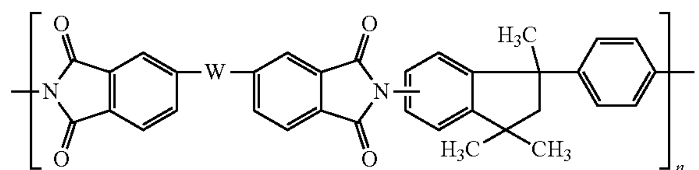
Structure IXa
