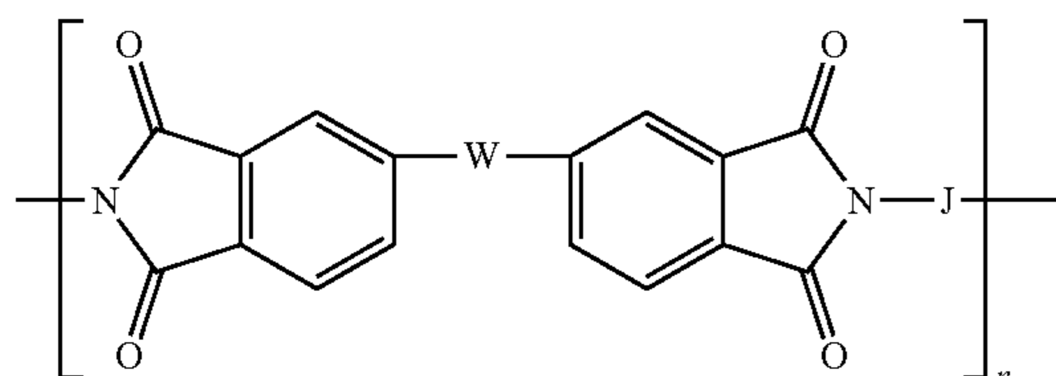
Structure III
