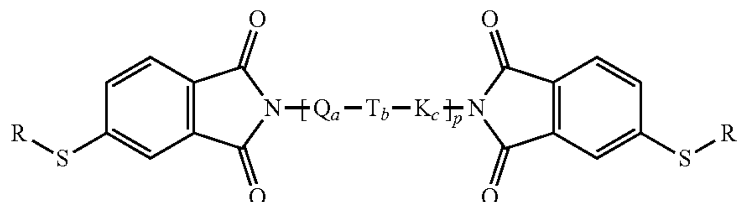
Structure XVIII
