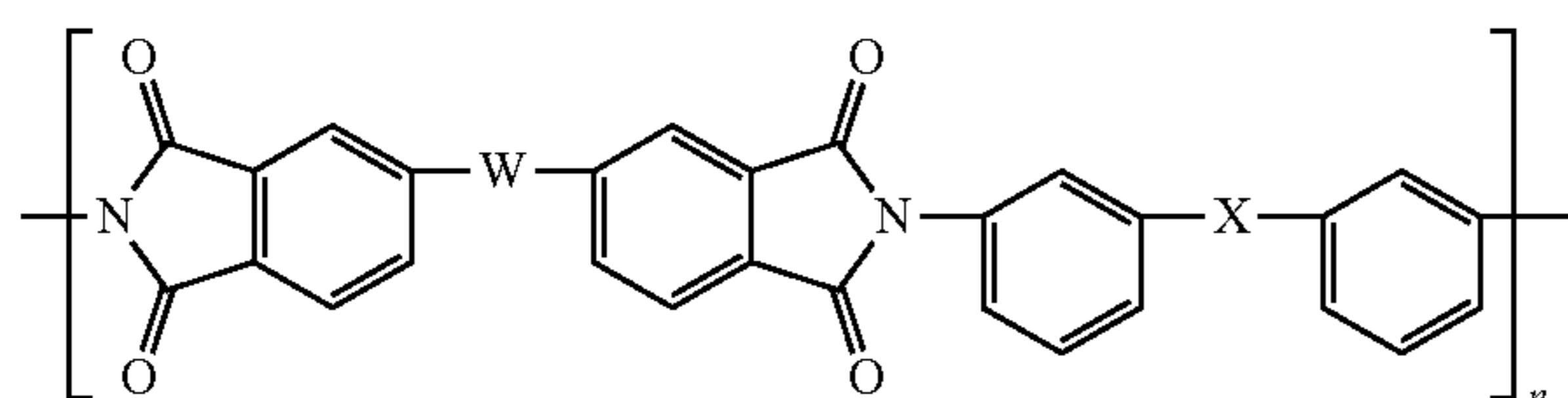
Structure IXb
