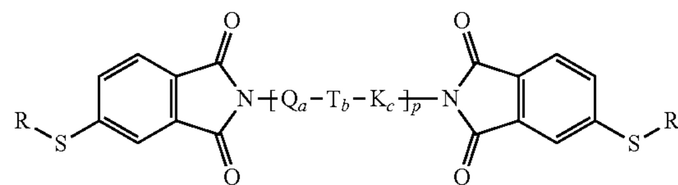
Structure XIX
