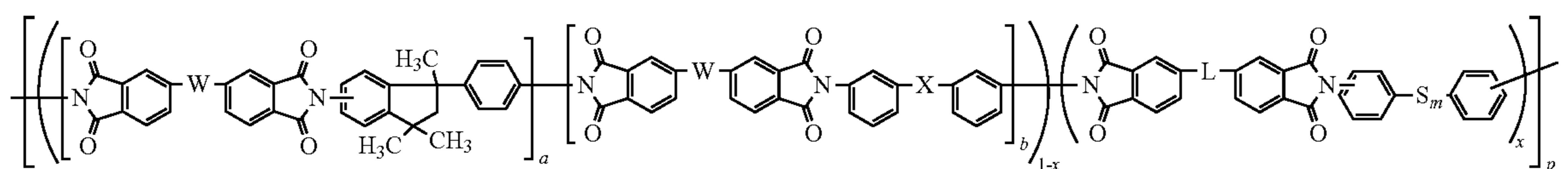
Structure XIIIa
