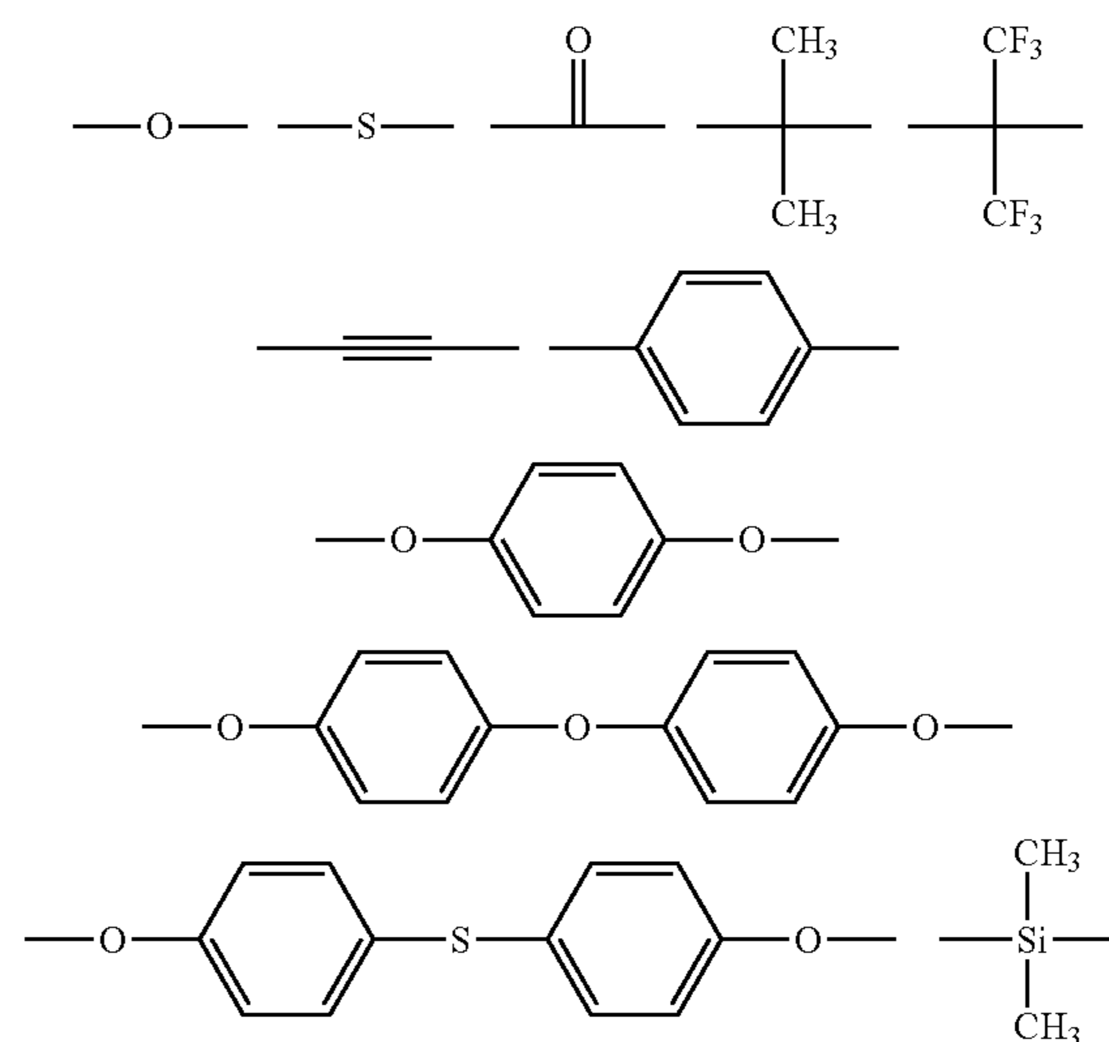
Structure XI
