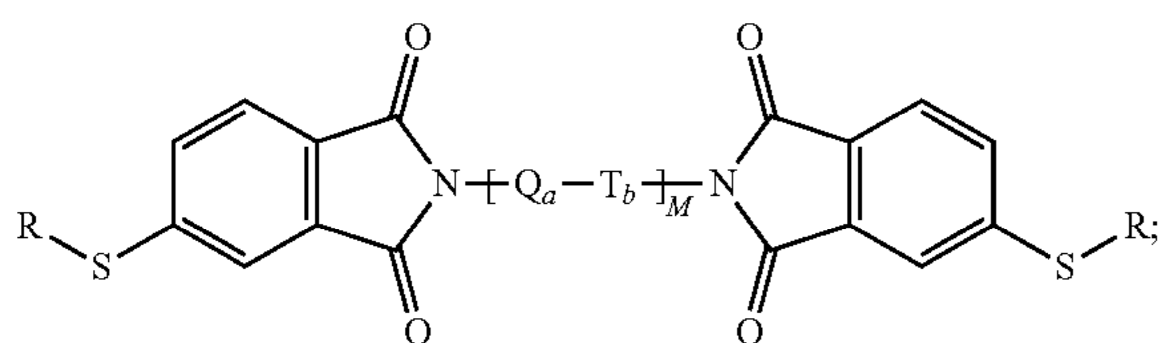
Structure XI
