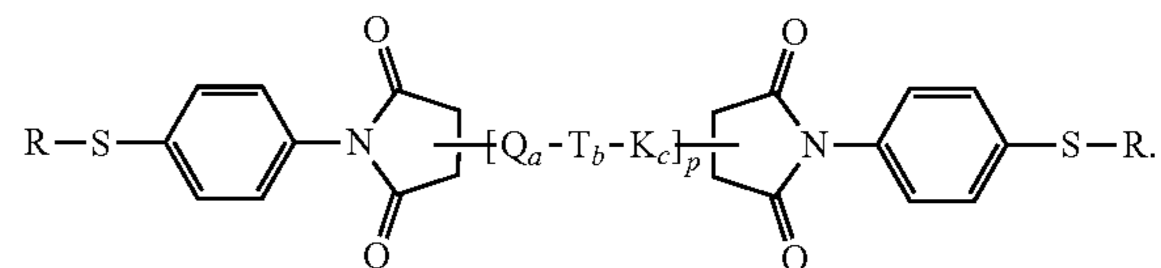
Structure XIX
