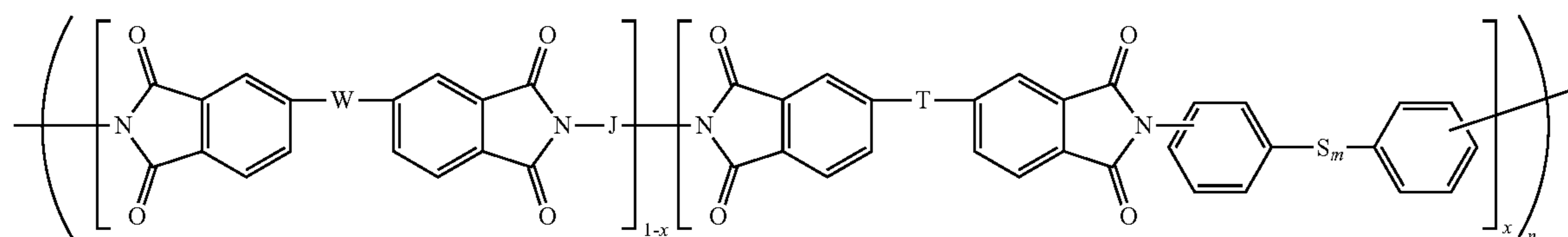
Structure V
