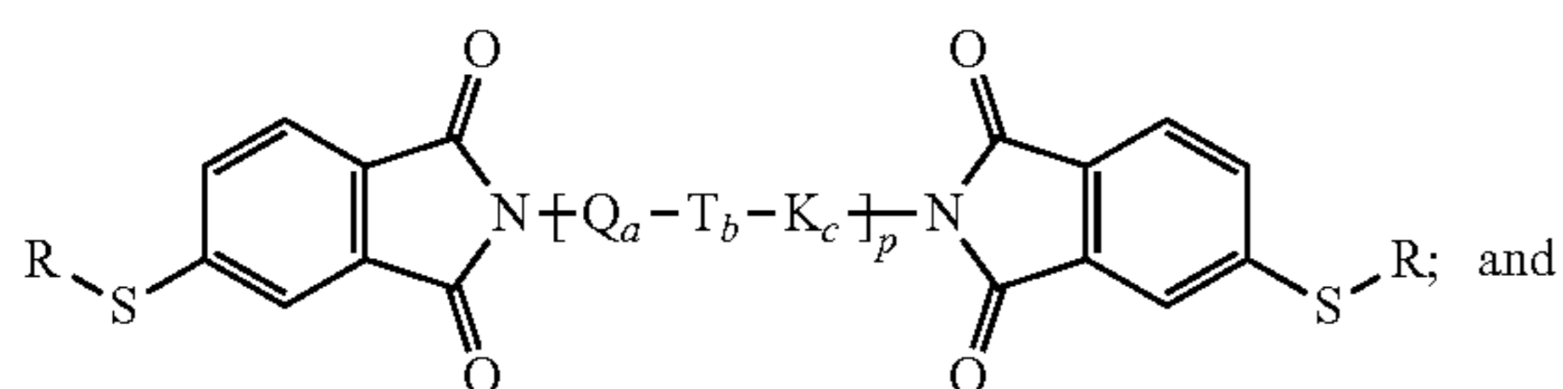
Structure XIII
