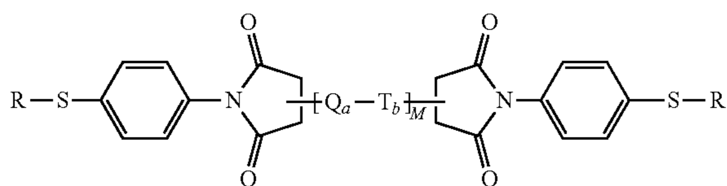
Structure XI
