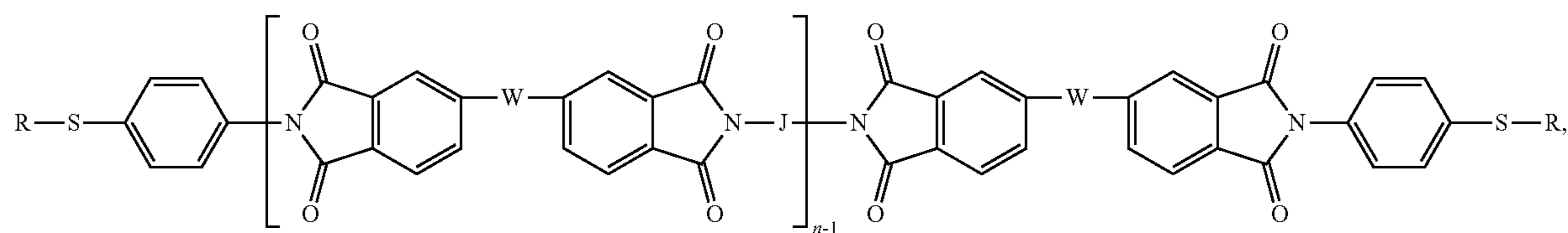
Structure IX
