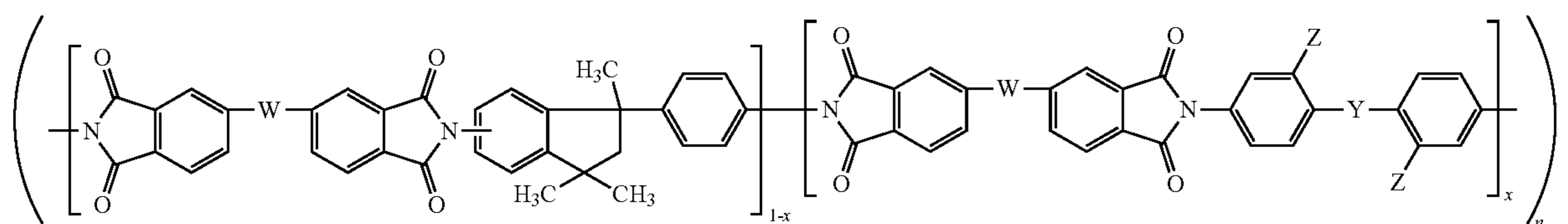
Structure Xb
