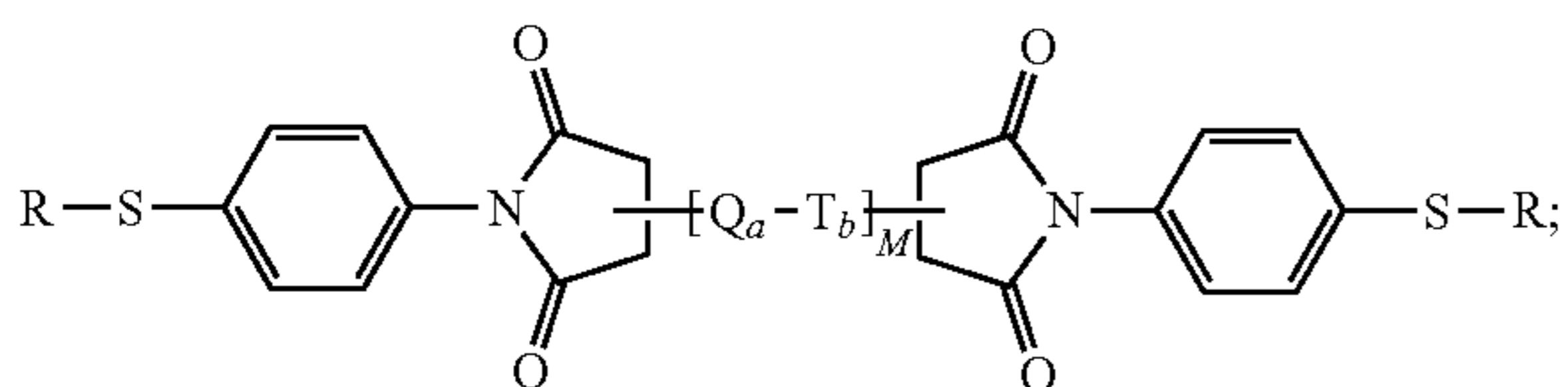
Structure XVII
