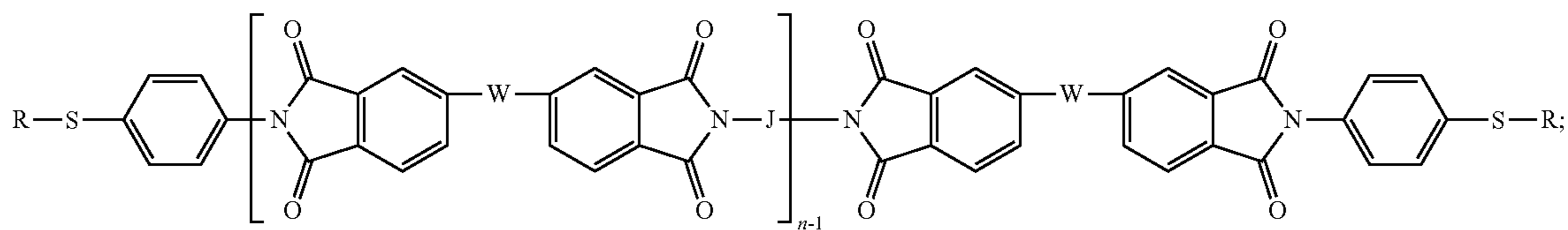
Structure XV
