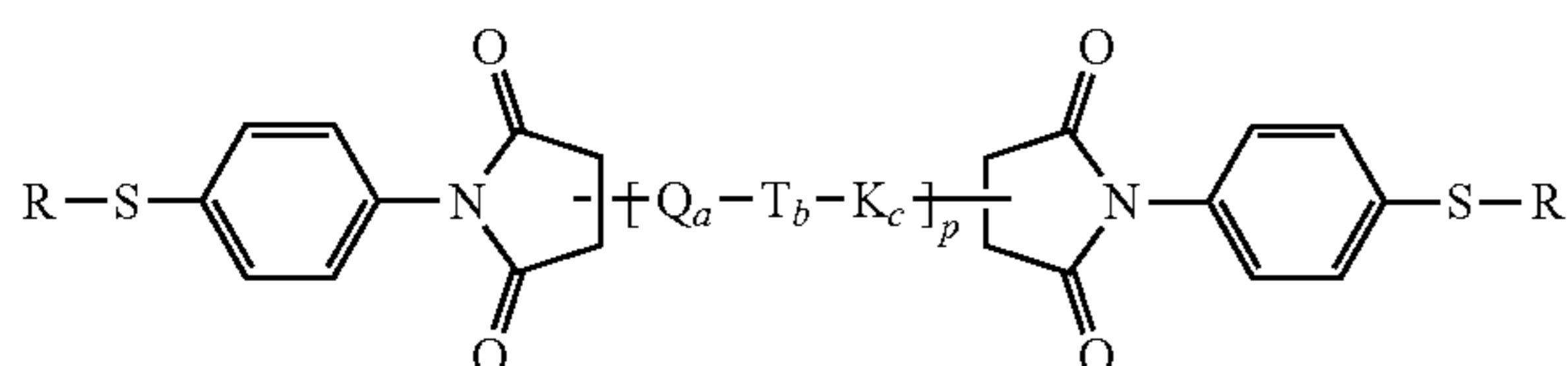
Structure XIII
