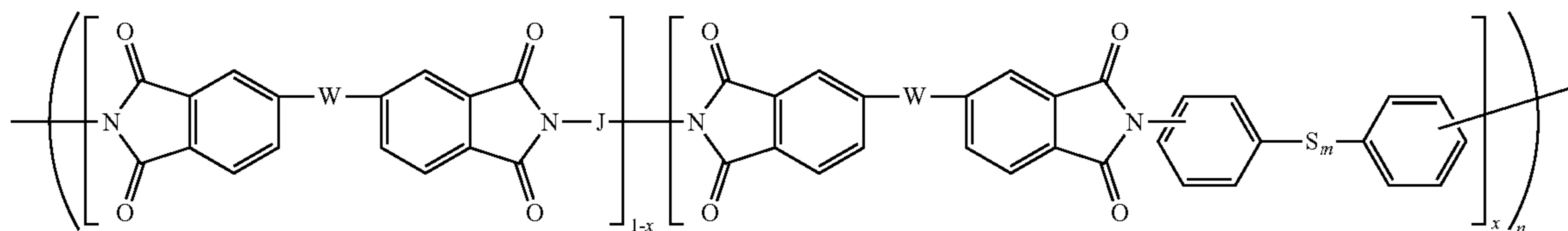
Structure XII
