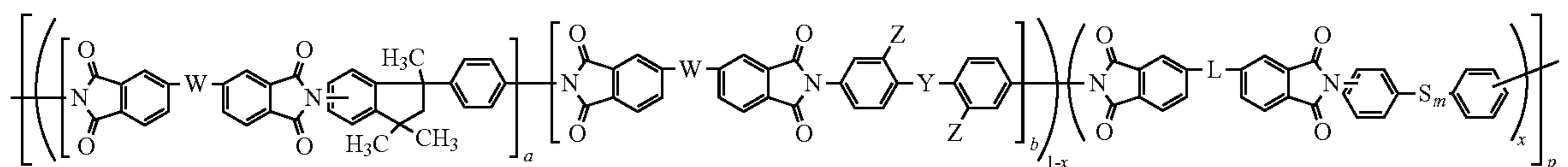
Structure XIIIb
