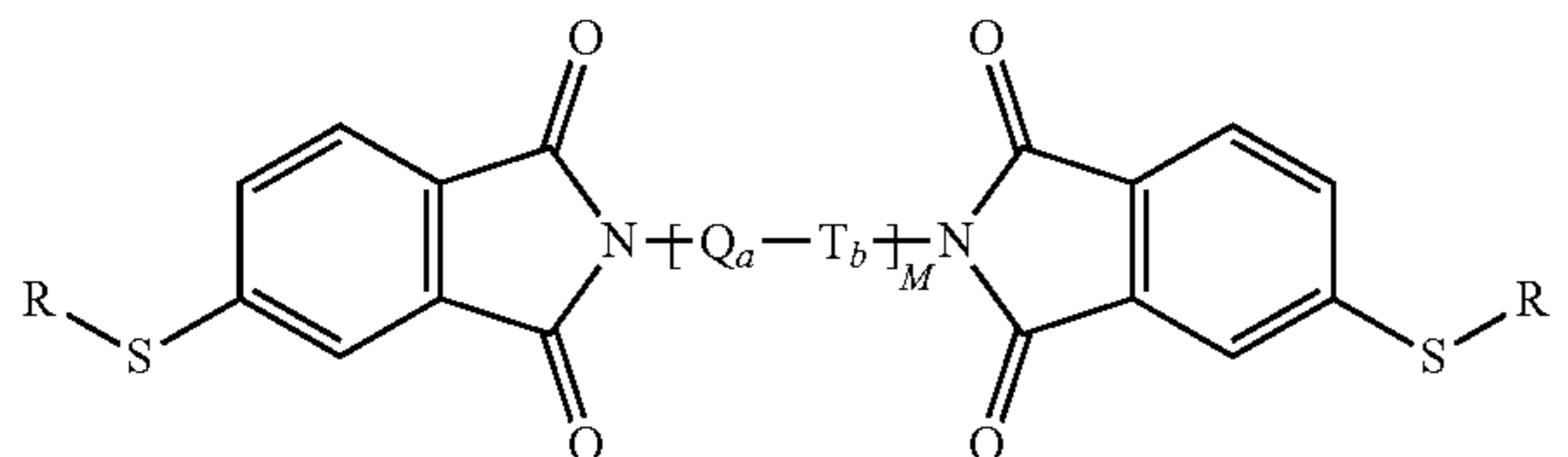
Structure XVII
