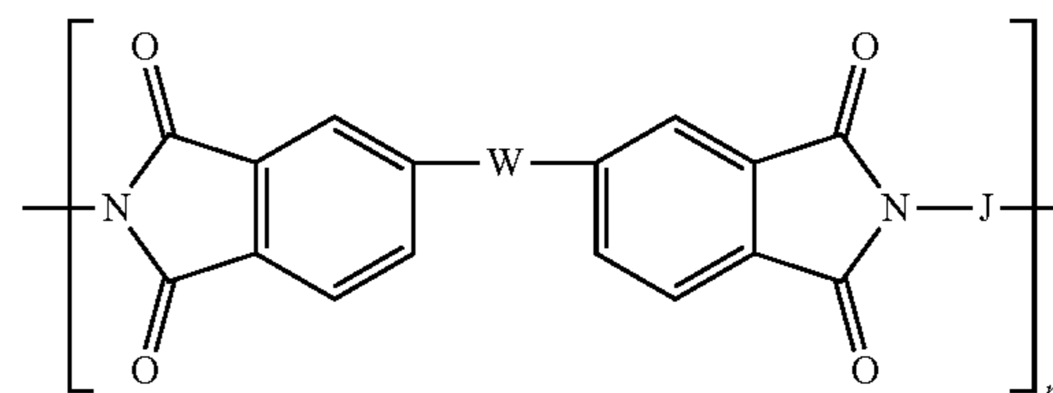
Structure VII
