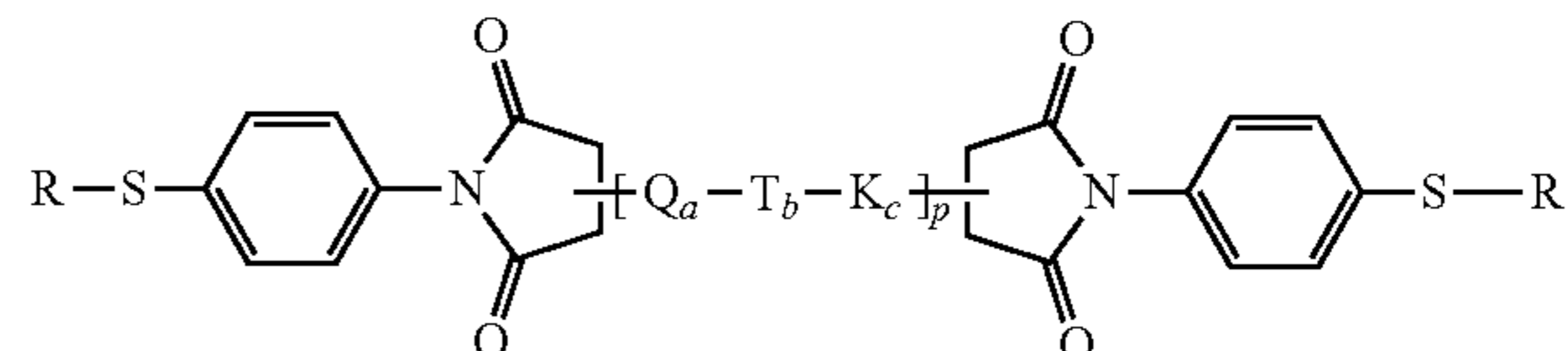
Structure XIX
