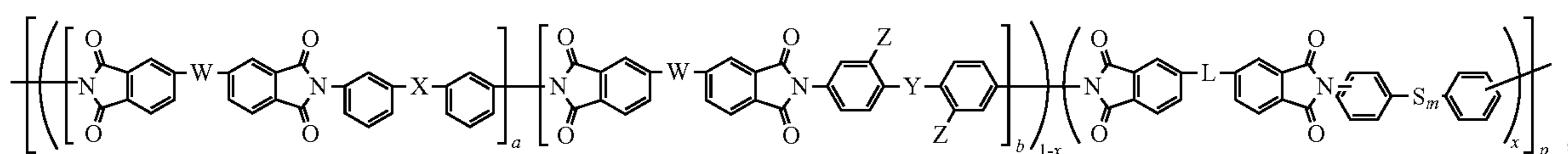
Structure XIIIc
