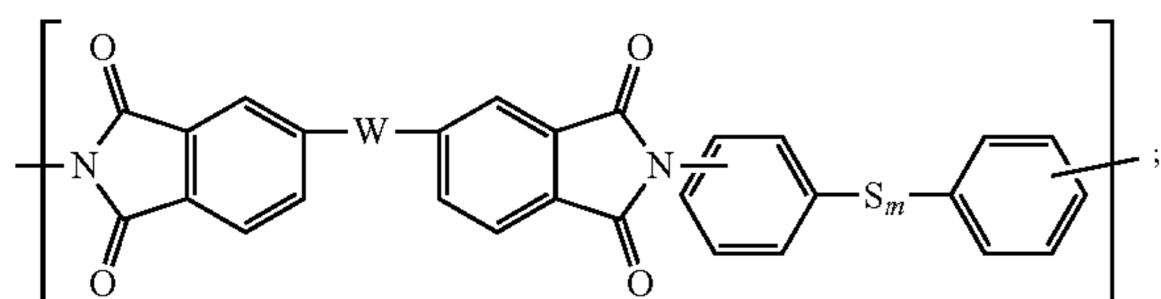
Structure XI
